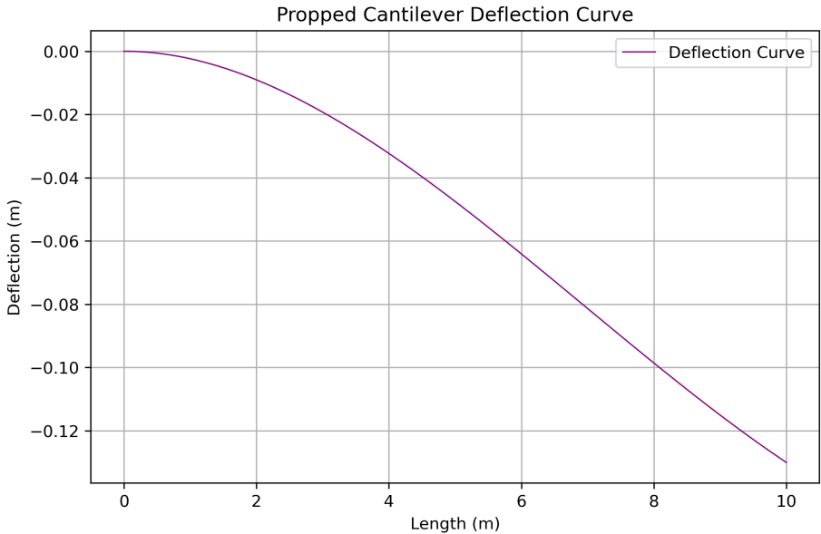
Fig. 1.2.12.1. Propped cantilever and support settlement.
