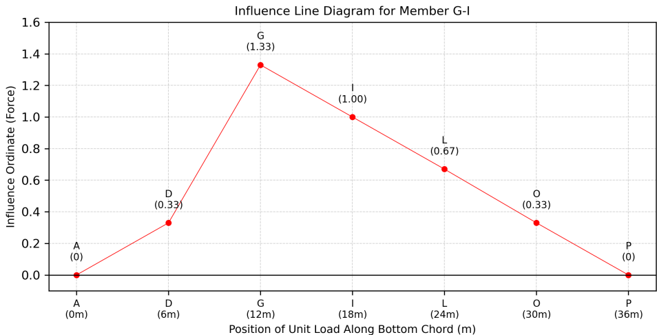
Fig. 1.2.8.2. Correct influence line for axial force in member G - I .
