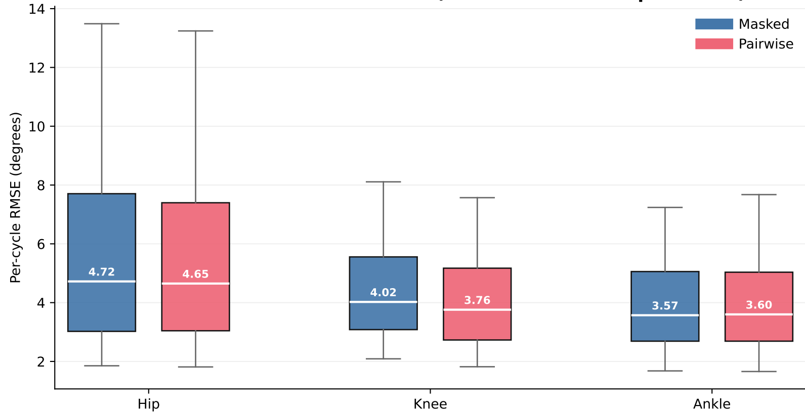
Out-of-fold reconstruction error (whiskers: 5th-95th percentile)
