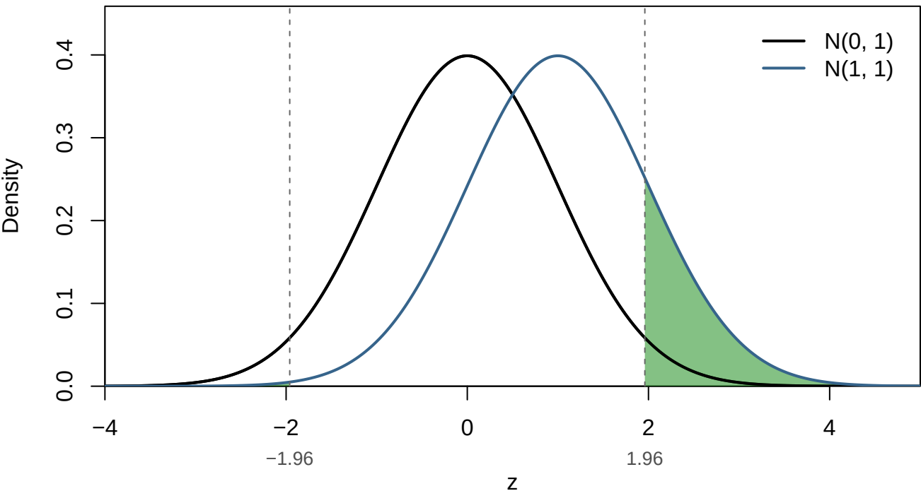
Standard Normal vs. N(1, 1)
