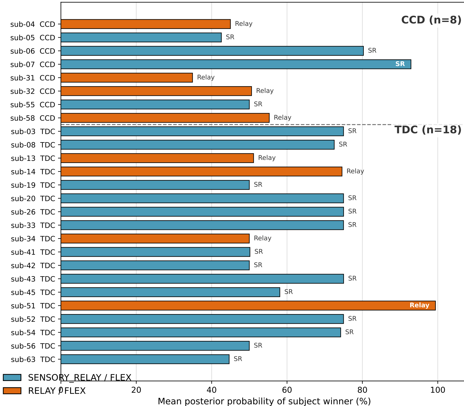
Subject-level winner and confidence
