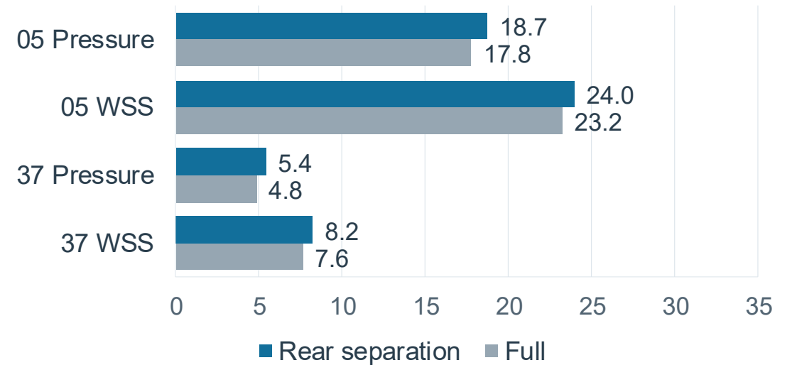
Surface relative L_2 error (%)
