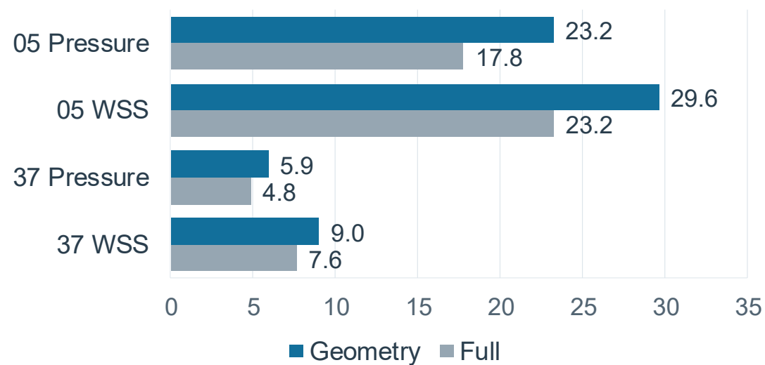
Surface relative L_2 error (%)
