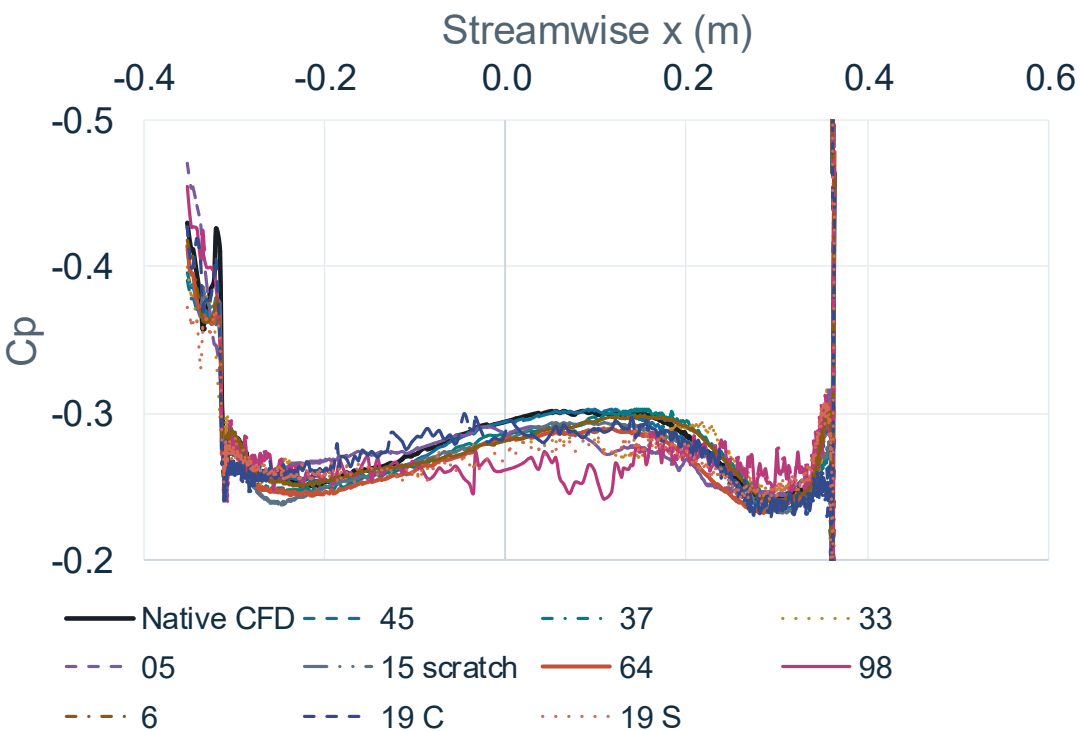
Front-left wheelhouse, y = -0.6 m
