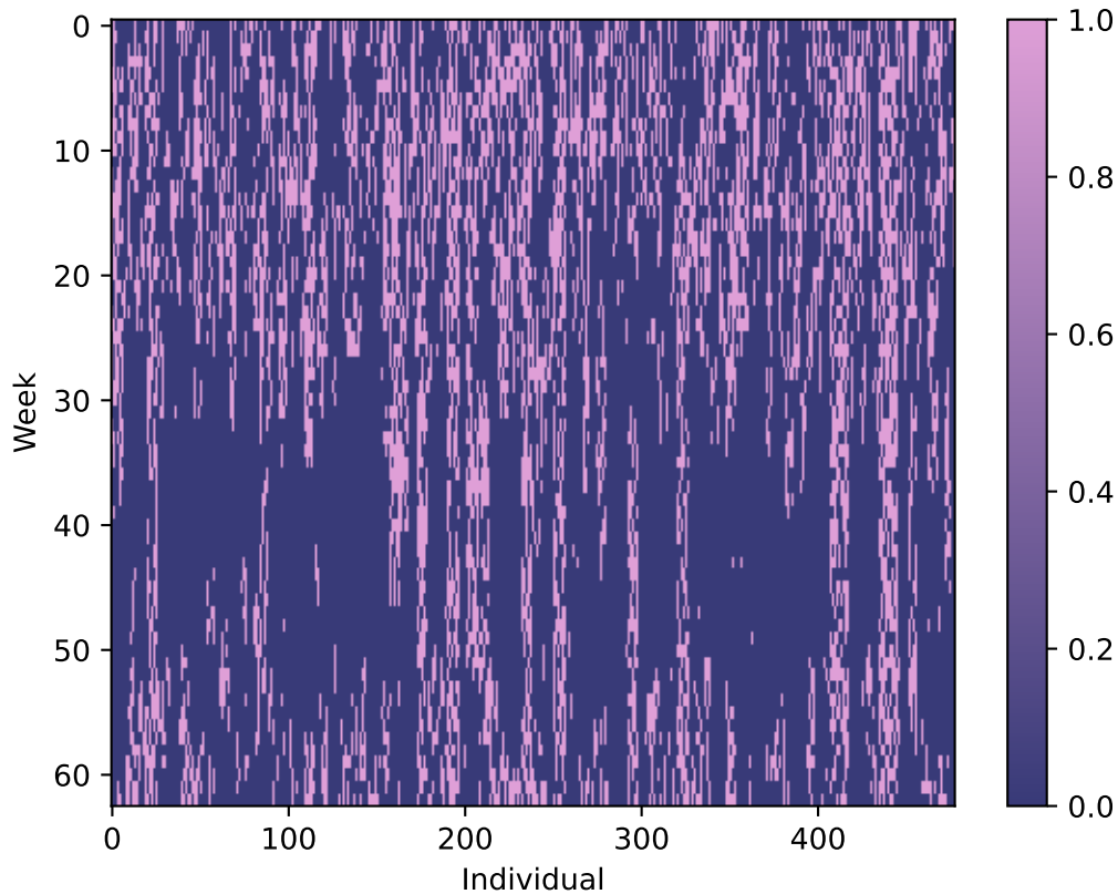
Simulated E. Coli Transmission
