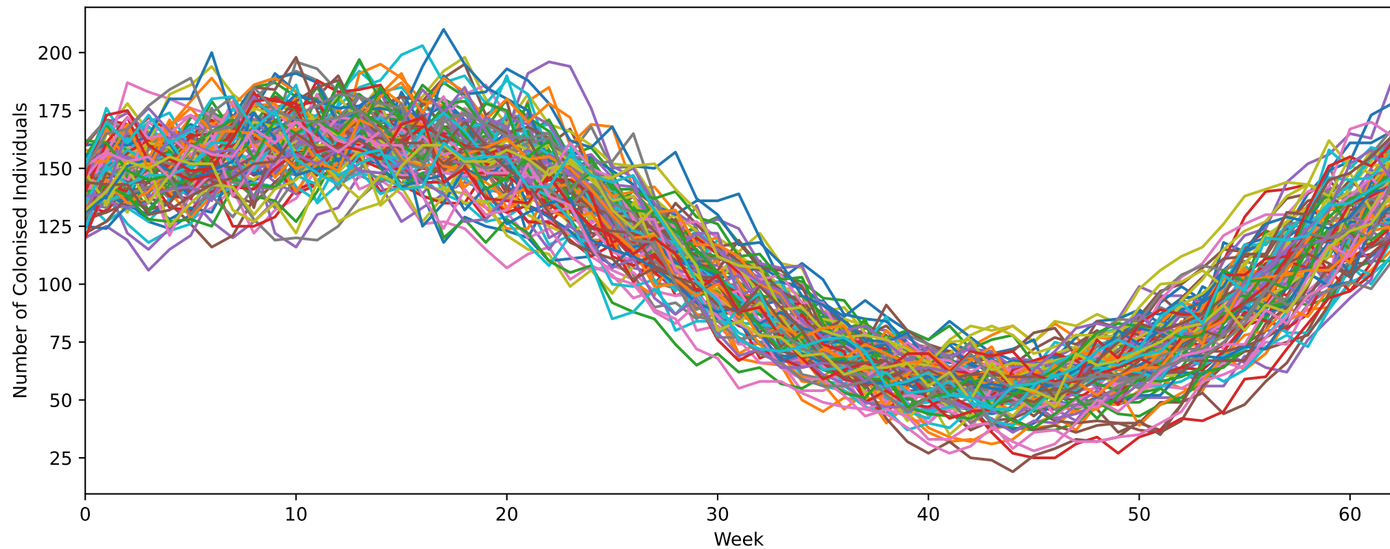
Total Number of Colonised Individuals over Time
