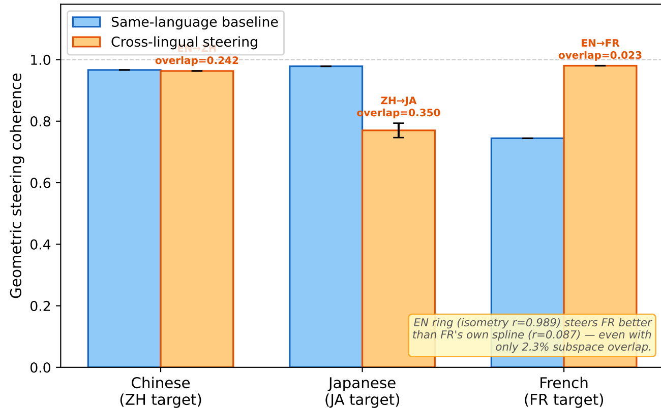
Cross-lingual steering coherence vs same-language baseline (Llama 3.1 8B · weekday arithmetic · Layer 28 last-token · geometric paths)
