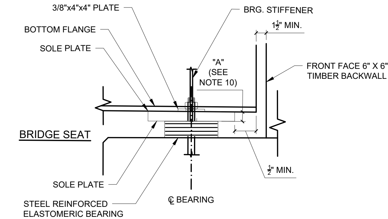
TYPICAL FIXED BEARING ELEVATION
