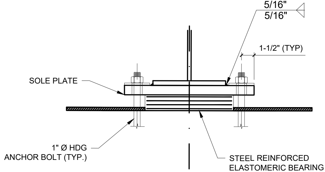
TYPICAL FIXED BEARING SECTION
