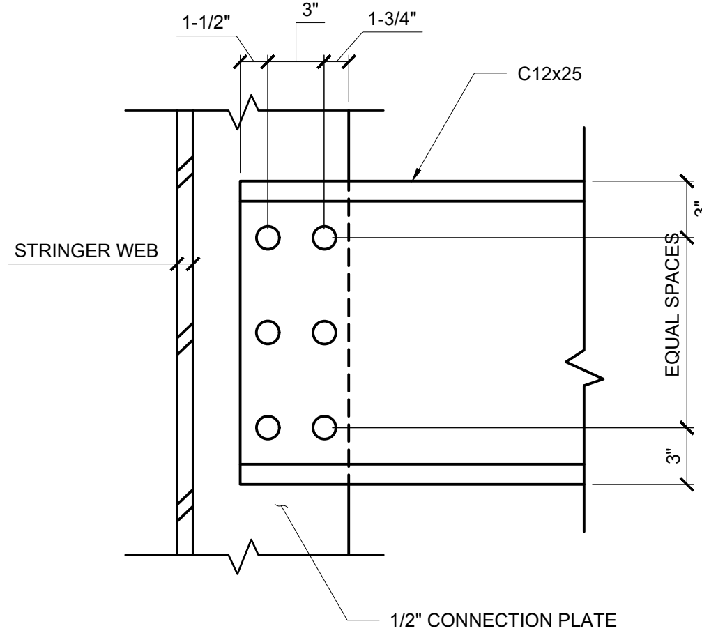
DIAPHRAGM CONNECTION DETAIL SCALE: NOT TO SCALE
