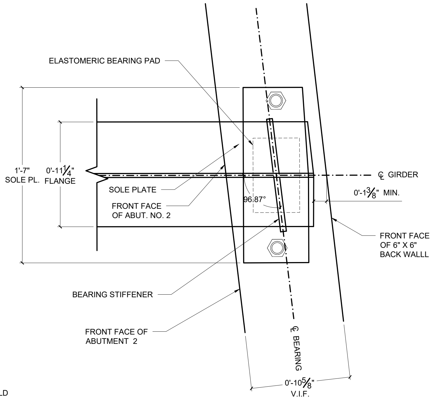
TYPICAL FIXED BEARING PLAN
