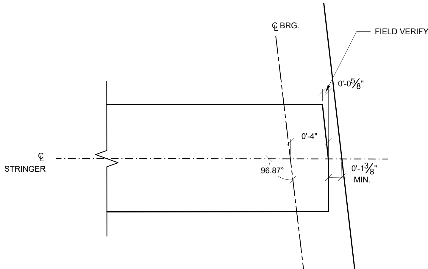
B - TYP. CLIPPING DETAIL @ ABUT. 2 SCALE: 2" = 1'
