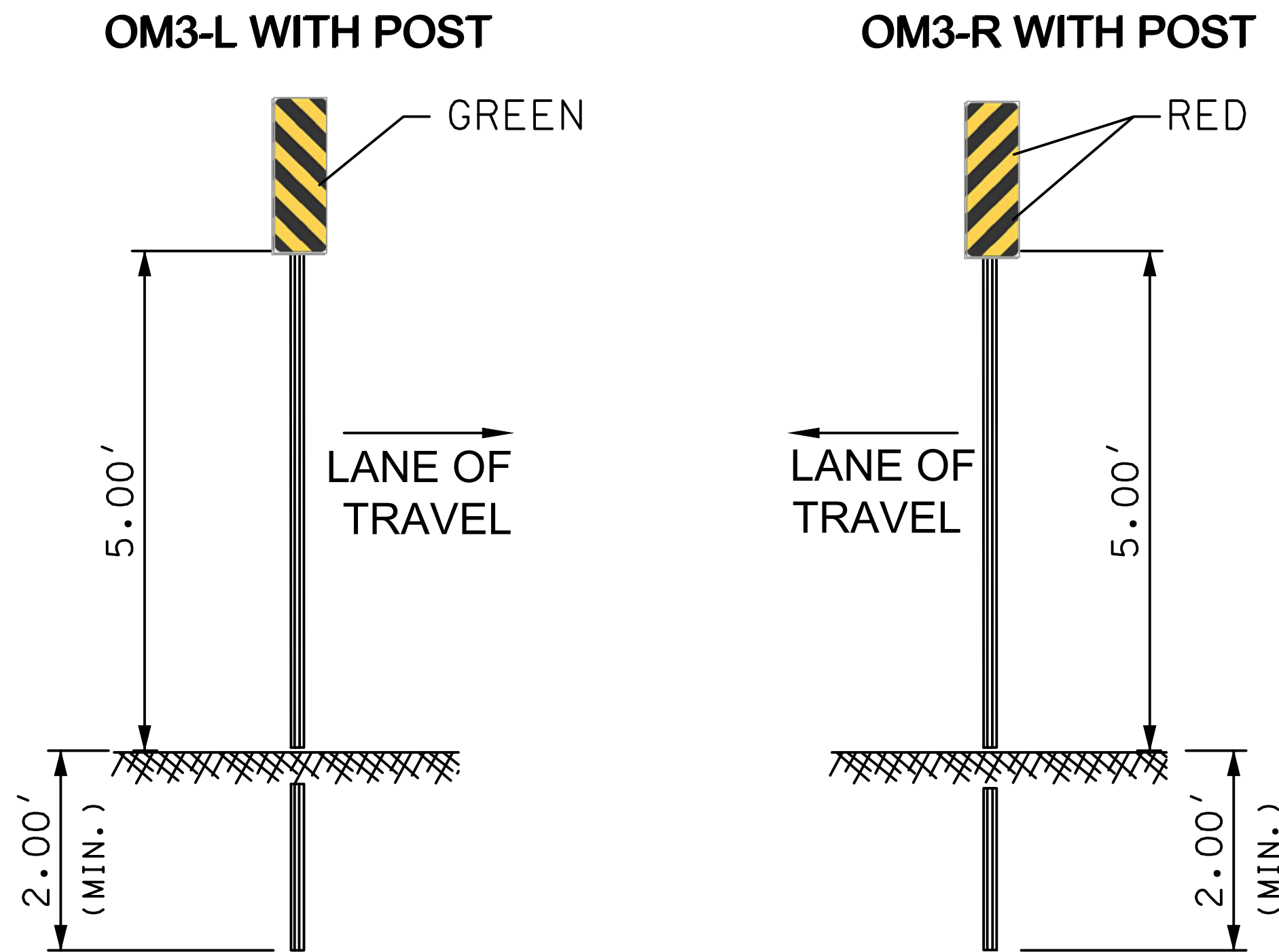
TYPICAL INSTALLATION
