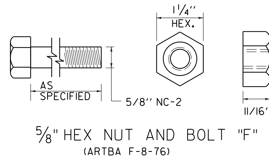
FASTENER DETAILS
