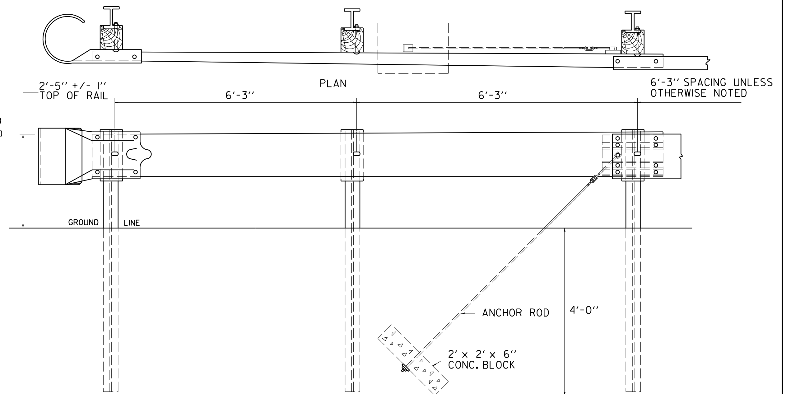
ASSEMBLY ELEVATION
