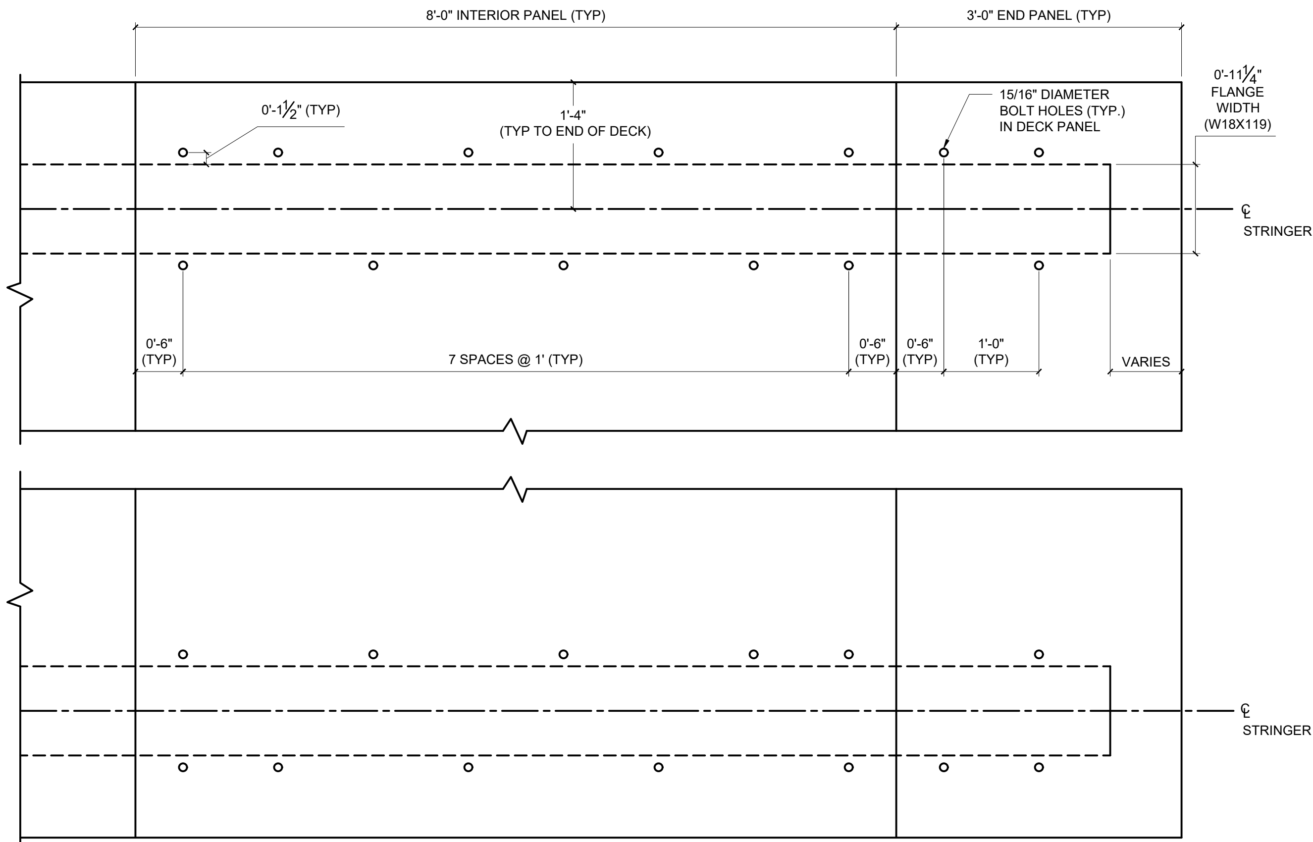
DECK TO GIRDER CONNECTION PLAN
