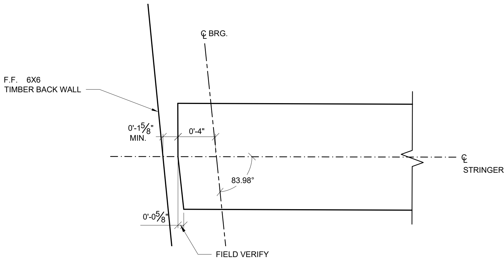
A - TYP. CLIPPING DETAIL @ ABUT. 1 SCALE: 2" = 1'
