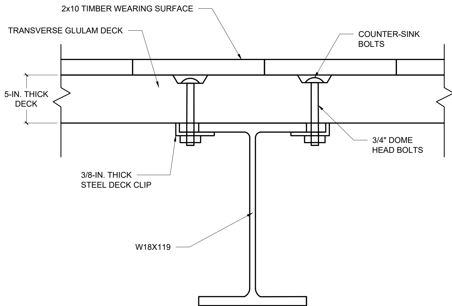
DECK TO GIRDER CONNECTION DETAIL NOT TO SCALE
