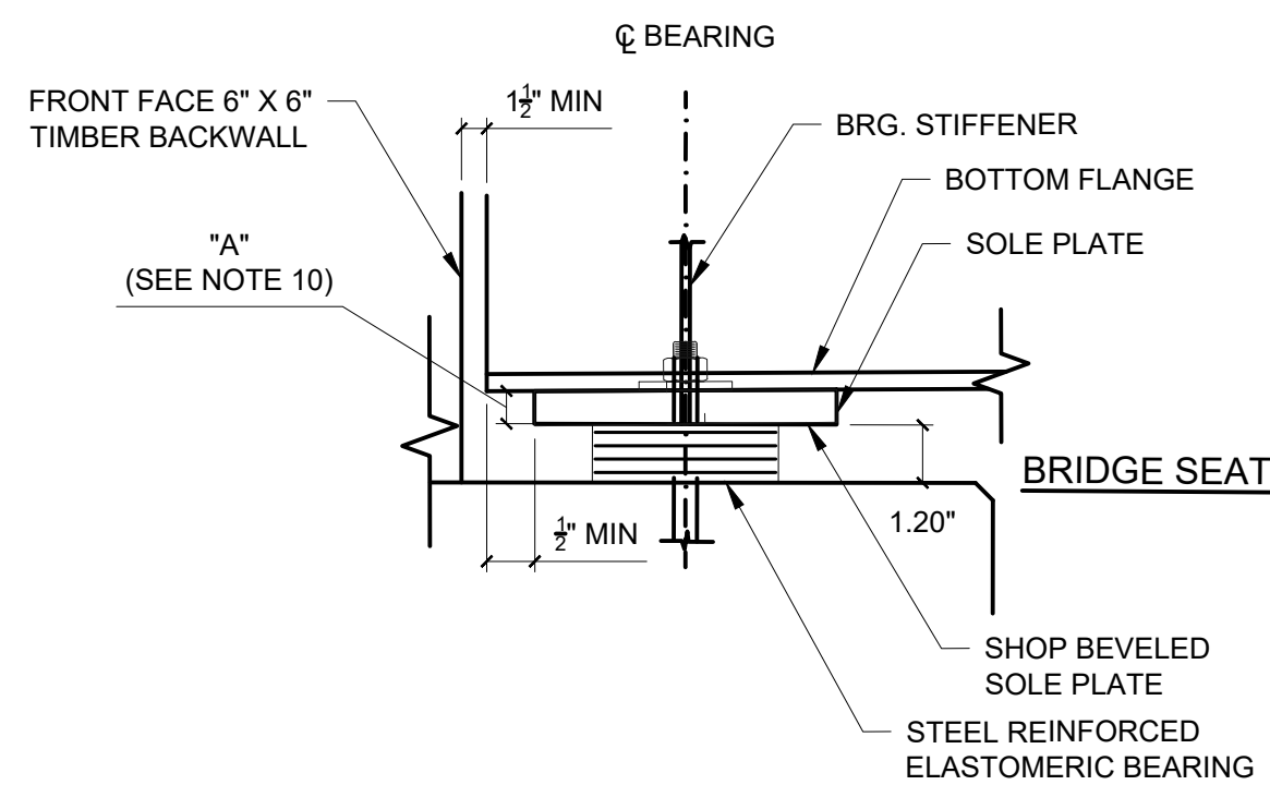
TYPICAL EXPANSION BEARING ELEVATION
