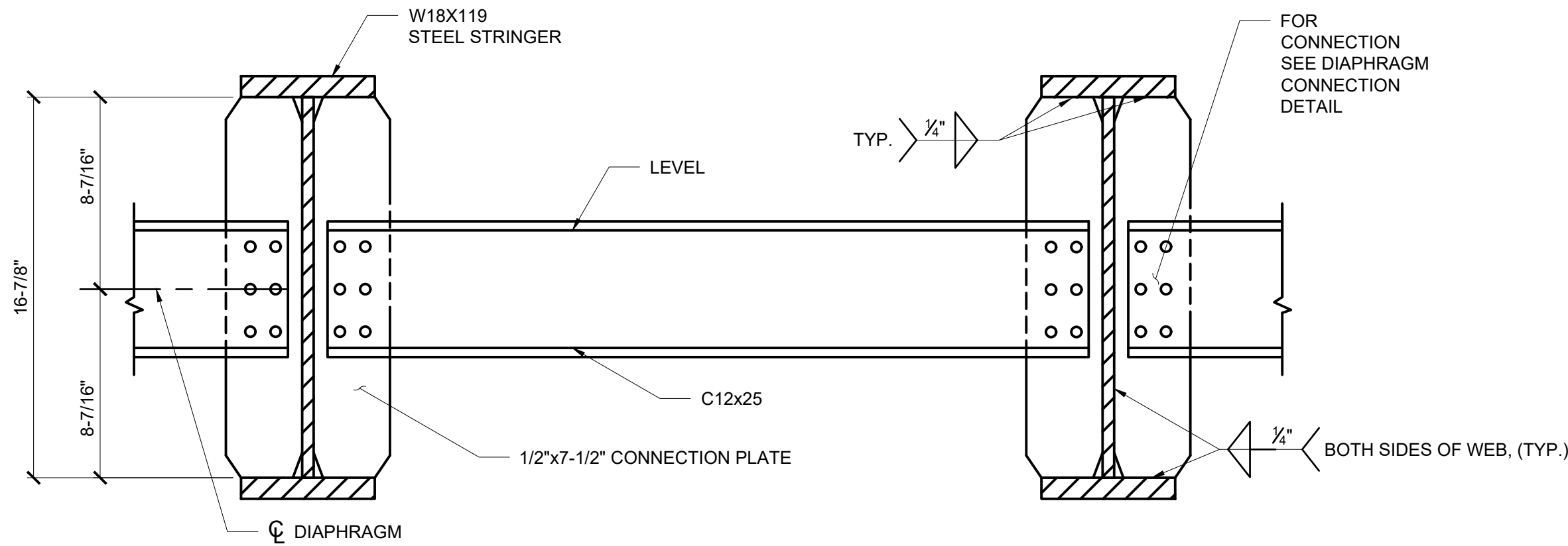
DIAPHRAGM DETAIL SCALE: NOT TO SCALE
