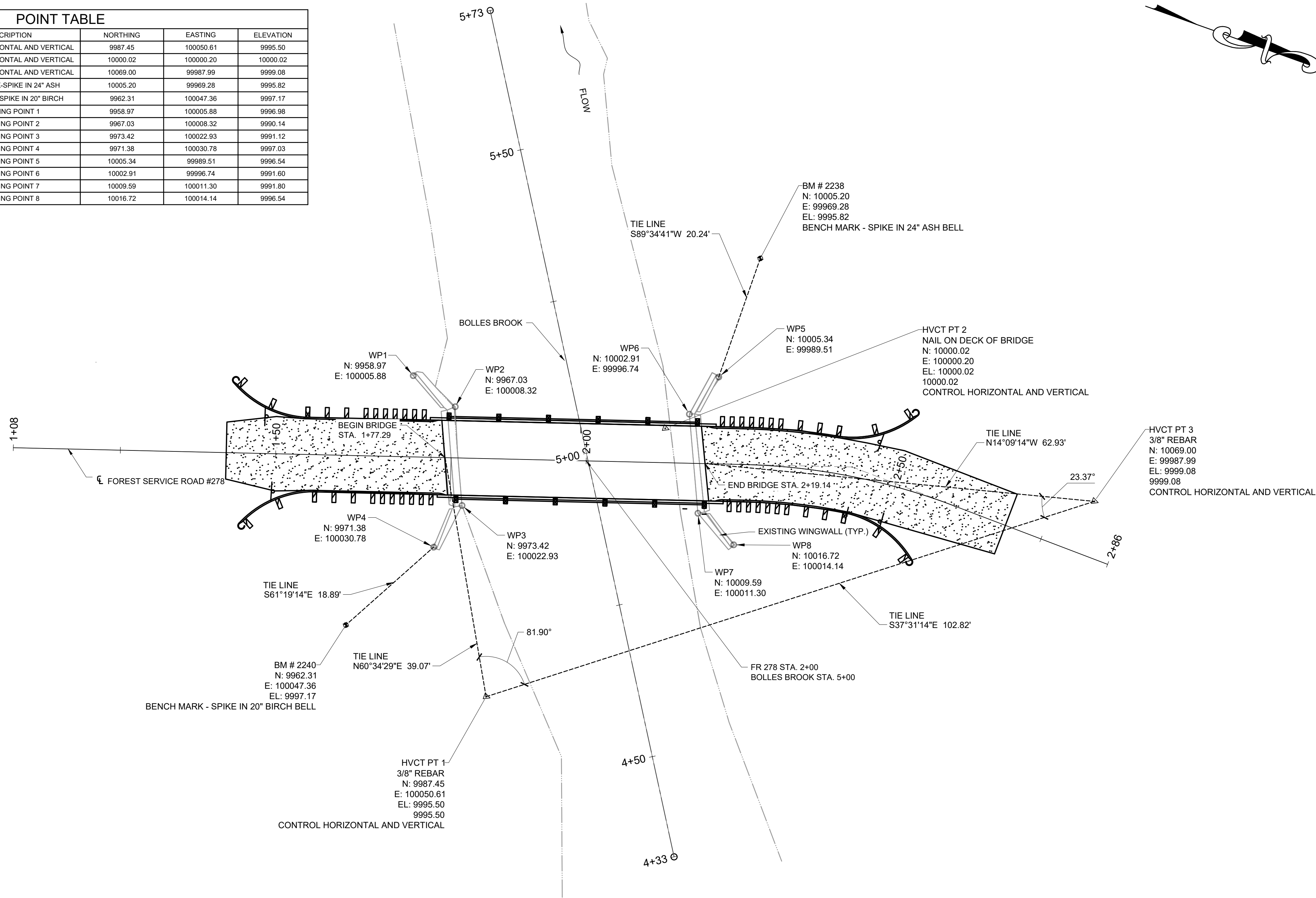
SURVEY TIE PLAN
