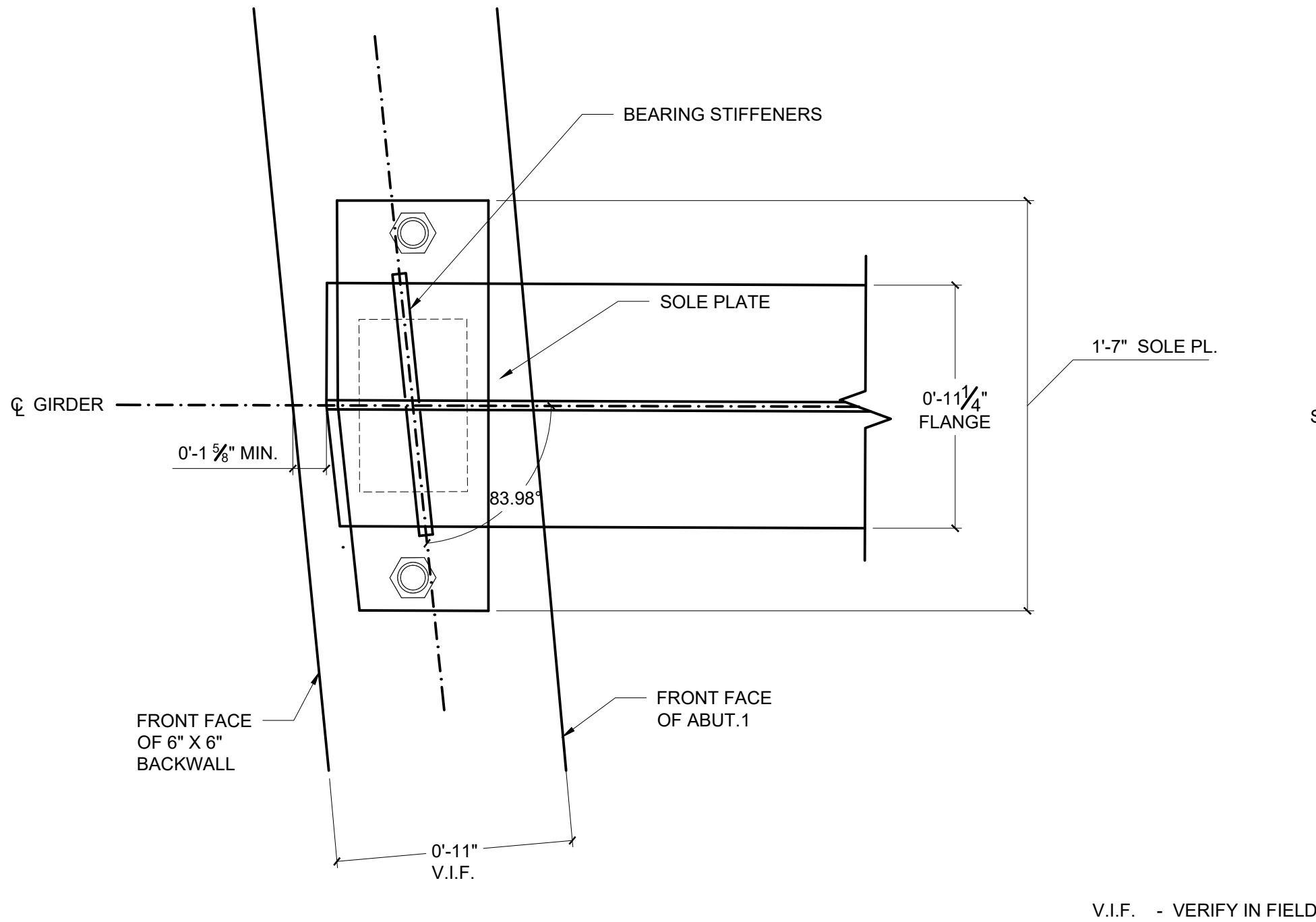
TYPICAL EXPANSION BEARING PLAN
