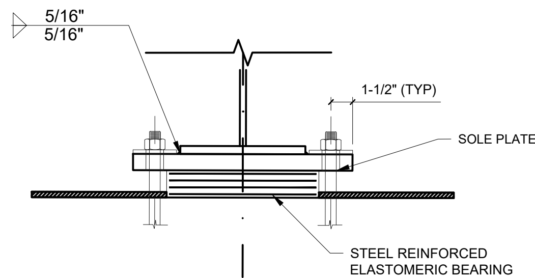
TYPICAL EXPANSION BEARING SECTION
