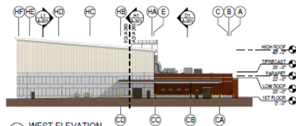
F1 WEST ELEVATION SCALE: 1" = 30'-0"
