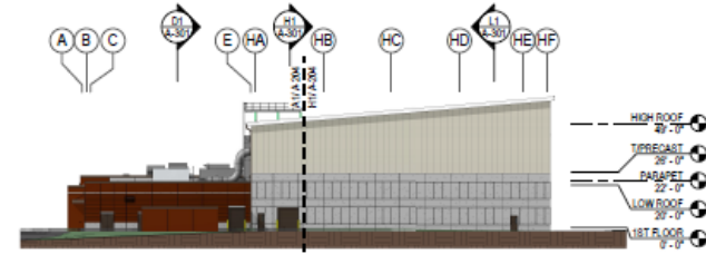
F10 EAST ELEVATION SCALE: 1" = 30'-0"
