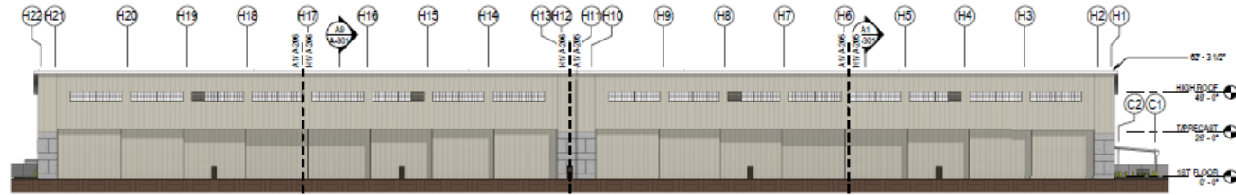
K1 NORTH ELEVATION SCALE: 1" = 30'-0"
