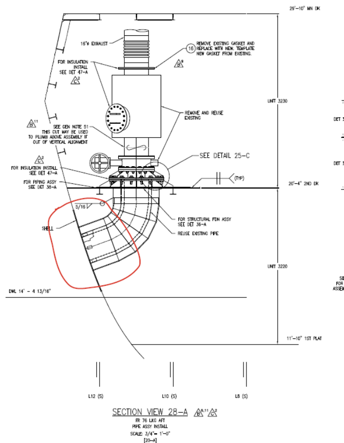
Figure 1 - Excerpt from CG Drawing 750-WMSL-259-505.
