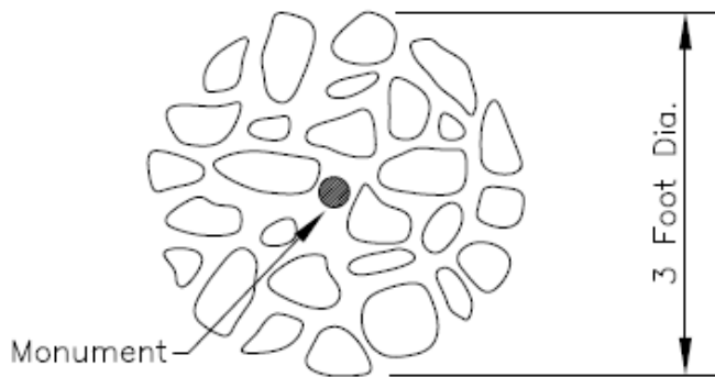
Monument w/Mound of Stone – Typical PLAN VIEW
