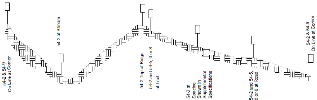
EXAMPLE PROFILE OF BOUNDARY LINE SHOWING SIGN PLACEMENT
