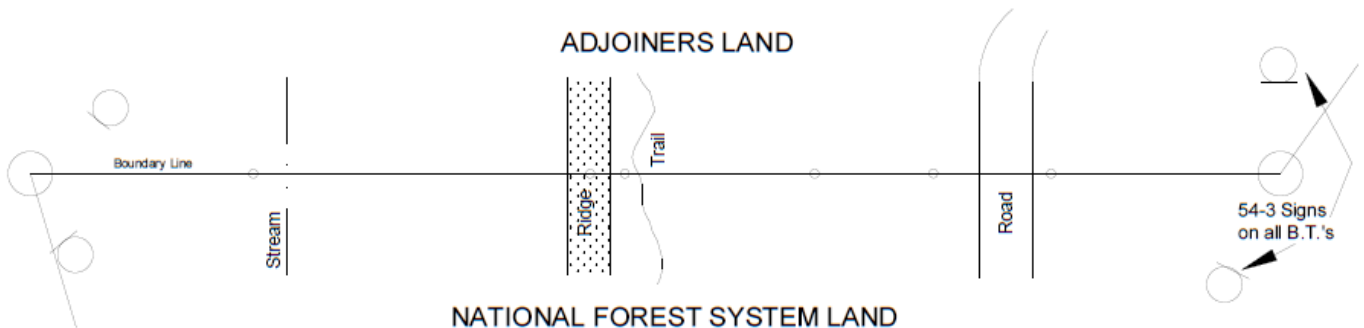
EXAMPLE PLAN VIEW OF BOUNDARY LINE SHOWING SIGN PLACEMENT
