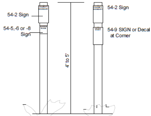
TYPICAL SIGN AND POST INSTALLATION
