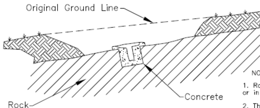
TYPICAL ROCK TABLET INSTALLATION
