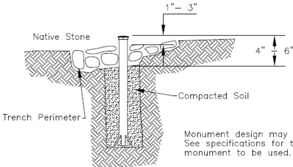
TYPICAL SECTION VIEW
