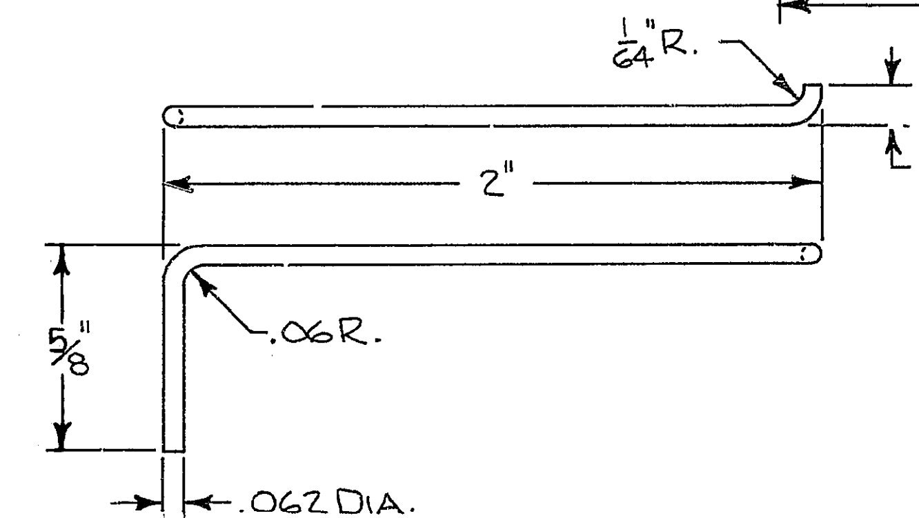
⑨ JUMPER. SCALE - 2/1.
