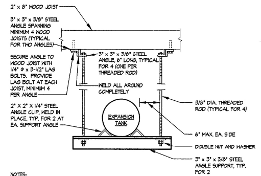
EXPANSION TANK MOUNTING DETAIL
