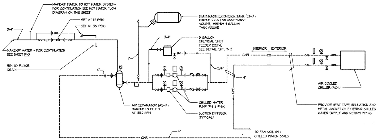
CHILLED WATER FLOW DIAGRAM
