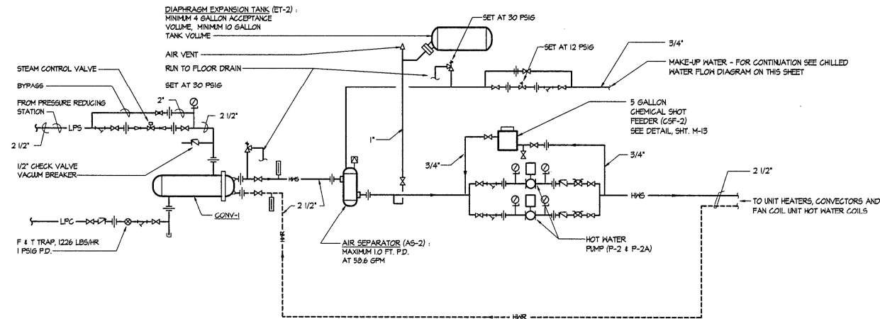
HOT WATER FLOW DIAGRAM
