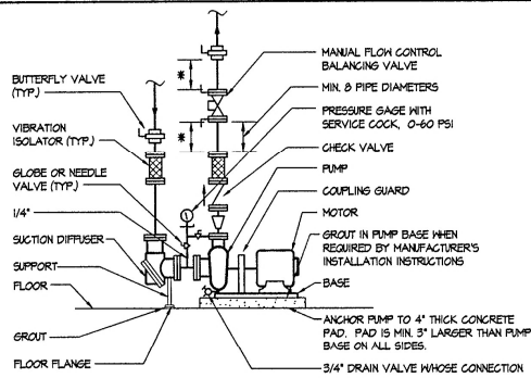
BASE MOUNTED CENTRIFUGAL PUMP DETAIL (P-1 & 1A) NO SCALE
