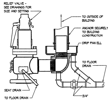
STEAM RELIEF VALVE DRIP PAN ELL NO SCALE
