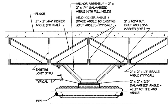
PIPE ANCHOR DETAIL NO SCALE
