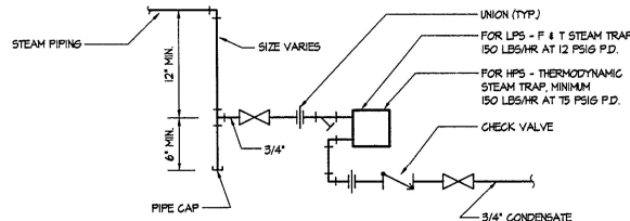
DRIP STATION DETAIL NO SCALE
