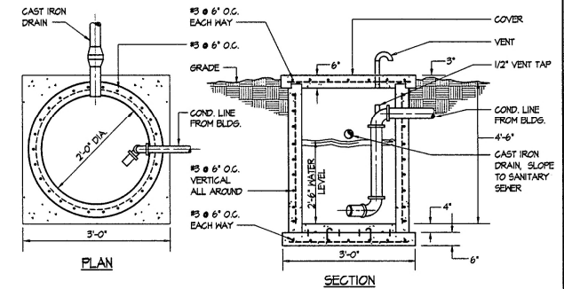
CONDENSATE COOLING WELL DETAIL NO SCALE
