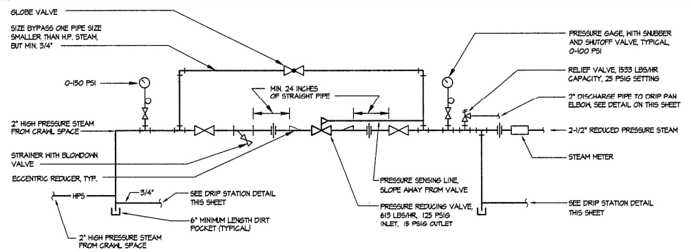
STEAM PRESSURE REDUCING STATION DETAIL NO SCALE
