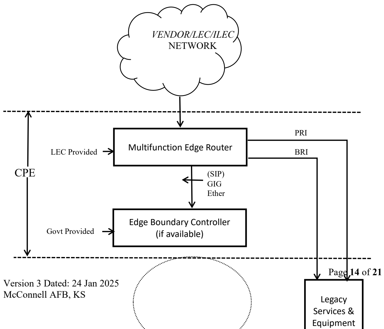
Diagram 2 EXAMPLE OF SIP VENDOR PROVIDED
