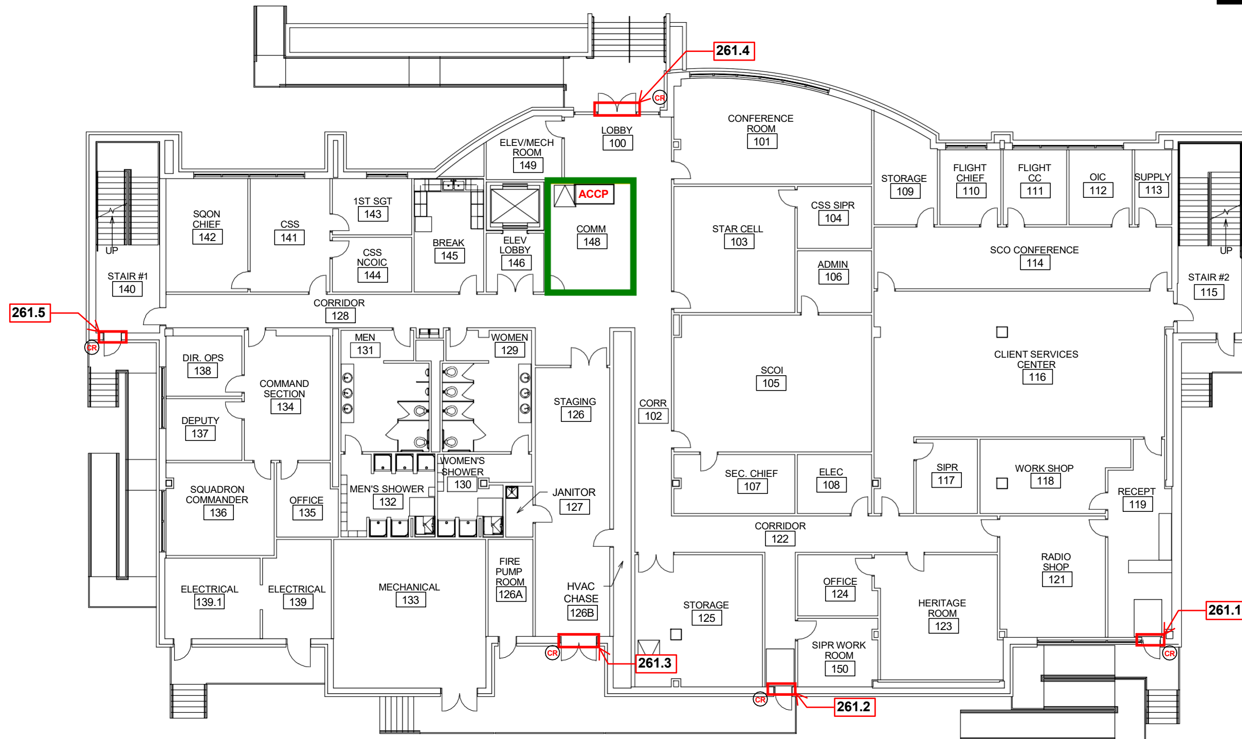
1ST FLOOR PLAN - BLDG 261
