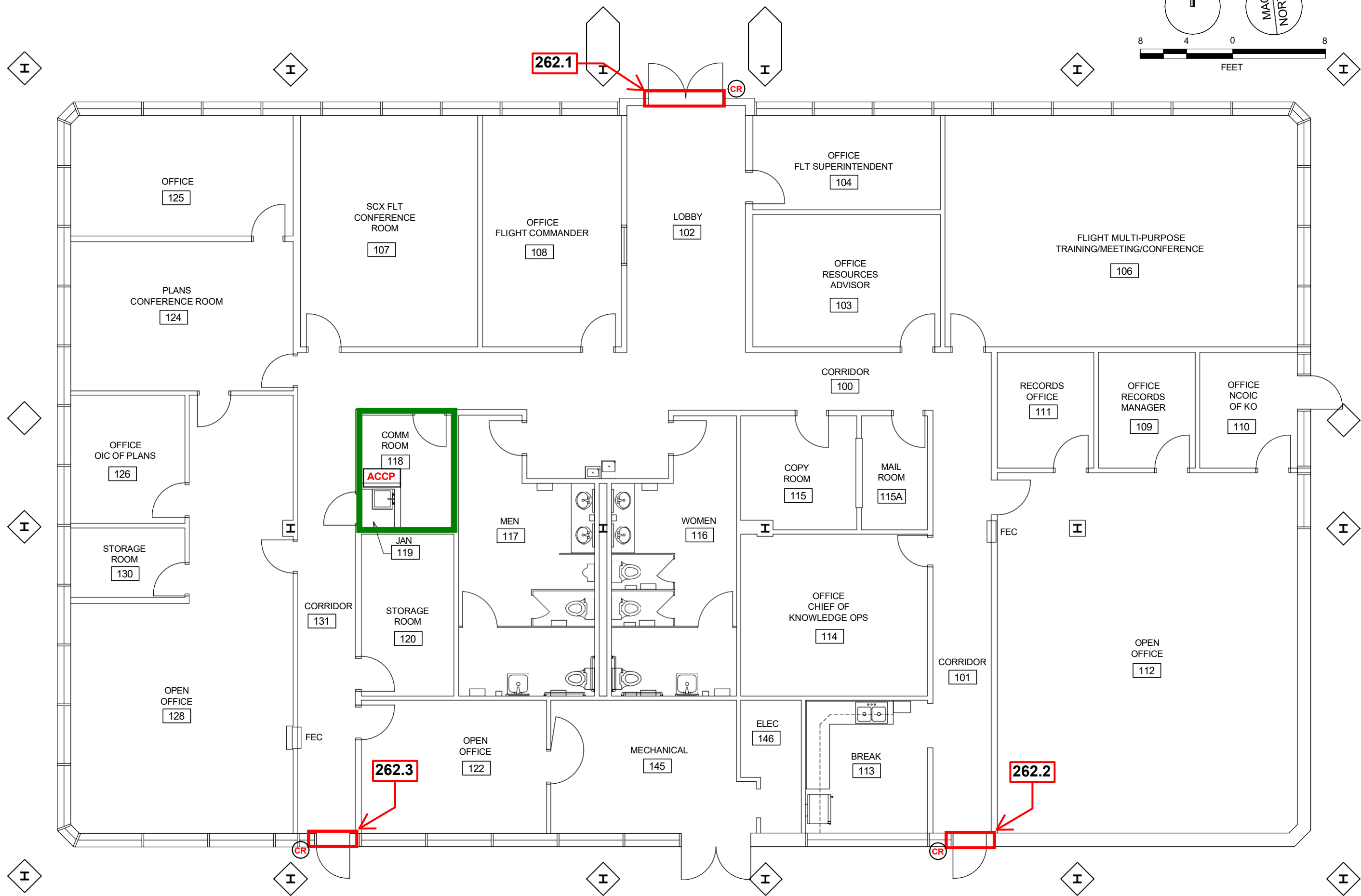
B262 - FLOOR PLAN SCALE: 1/8" = 1'-0"
