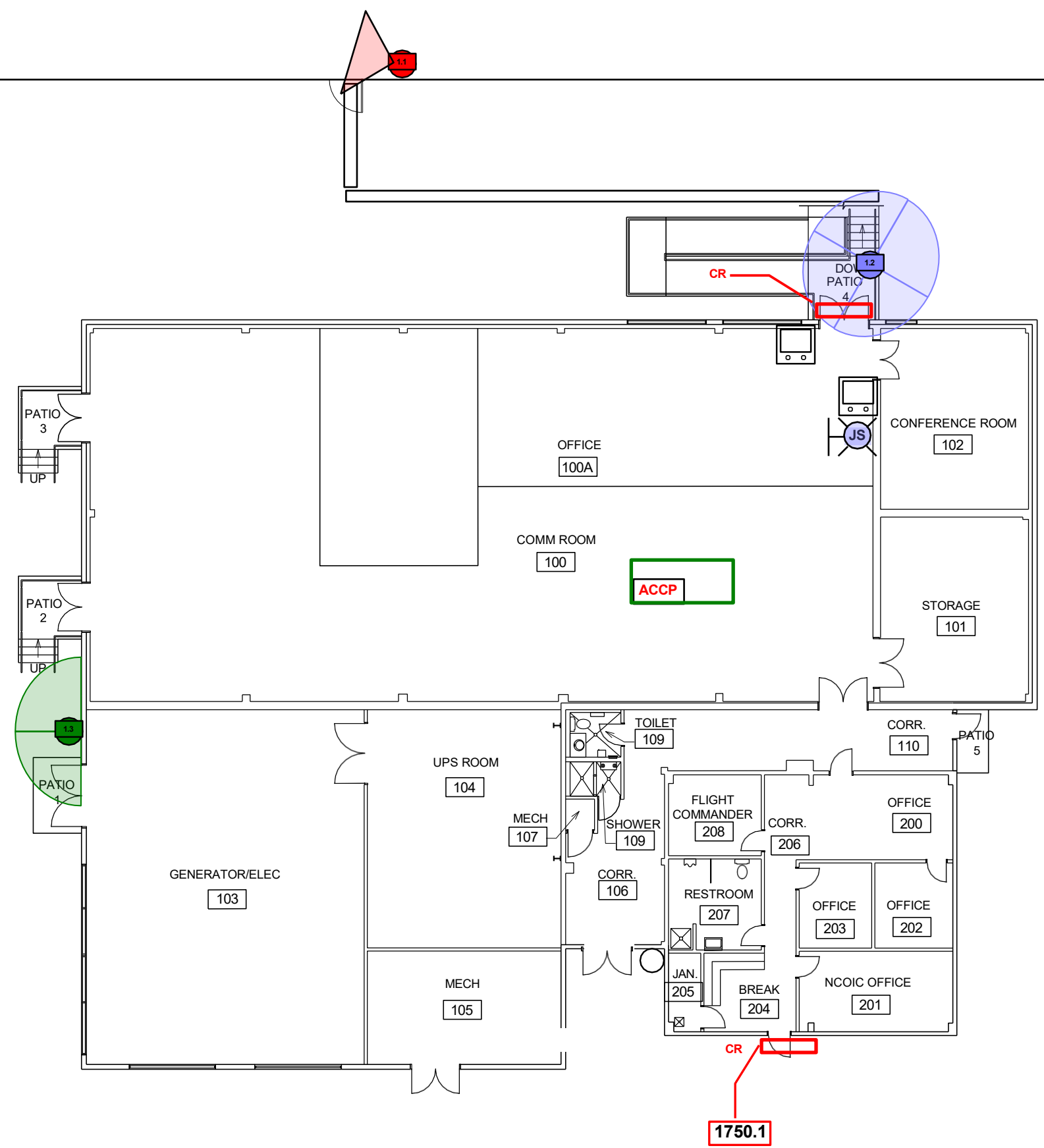
FLOOR PLAN - BLDG 1750 SCALE: 1/16" = 1'-0"
