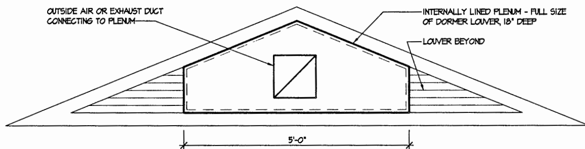
PLENUM AT DORMER LOUVER DETAIL NO SCALE
