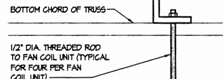
FCU SUPPORT DETAIL NO SCALE
