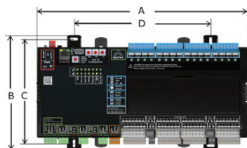
• Figure 1: Physical Dimensions
