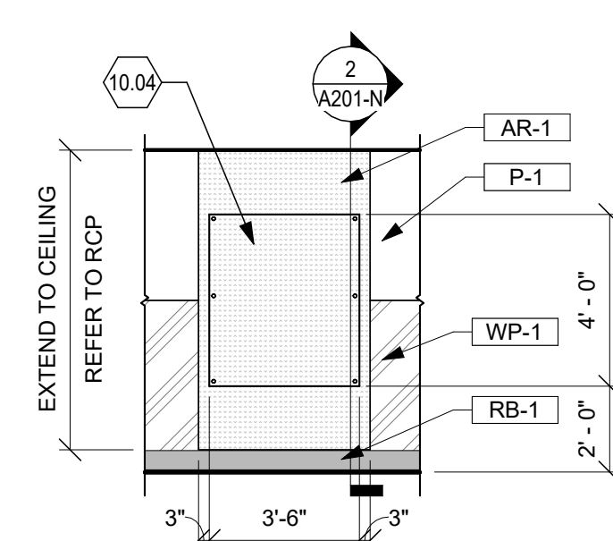
2 SIGNAGE TYP. Scale: 1/4" = 1'-0"
