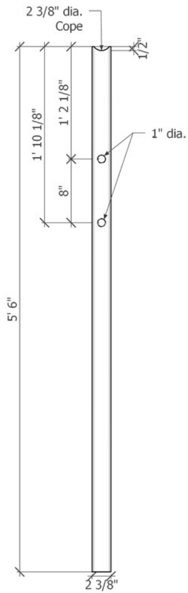
Figure 3 - Fence Post Specifications
