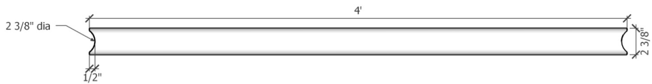
Figure 2 - Brace Rail Specifications
