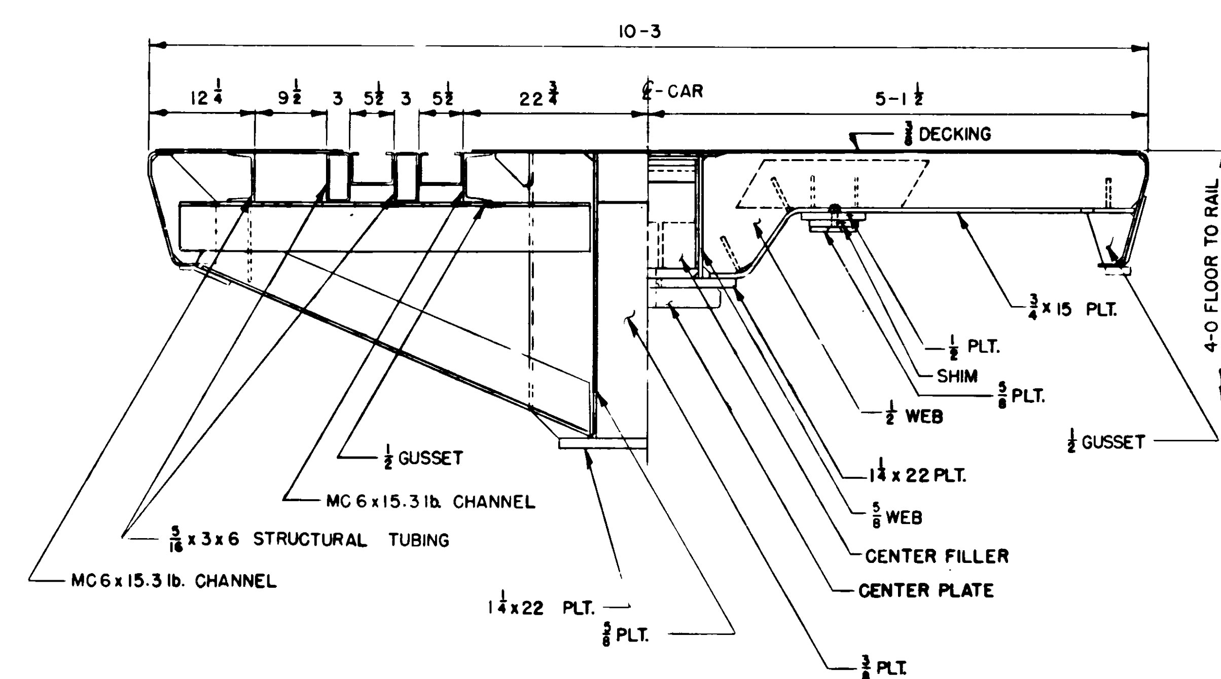
SECTIONS THRU CROSSBEARER AND BOLSTER SCALE: 1/4" = 1'-0"
