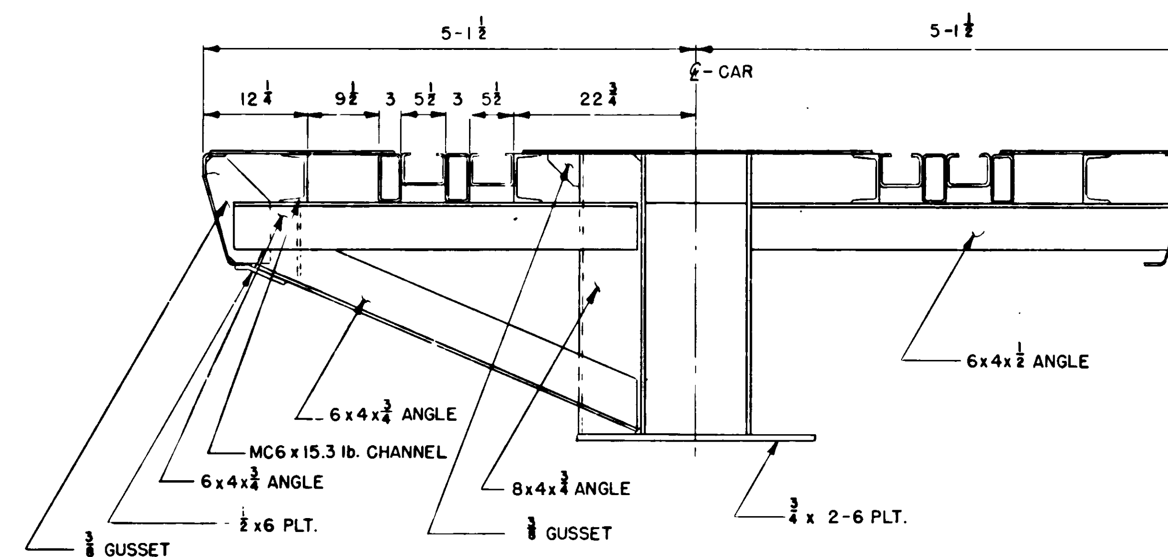
SECTION THRU CROSSBEARER NEXT TO CENTER LINE OF CAR SCALE: 1/4" = 1'-0"
