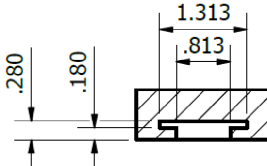
Figure 2: Section view of a Slot on the Replaceable Tracks.
