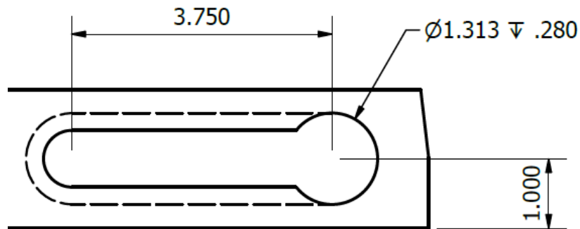
Figure 1: Top view of the Replaceable Tracks Slots.
