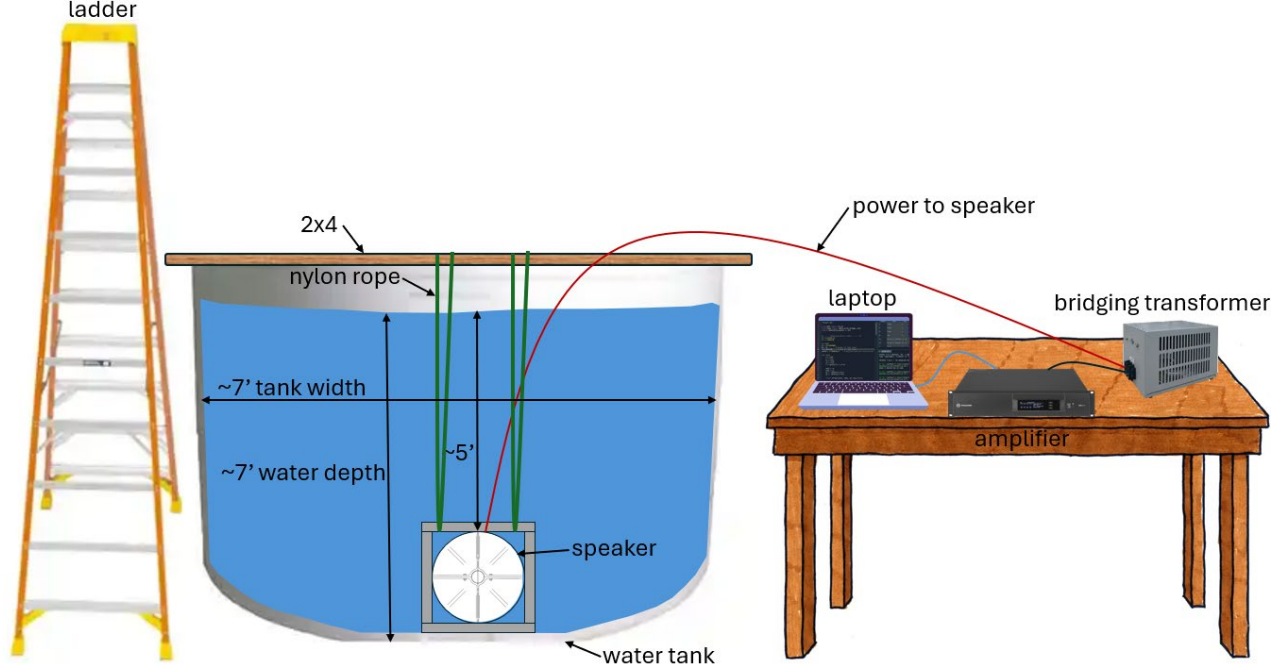
Figure 1 – Hydroacoustic Speaker Wet Test Setup
