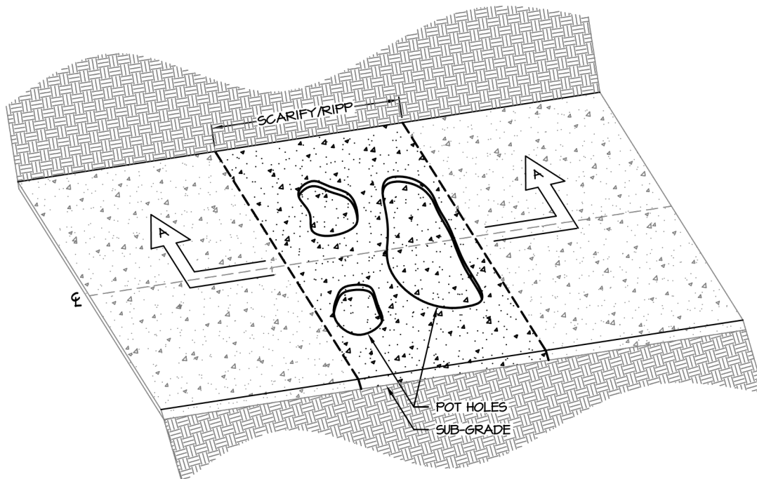
POT HOLE TREATMENT TYPICAL Not to Scale
