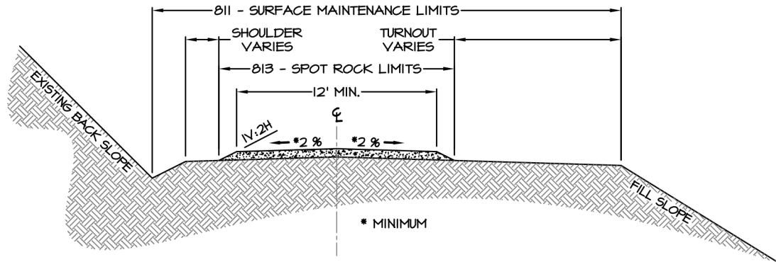
SURFACE MAINTENANCE & SPOT ROCK TYPICAL Not to Scale
