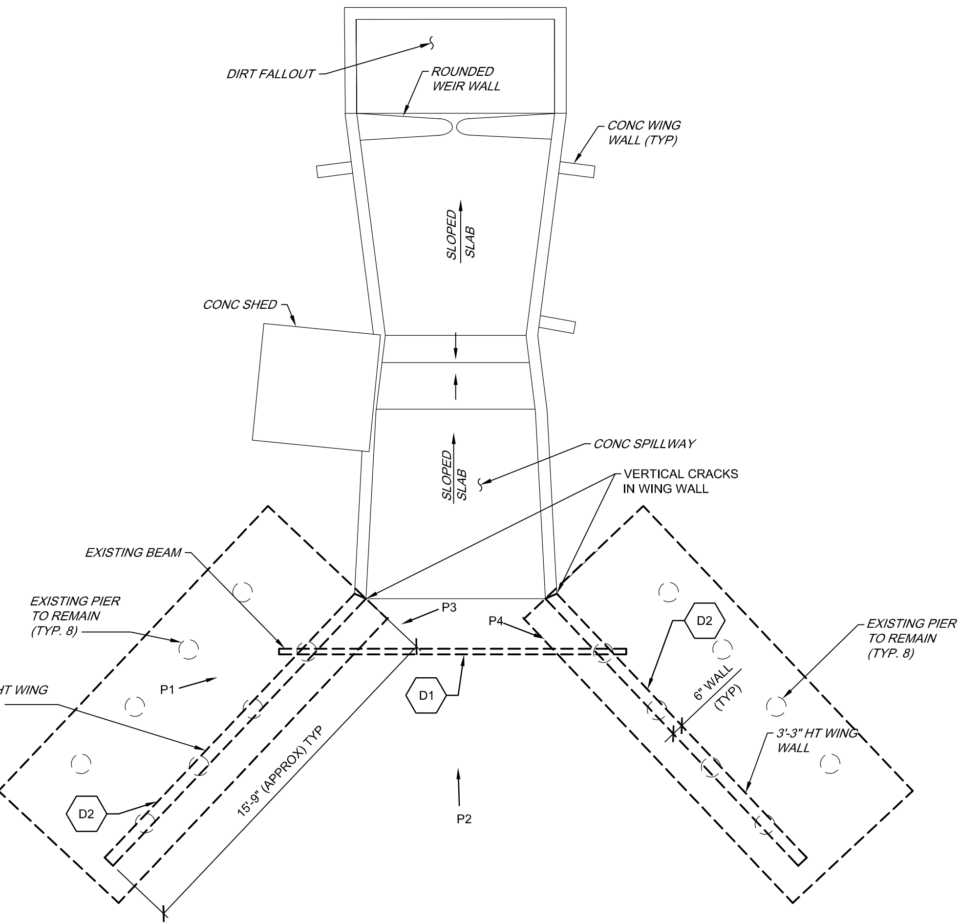
RUNOFF STATION W10 DEMOLITION PLAN
