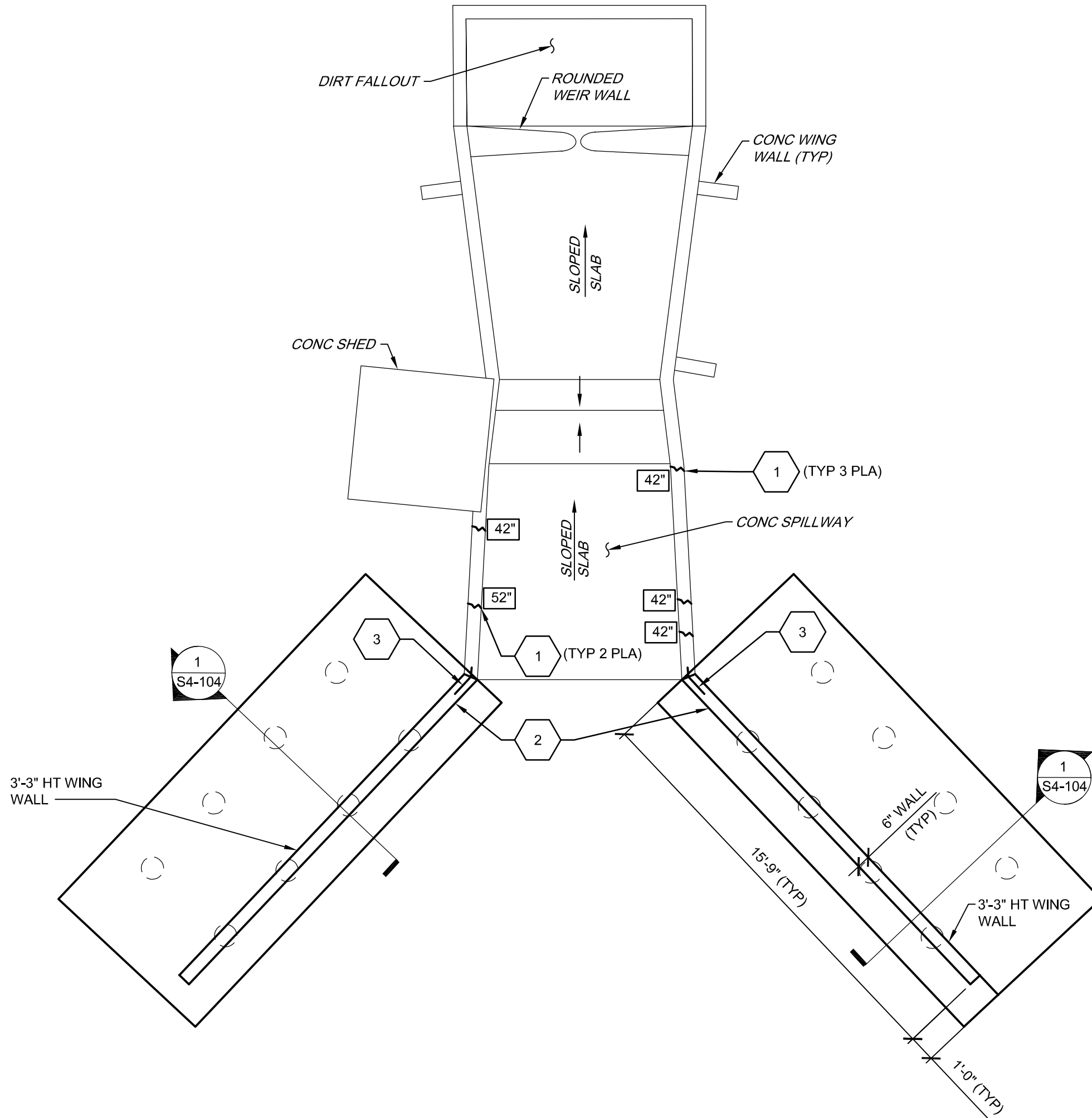
RUNOFF STATION W10 NEW WORK PLAN
