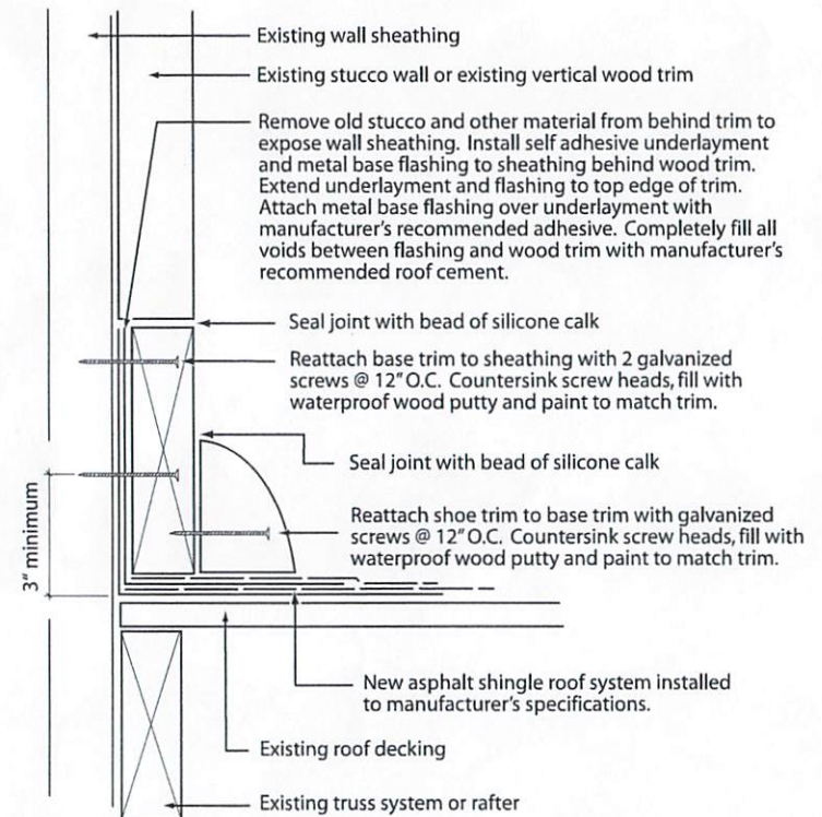
2 Vertical Wall Flashing With Wood Base and Shoe Trim A9 Not to Scale
