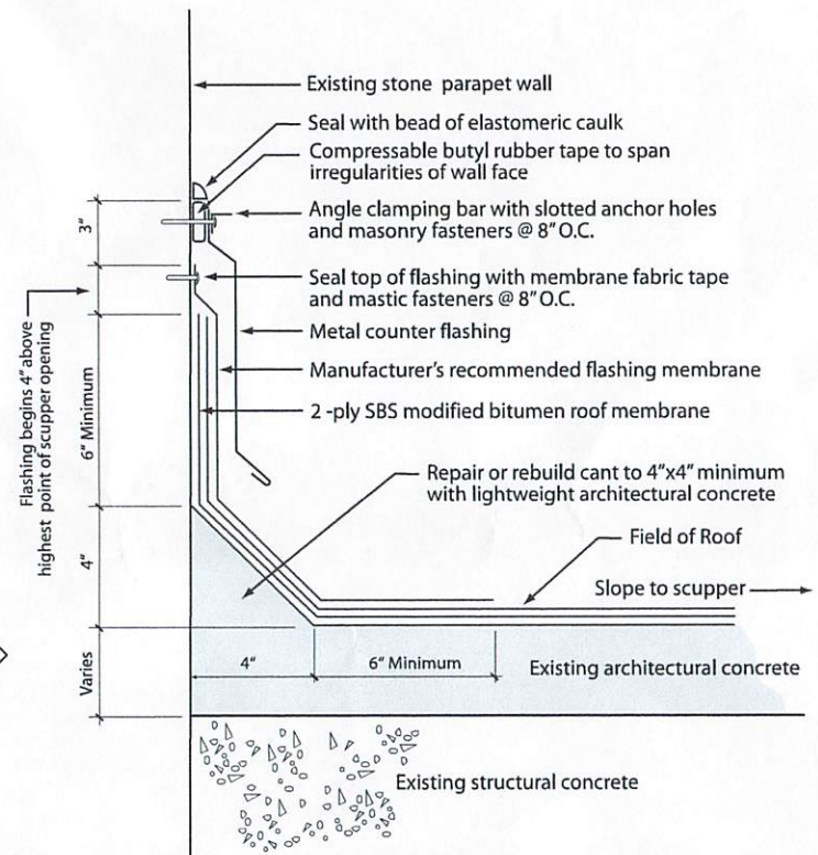
2 SECTION - FLASHING, CANT, AND COUNTER FLASHING A14 NOT TO SCALE
