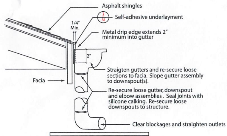
2 Drip Edge with Gutter Detail Not to Scale
