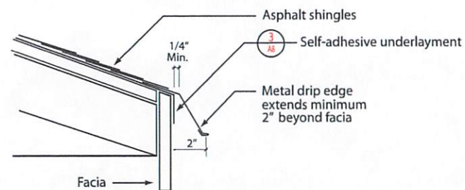
3 Drip Edge without Gutter Detail Not to Scale
