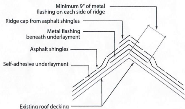
1 A8 Ridge Flashing Detail Not to Scale
