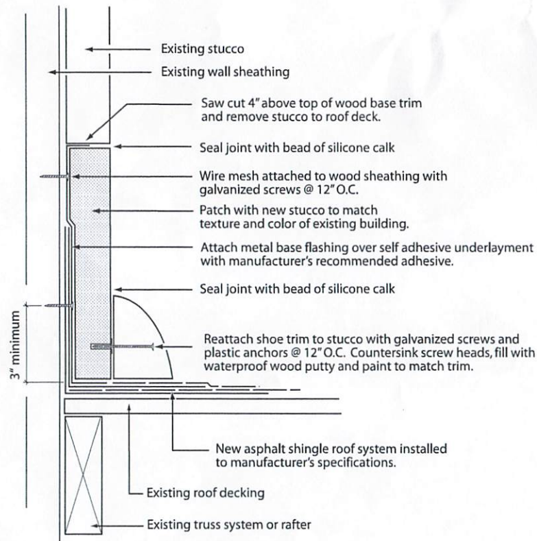
1 Vertical Wall Flashing on Stucco Wall with Wood Shoe Trim A9 Not to Scale
