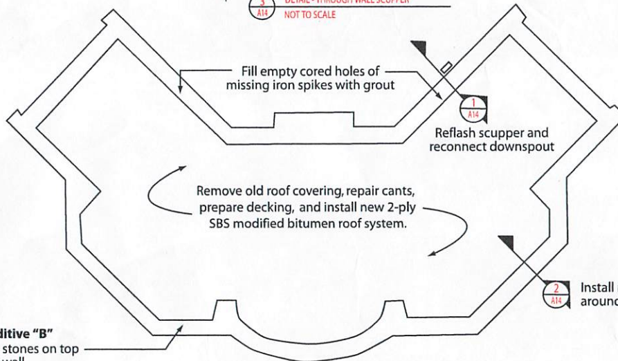
1 ROOF IMPROVEMENTS 14 NOT TO SCALE
