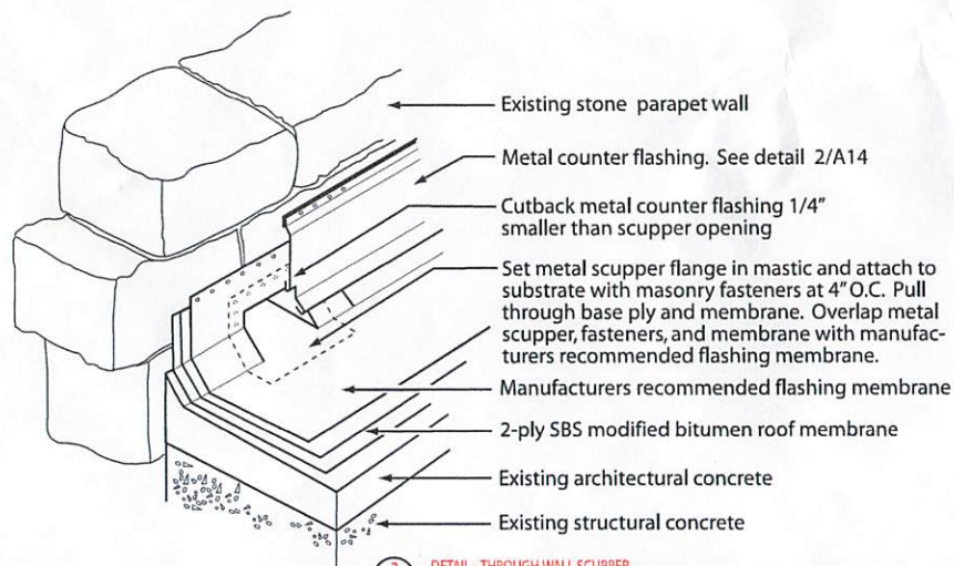
3 DETAIL - THROUGH WALL SCUPPER A14 NOT TO SCALE
