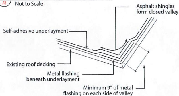
2 A8 Valley Flashing Detail Not to Scale
