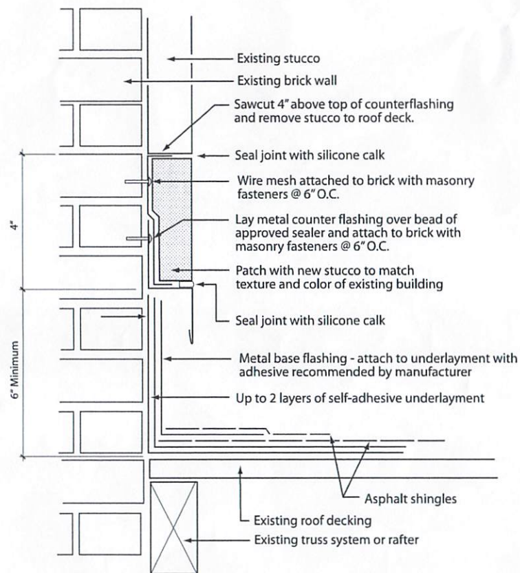
1 Vertical Wall Flashing on Stucco Wall Not to Scale
