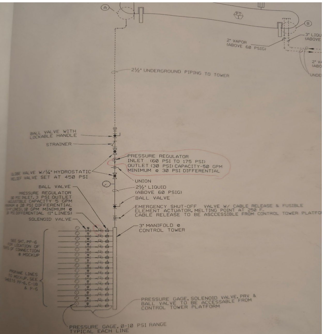
LPG PIPING DIAGRAM
