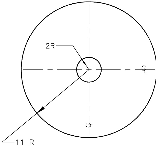
BASE SUPPORT (4)
