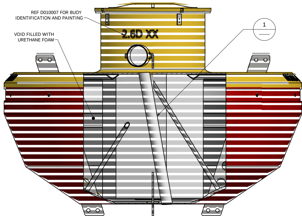
BREAK OUT VIEW NTS
