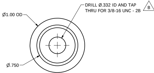
TOP VIEW SCALE 2 : 1
