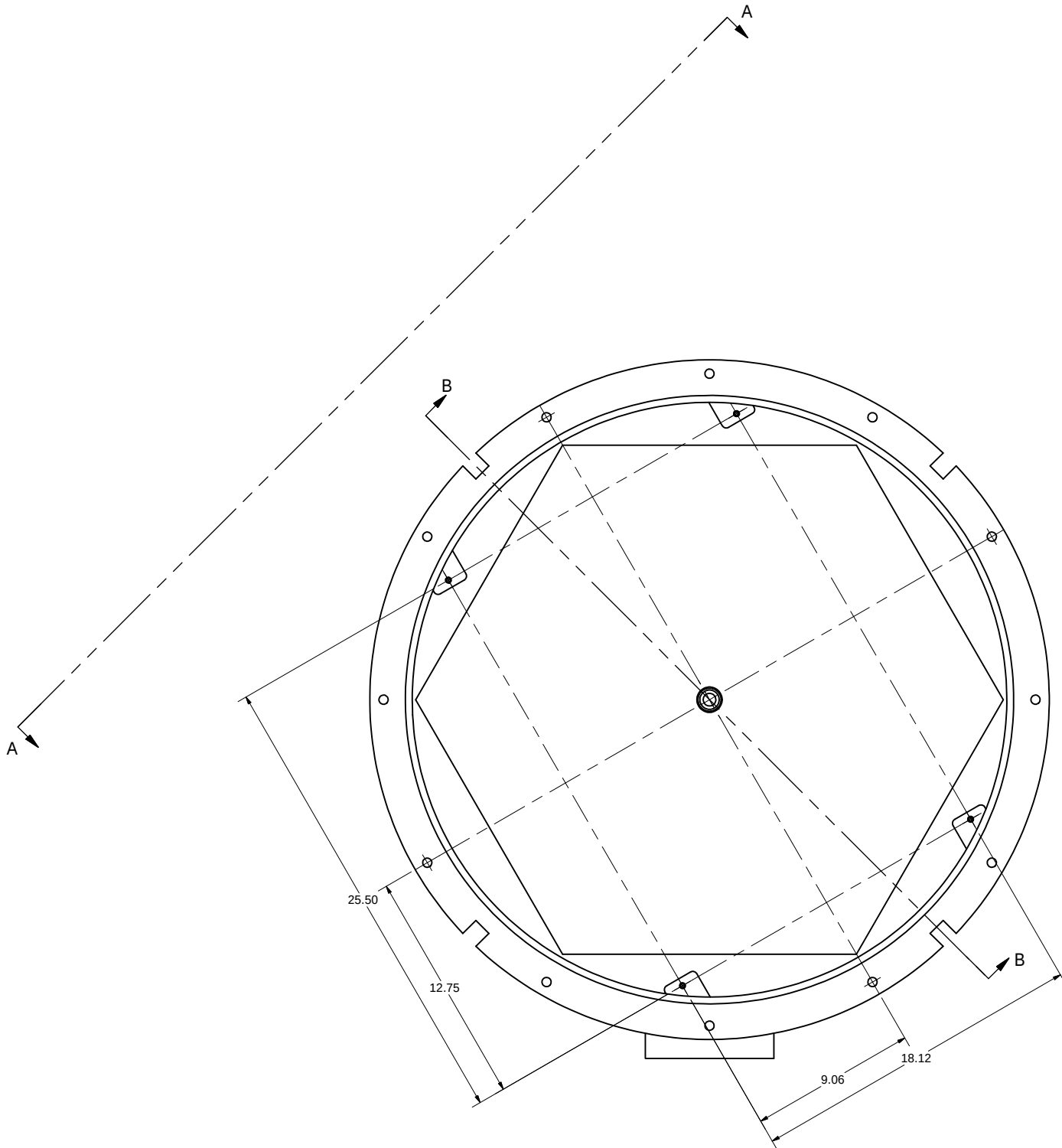
TOP VIEW SCALE 1 : 4
