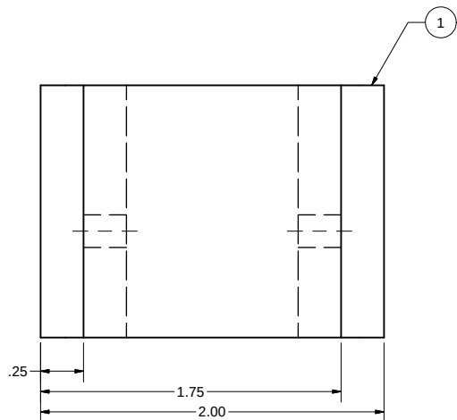
SIDE VIEW SCALE 2 : 1
