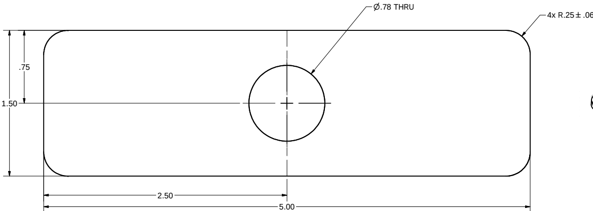
FLAT PATTERN SCALE 2 : 1
