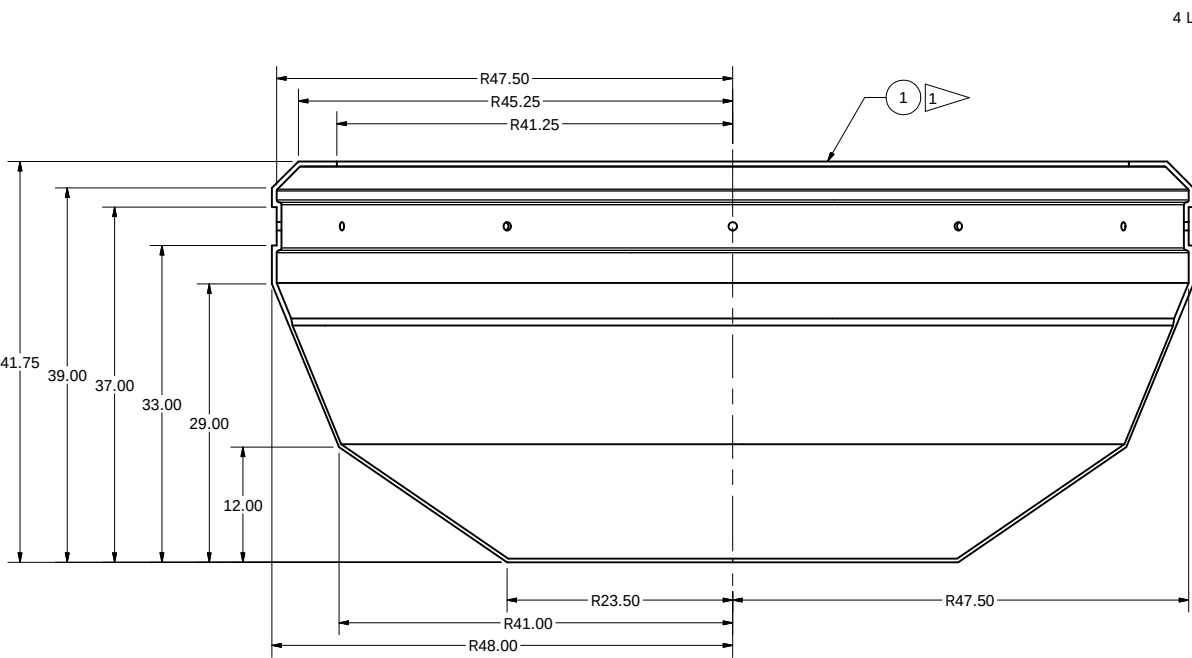
FRONT VIEW SCALE 1 : 10
