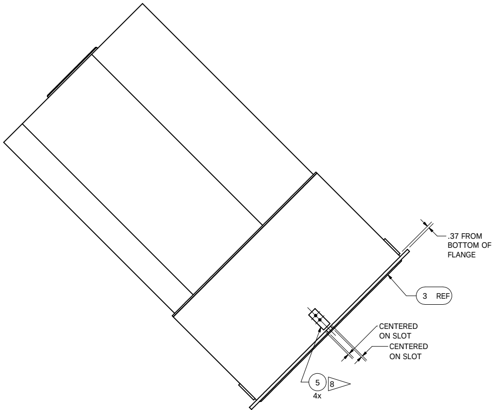
VIEW A-A NTS
