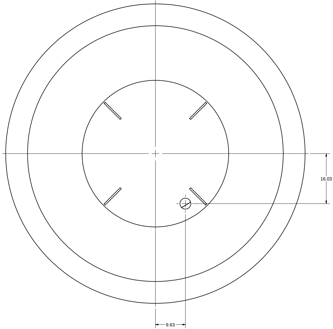
BOTTOM VIEW NTS
