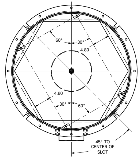
TOP VIEW NTS
