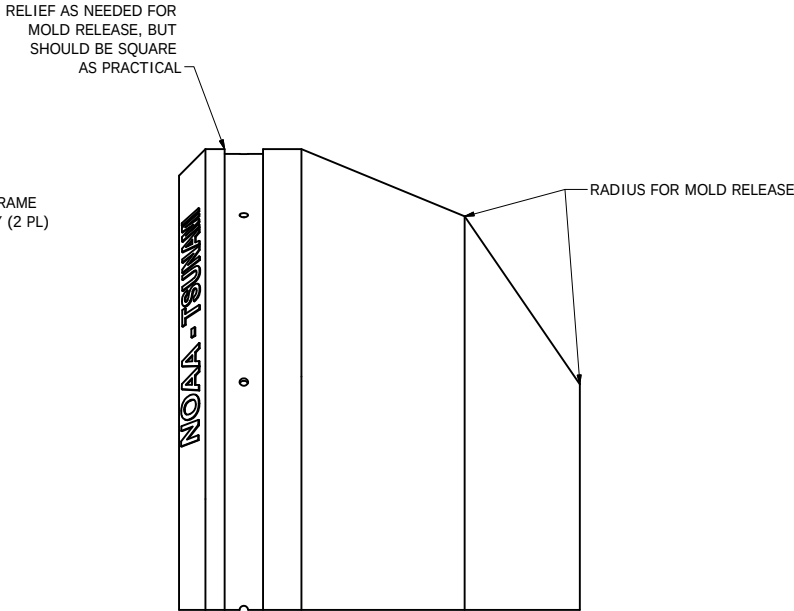
SIDE VIEW SCALE 1 : 10
