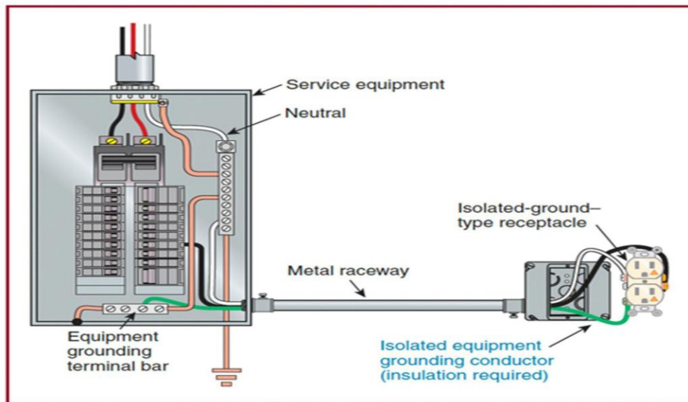
Proper wiring and grounding of lighting and receptacle loads
