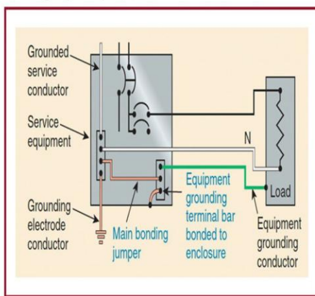
Proper wiring and grounding of equipment
