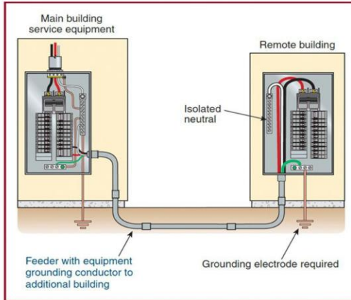
Proper wiring, grounding, and bonding when you have main panel and sub-panels.
