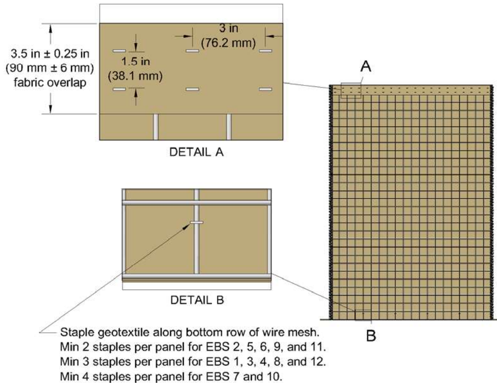
FIGURE 4. Typical geotextile staple pattern
