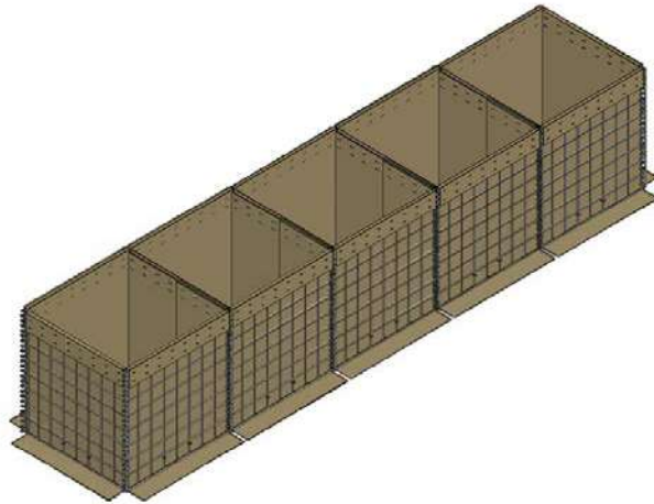
FIGURE 10. Type 5 (5cells (1x5)).
