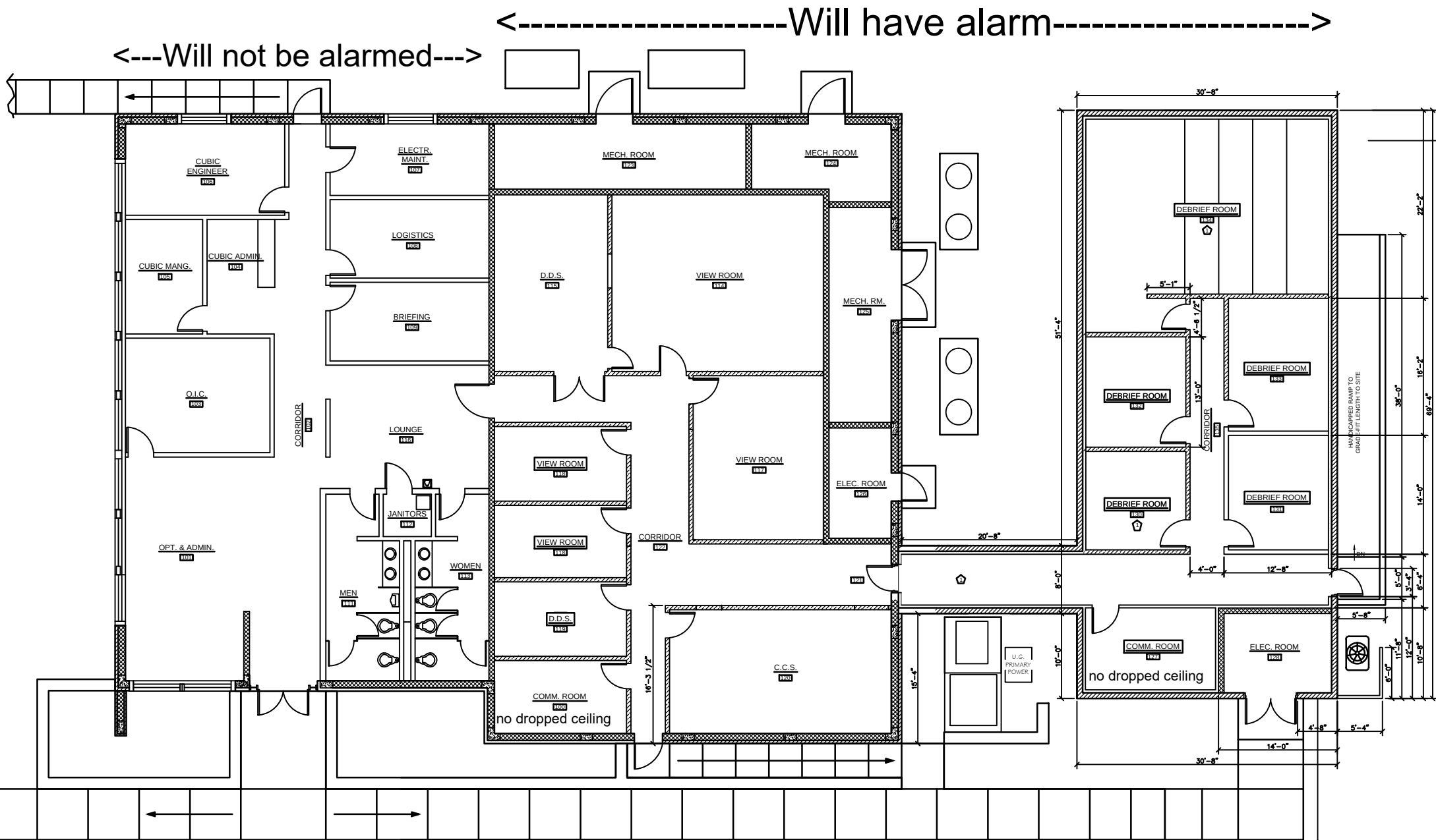
FLOOR PLAN - BLDG 503
