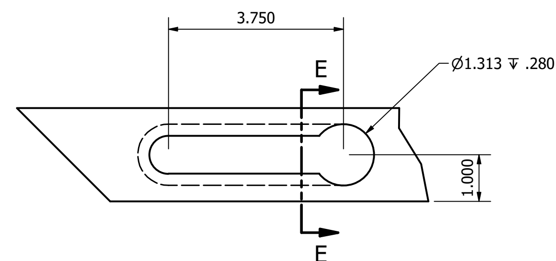
DETAIL H SCALE 1 / 2
