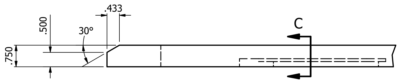
DETAIL D SCALE 1 / 2
