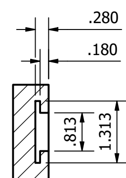
SECTION E-E SCALE 1 / 2
