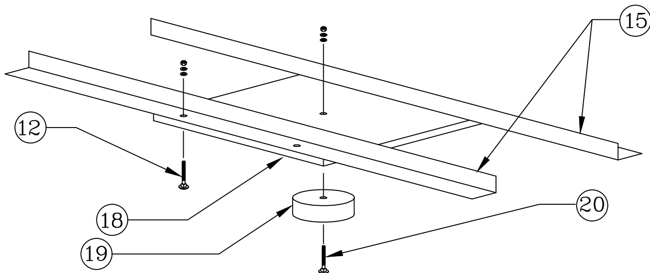
TOP HOLD-DOWN ASSEMBLY
