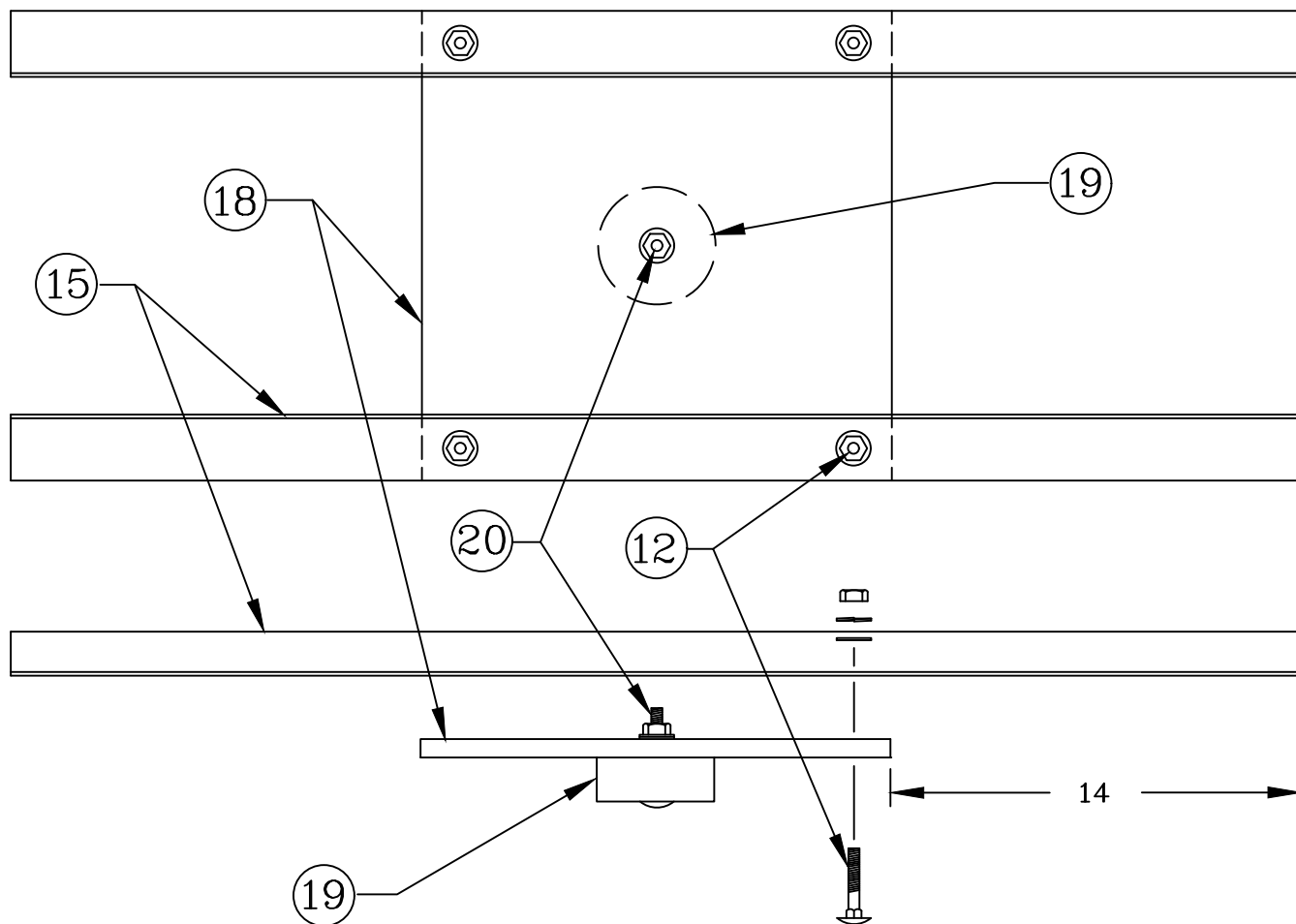
TOP HOLD-DOWN ASSEMBLY
