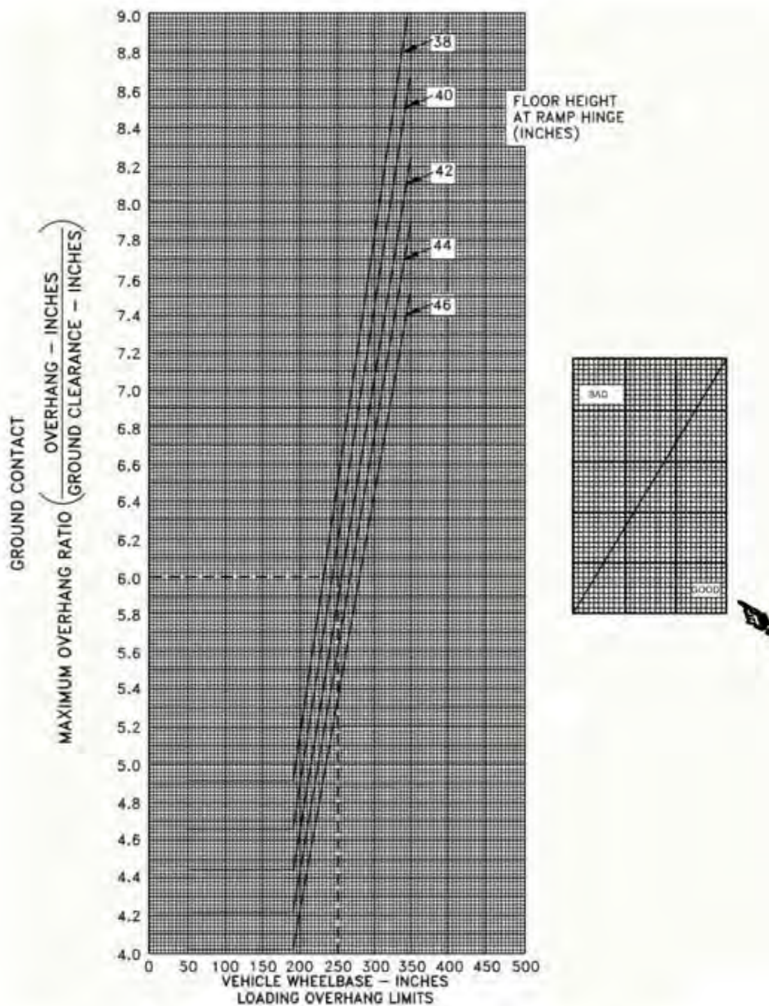
FIGURE B-87. Overhang and projection limits (vehicle).
