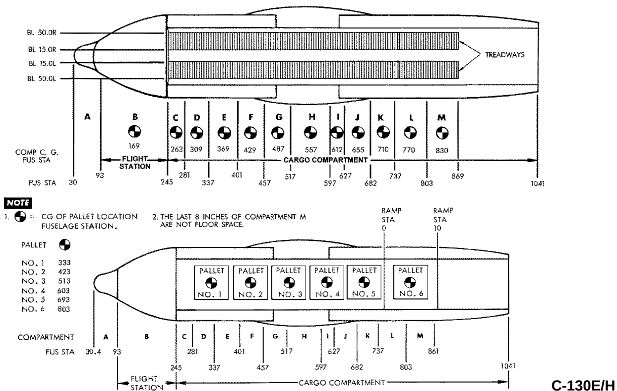
FIGURE B-89 C-130E/H compartments and pallet centroids.
