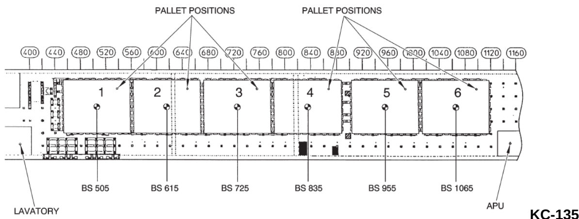
FIGURE B-128. Cargo roller handling system (six pallets installed).
