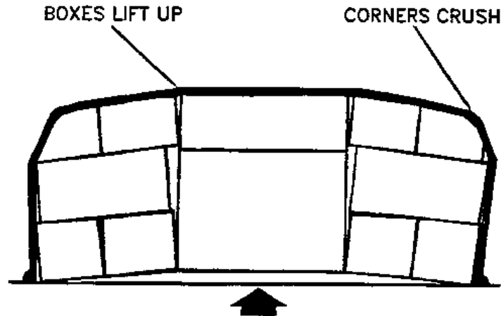
FIGURE A-36. Vertical cargo shift.
