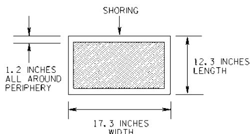
FIGURE B-34. Concentrated cargo maximum allowable floor loads (sheet 3 of 3).
