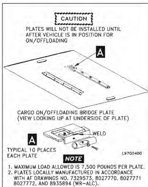
Bridge Plates
