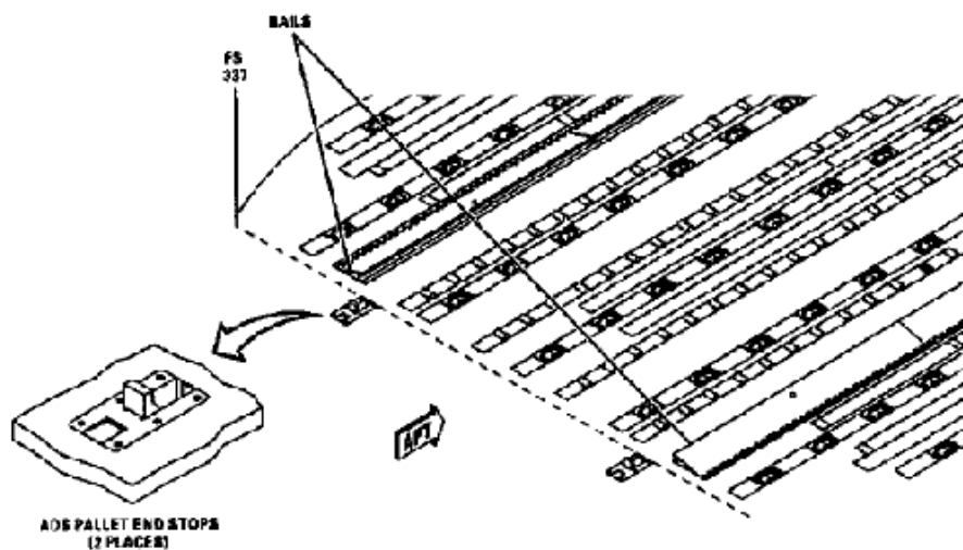
FIGURE B-67. C-17 ADS system.
