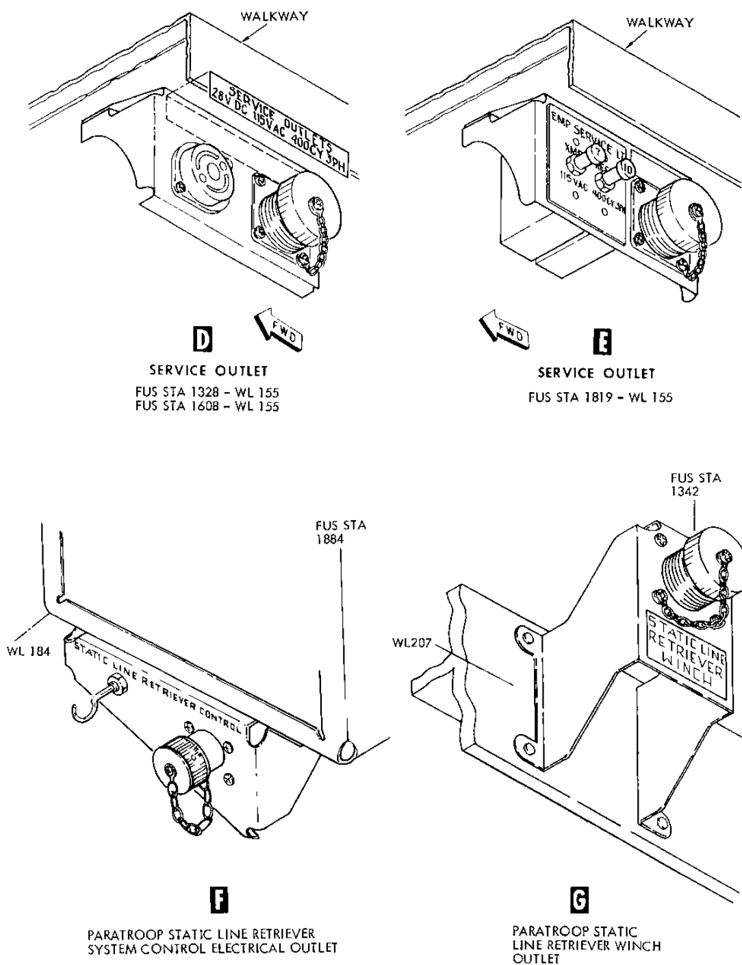
FIGURE B-46. Cargo compartment electrical outlets - Continued.
