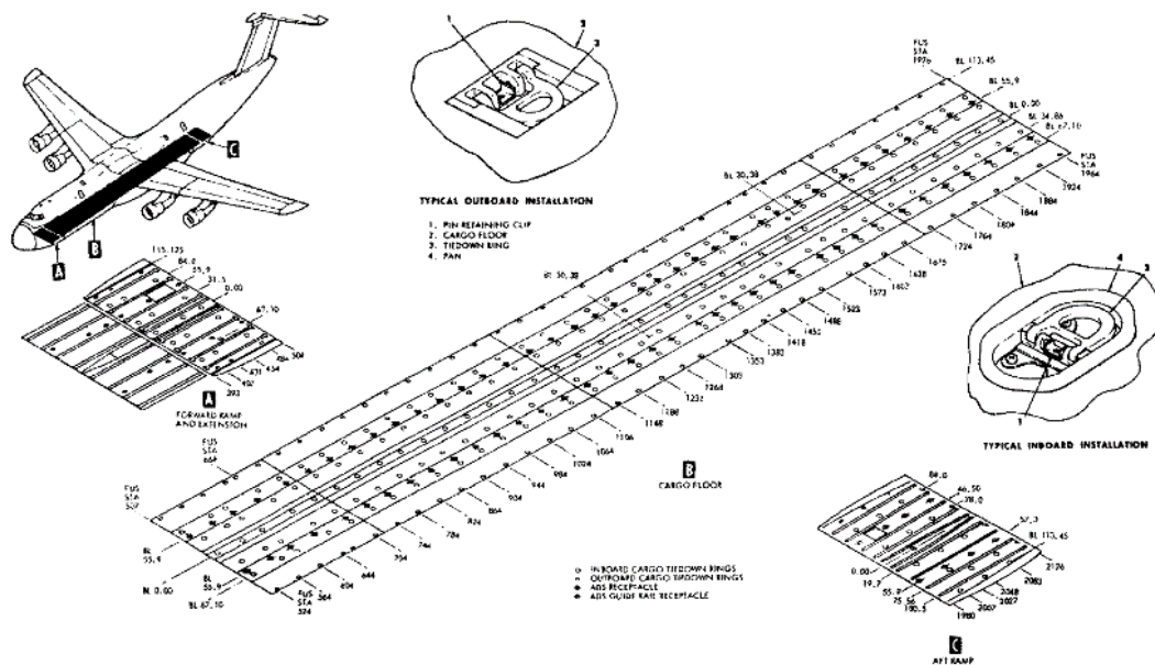
FIGURE B-41. Cargo floor tiedown rings and ADS receptacles.
