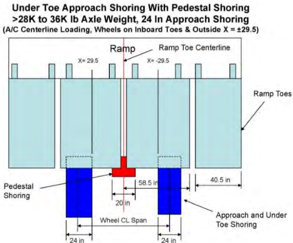
FIGURE B-59. C-17 minimum approach shoring width under ramp toes - (sheet 3 of 4).
