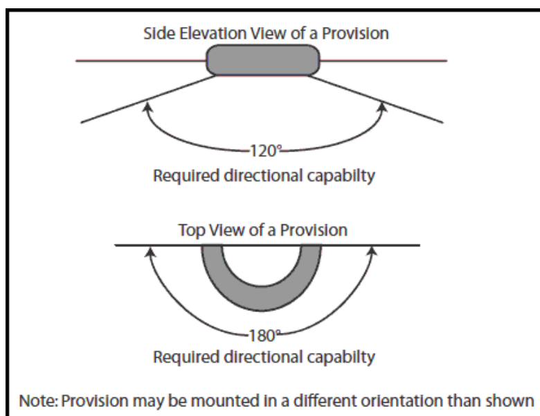
FIGURE 2. Tiedown rings.
