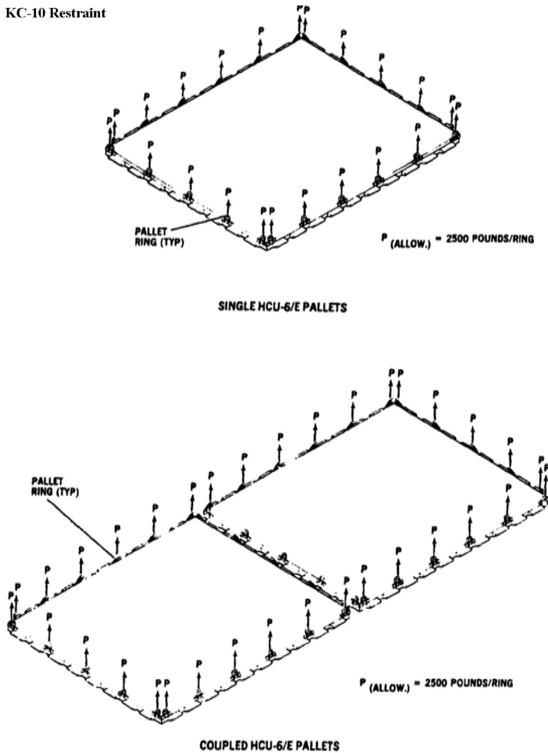
FIGURE B-121. HCU-6/E pallet ring vertical allowables.
