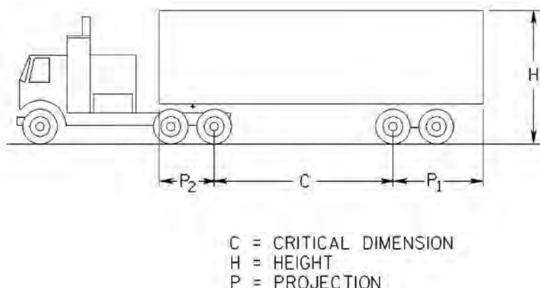
FIGURE B-9. Forward and aft end loading - vehicle projection.
