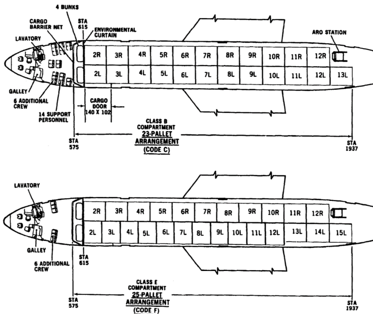
FIGURE B-107. Cargo compartment envelope.
