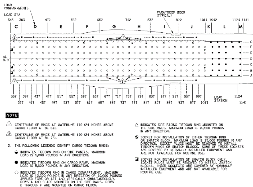
FIGURE B-100. C-130J-30 tiedown fittings locations.
