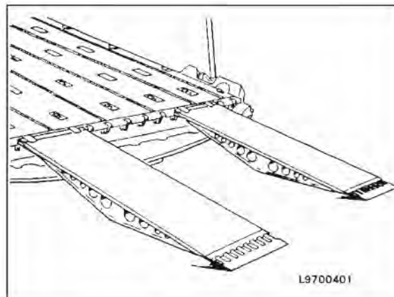
Auxiliary Ground Loading Ramps Installed
