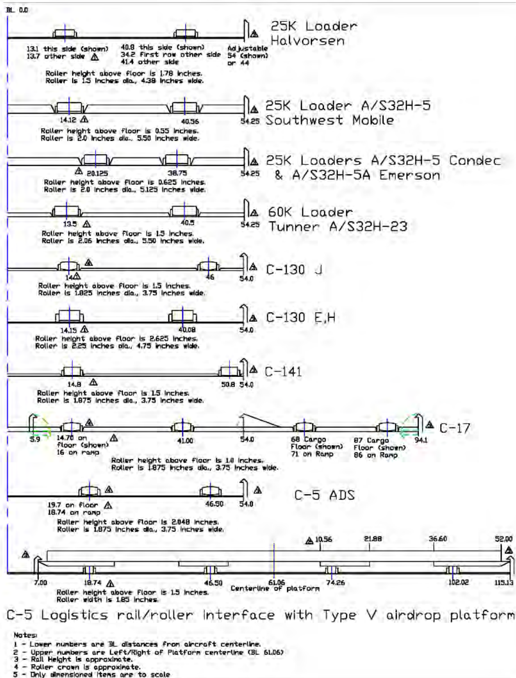
FIGURE A-11. Logistics rail/roller interface with type V airdrop platform.
