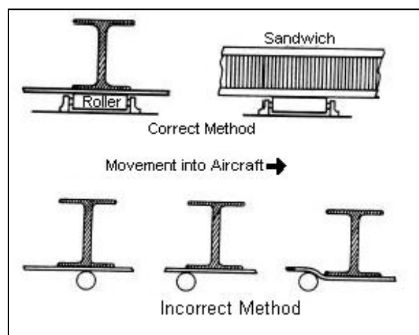
FIGURE 4. Pallet/roller interface.
