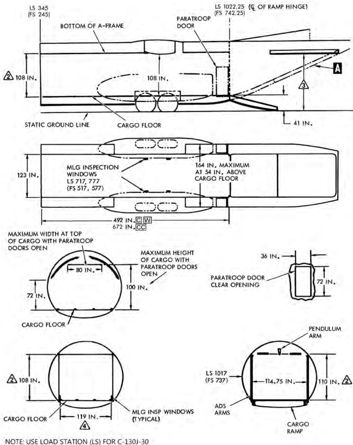
FIGURE B-82.b. C-130J and C-130J-30 cargo compartment dimensions.
