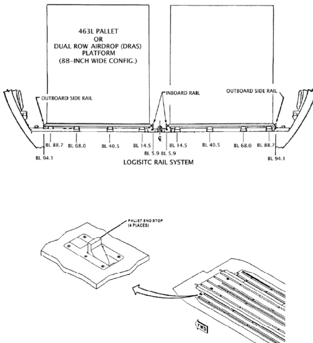
FIGURE B-68. C-17 logistic rail system.
