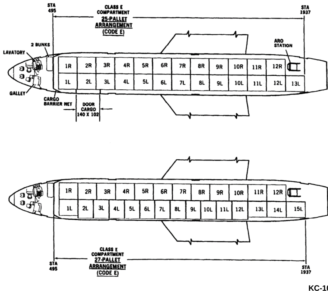
FIGURE B-113. All-cargo configuration.
