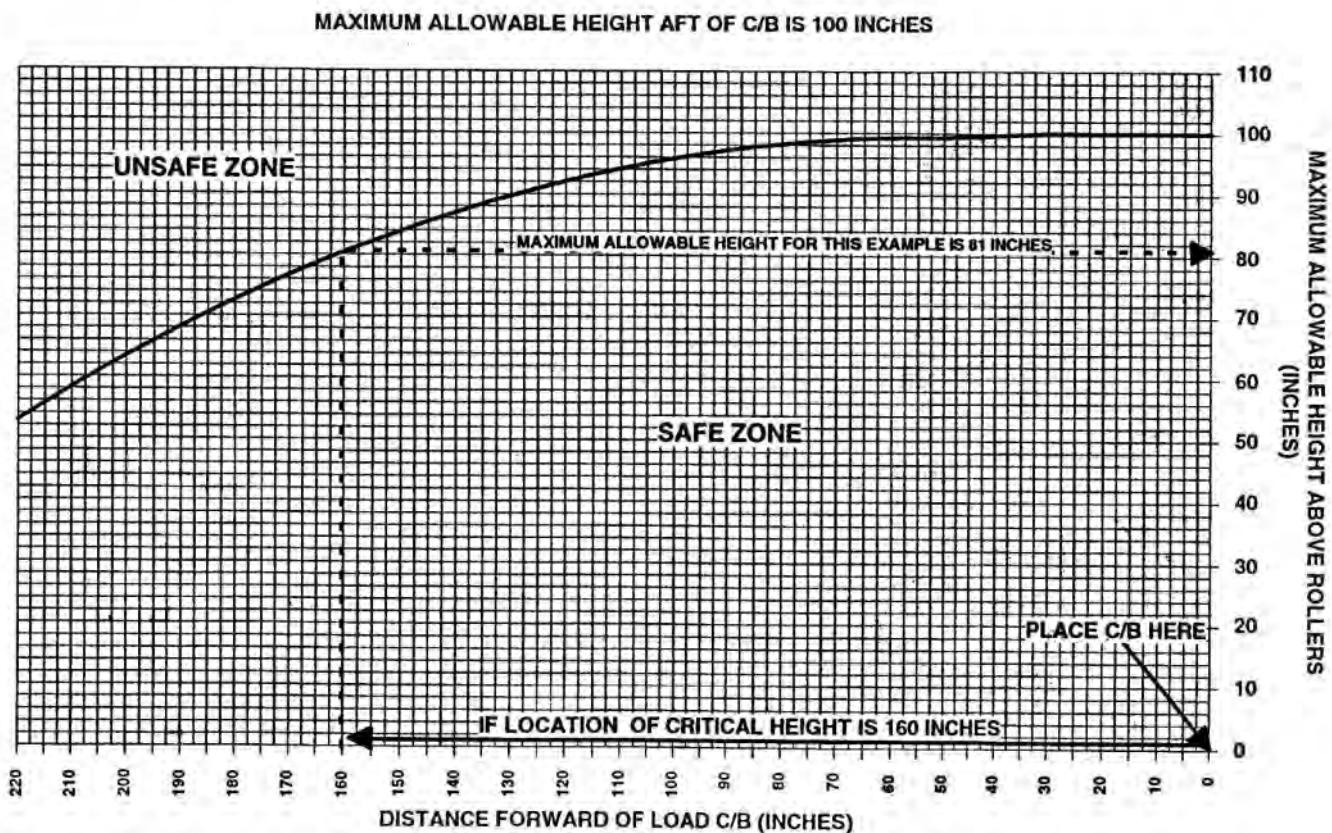
FIGURE B-103. C-130 tip off or jettison height limit curve (all variants).
