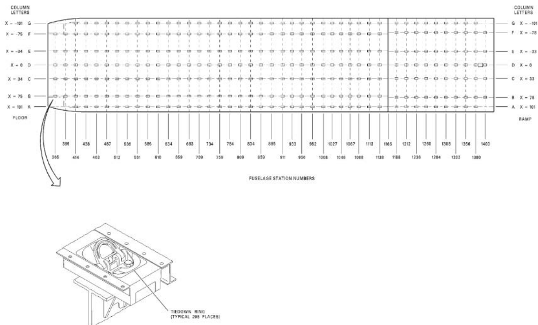
FIGURE B-74. Cargo tiedown rings/location.
