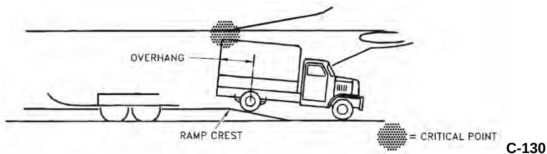
FIGURE B-85. Overhang and projection limits (vehicle).
