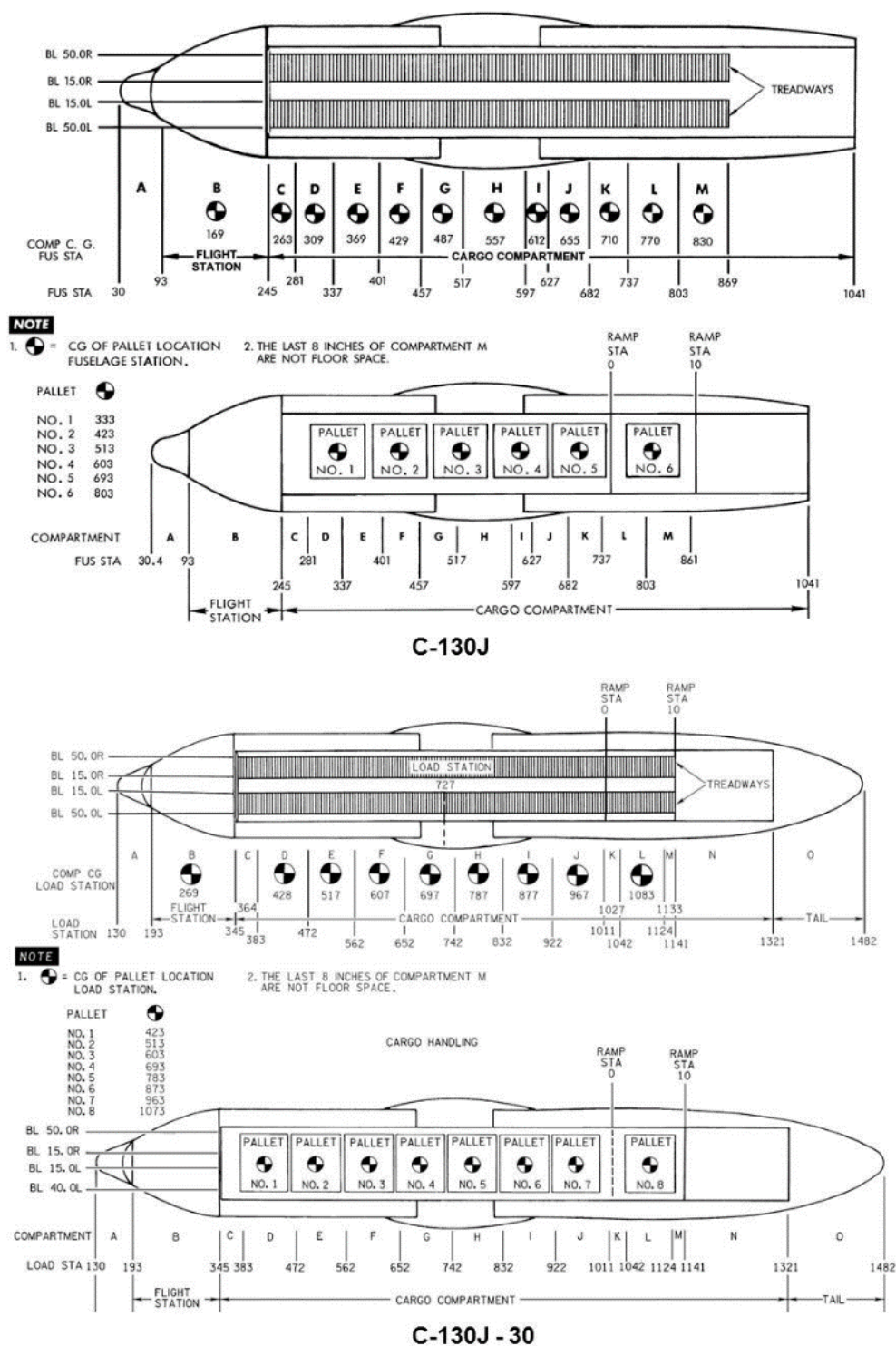
FIGURE B-93. C-130J and -30 compartments, treadways and pallet centroids.
