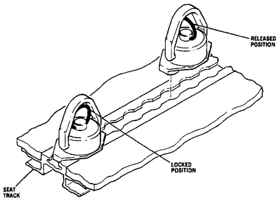
Figure A-7000 Tiedown Fitting
