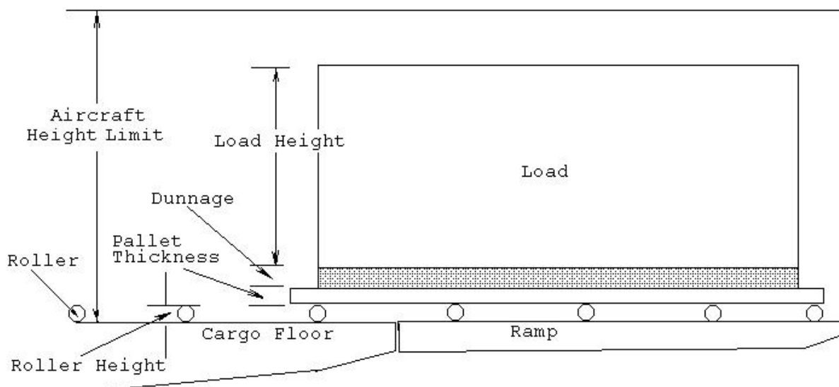
FIGURE A-14. Palletized cargo height.
