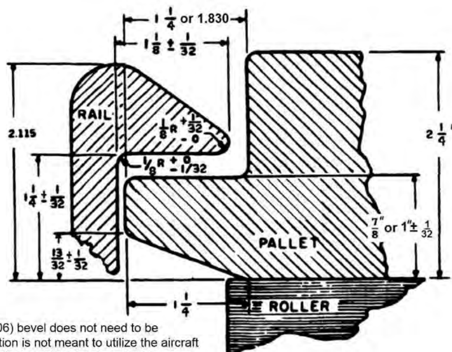
FIGURE 5. Pallet rail exterior profile.
