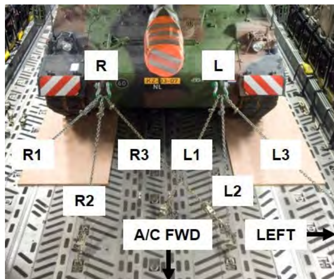
FIGURE A-34. Example complex tiedown.
