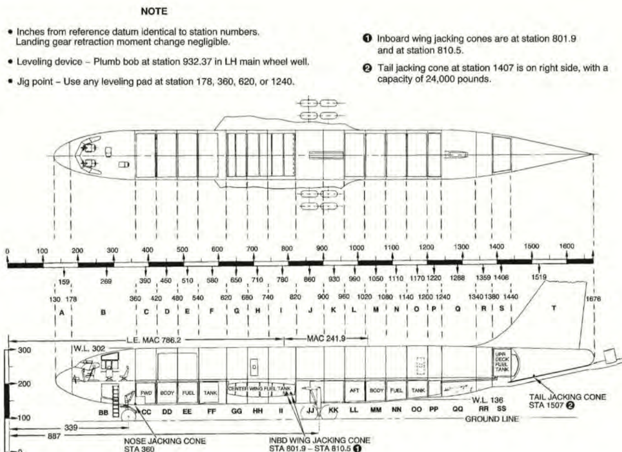
FIGURE B-126. Aircraft diagram (typical).
