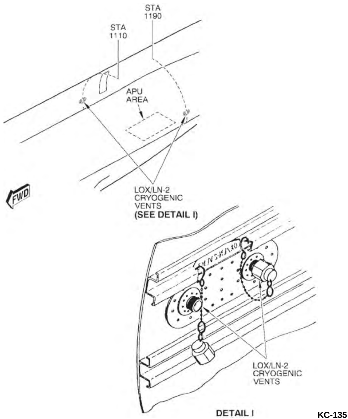
FIGURE B-137. KC-135 cryogenic vents.
