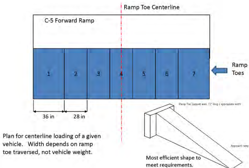
FIGURE B-29. C-5 minimum approach shoring width under forward ramp toes.
