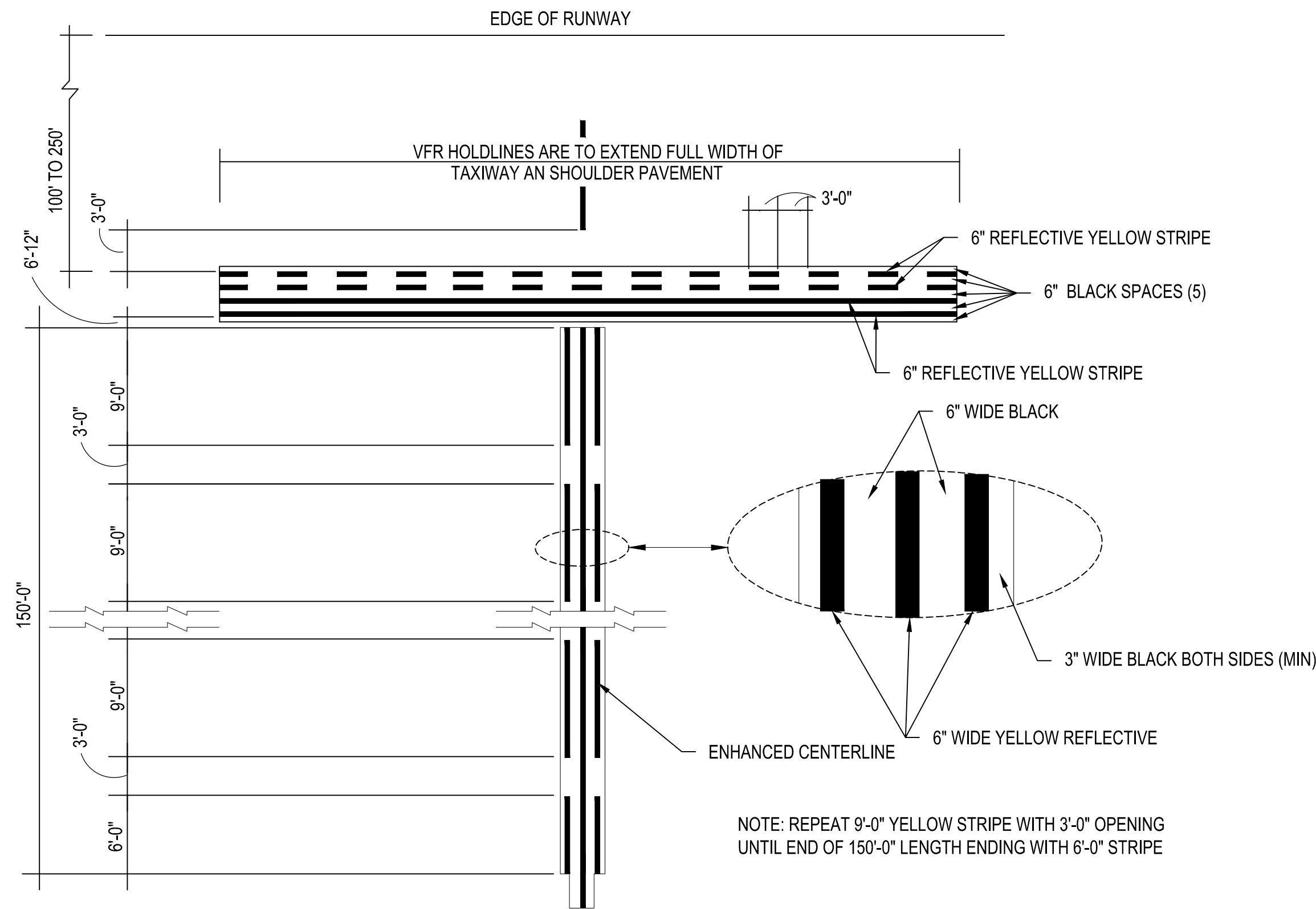
B VFR HOLDING POSITION MARKING PLAN CP502 NOT TO SCALE (HOLDING POSITION PER LF (LENGTH VARIES); REF. YELLOW = 1.51 SF / LF AND BLACK = 2.98 SF / LF) (ENHANCED CENTERLINE TOTAL: REF. YELLOW = 189 SF AND BLACK = 261 SF)
