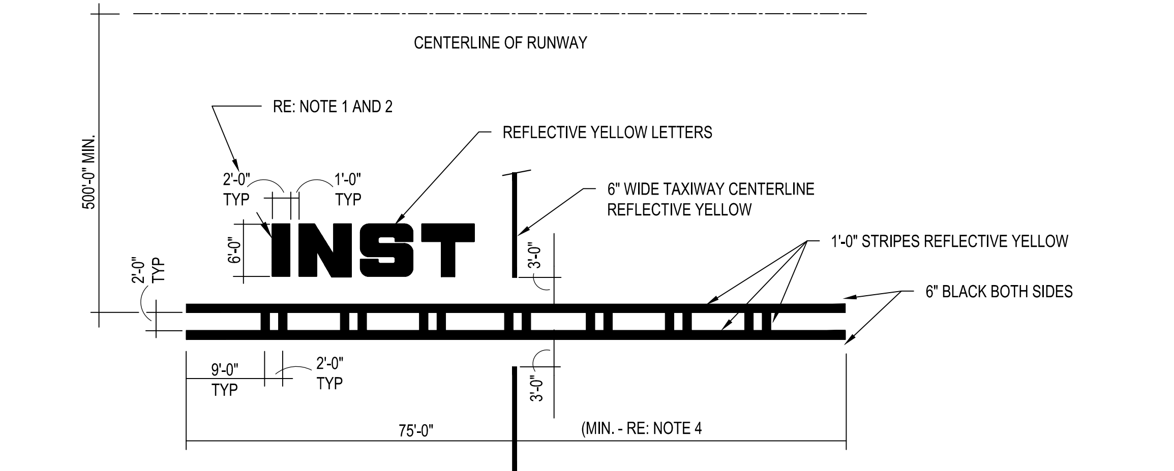
C INSTRUMENT HOLDING POSITION MARKINGS PLAN CP502 NOT TO SCALE NOTES FOR INSTRUMENT HOLD LOCATE LETTERS "INST" ON RUNWAY SIDE OF THE HOLD LINE AND ON THE LEFT SIDE OF CENTERLINE THE "INST" DESIGNATOR MUST BE PLACED SYMMETRICAL BETWEEN THE TAXIWAY CENTERLINE AND THE TAXIWAY EDGE.
