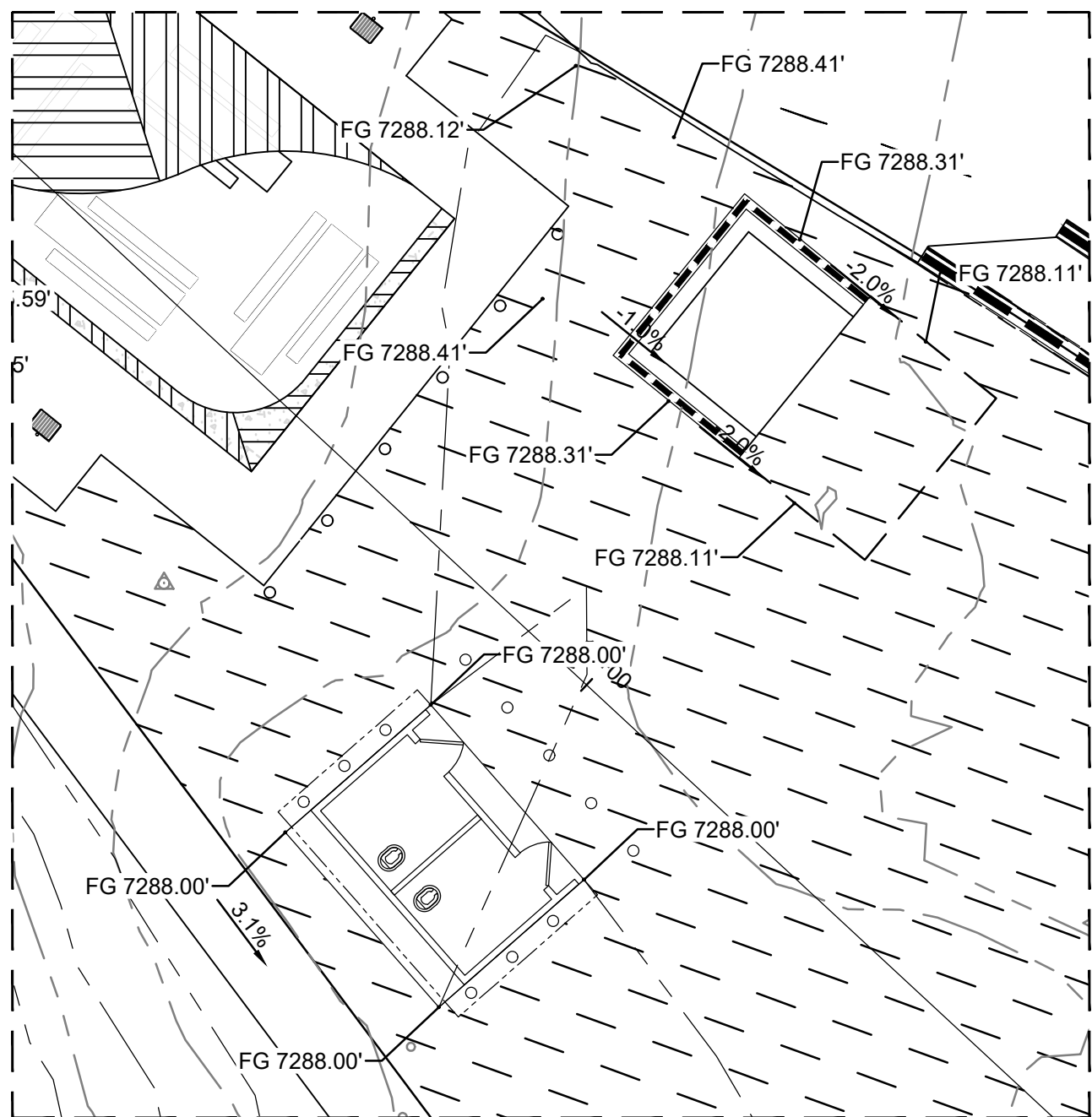
ENLARGED GRADING PLAN
