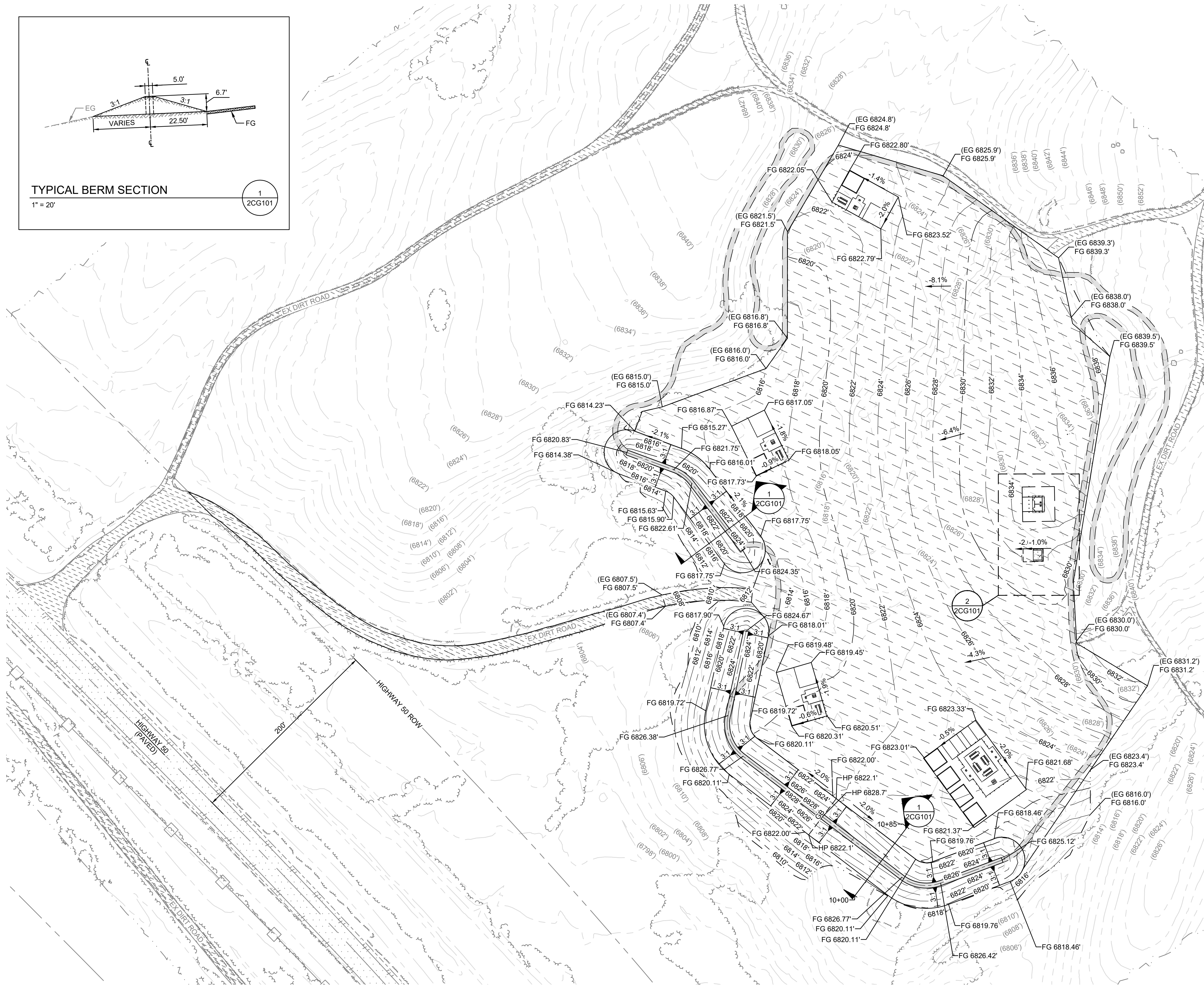
EGAN CREST GRADING PLAN 1" = 50'
