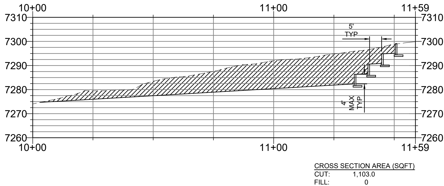
SECTION 1 HOR 1" = 20' | VERT 1" = 20'
