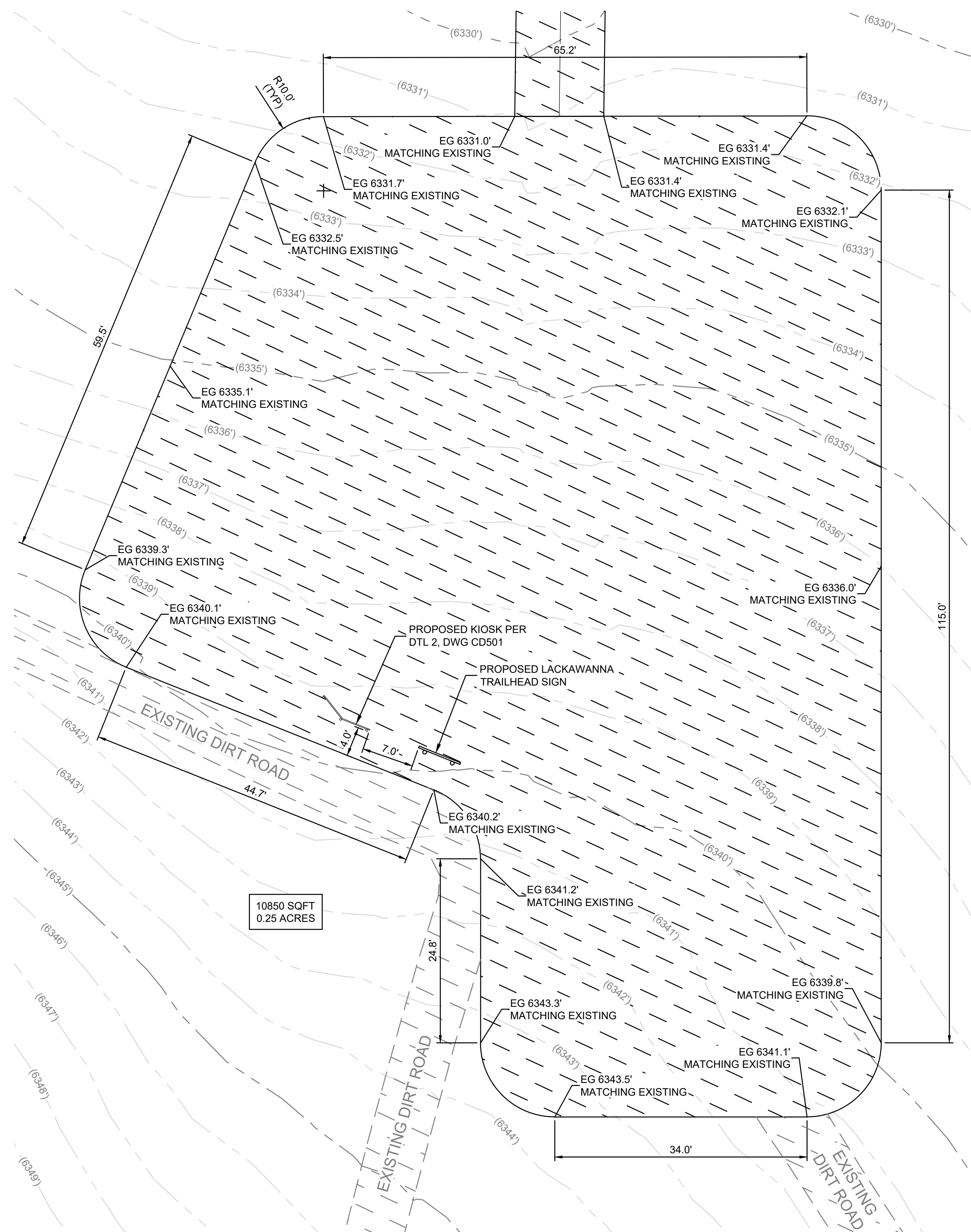
LACKAWANNA GRADING PLAN
