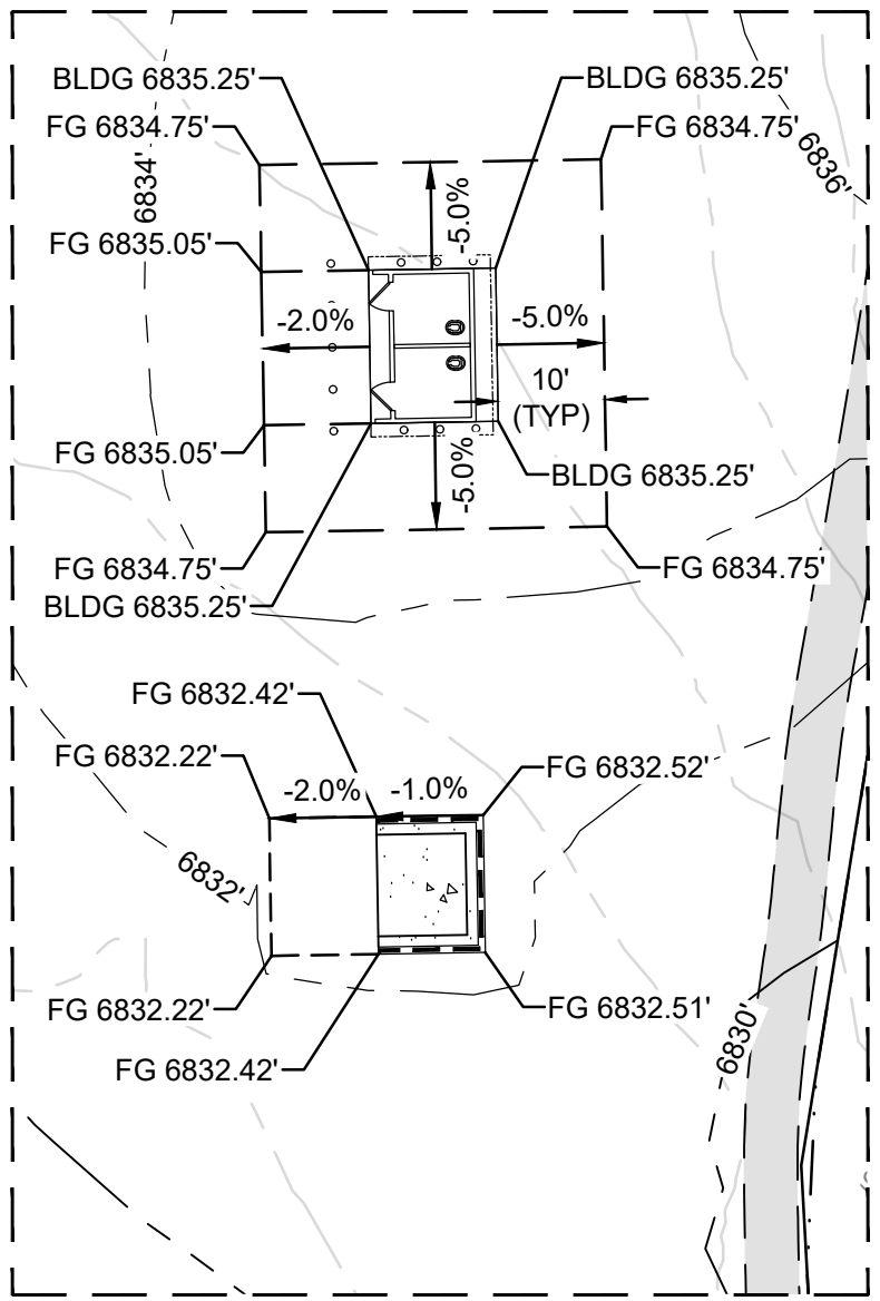
ENLARGED GRADING PLAN 1" = 20'
