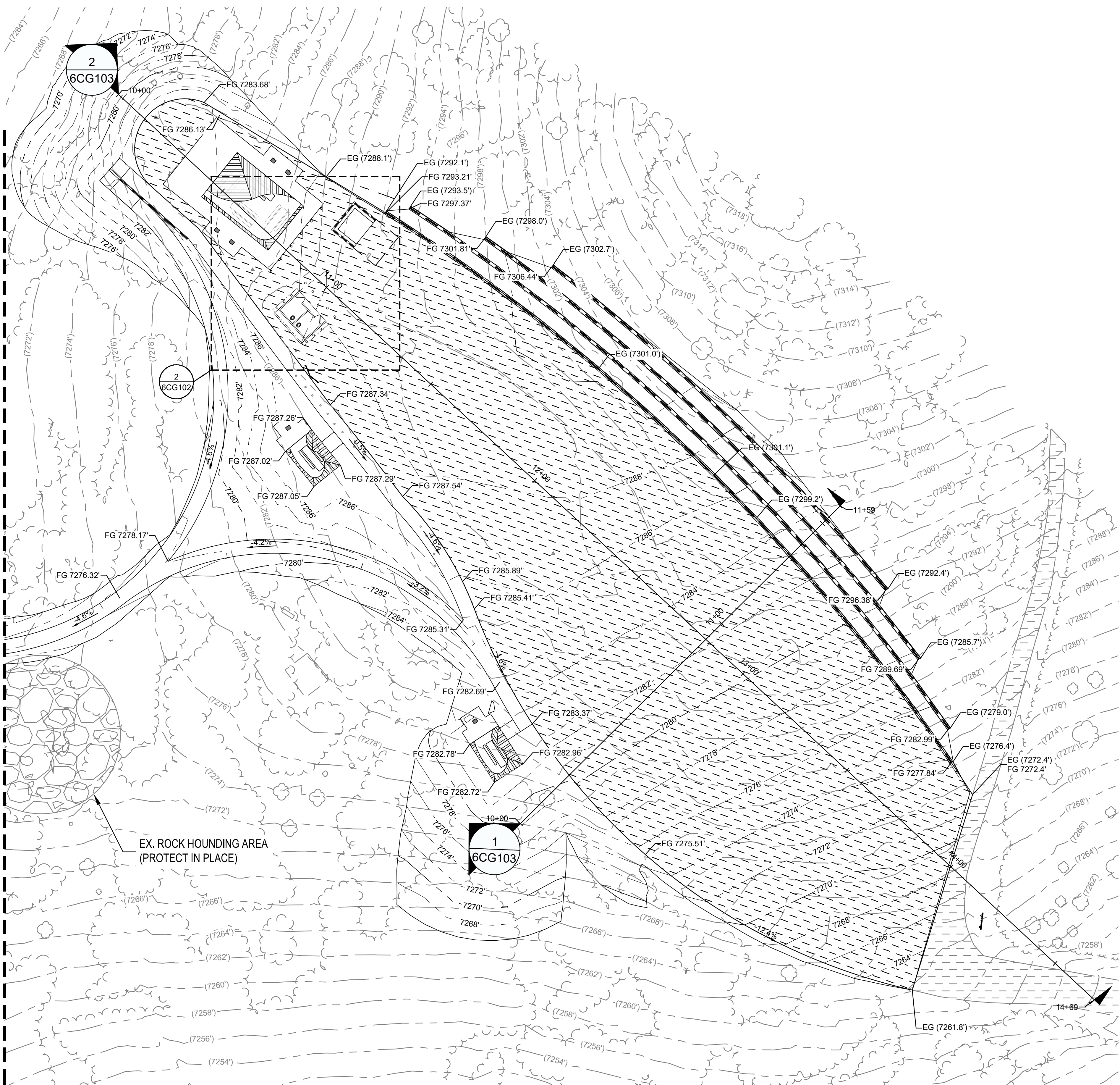
GARNET HILL MAIN TRAIL PARKING AREA
