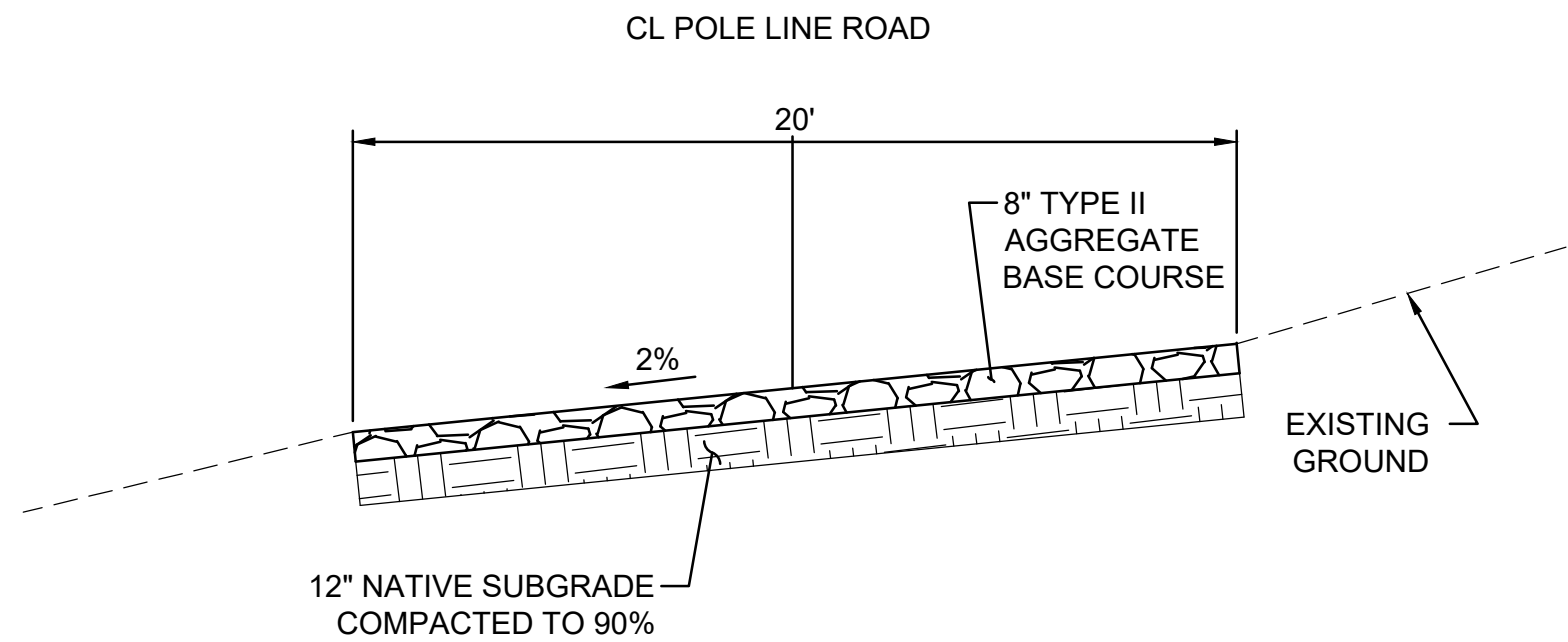
TYPICAL SECTION NOT TO SCALE 1
