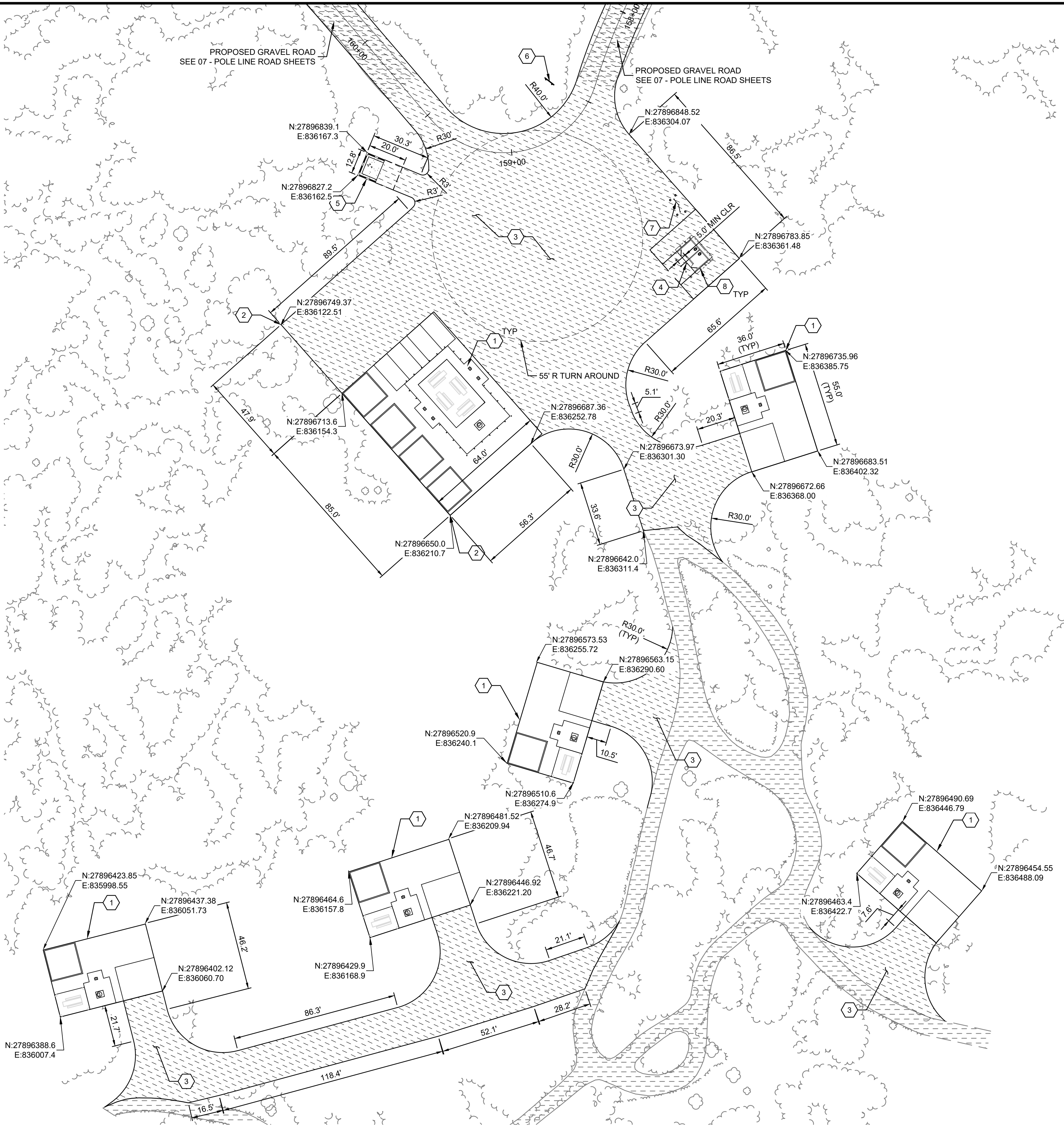
UPPER CAMPGROUND SITE PLAN 1" = 30'
