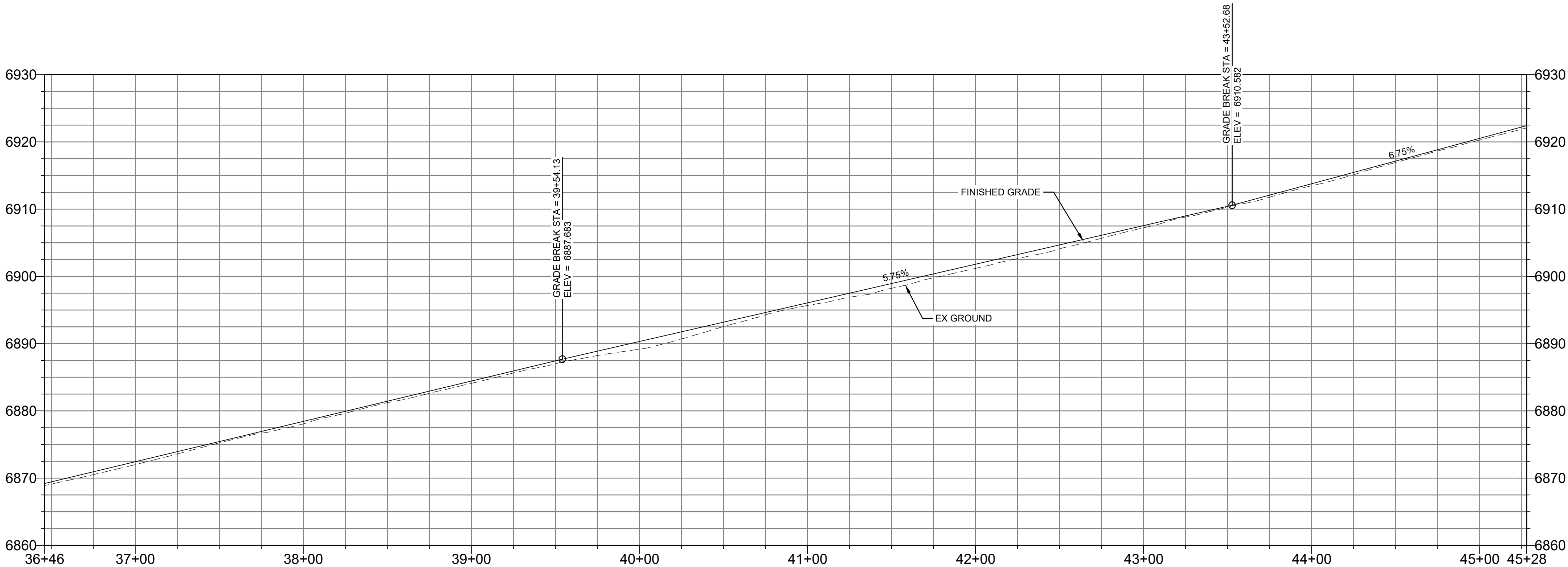
POLE LINE ROAD PLAN & PROFILE HORIZ: 1" = 40' | VERT: 1" = 4'
