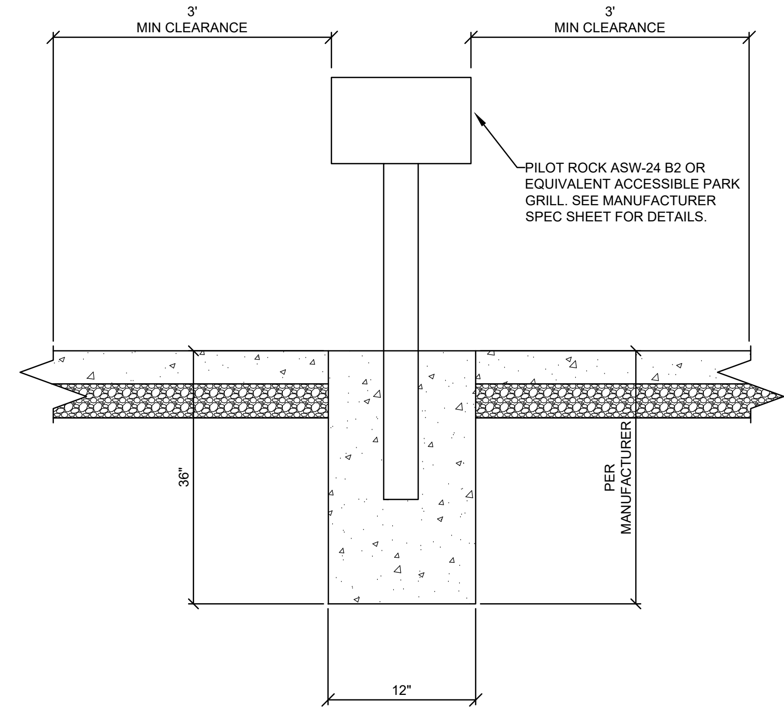
GRILL FOUNDATION DETAIL
