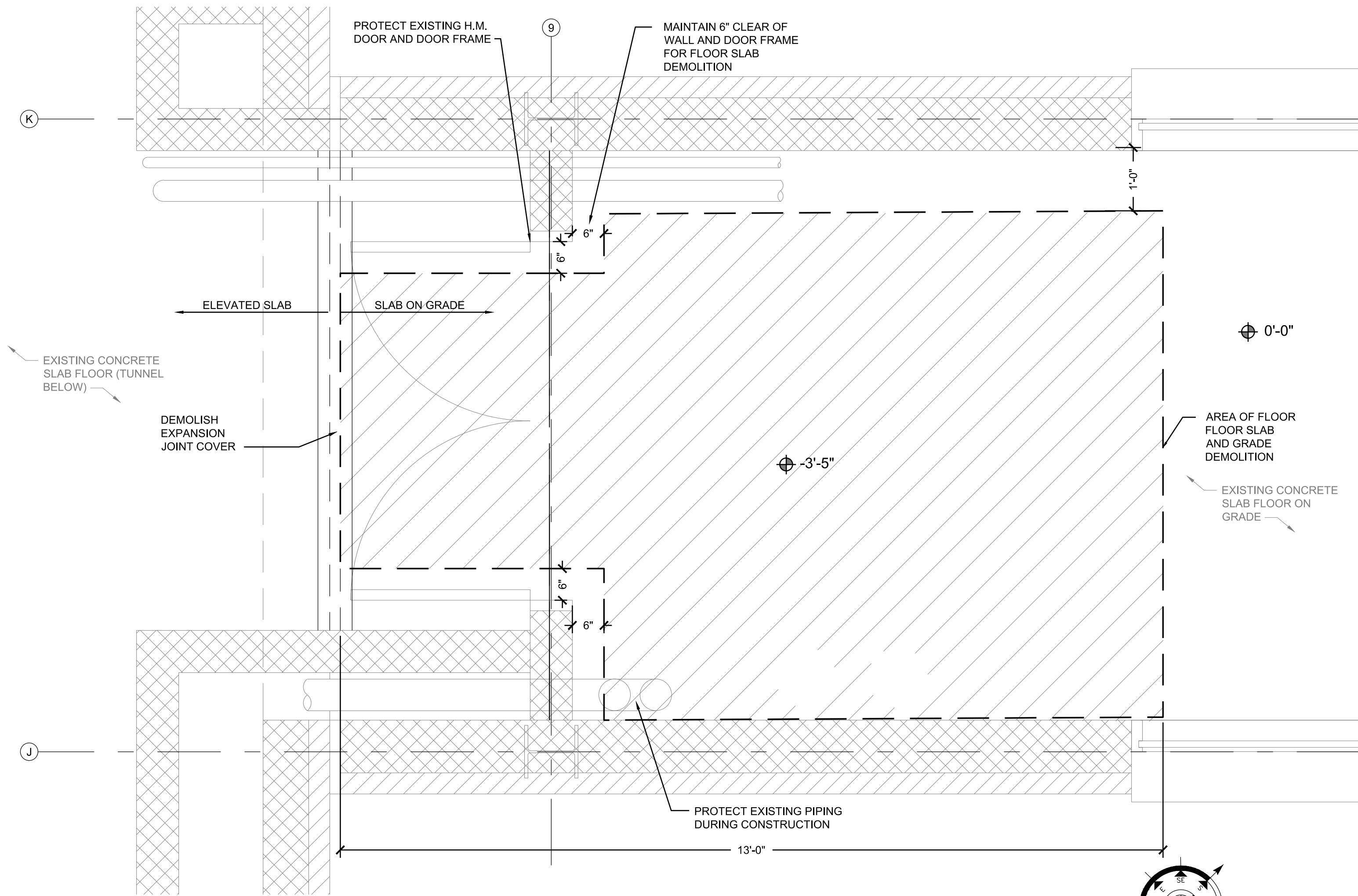
C2 ENLARGED DEMOLITION PLAN SCALE: 3/4" = 1'-0"
