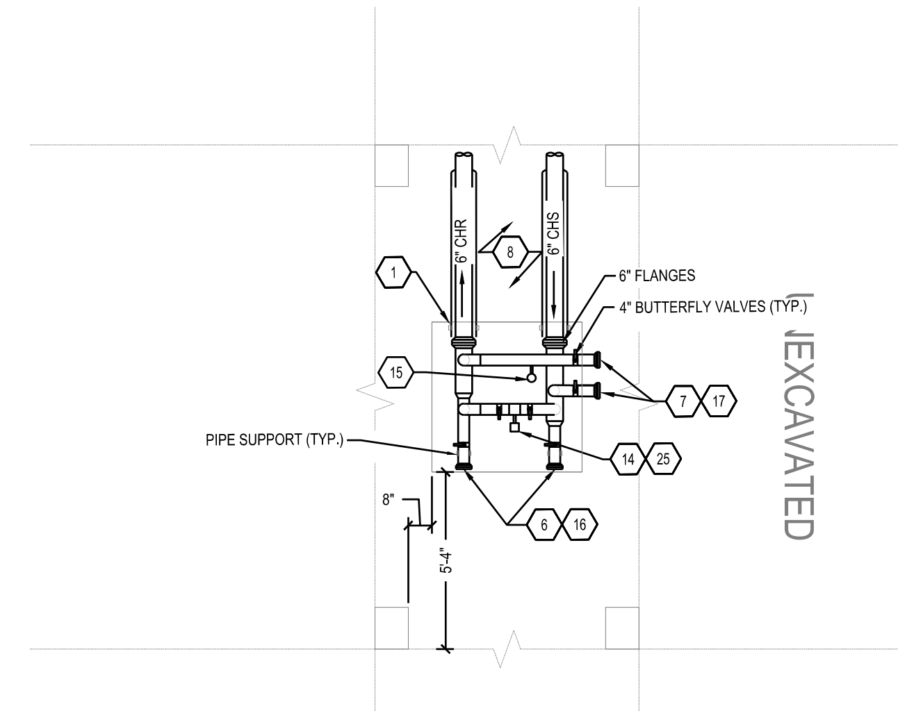
PARTIAL BUILDING 3 CRAWL SPACE CHILLED WATER PIPING PLAN SCALE: 1/2" = 1'-0"
