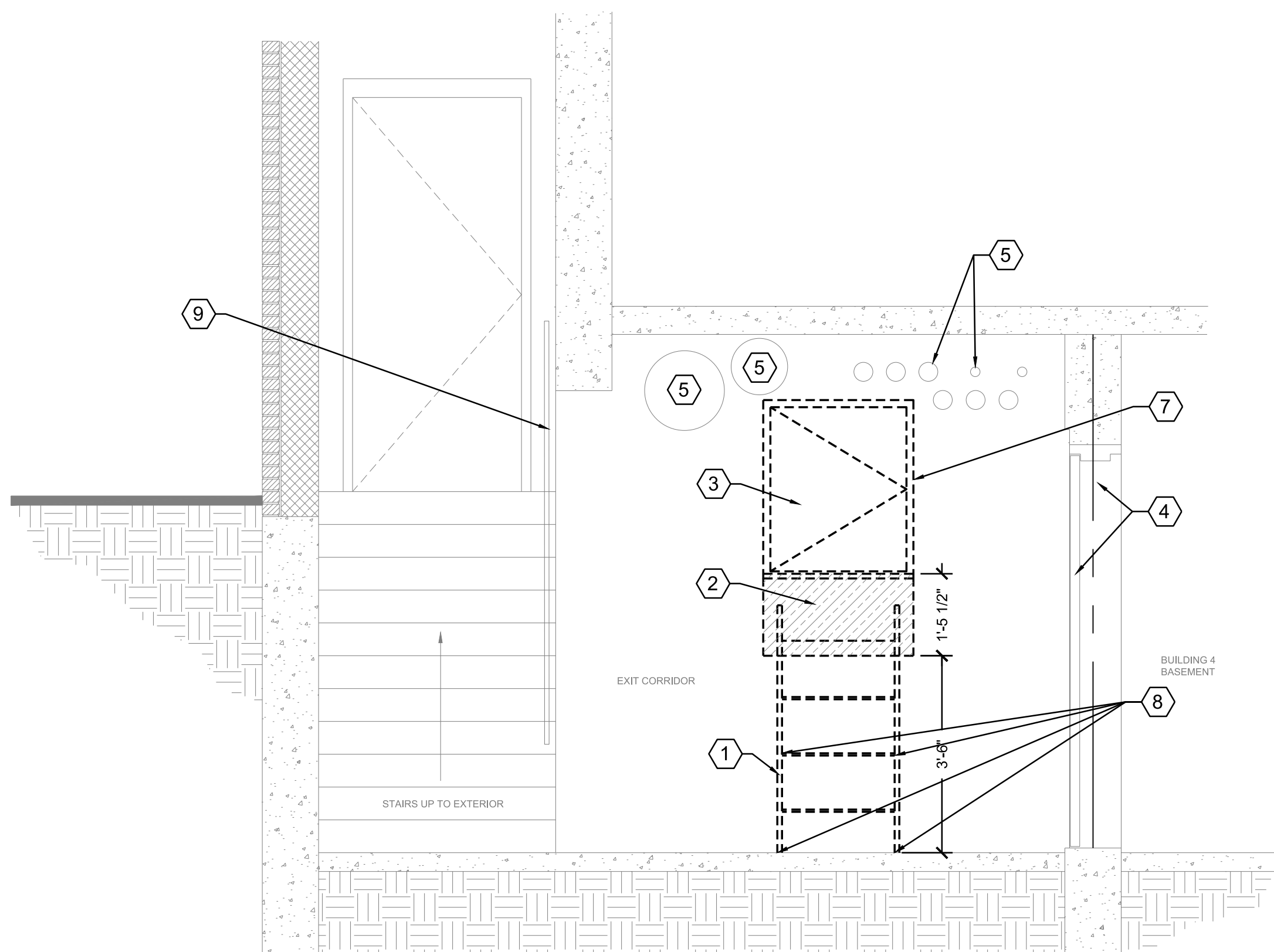
DEMOLITION SECTION FOR EXIT CORRIDOR AT BUILDING 4 (C7) SCALE: 1/2" = 1'-0" 0 1' 2' 4'
