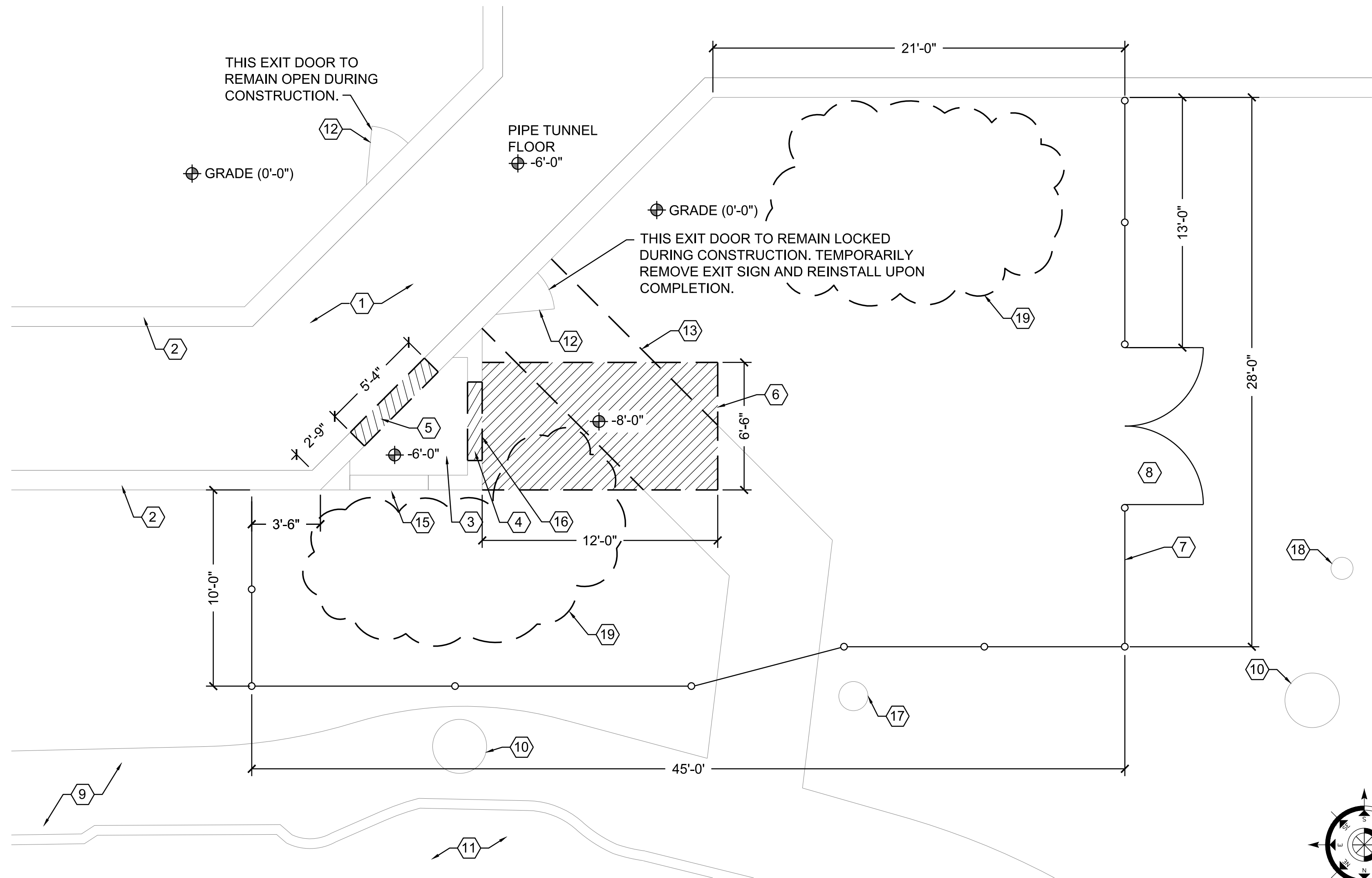
C2 ENLARGED DEMOLITION PLAN SCALE: 3/4" = 1'-0"
