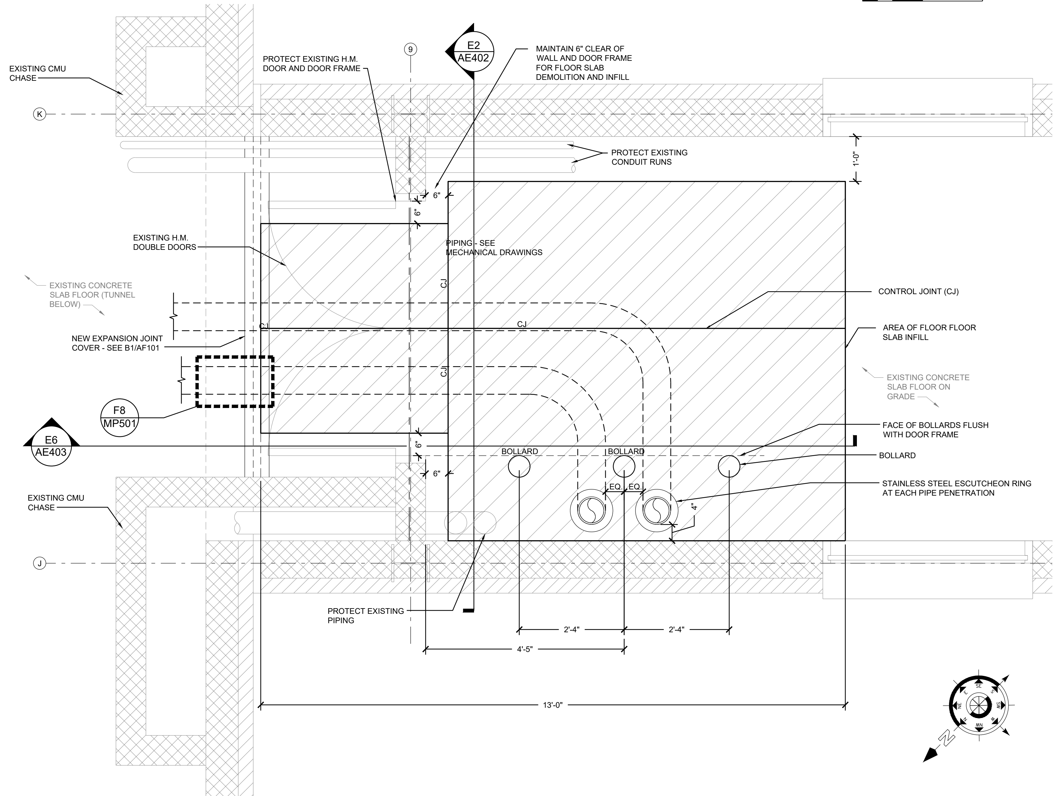
E6 CORRIDOR PLAN SCALE: 3/4" = 1'-0"
