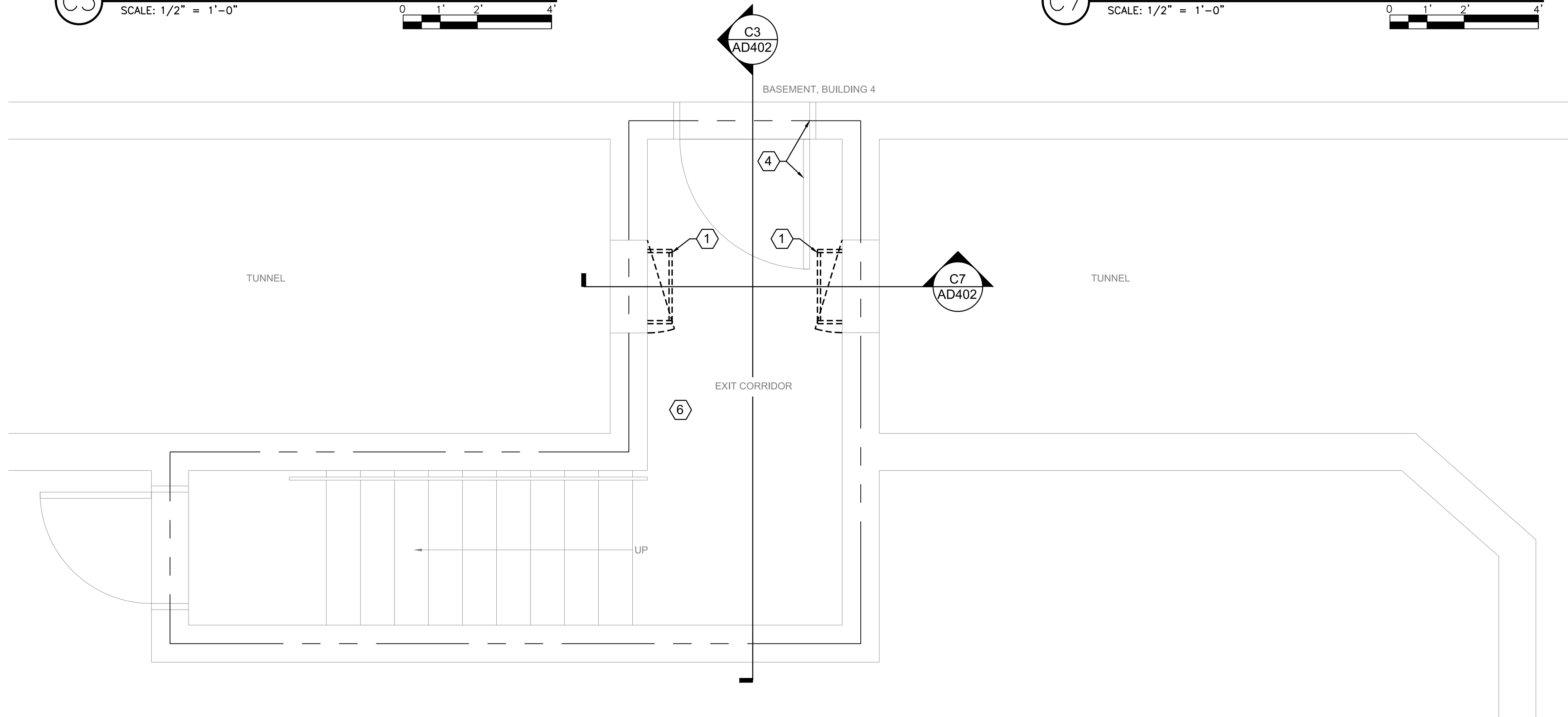
DEMOLITION PLAN FOR EXIT CORRIDOR CORRIDOR AT BUILDING 4 E6 SCALE: 1/2" = 1'-0" 0 1' 2' 4'
