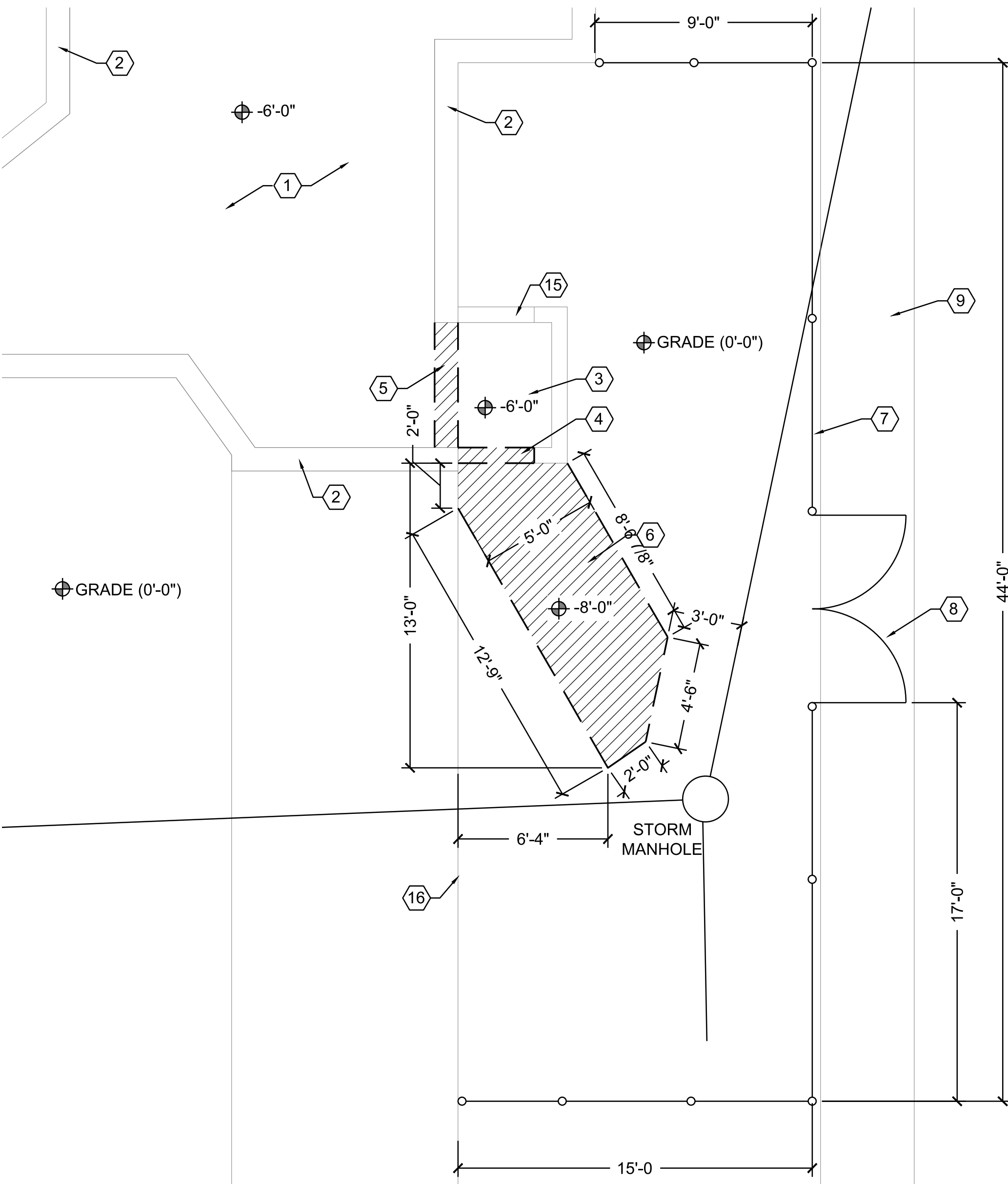
F3 ENLARGED DEMOLITION PLAN SCALE: 1/4" = 1'-0"
