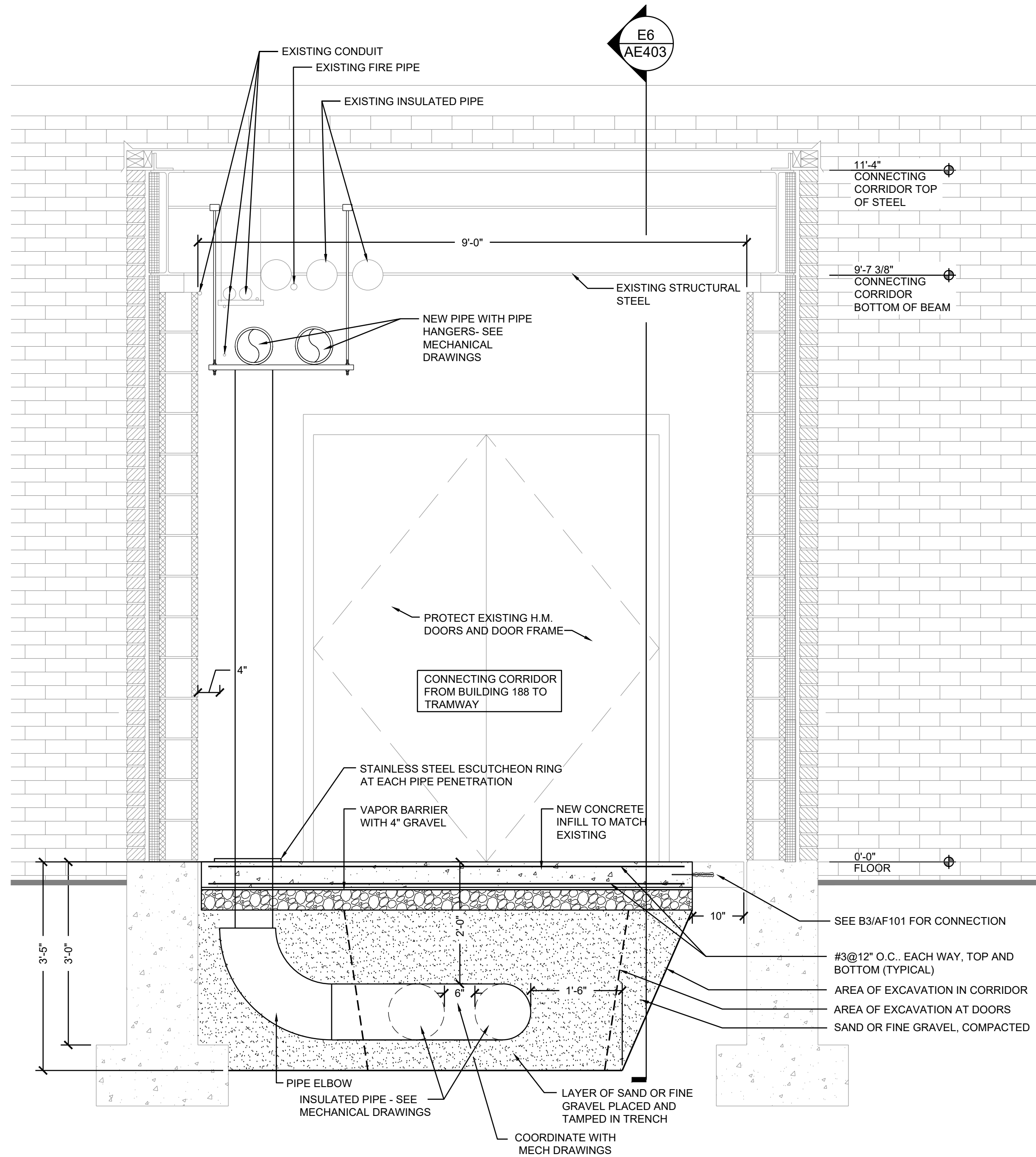
E2 CORRIDOR SECTION SCALE: 3/4" = 1'-0"
