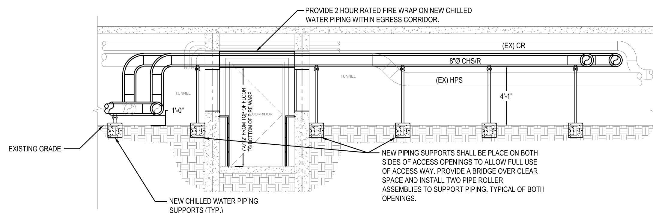
F3 TUNNEL SECTION SCALE: 1/4" = 1'-0"
