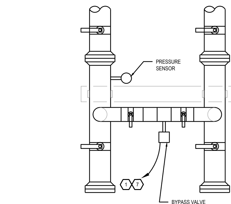
DEDUCT ALTERNATE NO. 1: E8 CHILLED WATER PIPING BYPASS SCALE: NONE
