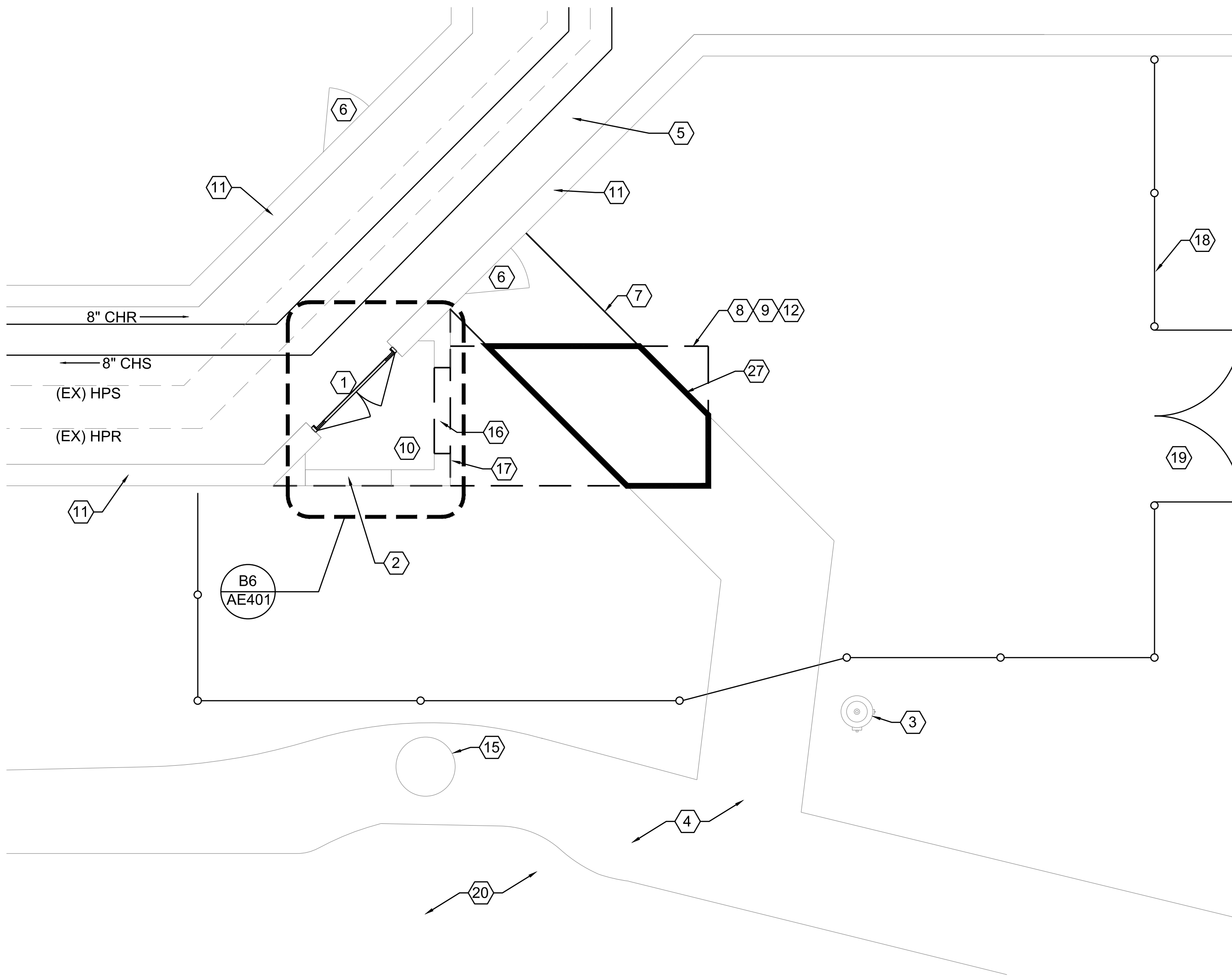
ENLARGED SITE PLAN PIPE FEED LOCATION F4 SCALE: 1/4" = 1'-0" 0 2' 4'
