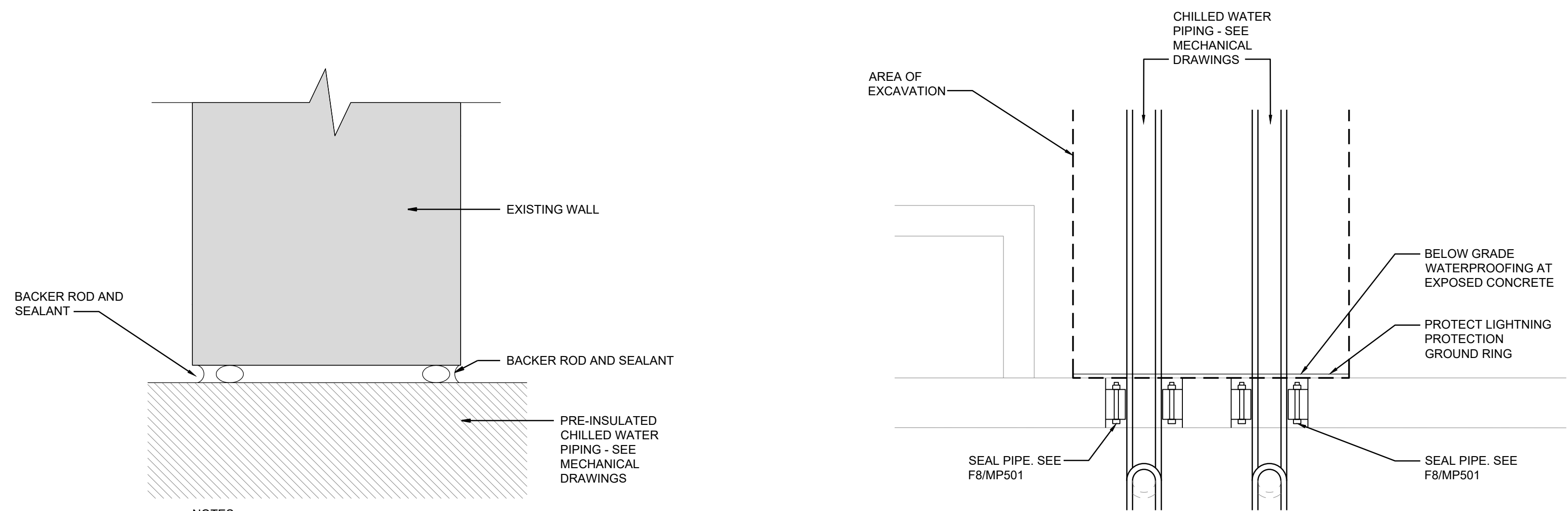
SECTION-MECHANICAL PENETRATION TRAMWAY WALL SCALE: NONE
