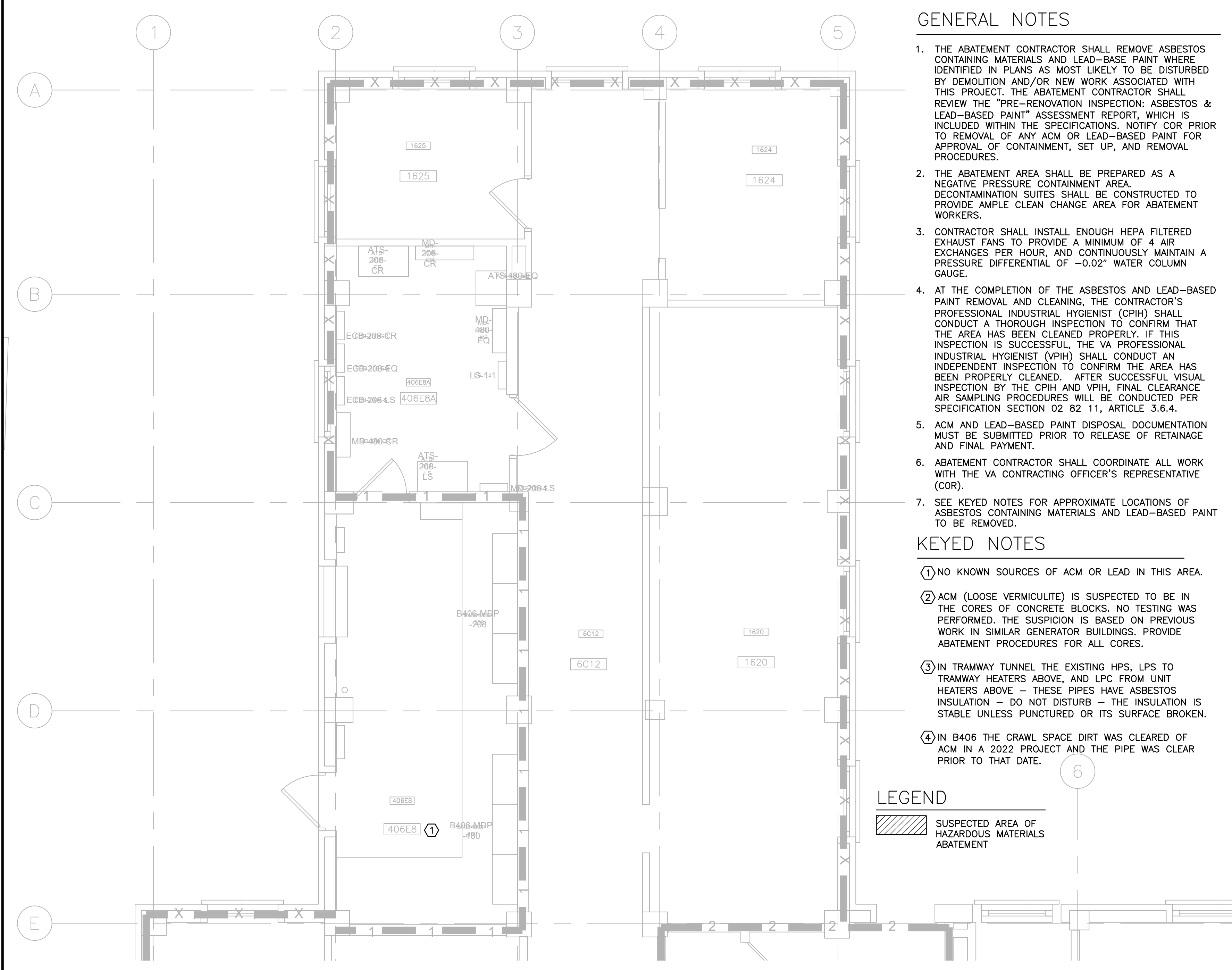
2 PARTIAL FIRST FLOOR PLAN - B406 1/4"= 1'-0"
