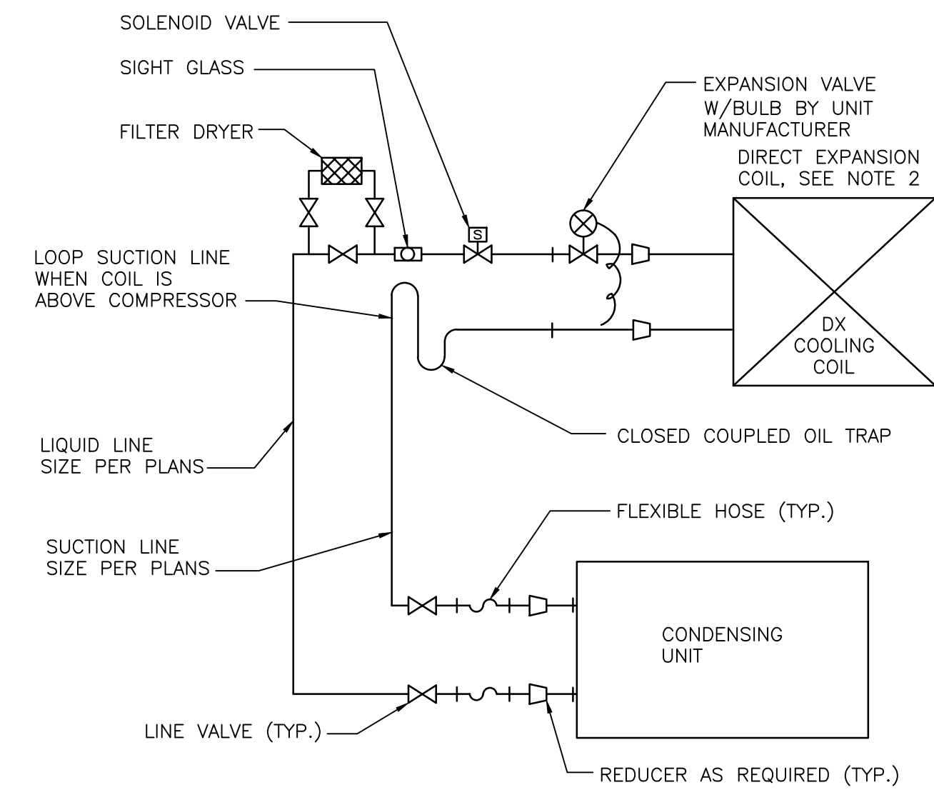
4 SPLIT DX SYSTEM REFRIGERANT PIPING DIAGRAM
