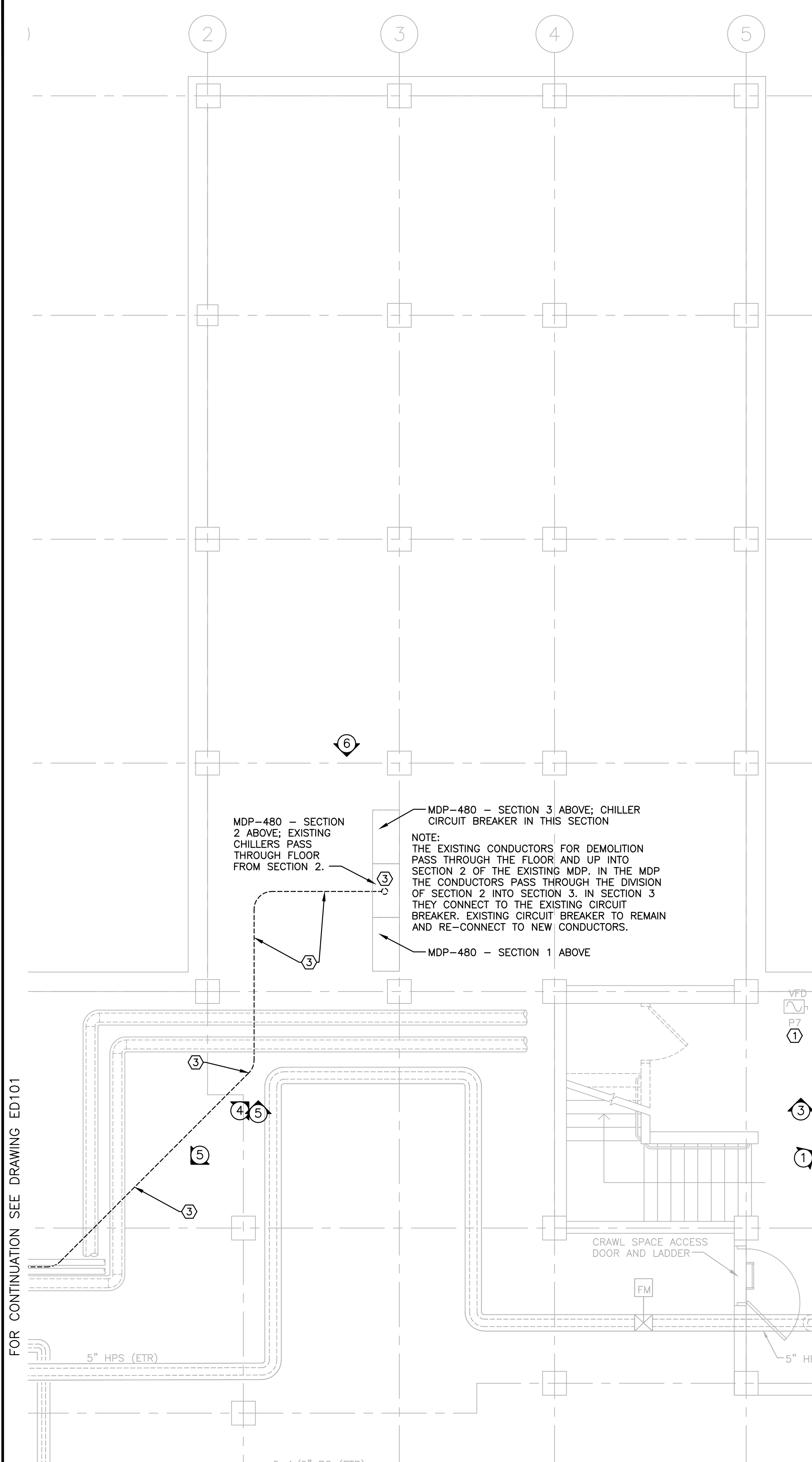
1 CRAWLSPACE/ MECHANICAL ROOM PLAN 1/4"= 1'-0" NORTH
