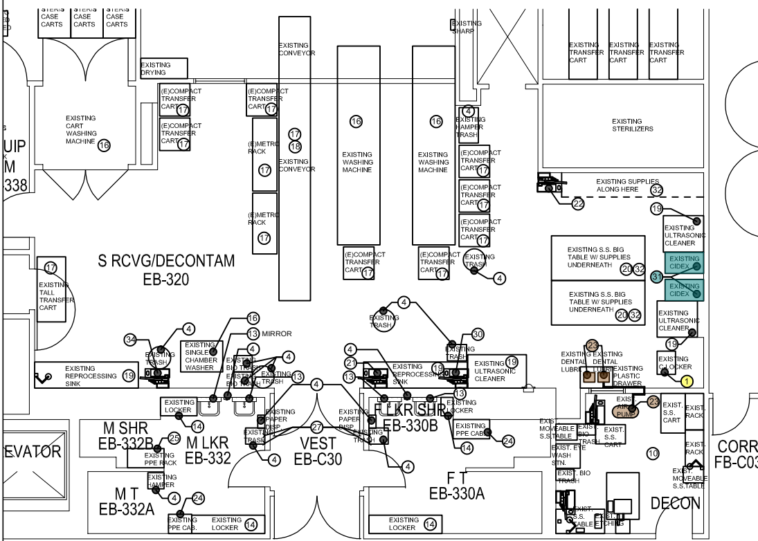
3 ENLARGED PARTIAL EXISTING B-100 BASEMENT IN SPS DECONT. AREA FLOOR PLAN
