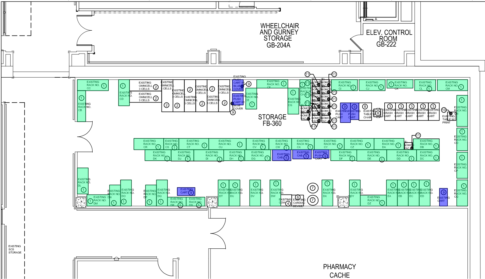
1 ENLARGED PARTIAL EXISTING B-100 BASEMENT ROOM FB-360 FLOOR PLAN 1/8" = 1'-0"
