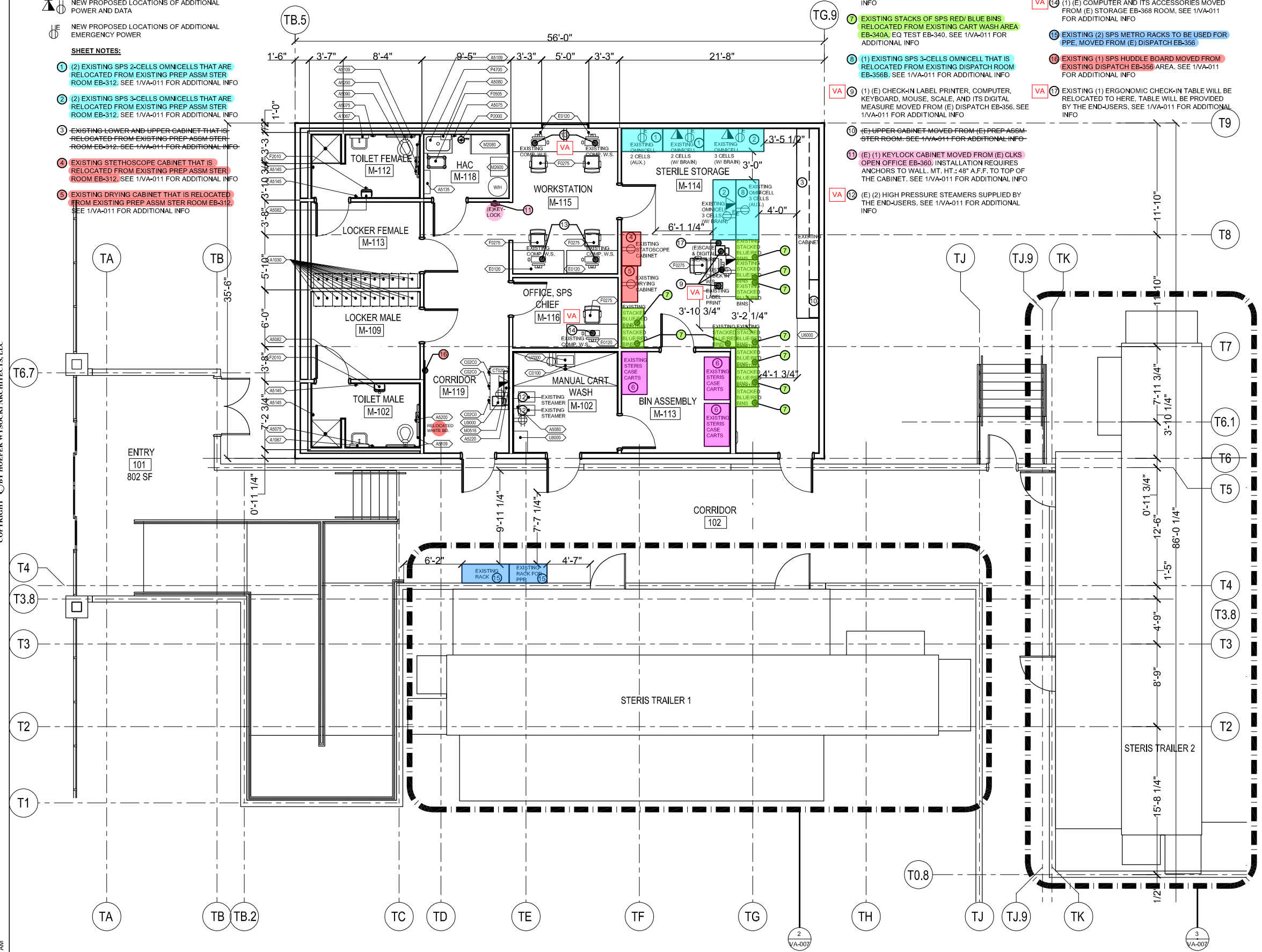
1 NEW SPS TEMP. MODULAR BUILDING 1 FLOOR PLAN
