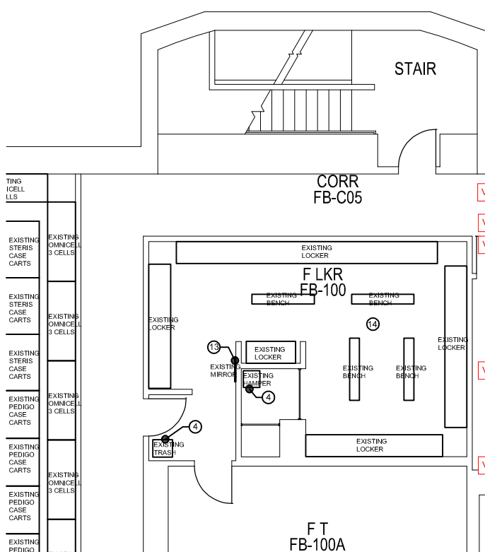
2 ENLARGED PARTIAL EXISTING B-100 BASEMENT IN SPS/ SCS FEMALE LOCKER FLOOR PLAN
