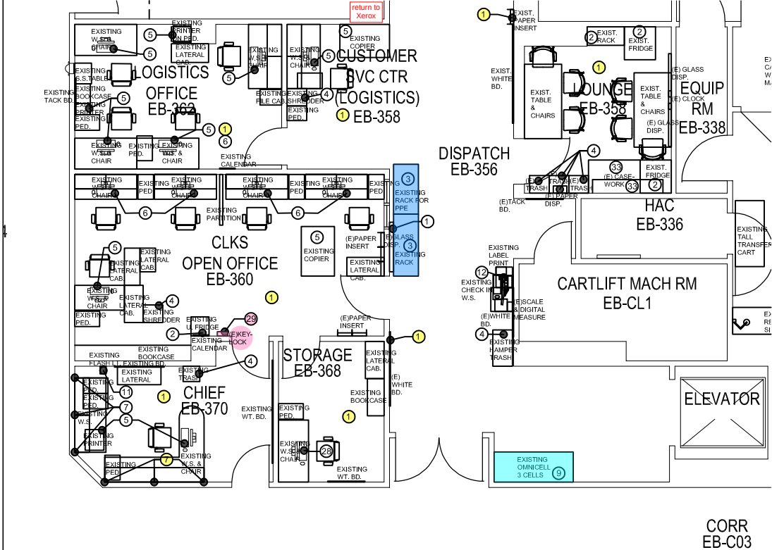
1 ENLARGED PARTIAL EXISTING B-100 BASEMENT IN SPS/ SCS OFFICES FLOOR PLAN
