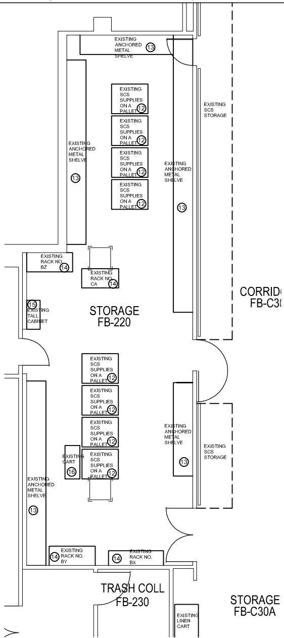
2 ENLARGED PARTIAL EXISTING B-100 BASEMENT ROOM FB-220 FLOOR PLAN 1/8" = 1'-0"
