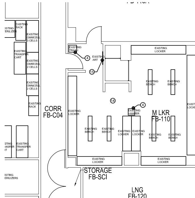
4 ENLARGED PARTIAL EXISTING B-100 BASEMENT IN SPS/ SCS M LOCKER FLOOR PLAN
