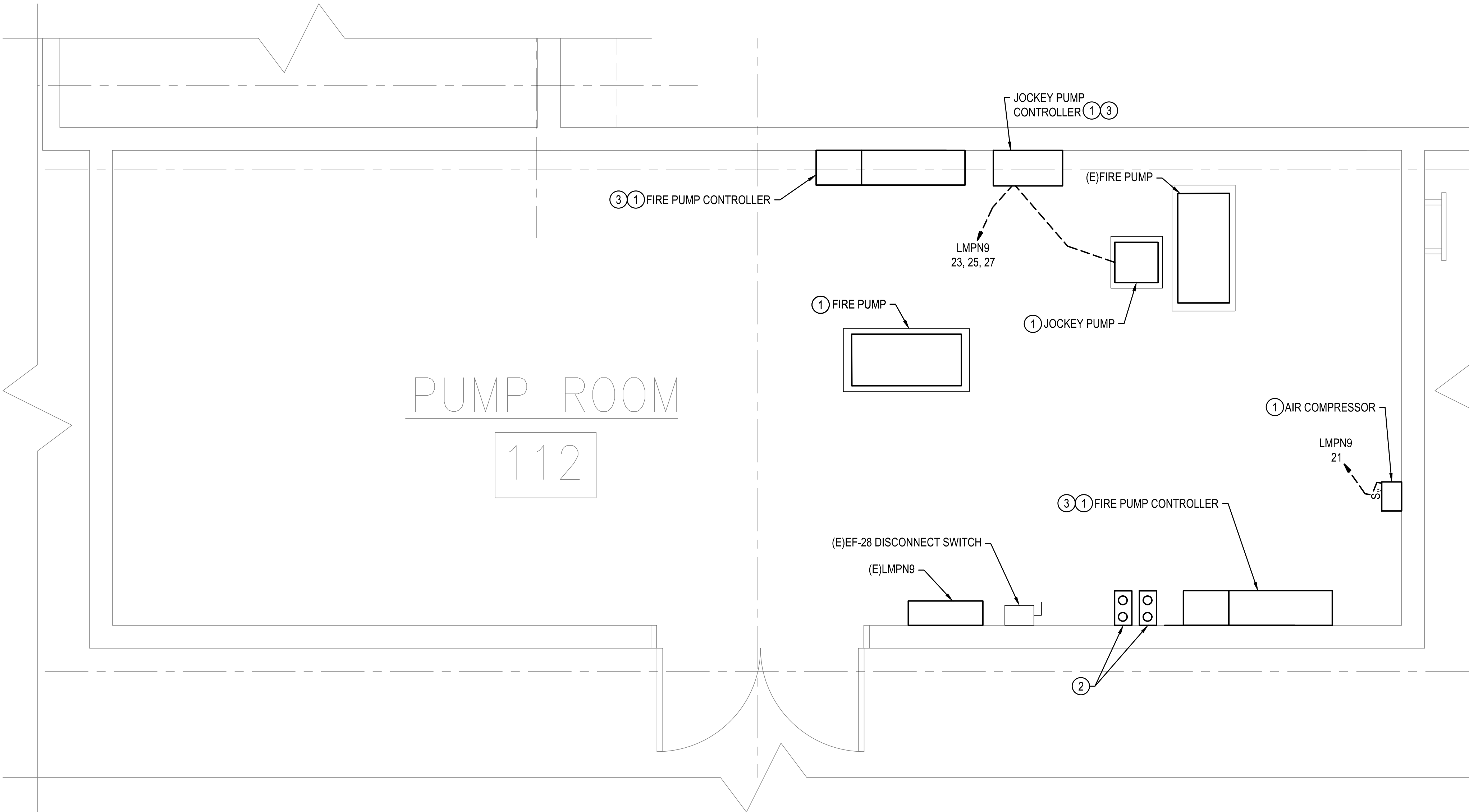
2 DETAIL - PUMP ROOM E-101
