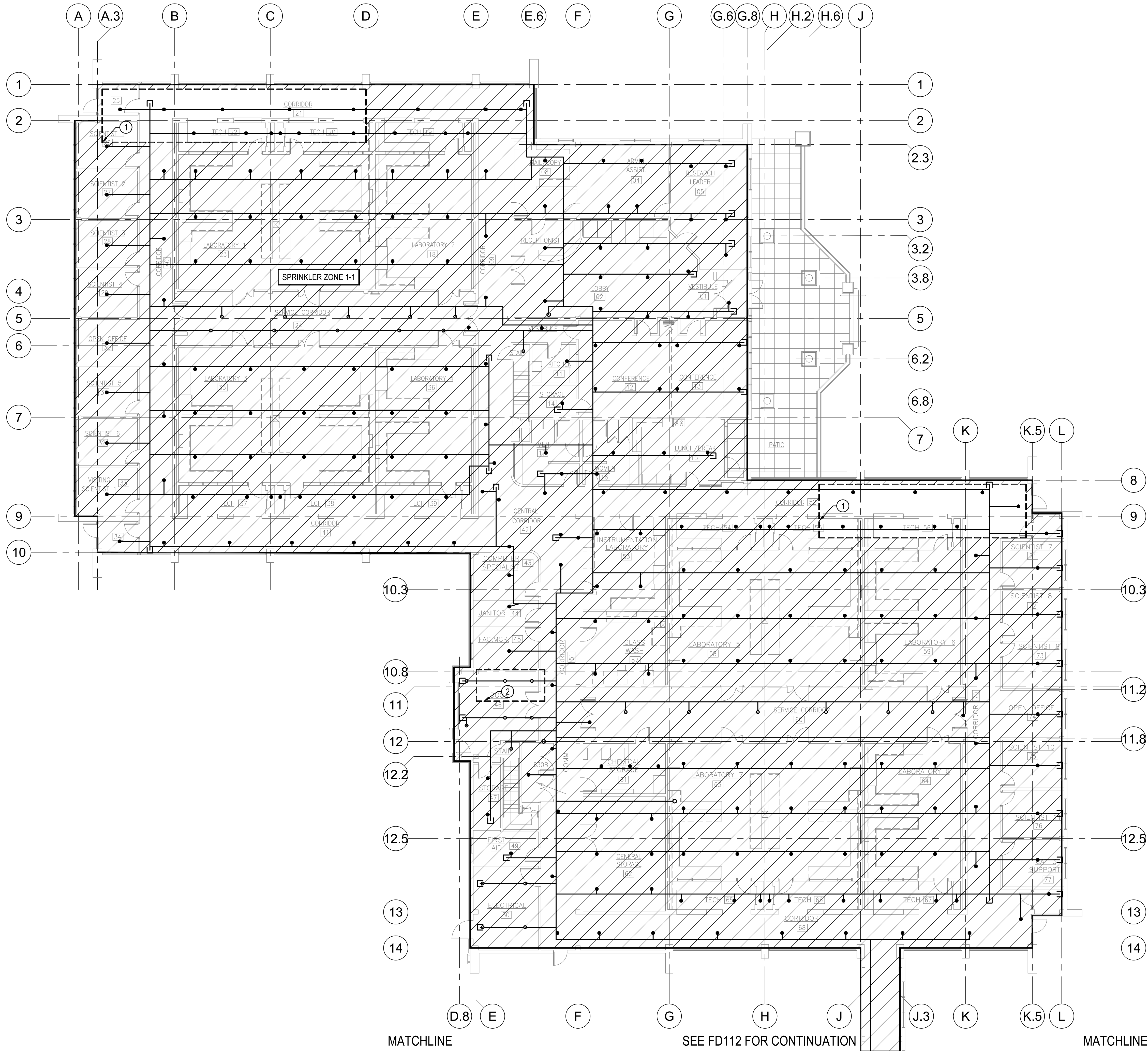
1 FIRST FLOOR MAIN BUILDING - DEMOLITION
