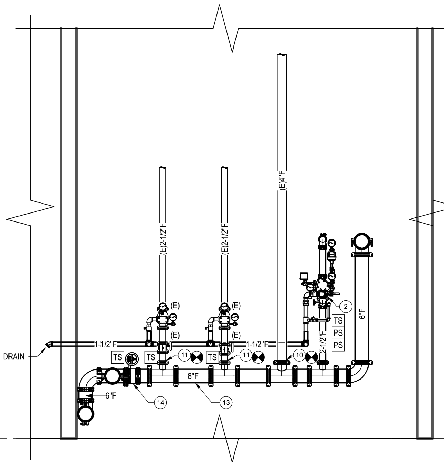
2 RISER DETAIL FX401 1/2"=1'-0"
