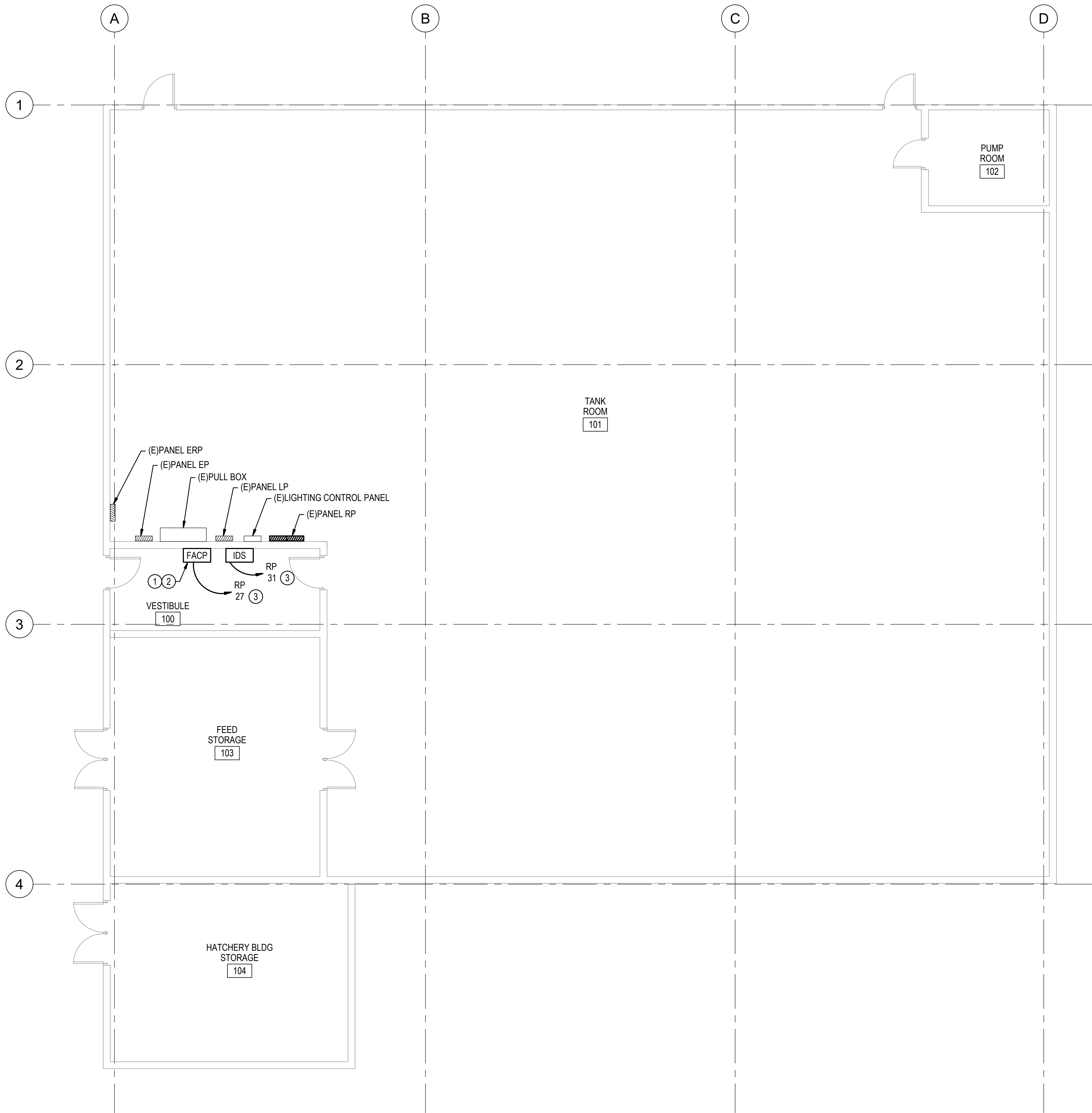
1 BROODSTOCK BUILDING 3/16"=1'-0" 0 4' 8' 12'
