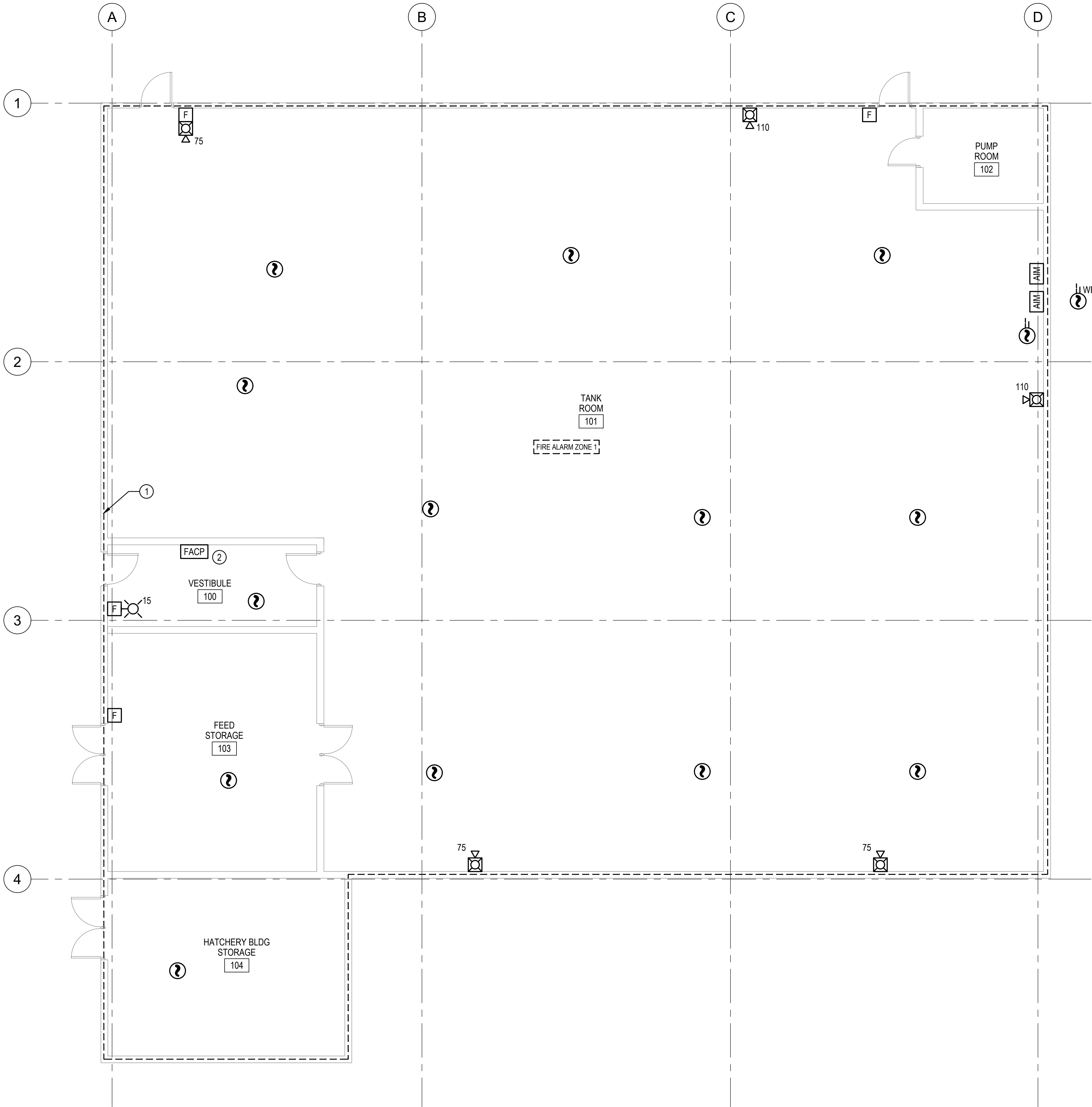
1 BROODSTOCK BUILDING - DEMOLITION 3/16"=1'-0" 0 4' 8' 12'
