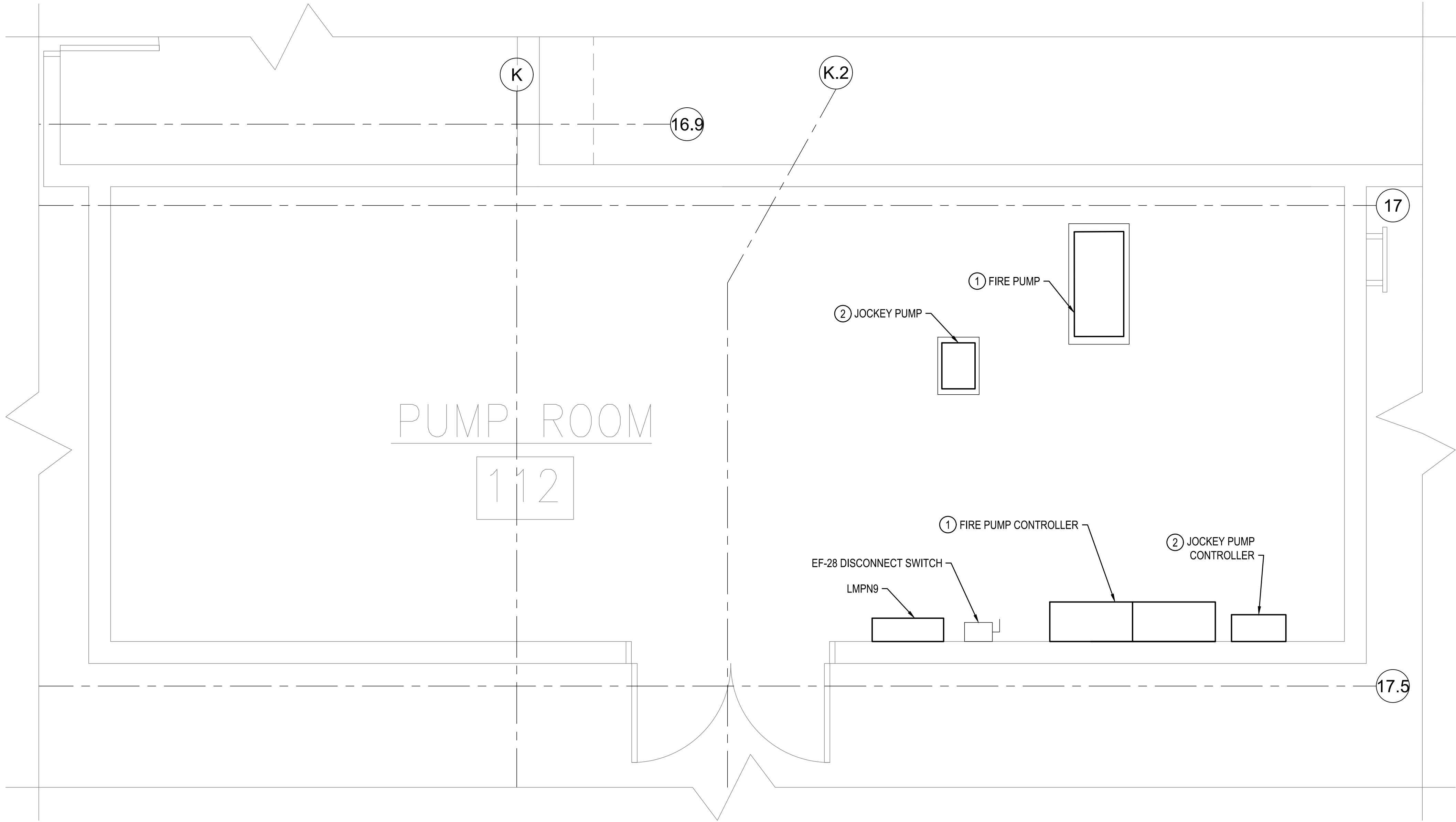
1 DETAIL - PUMP ROOM - DEMOLITION E-101 1/2"=1'-0" 0 2' 4'
