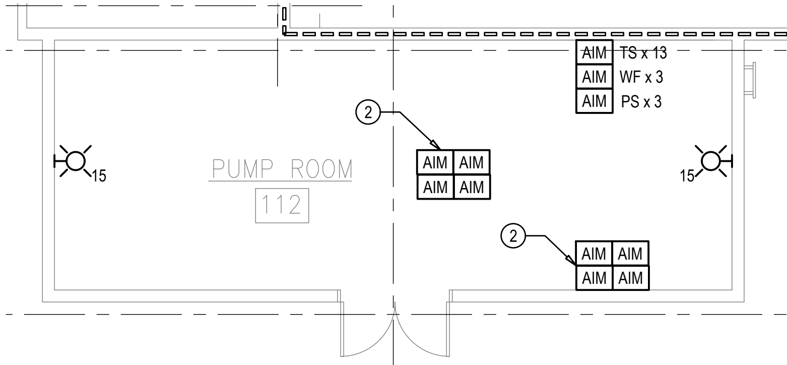
2 ENLARGED PUMP ROOM
