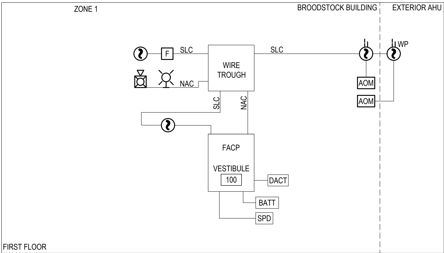
3 FIRE ALARM RISER DIAGRAM - BROODSTOCK NOT TO SCALE
