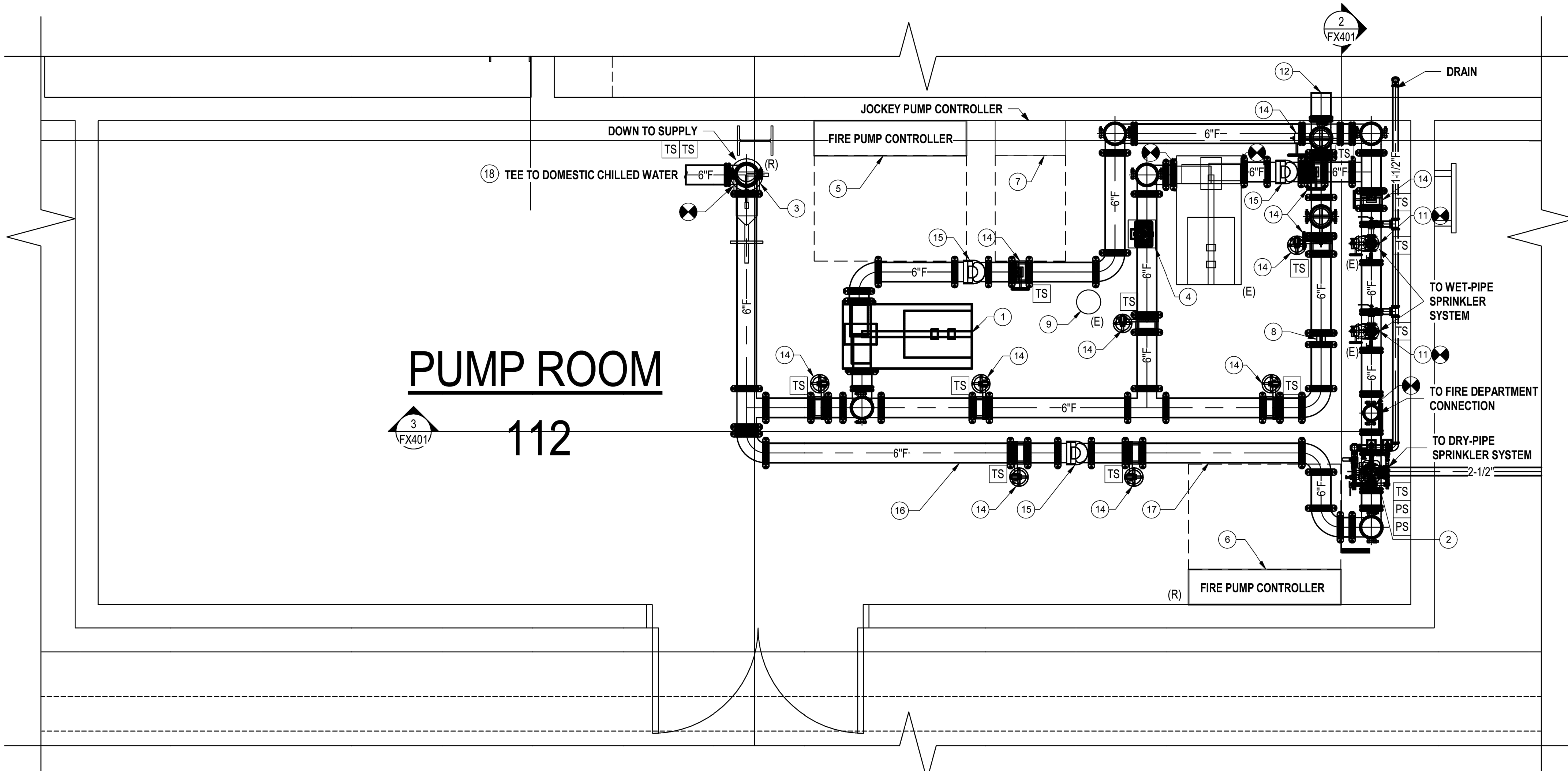
1 FIRE PUMP ROOM DETAIL FX401 1/2"=1'-0"
