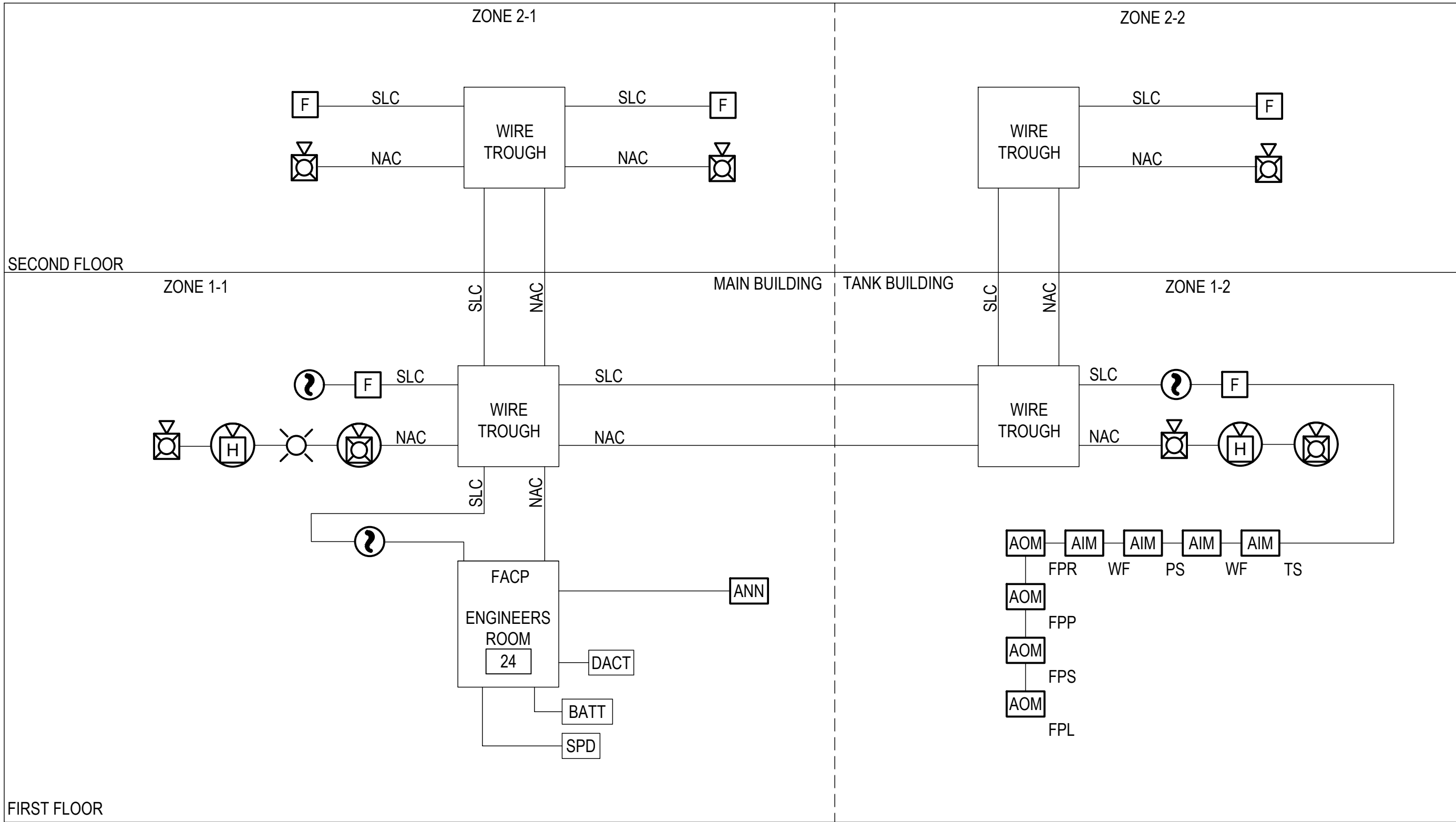
1 FIRE ALARM RISER DIAGRAM NOT TO SCALE
