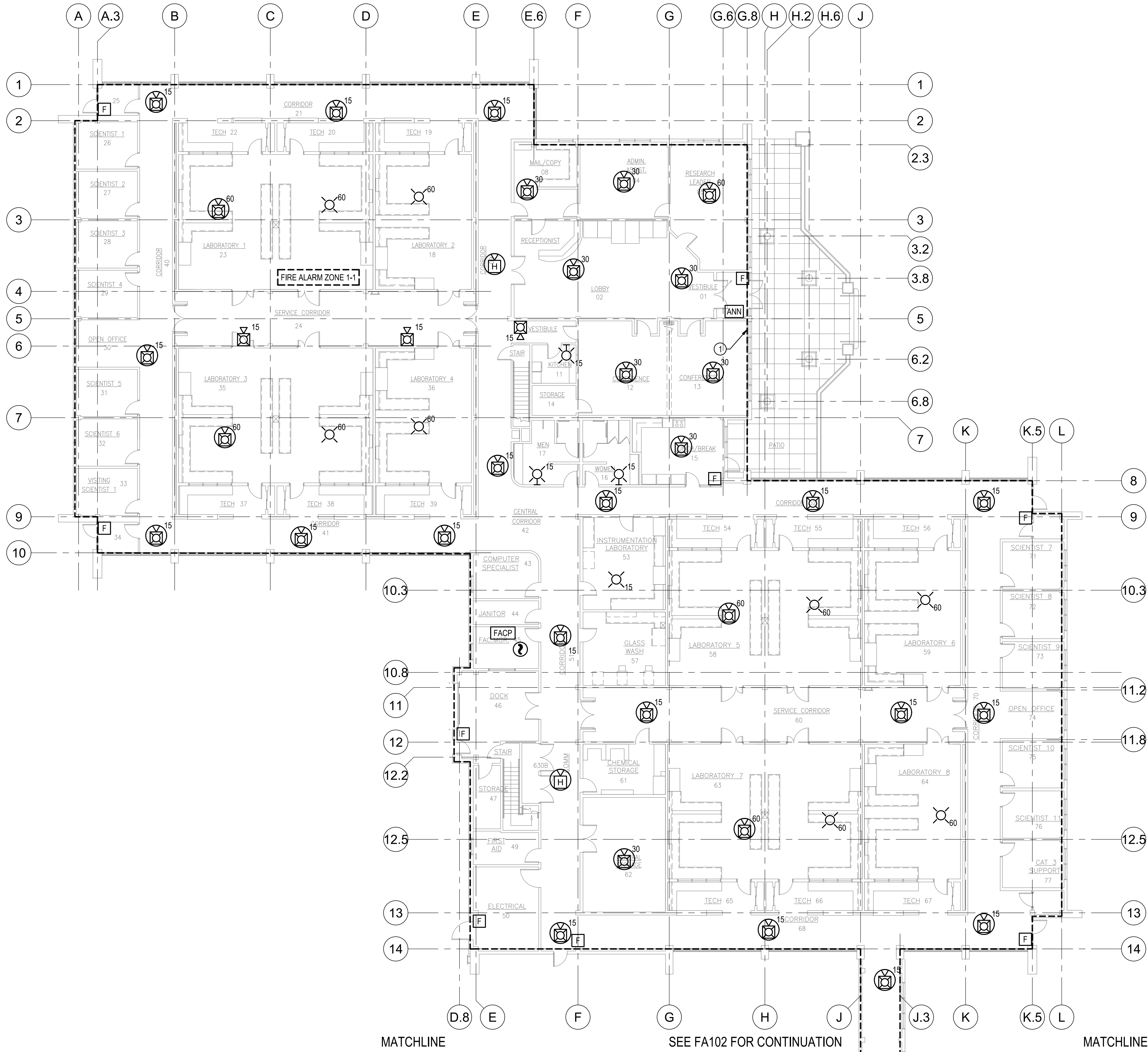
1 FIRST FLOOR MAIN BUILDING 3/32"=1'-0" 0 8 16 24'
