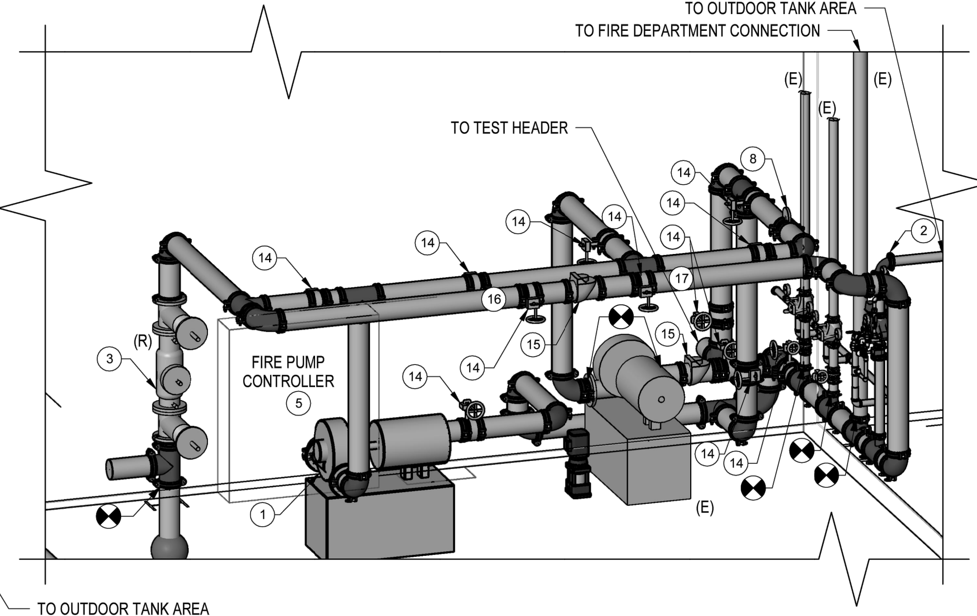
4 FIRE PUMP ROOM 3D VIEW 3/8"=1'-0"
