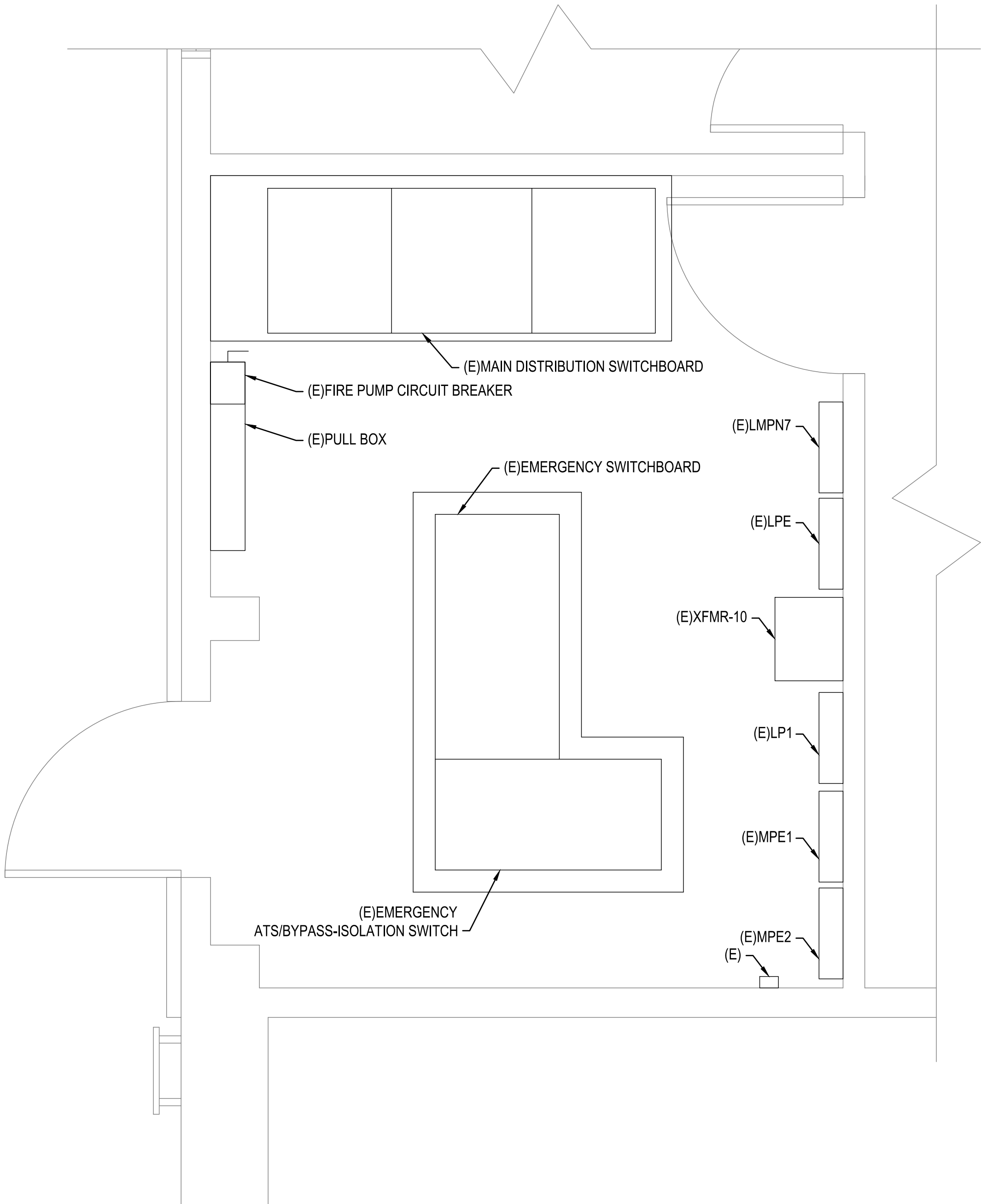
1 DETAIL - ELECTRIC ROOM E-101
