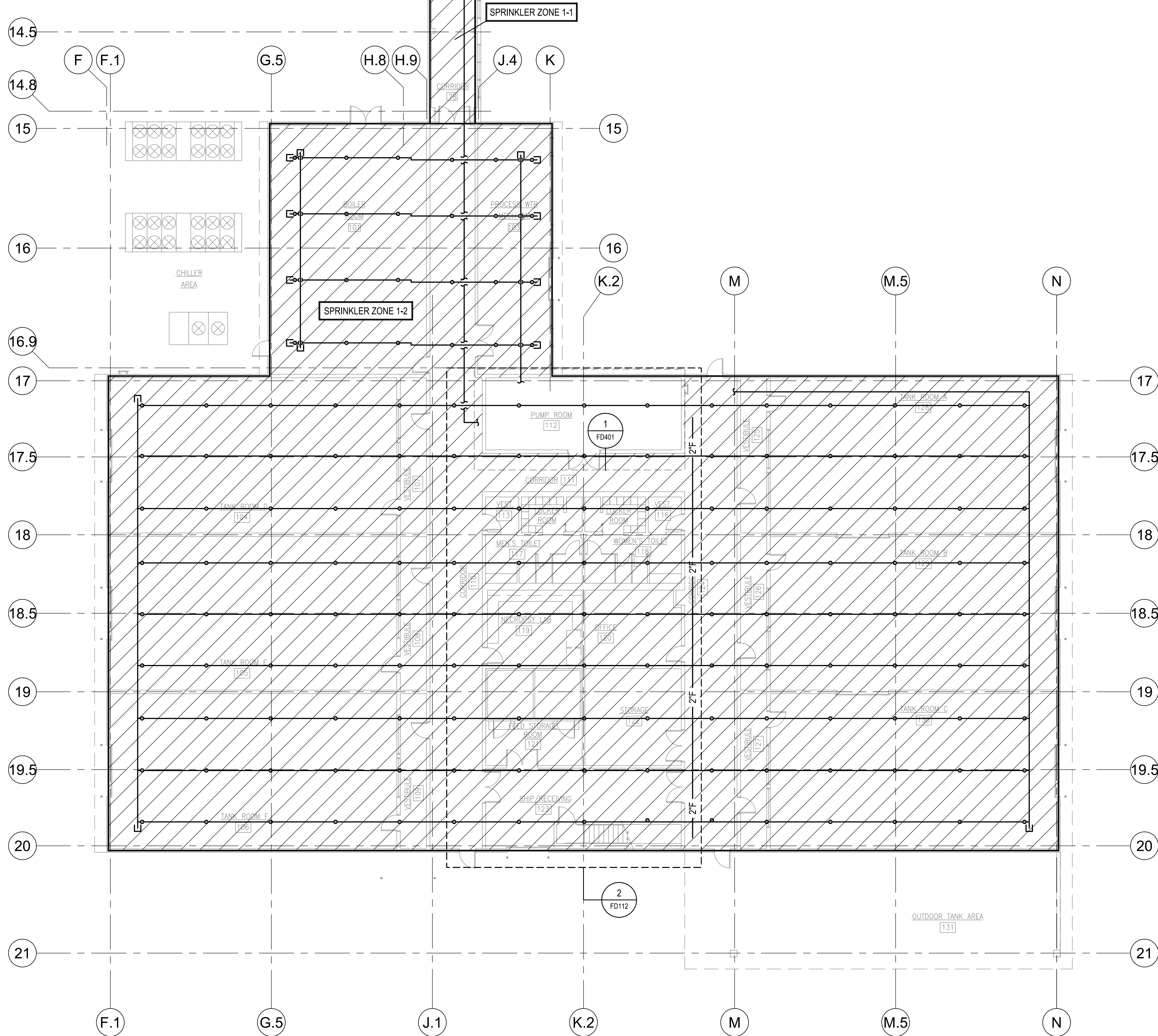
1 ROOF SPRINKLER SYSTEM FIRST FLOOR TANK BUILDING - DEMOLITION
