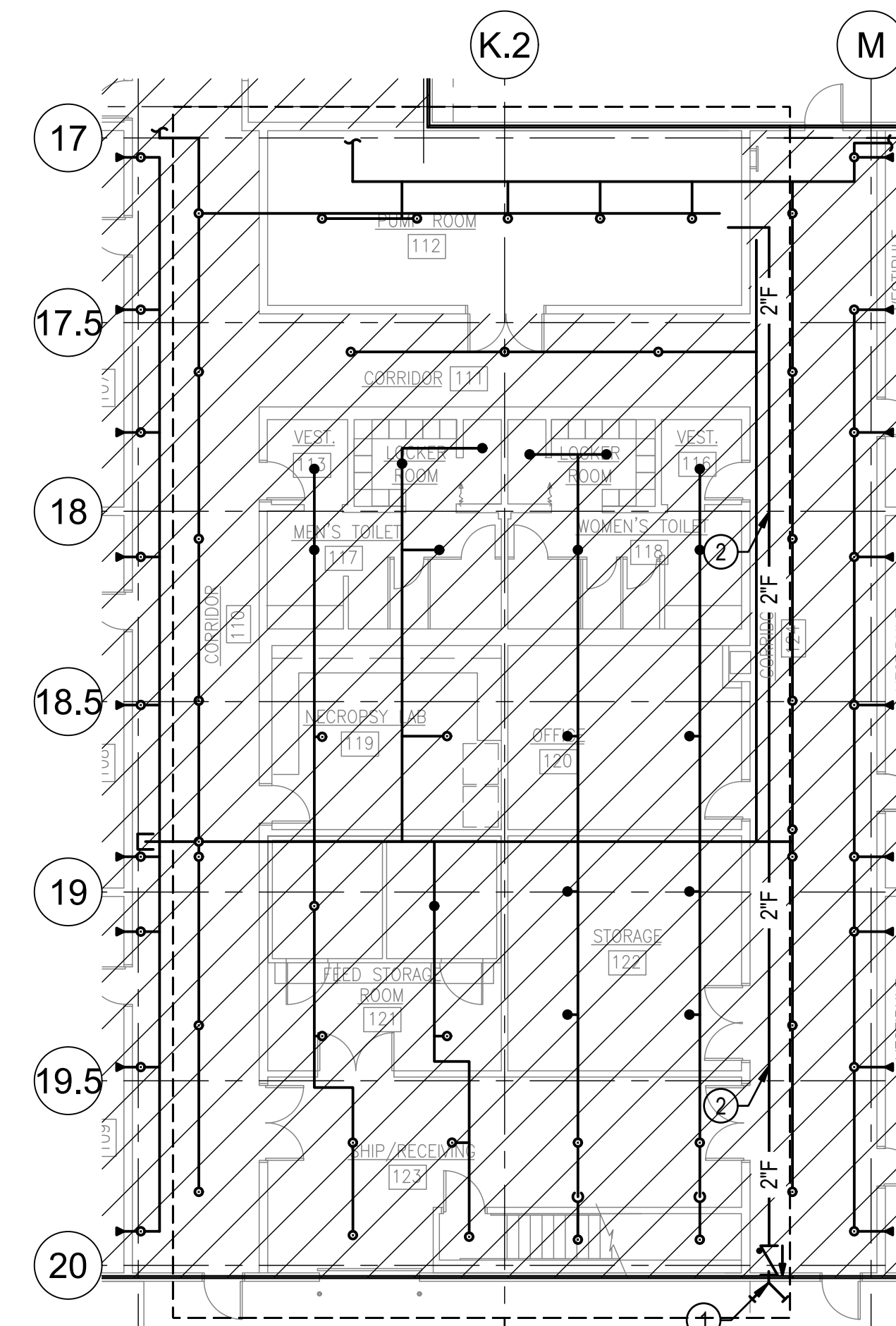
CEILING SPRINKLER SYSTEM FIRST FLOOR TANK BUILDING - DEMOLITION
