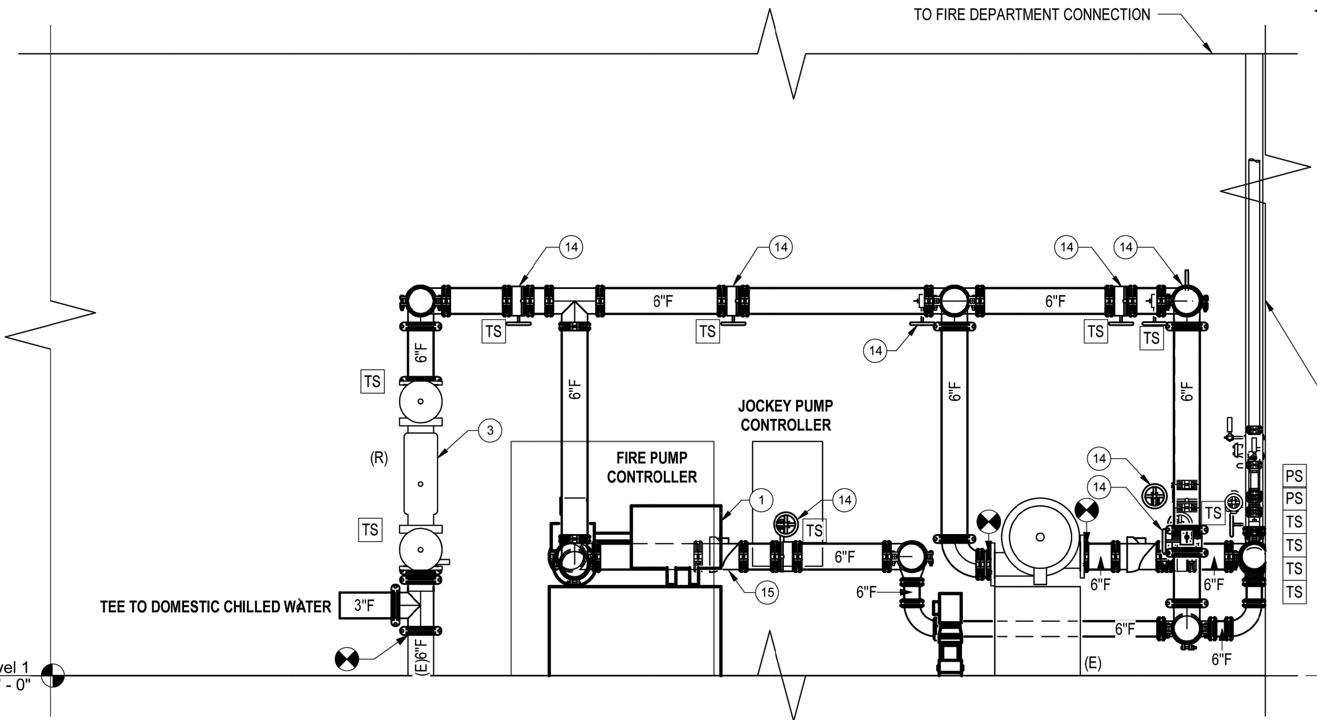
3 FIRE PUMP ROOM FRONT VIEW FX401 1/2"=1'-0"
