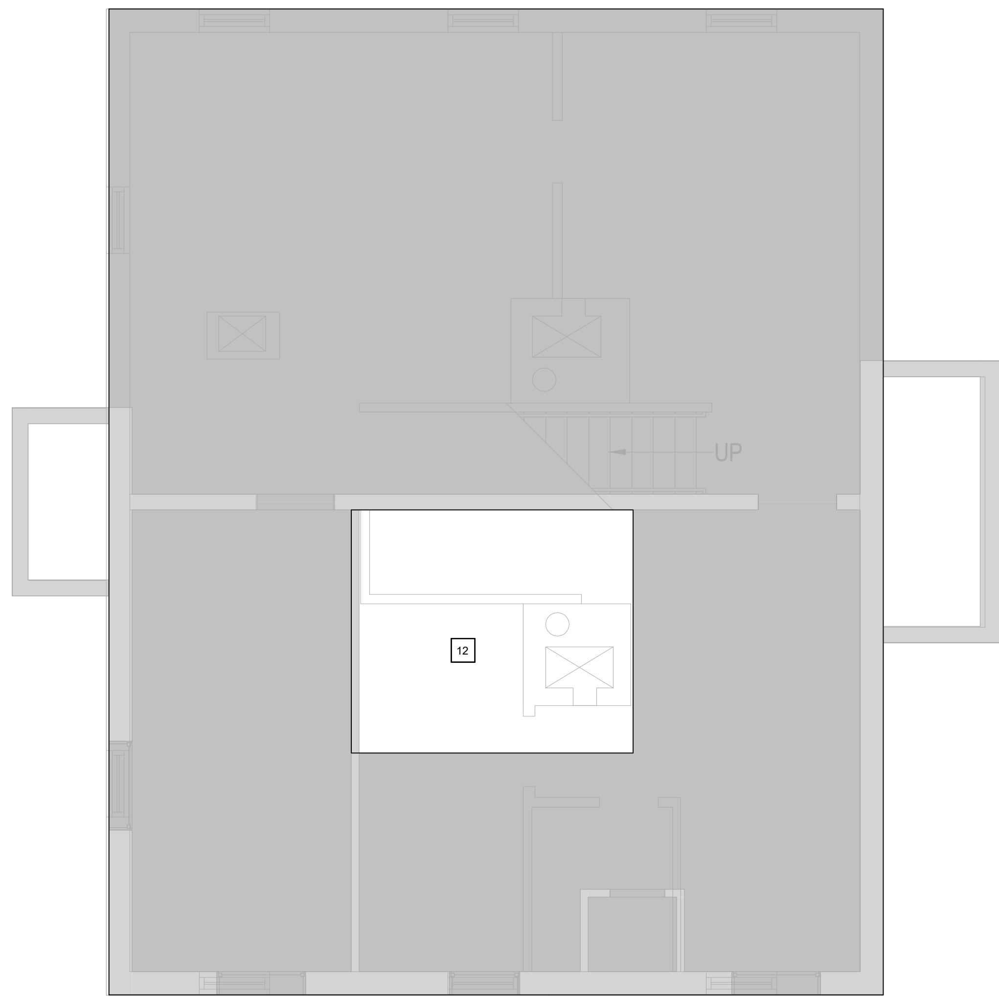
2 BUILDING 109 BASEMENT DEMO RCP 1/4" = 1'-0"
