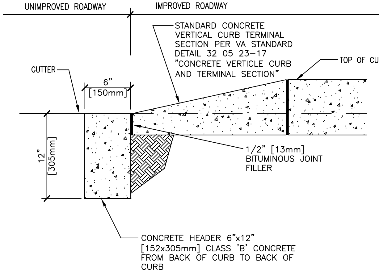
3 CONCRETE HEADER NTS
