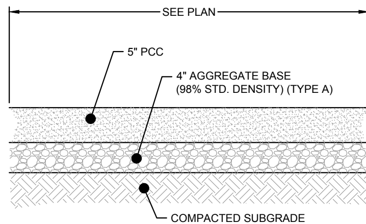
1 PCC SIDEWALK DETAIL NTS
