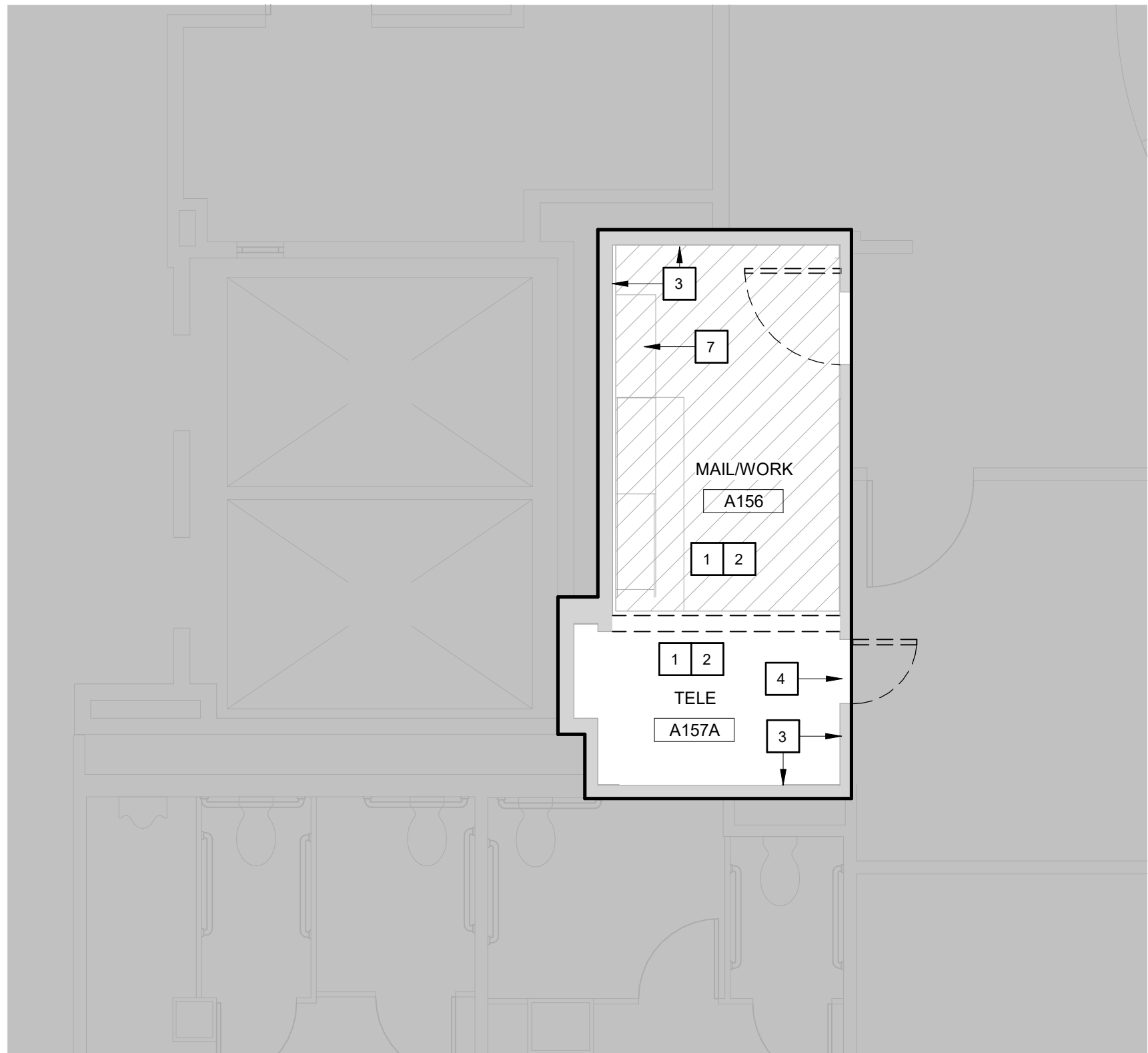
1 BUILDING 43 FIRST FLOOR ENLARGED DEMO PLAN 1/4" = 1'-0"
