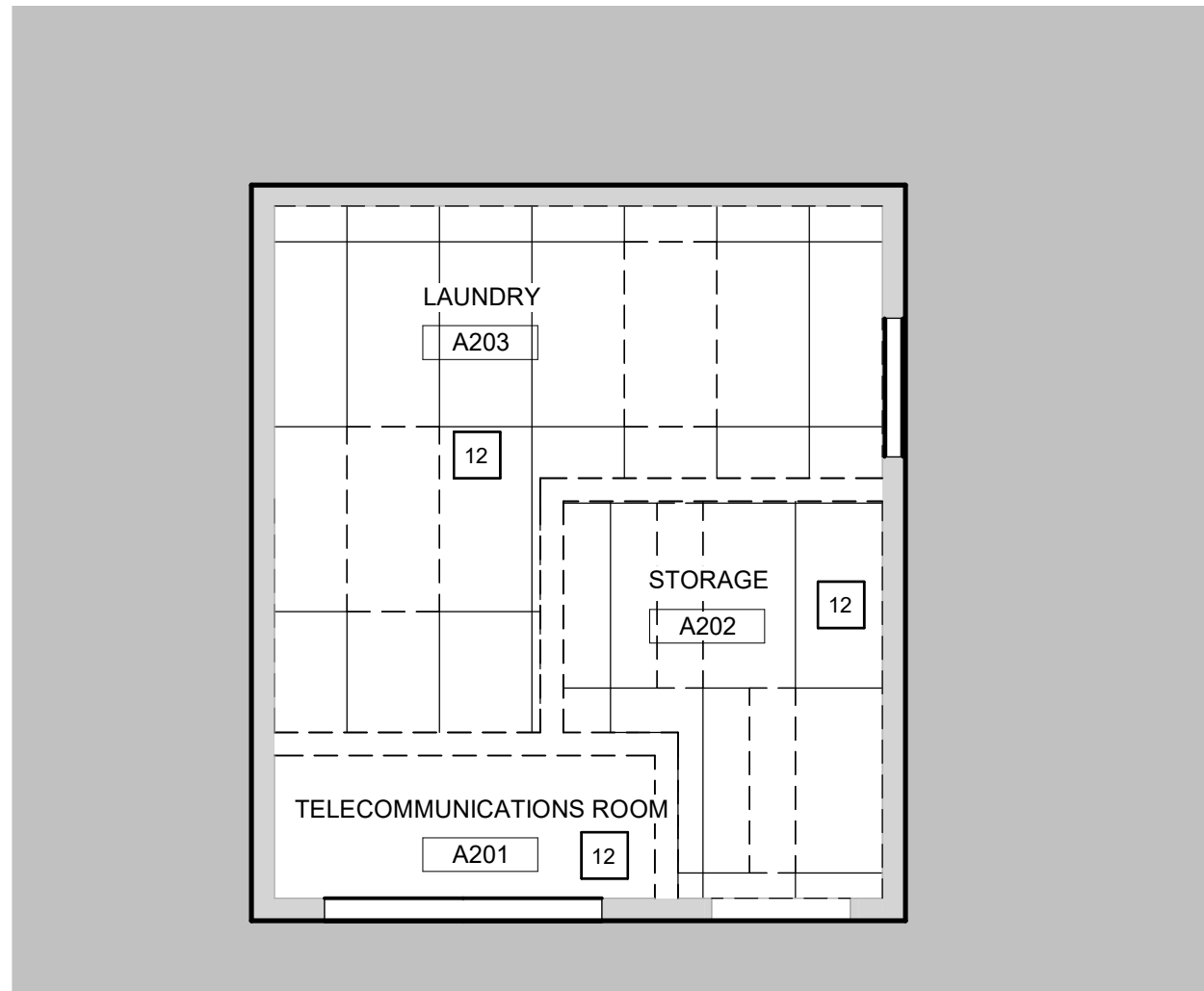
4 BUILDING 43 SECOND FLOOR RCP DEMO PLAN 1/4" = 1'-0"
