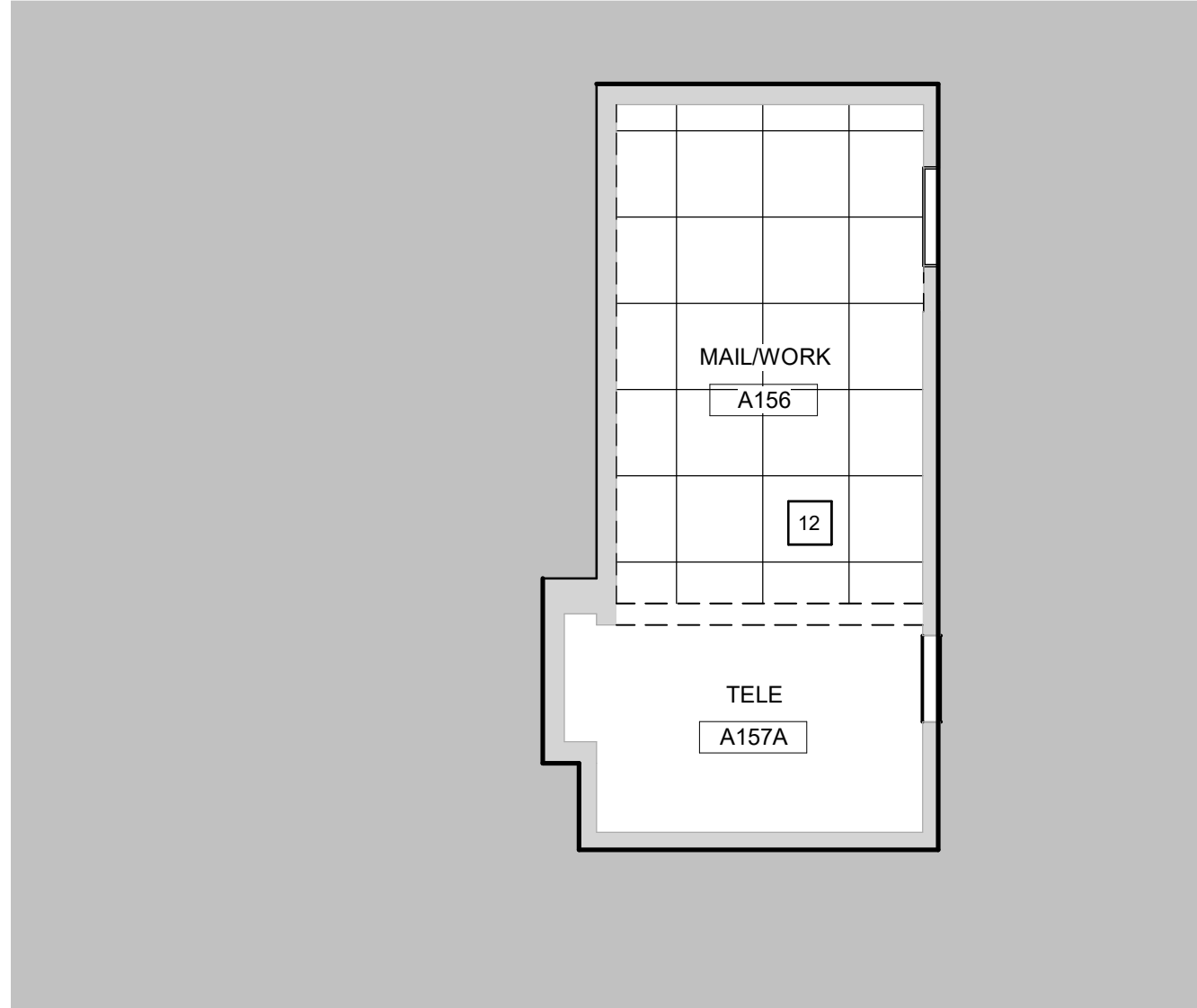
3 BUILDING 43 FIRST FLOOR RCP DEMO PLAN 1/4" = 1'-0"
