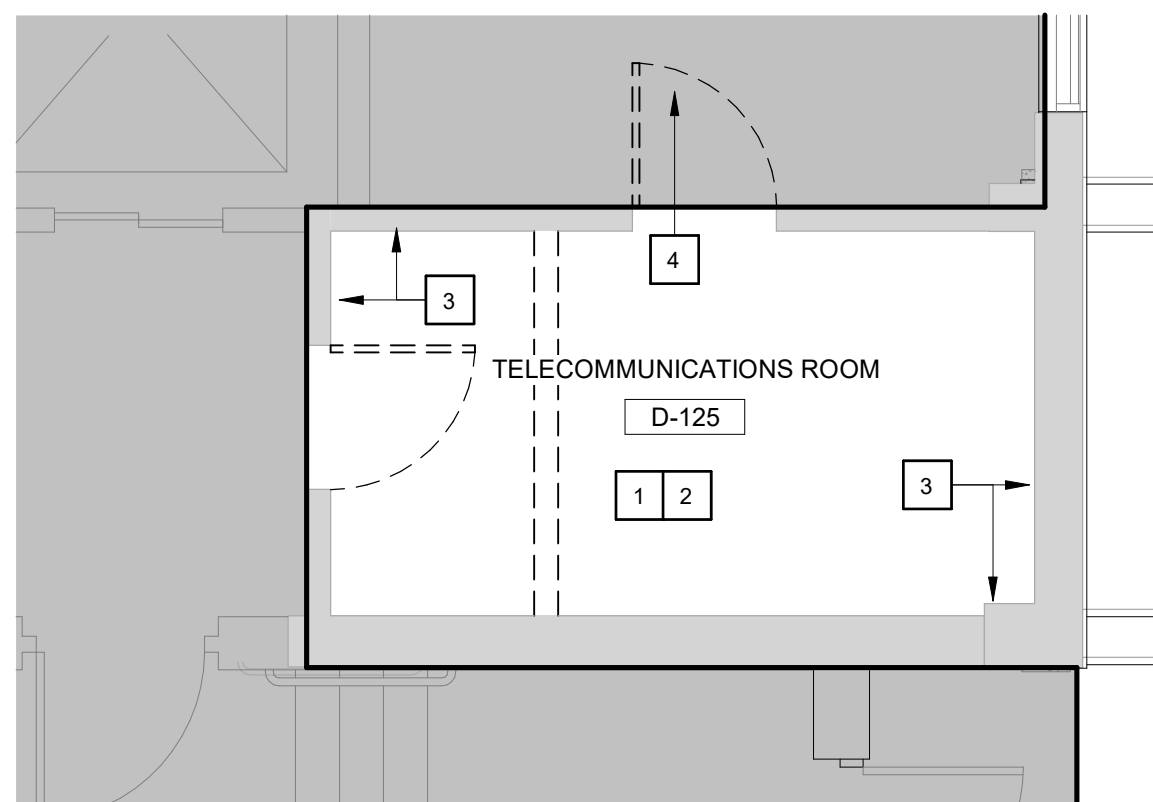
1 BUILDING 70 FIRST FLOOR ENLARGED DEMO - D-125 1/4" = 1'-0"
