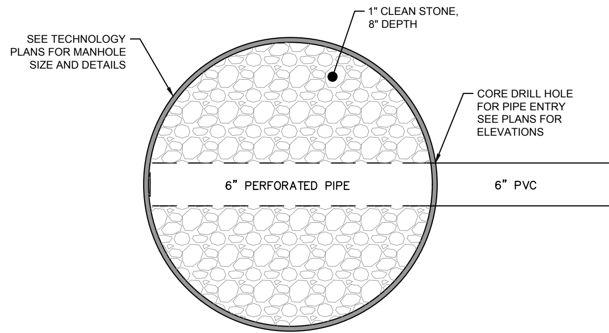
7 MANHOLE DRAINAGE DETAIL NTS
