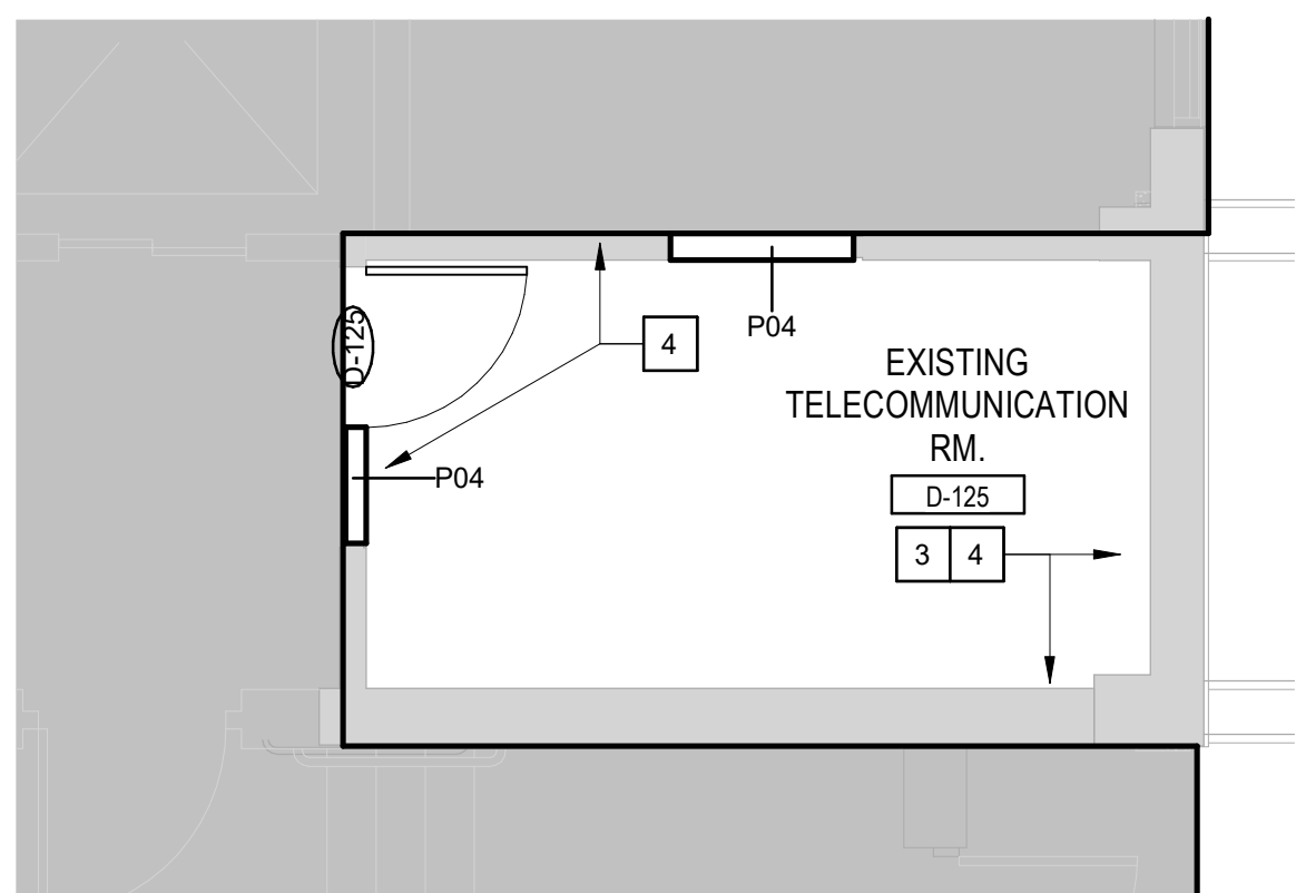
1 BUILDING 70 LEVEL 01 ENLARGED FLOOR PLAN 5 1/4" = 1'-0"
