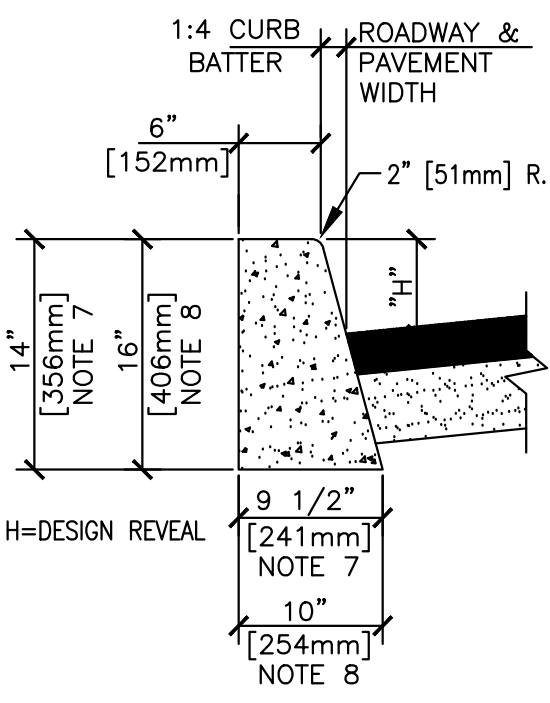
2 CONCRETE CURB AND TERMINAL SECTION NTS
