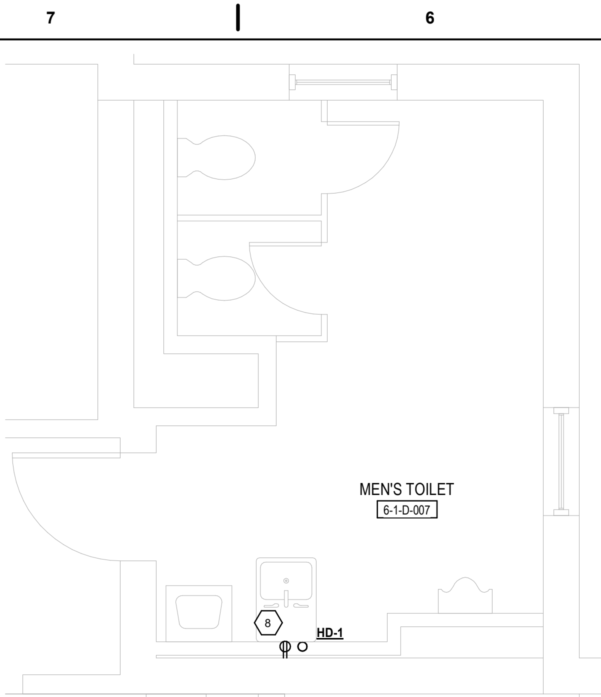
4 BLDG 6 - FIRST FLOOR - ENLARGED ELECTRICAL NEW WORK - ROOM 6-1-D-007J 3/8" = 1'-0"
