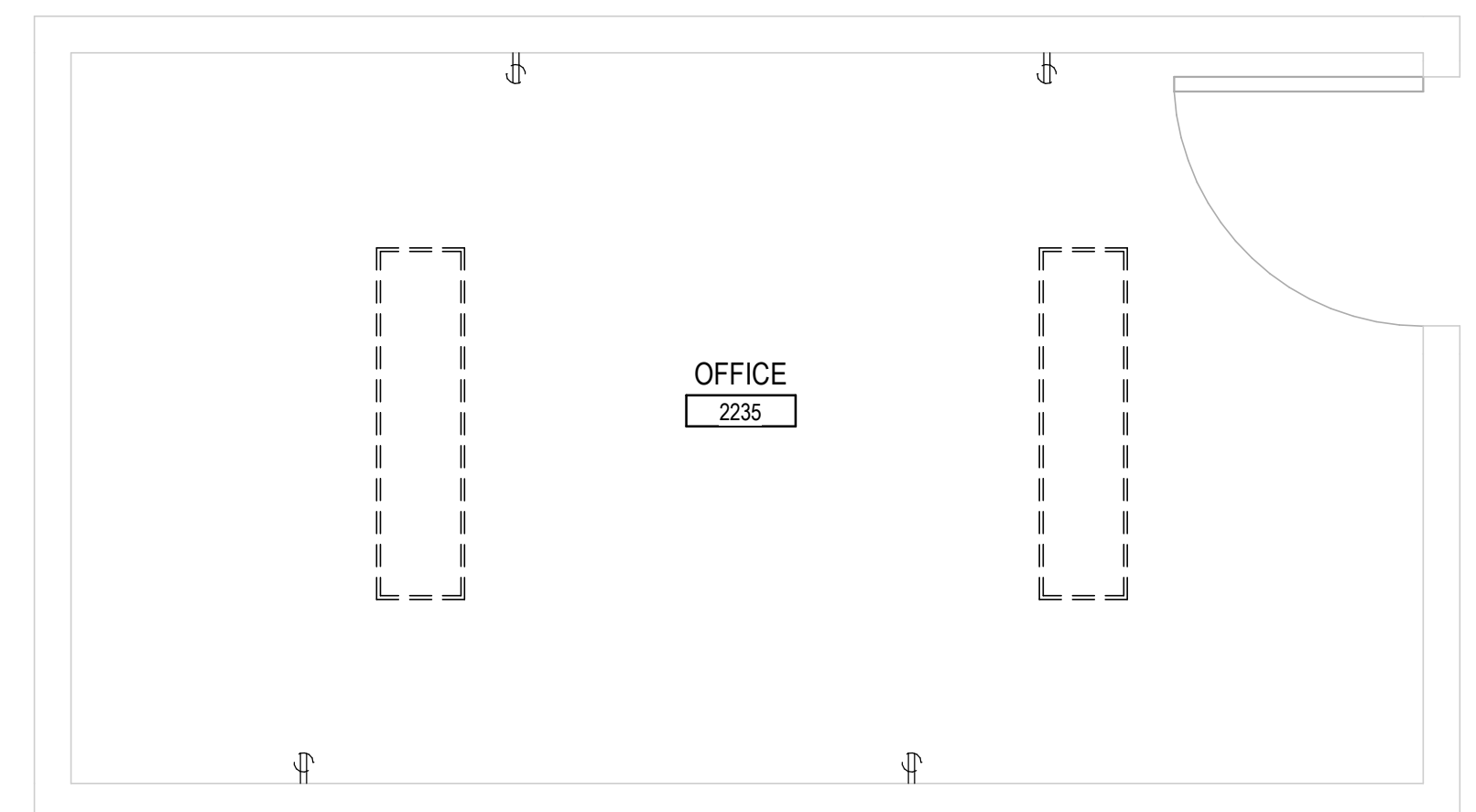
4 BLDG 111 - SECOND FLOOR - ENLARGED ELECTRICAL DEMOLITION - 2235 1/2" = 1'-0"
