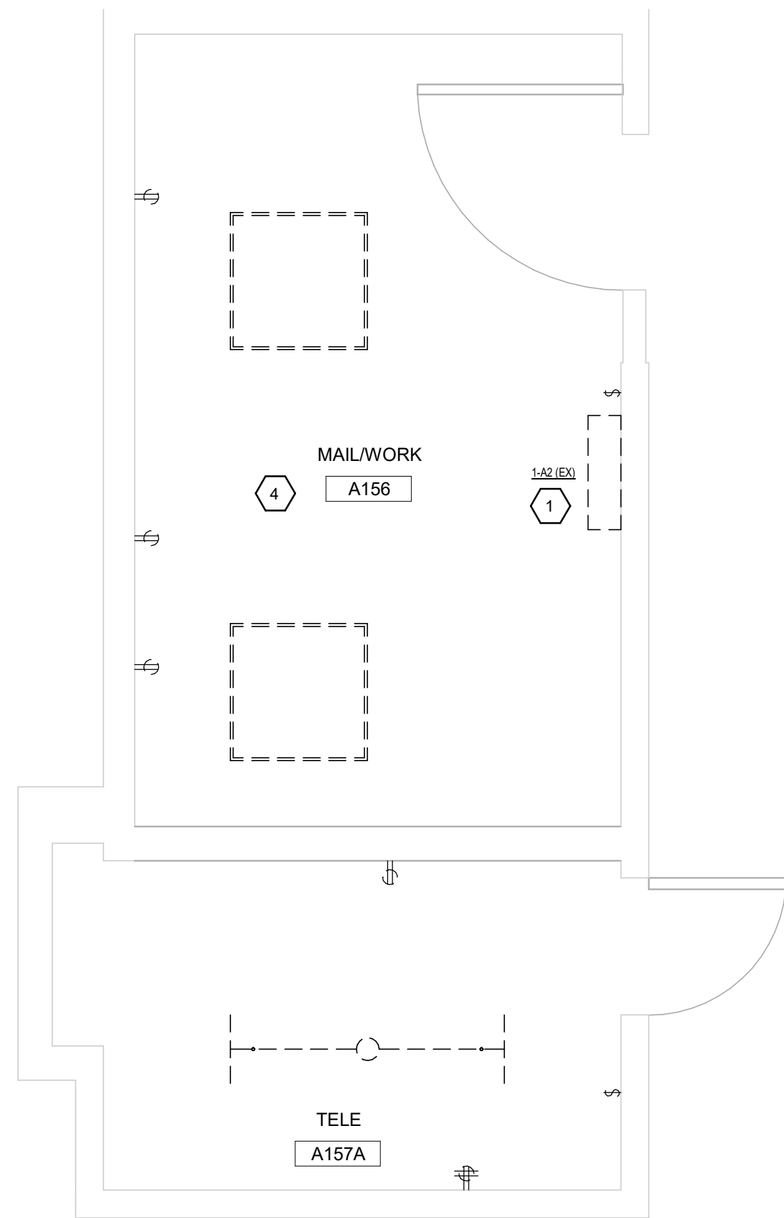
2 BLDG 43 - FIRST FLOOR - ENLARGED ELECTRICAL DEMOLITION - ROOM A156,A157A 1/2" = 1'-0"
