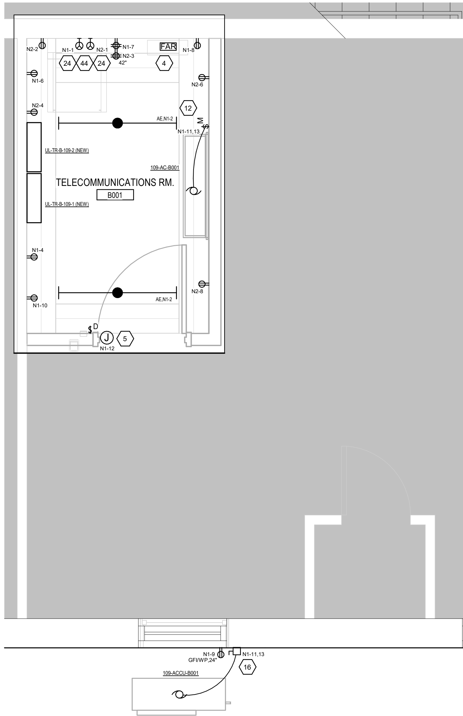
2 BLDG 109 - BASEMENT - ENLARGED ELECTRICAL NEW WORK - ROOM B001 1/2" = 1'-0"
