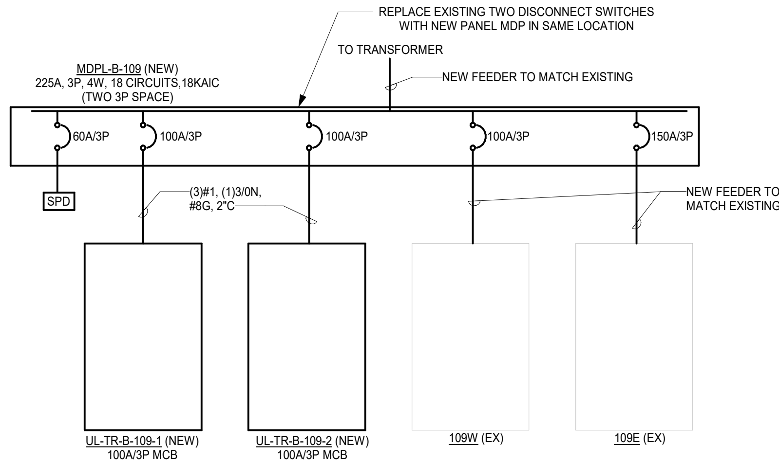
3 BLDG 109 - BASEMENT - PARTIAL ONE LINE DIAGRAM NTS
