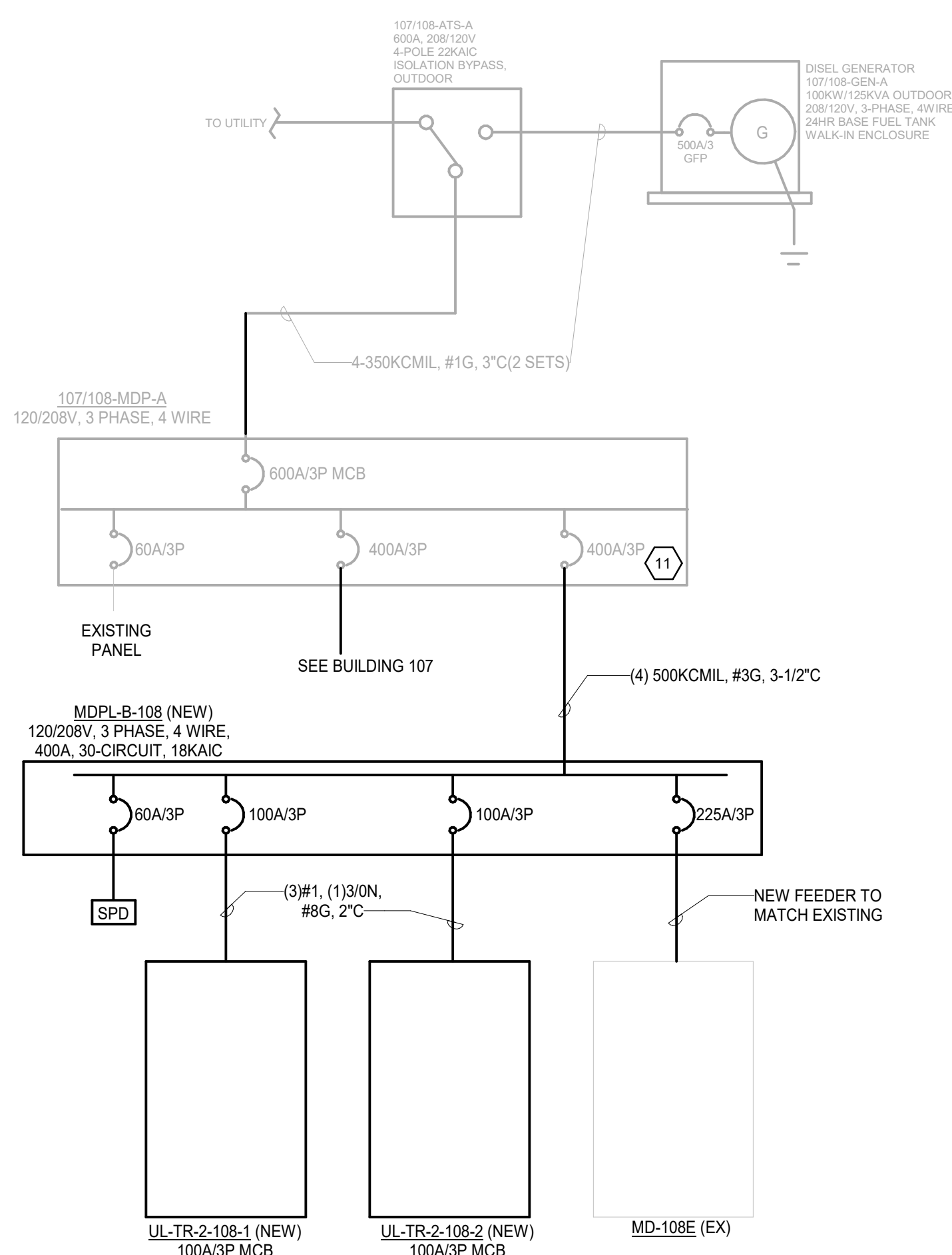
3 BLDG 108 - PARTIAL ONE LINE DIAGRAM NTS
