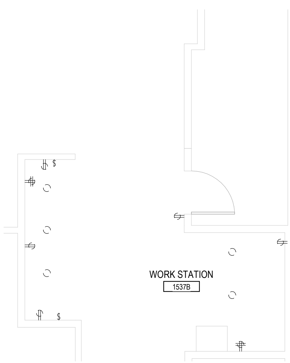
④ BLDG 111 - FIRST FLOOR - ENLARGED ELECTRICAL DEMOLITION - ROOM 1537B 1/4" = 1'-0"
