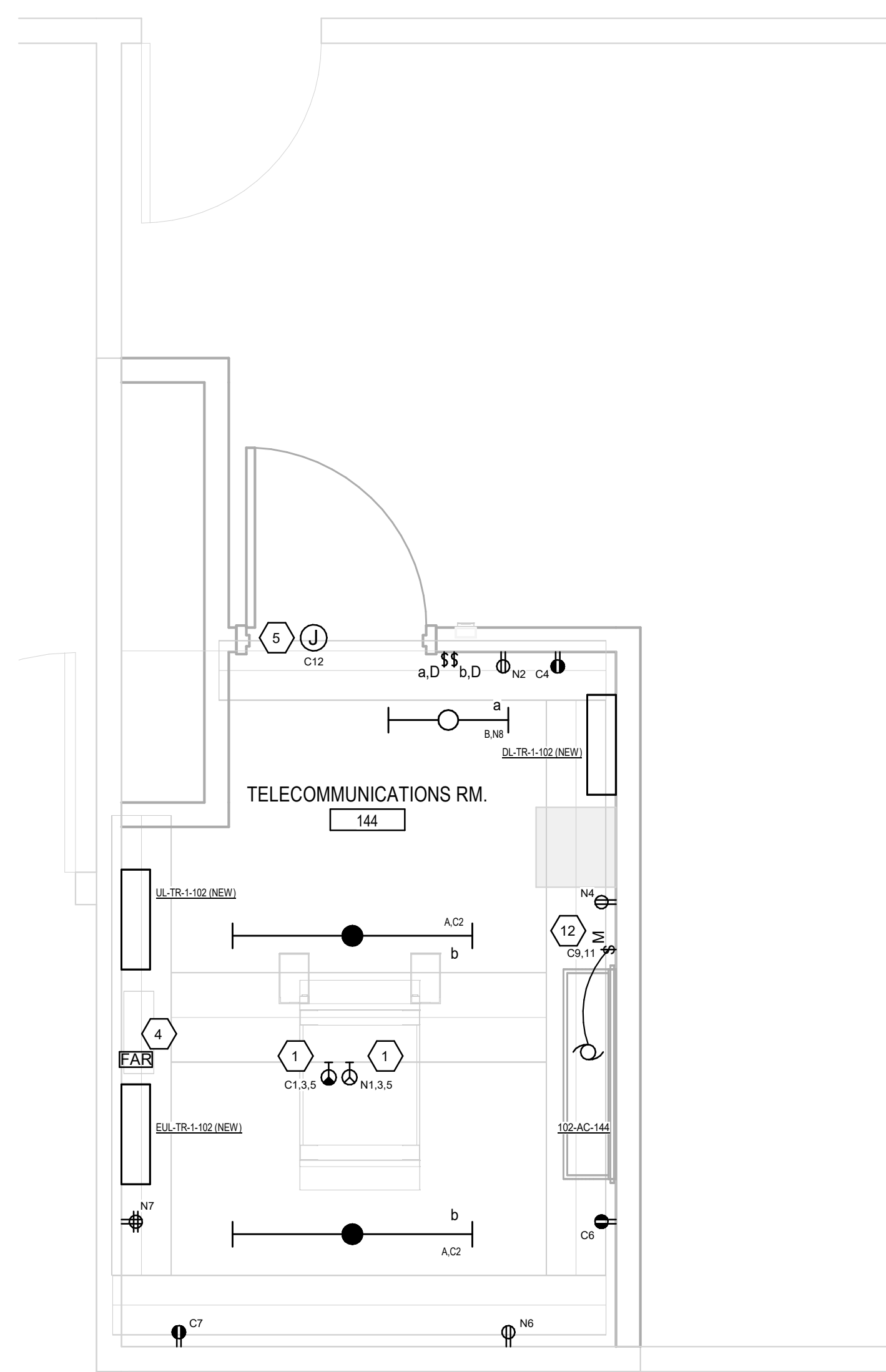
② BLDG 102 - FIRST FLOOR - ENLARGED ELECTRICAL NEW WORK - ROOM 144 1/2" = 1'-0"
