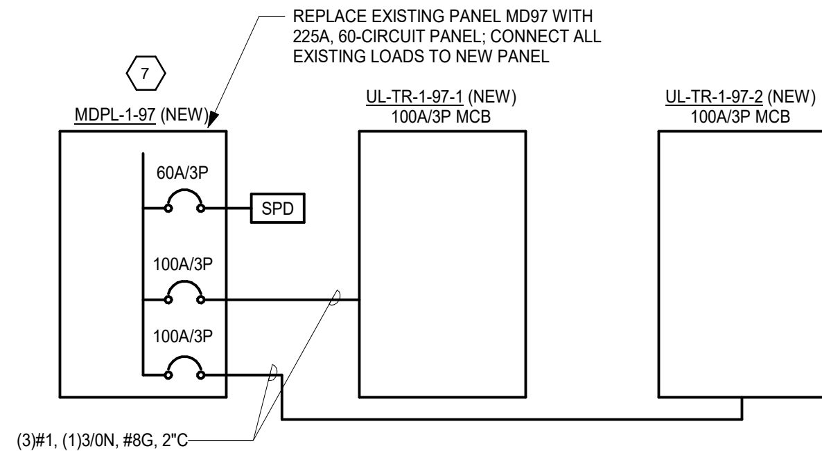
3 BLDG 97 - FIRST FLOOR - PARTIAL ONE LINE DIAGRAM NTS
