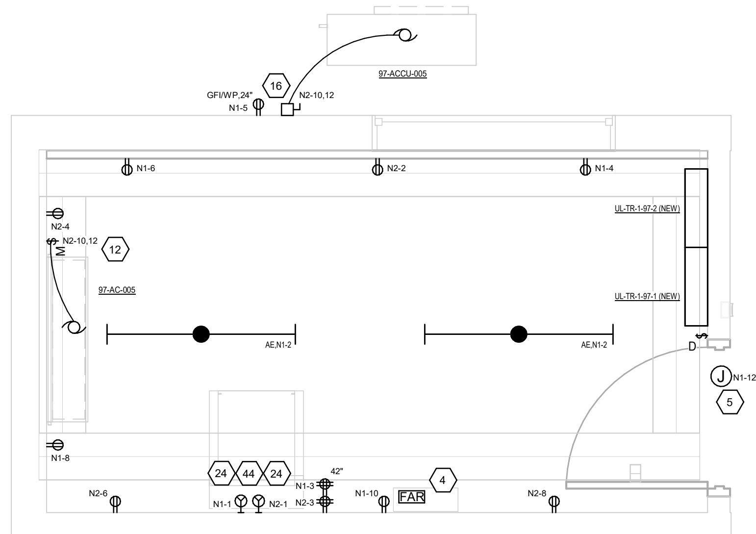
② BLDG 97 - FIRST FLOOR - ENLARGED ELECTRICAL NEW WORK - ROOM 005 1/2" = 1'-0"
