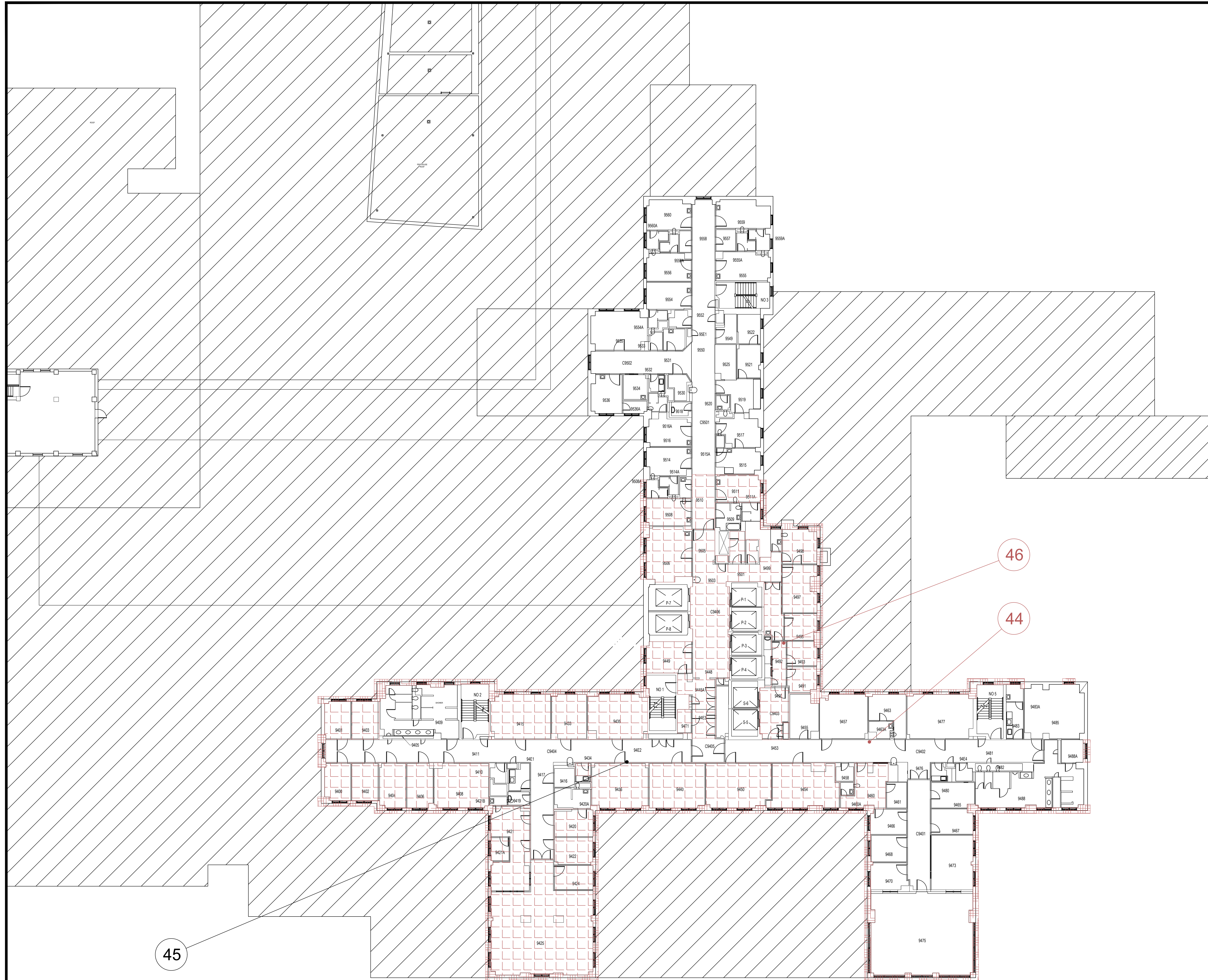
BUILDING # 1A & 1B - NINTH FLOOR PLAN
