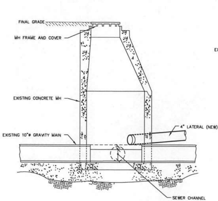
TYPICAL LATERAL TO MANHOLE CONNECTION DETAIL NO SCALE
