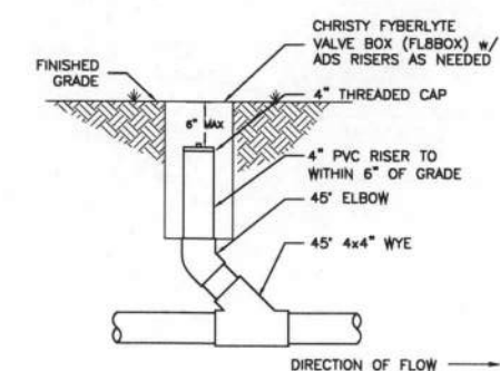
TYPICAL 4" SANITARY CLEANOUT DETAIL NO SCALE
