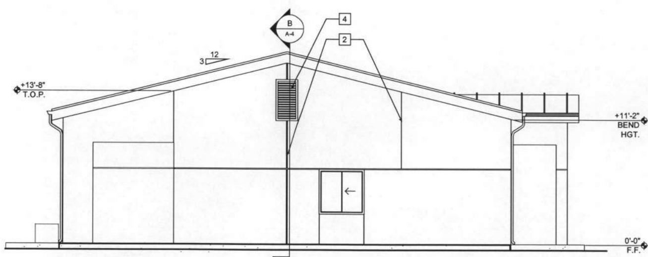
3 EAST ELEVATION AERO CLUB 1/4" = 1'-0"
