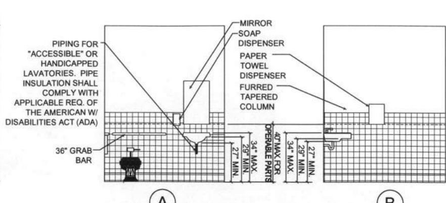
5 INT. ELEVATION - ADA RESTROOM AERO CLUB 3/8" = 1'-0"
