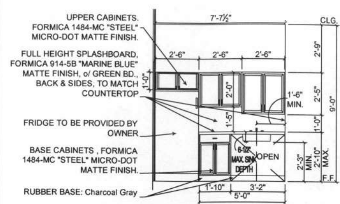
6 INT. ELEVATION - BREAK ROOM AERO CLUB 3/8" = 1'-0"
