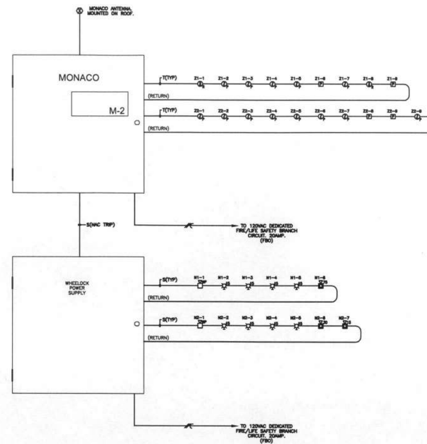
ONE-LINE RISER DIAGRAM
