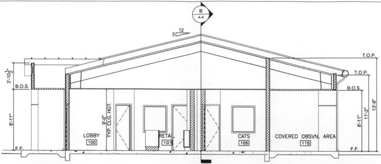
A SECTION AERO CLUB
