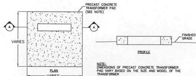
TRANSFORMER PAD DETAIL NO SCALE
