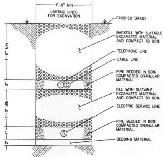
ELECTRIC SERVICE TRENCH SECTION NO SCALE
