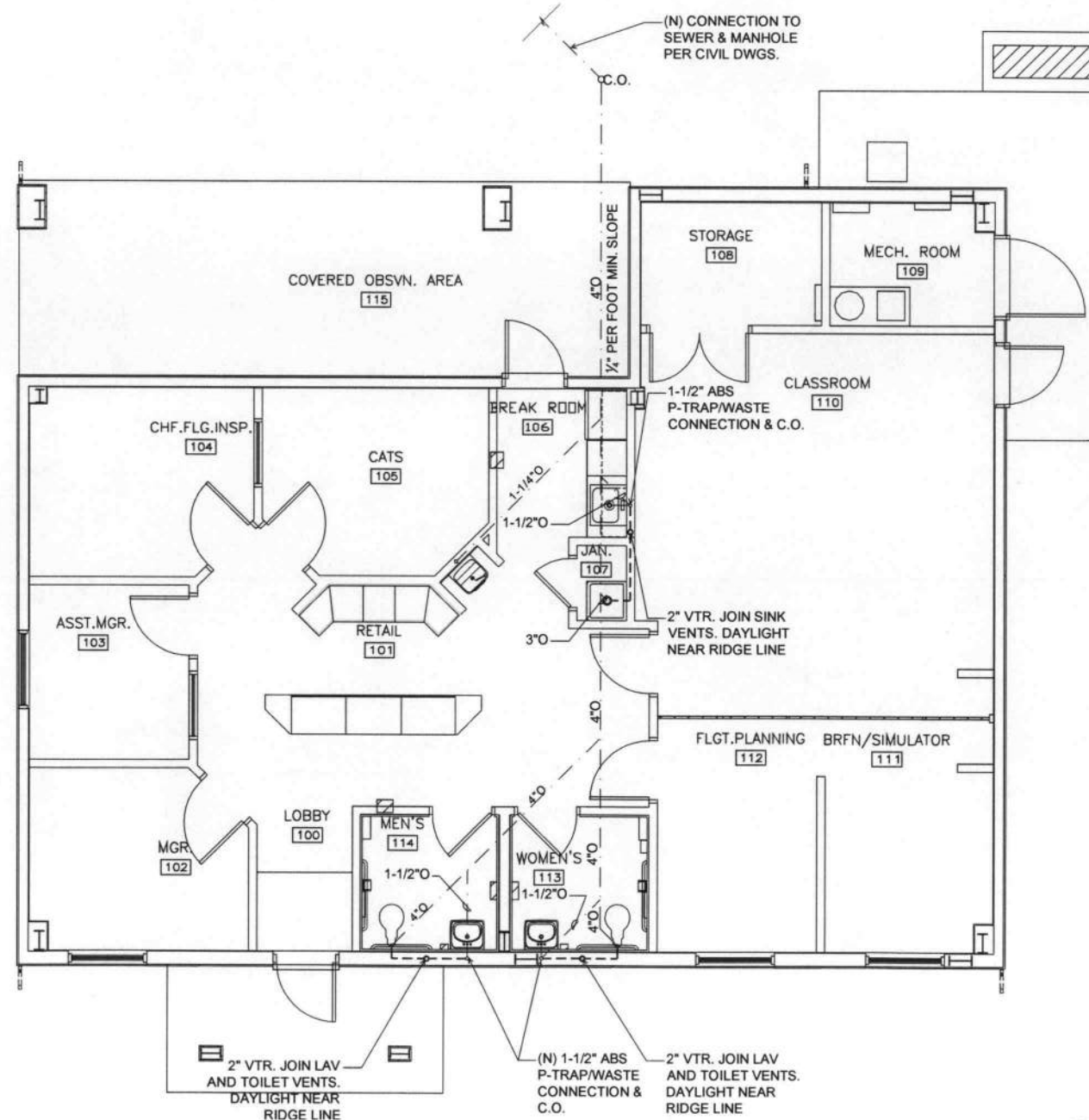
1 PLUMBING FLOOR PLAN - WASTE & VENTS AERO CLUB
