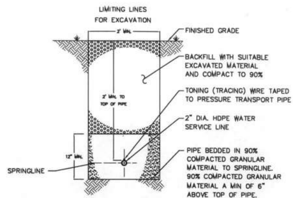
WATER SERVICE TRENCH SECTION NO SCALE
