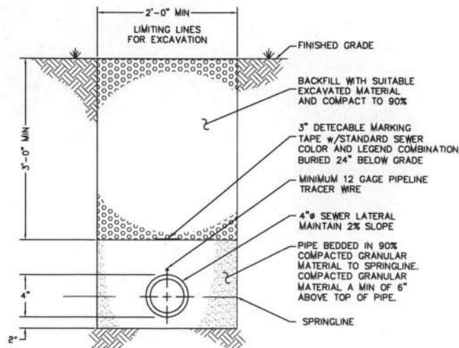
SEWER LATERAL TRENCH SECTION NO SCALE
