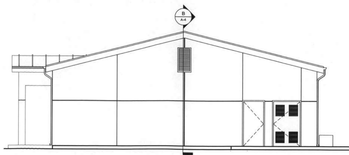
4 WEST ELEVATION AERO CLUB 1/4" = 1'-0"
