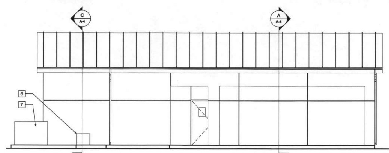
2 SOUTH ELEVATION AERO CLUB 1/4" = 1'-0"
