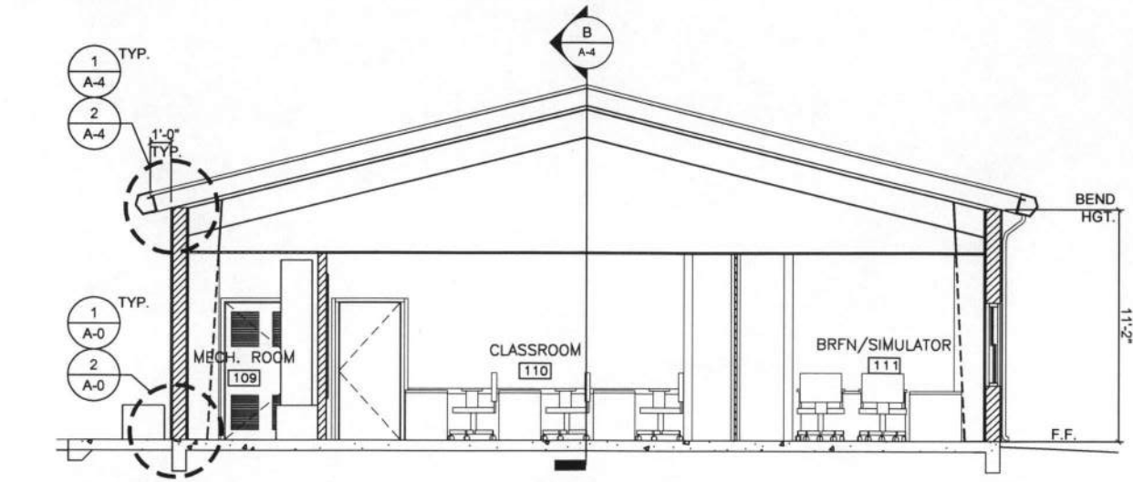
C SECTION AERO CLUB
