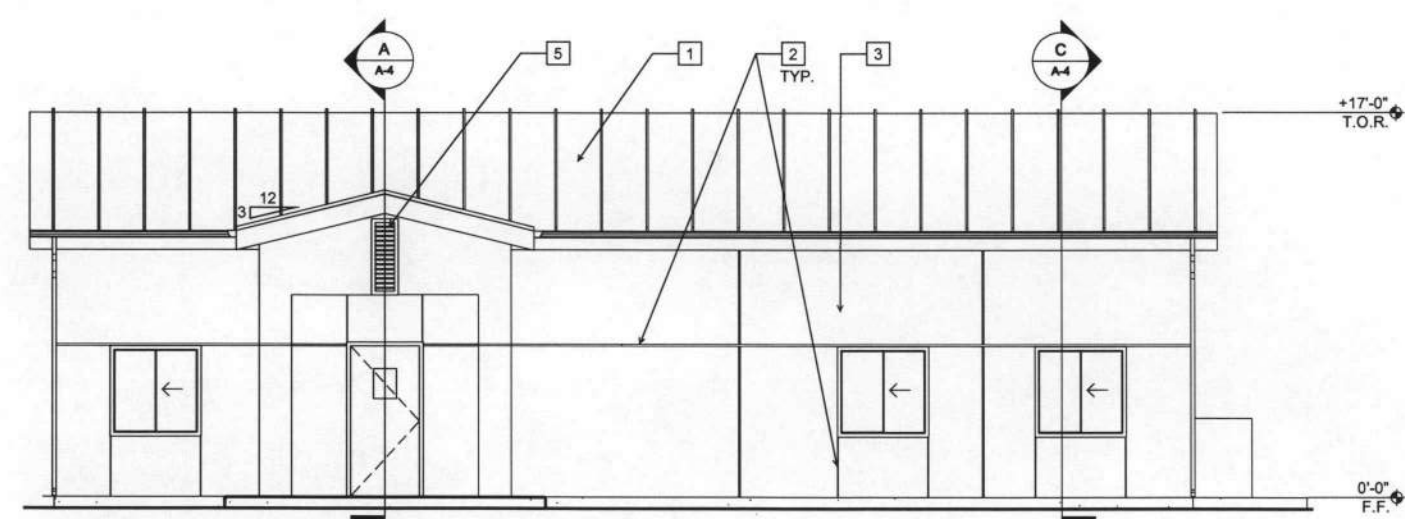
1 NORTH ELEVATION AERO CLUB 1/4" = 1'-0"
