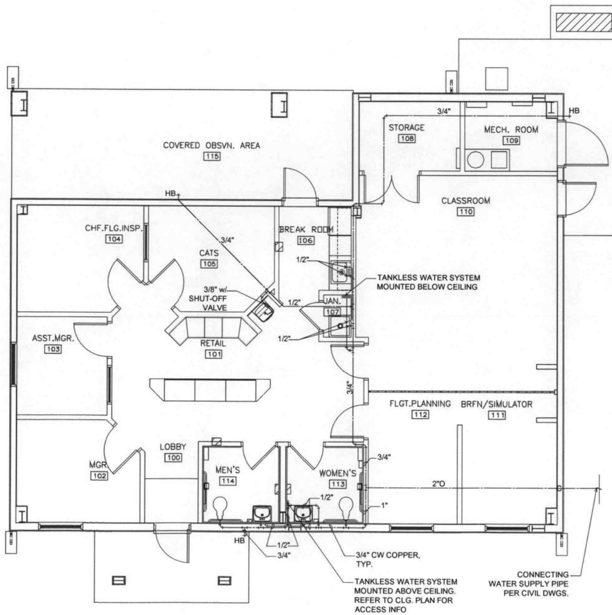
2 PLUMBING FLOOR PLAN - SUPPLY AERO CLUB
