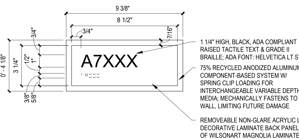
IN-03.01 ADA ROOM NUMBER NOT TO SCALE
