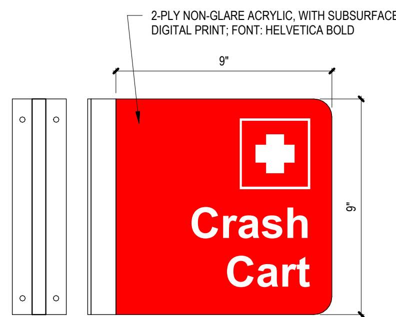
IN-01.37 CRASH CART NOT TO SCALE
