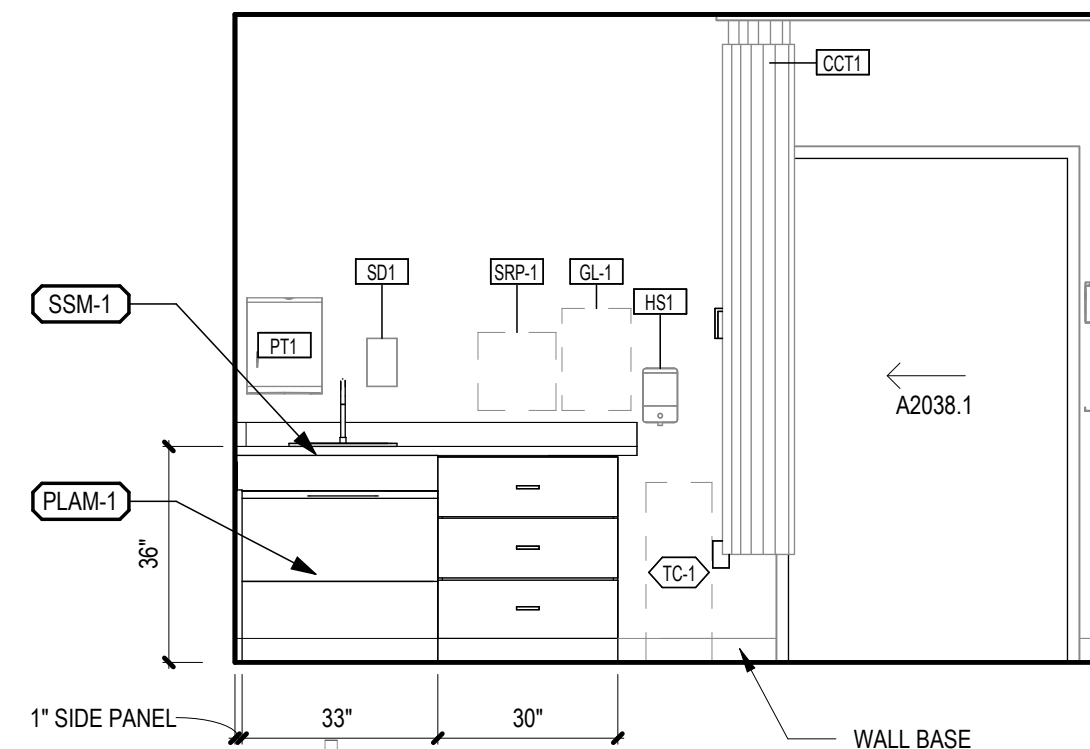
14 EXAM A2038 - NORTH A-102.1A 3/8" = 1'-0"
