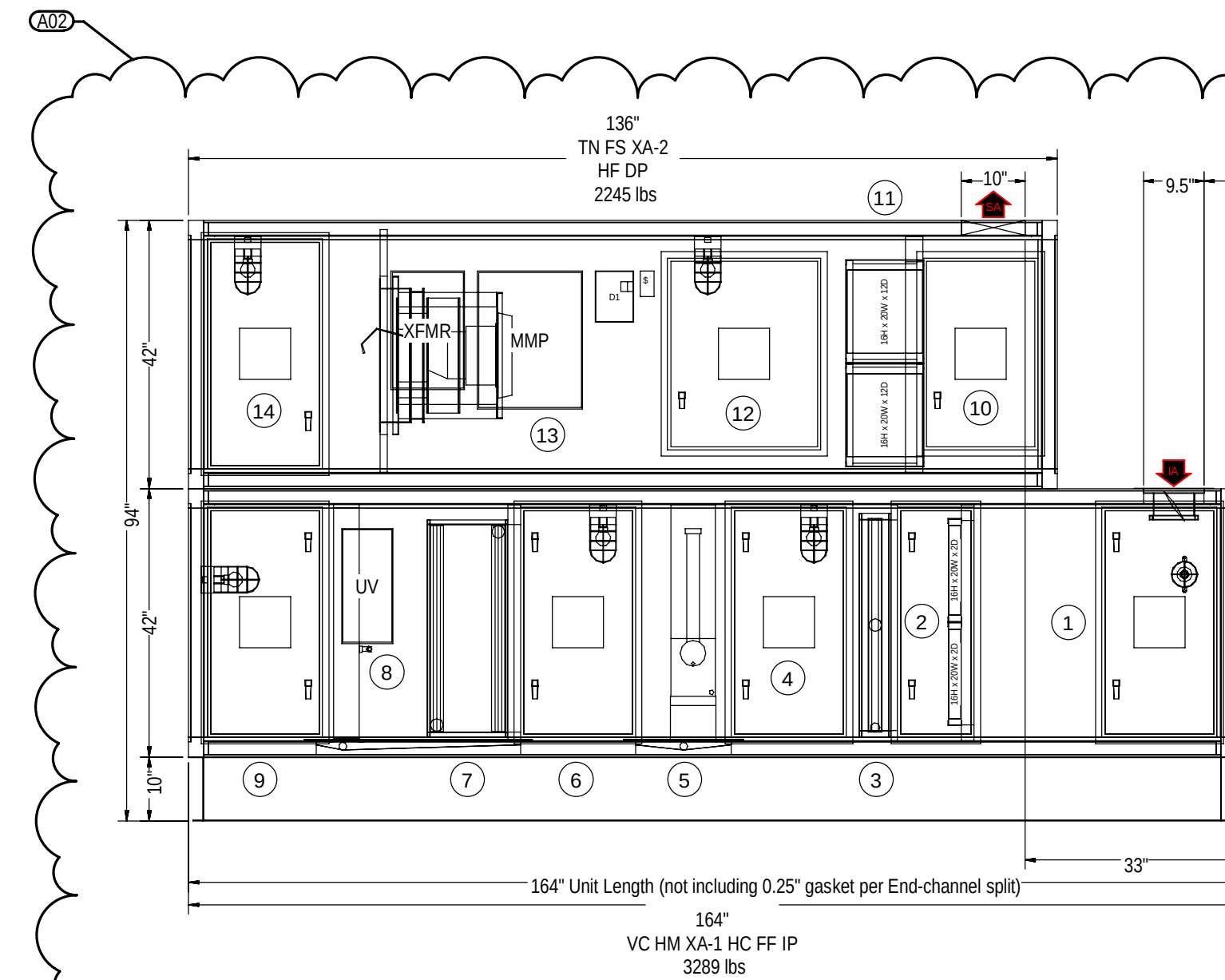
ELEVATION VIEW 1
