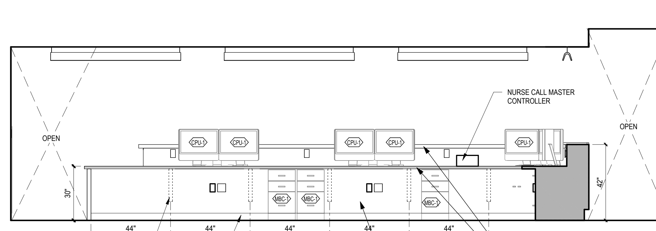
1 NURSE STATION INTERIOR A2075 - NORTH A-102.1C 3/8" = 1'-0"
