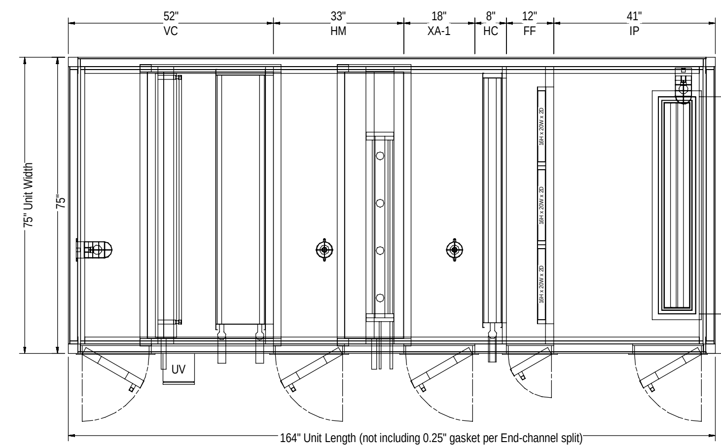
PLAN VIEW - TIER 1 1
