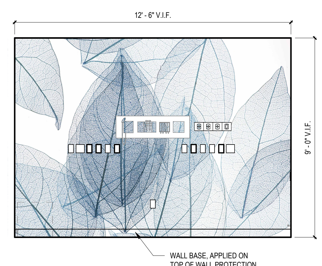
5 INFUSION ROOM - CUSTOM WALL PROTECTION A-405 3/8" = 1'-0"
