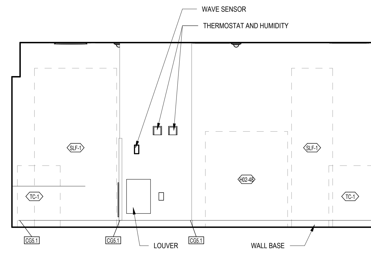
13 STERILE HAZARDOUS DRUG BUFFER ROOM A2057 - WEST A-132 3/8" = 1'-0"
