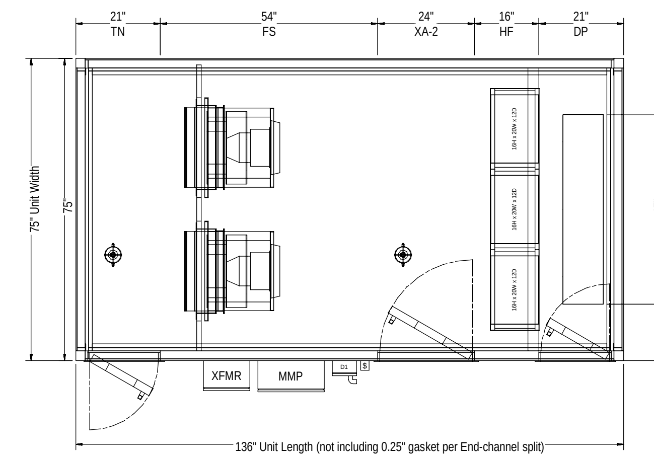
PLAN VIEW - TIER 2 1
