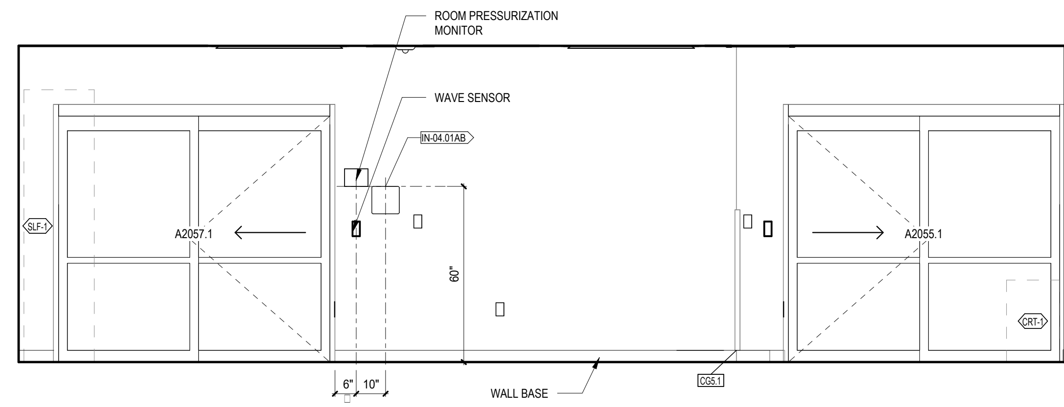
10 ANTE ROOM A2055 - NORTH A-132 3/8" = 1'-0"
