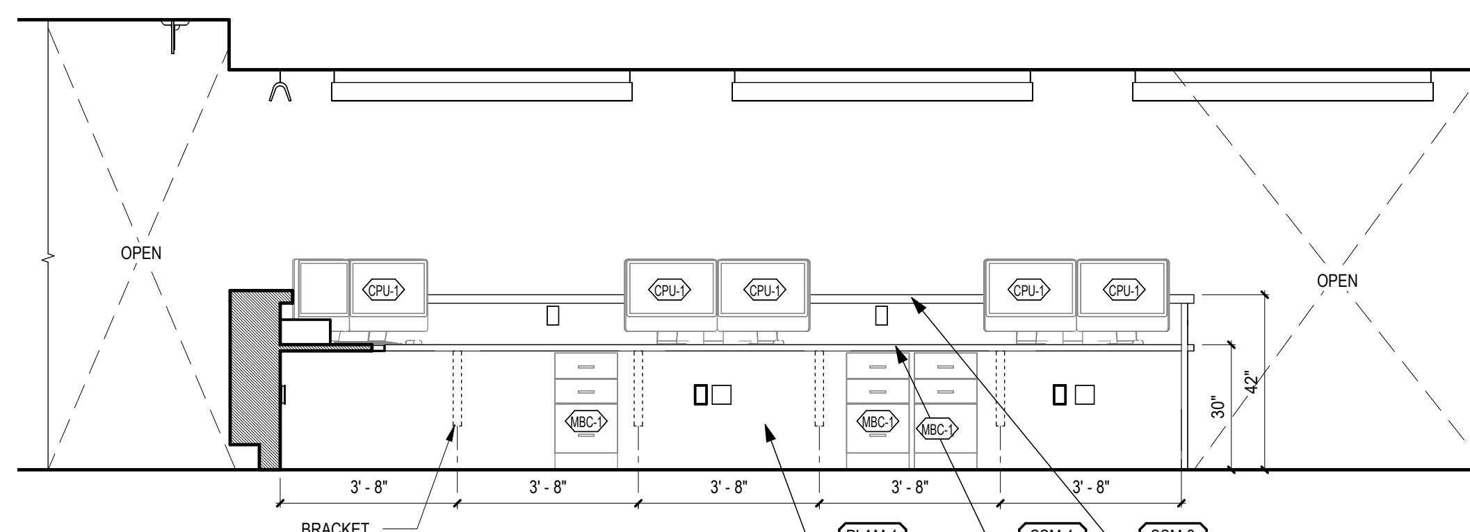
7 NURSE STATION INTERIOR A2075 - EAST A-102.1C 3/8" = 1'-0"
