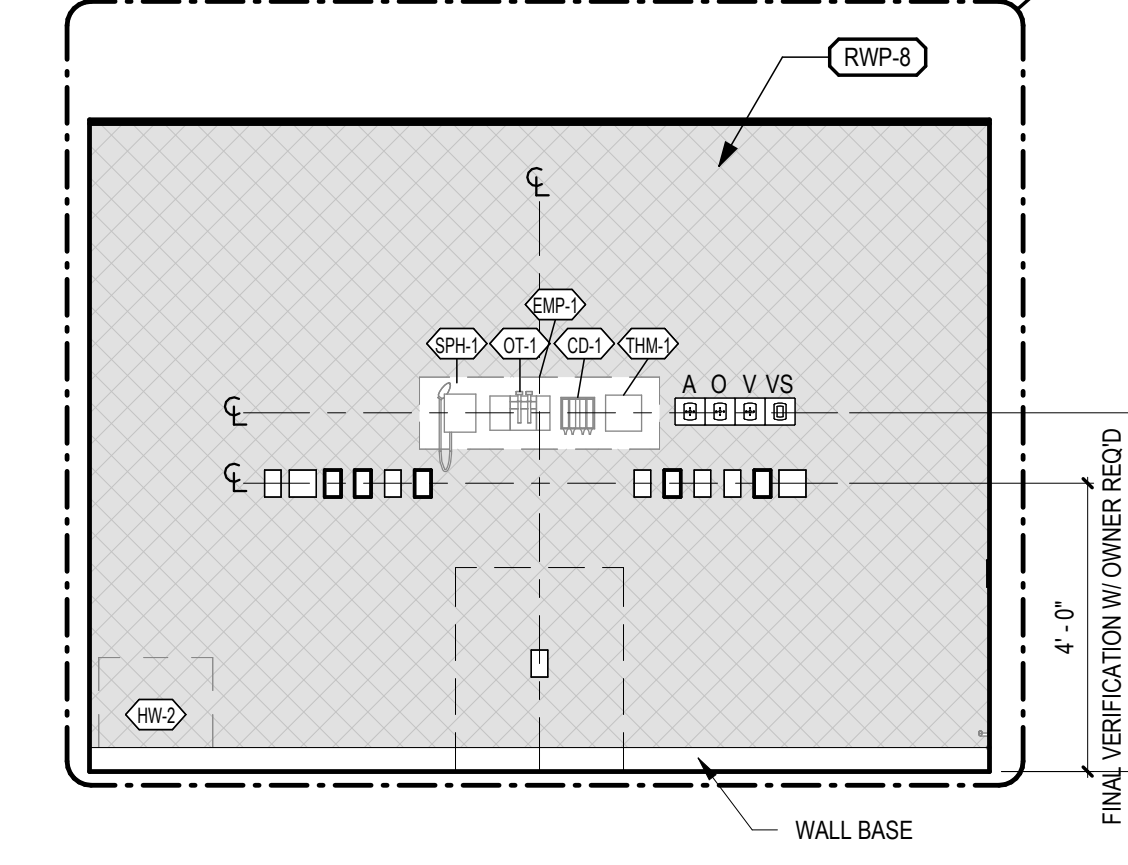
4 INFUSION ROOM A2064 - WEST A-102.1A 3/8" = 1'-0"
