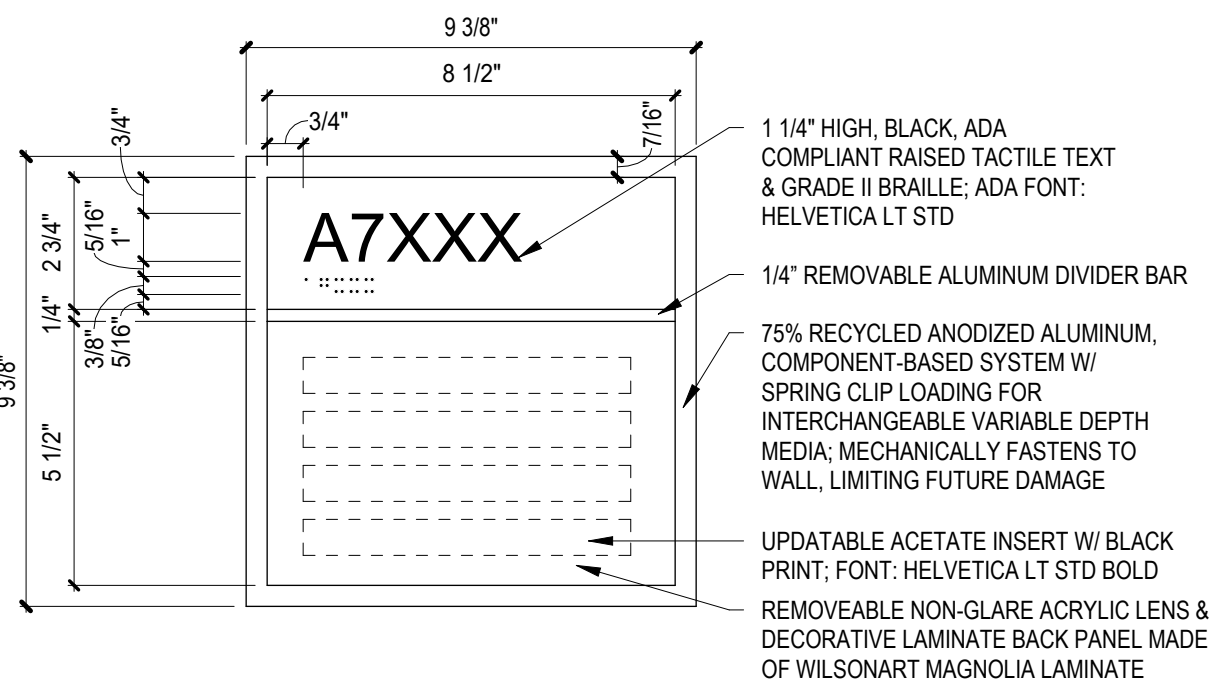
IN-04.01AB ADA ROOM IDENTIFICATION NOT TO SCALE
