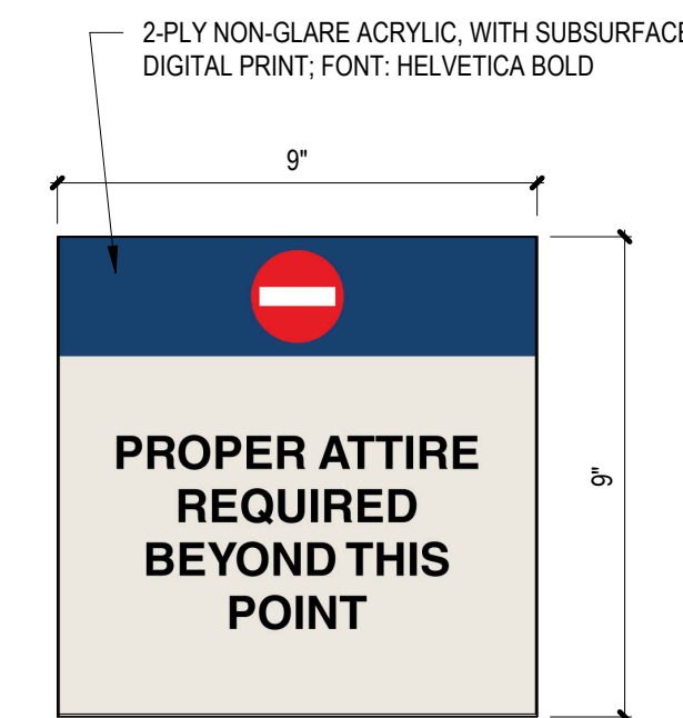
IN-01.34 PROPER ATTIRE NOT TO SCALE
