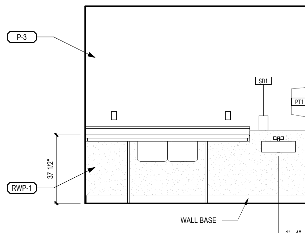
14 SOILED UTILITY A2052 - WEST A-102.1C 3/8" = 1'-0"
