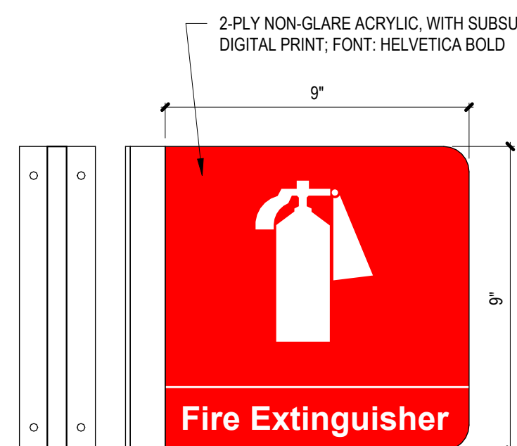
IN-01.31 FIRE EXTINGUISHER NOT TO SCALE
