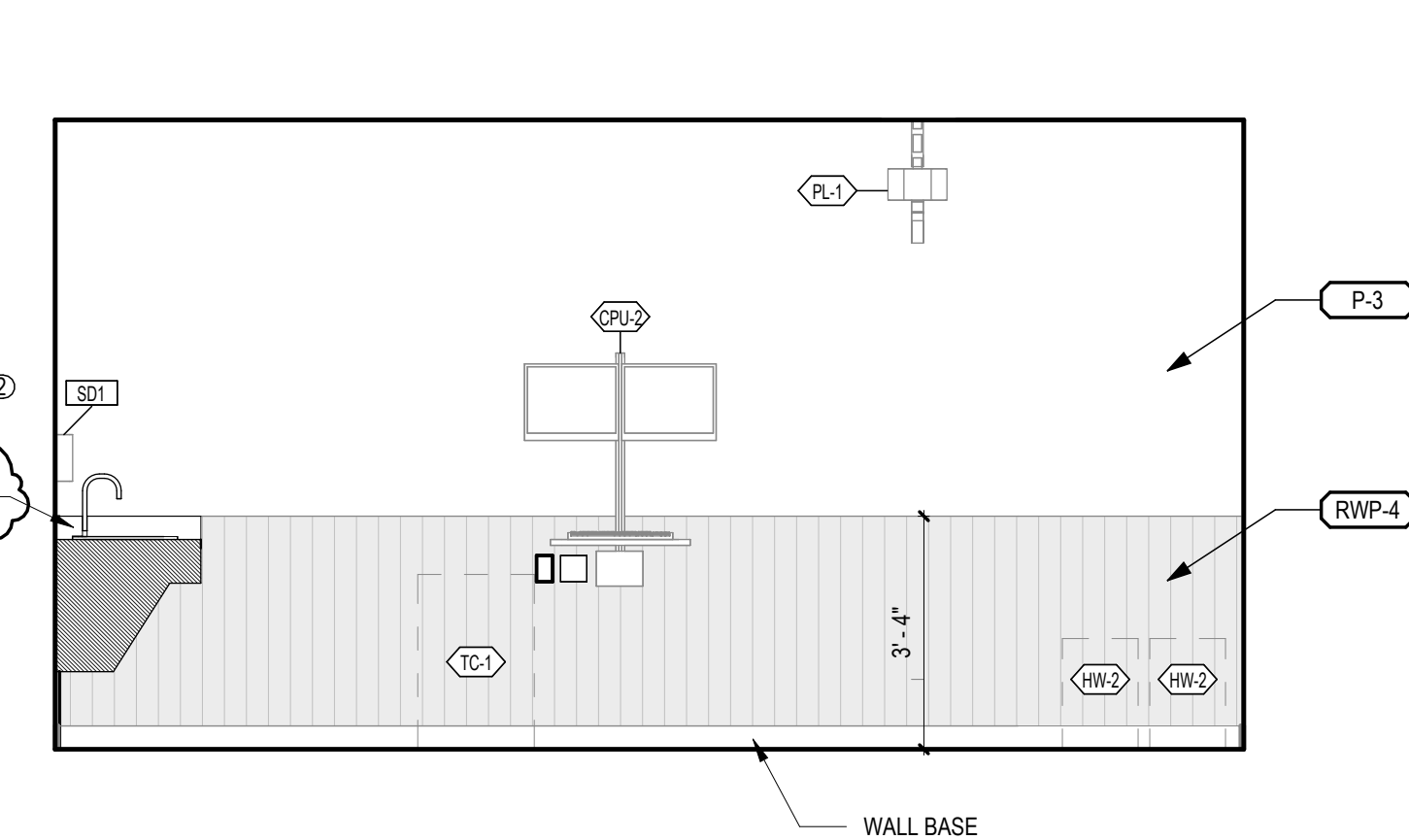
3 INFUSION ROOM A2064 - SOUTH A-102.1A 3/8" = 1'-0"
