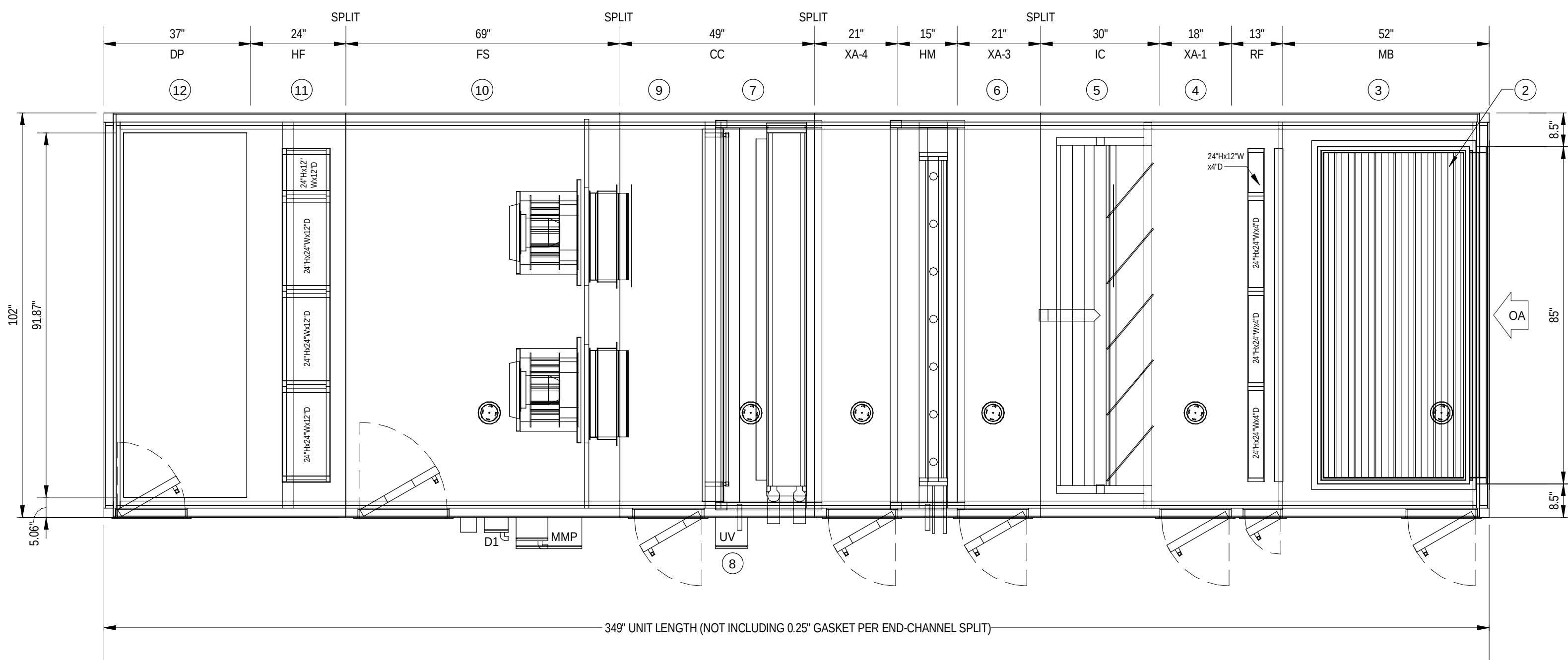
PLAN VIEW 1
