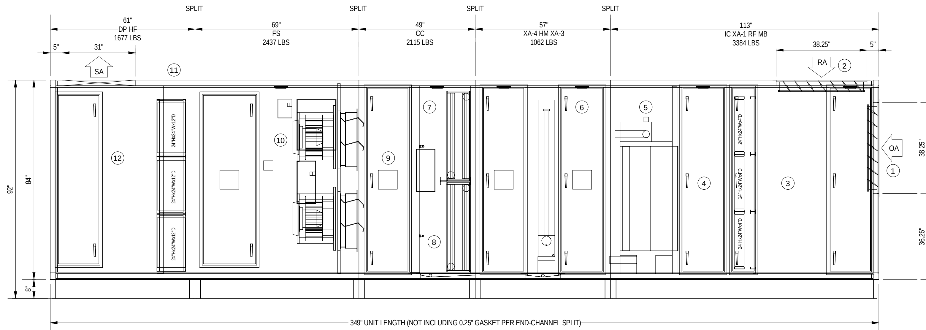
ELEVATION VIEW 1
