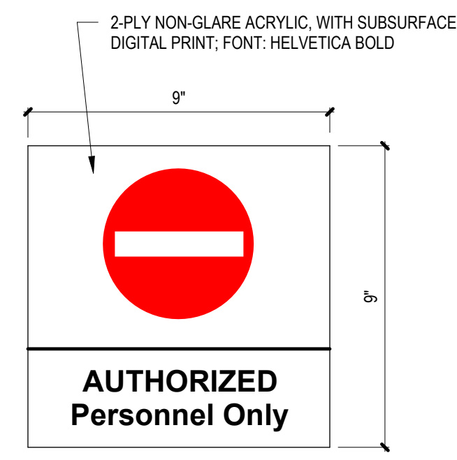
IN-08.02A AUTHORIZED PERSONNEL NOT TO SCALE
