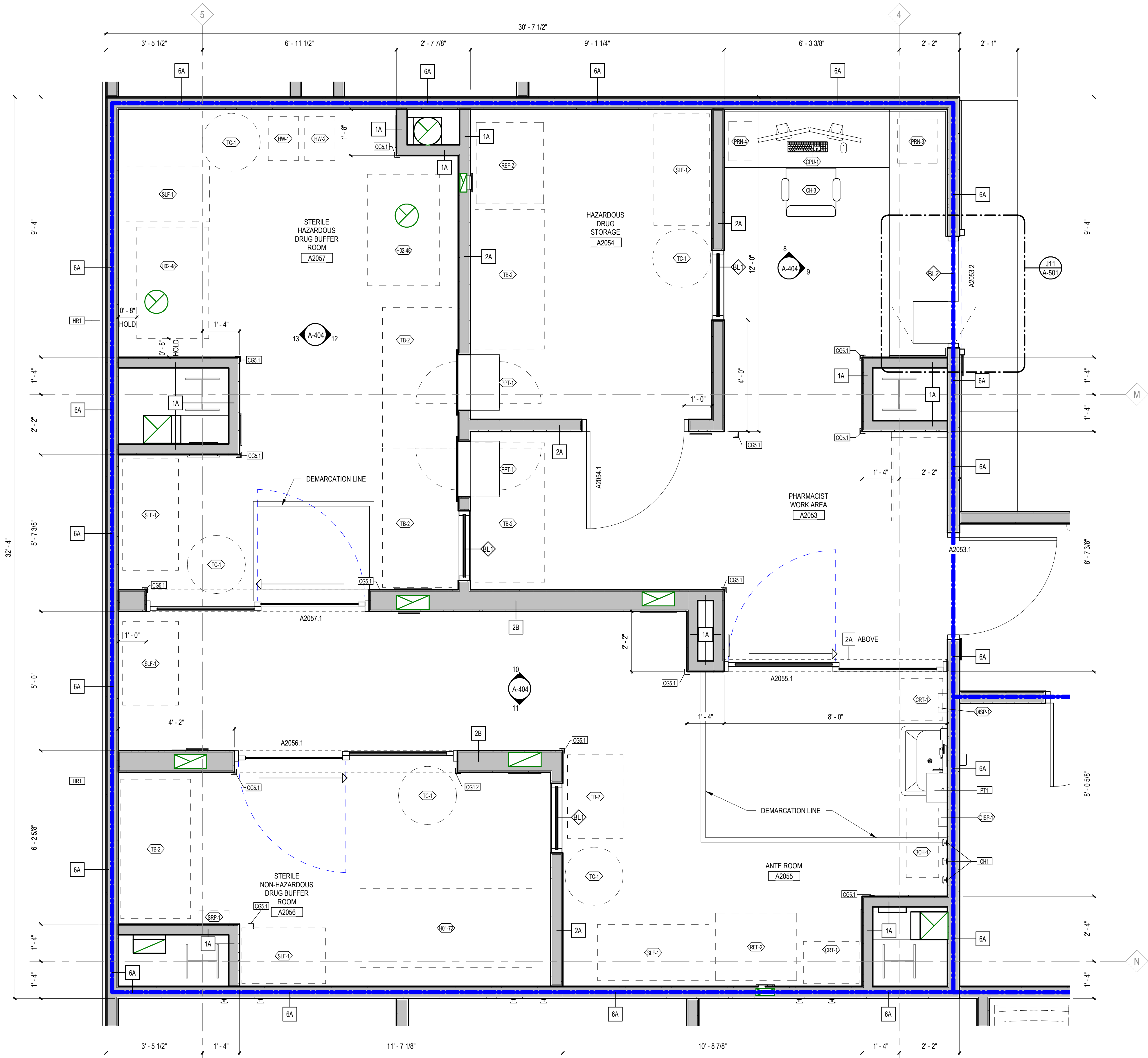
1 ENLARGED PLAN - SATELLITE PHARMACY 1/2" = 1'-0"
