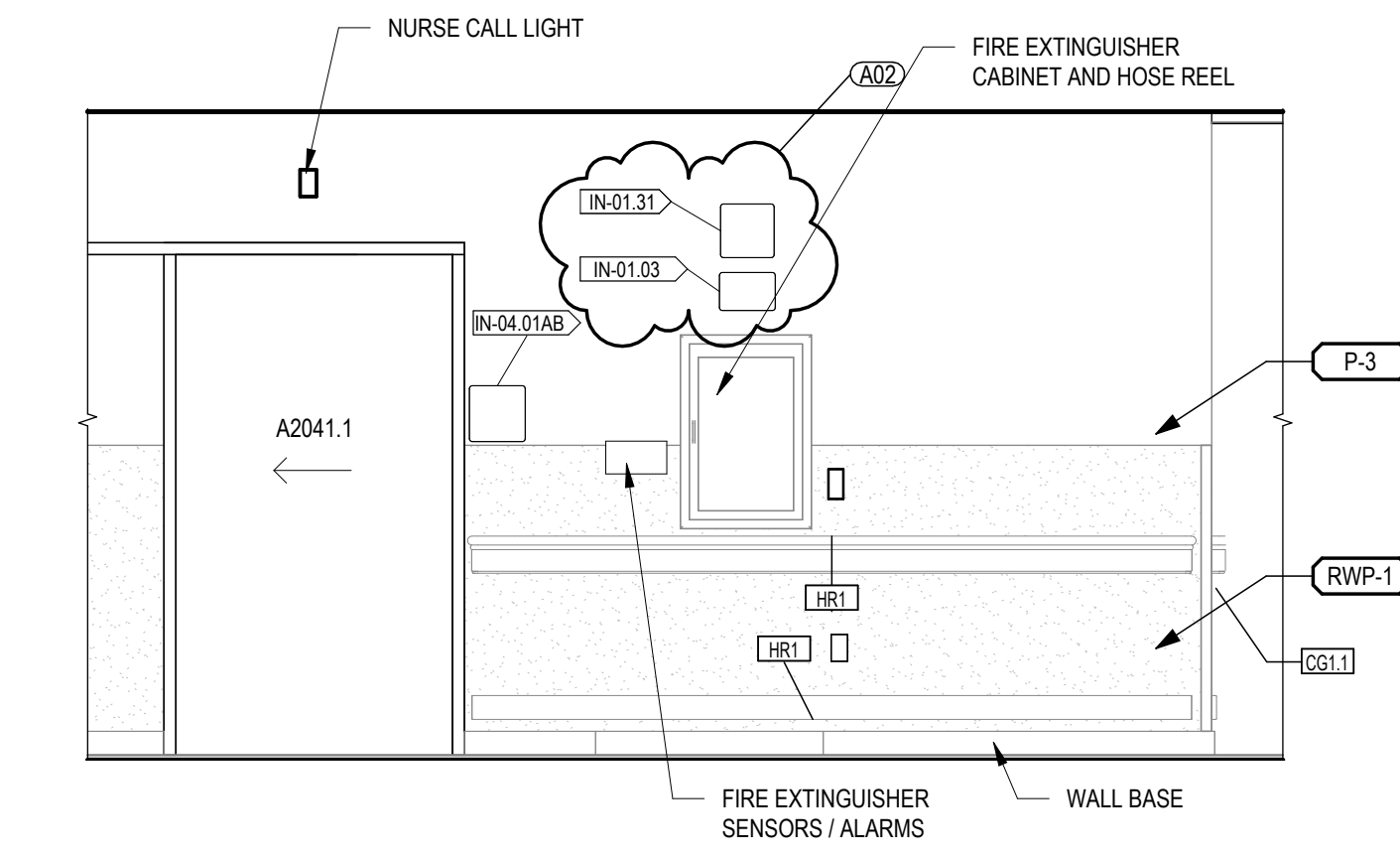
18 CORRIDOR CA213 - NORTH 2 A-102.1C 3/8" = 1'-0"
