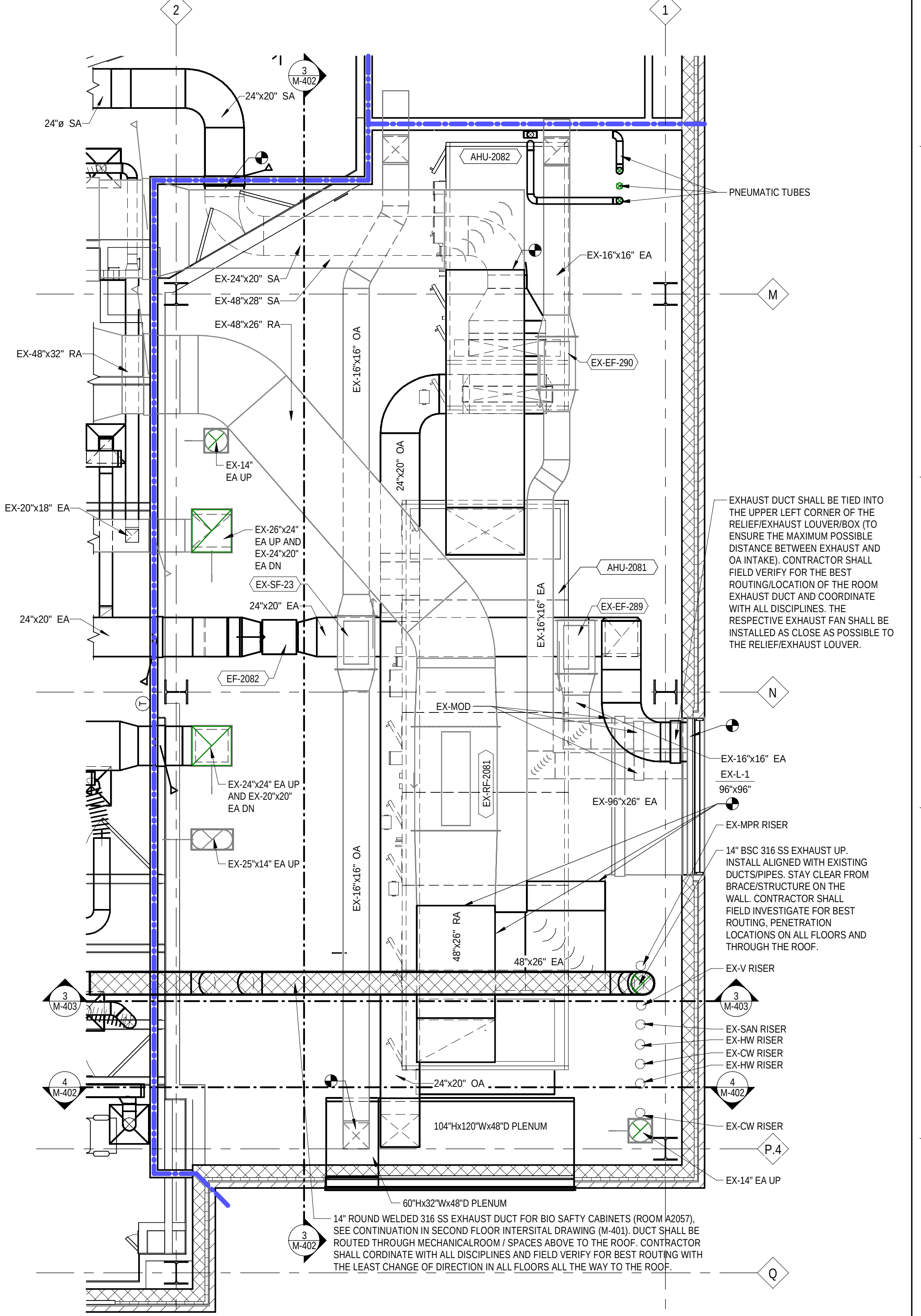
ENLARGED MECHANICAL ROOM A2032 HVAC PLAN MH102/ 1/4" = 1'-0"
