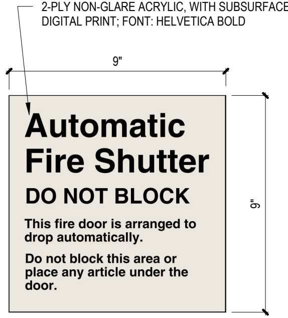
IN-01.09 AUTOMATIC FIRE SHUTTER NOT TO SCALE
