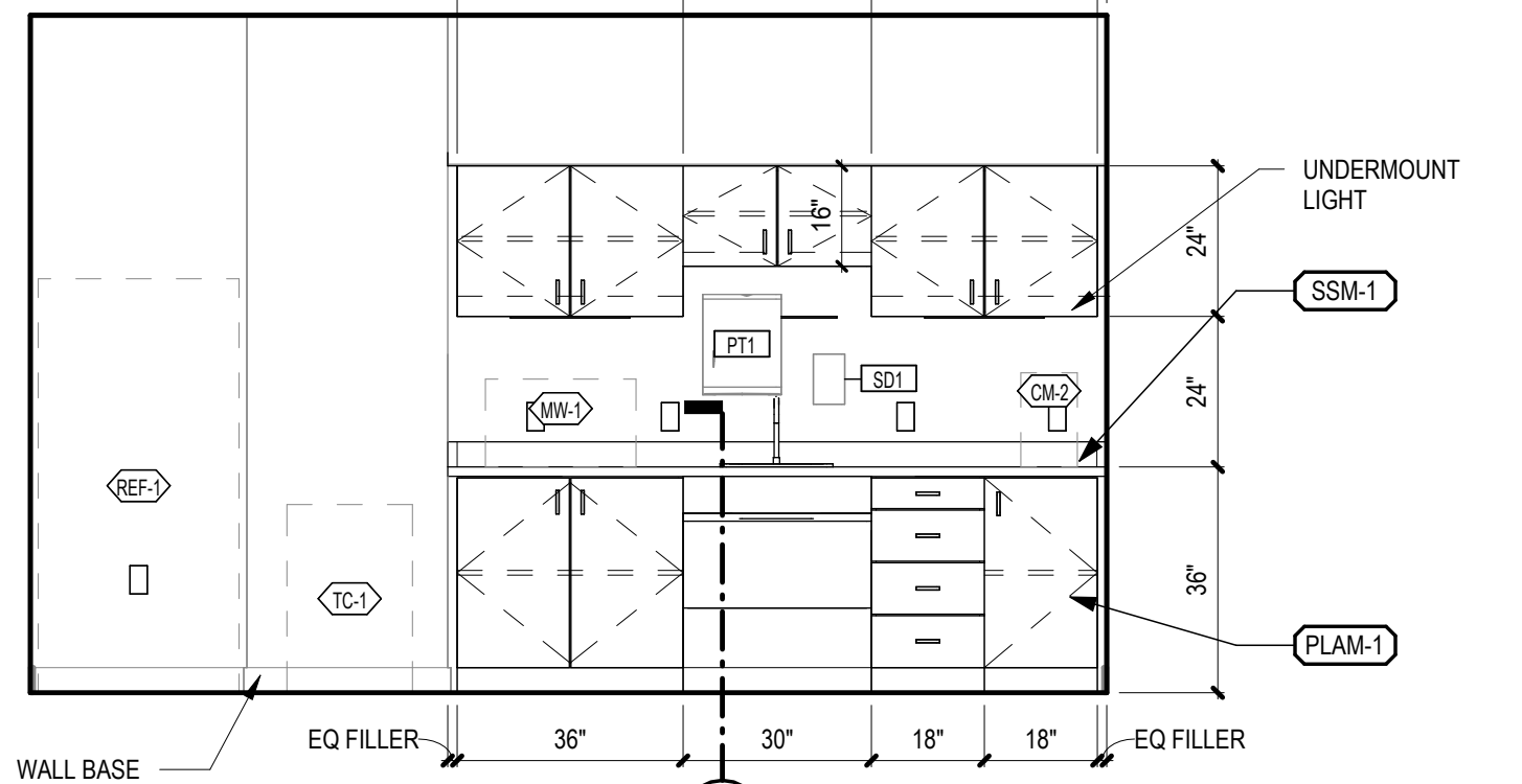
6 BREAK ROOM A2047 - WEST A-102.1C 3/8" = 1'-0"
