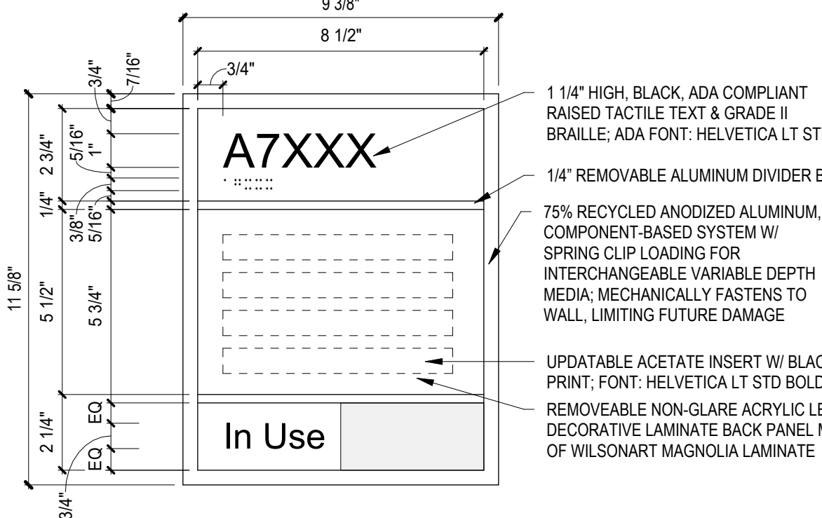
IN-07.01A ADA ROOM ID W/ SLIDER UNIT NOT TO SCALE
