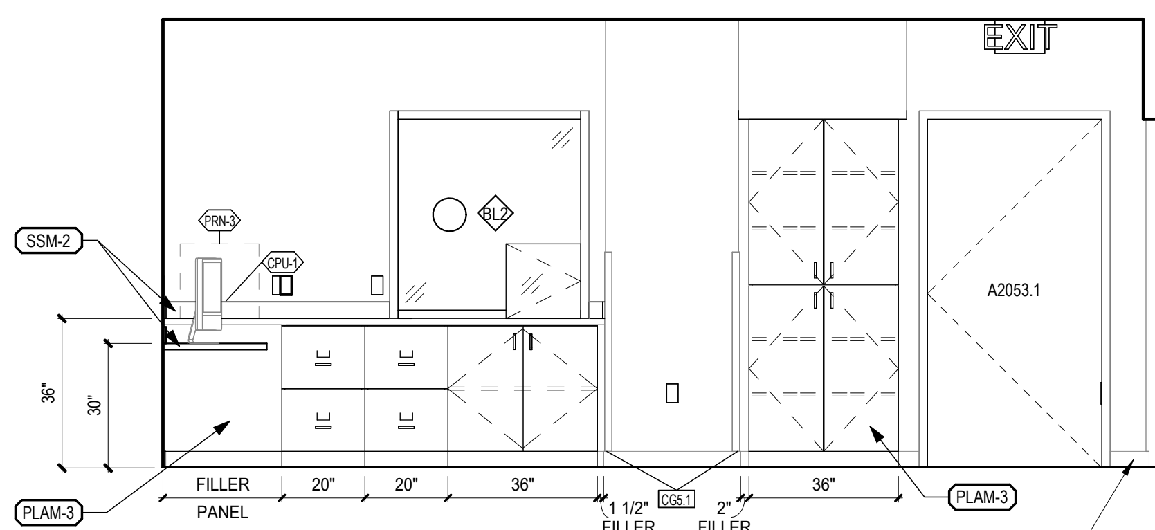
9 PHARMACIST WORK AREA A2053 - EAST A-132 3/8" = 1'-0"
