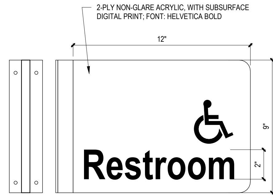
IN-13.01A RESTROOM NOT TO SCALE
