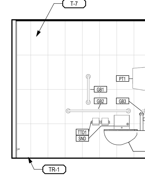
8 STAFF TOILET A2045 - NORTH A-102.1C 3/8" = 1'-0"
