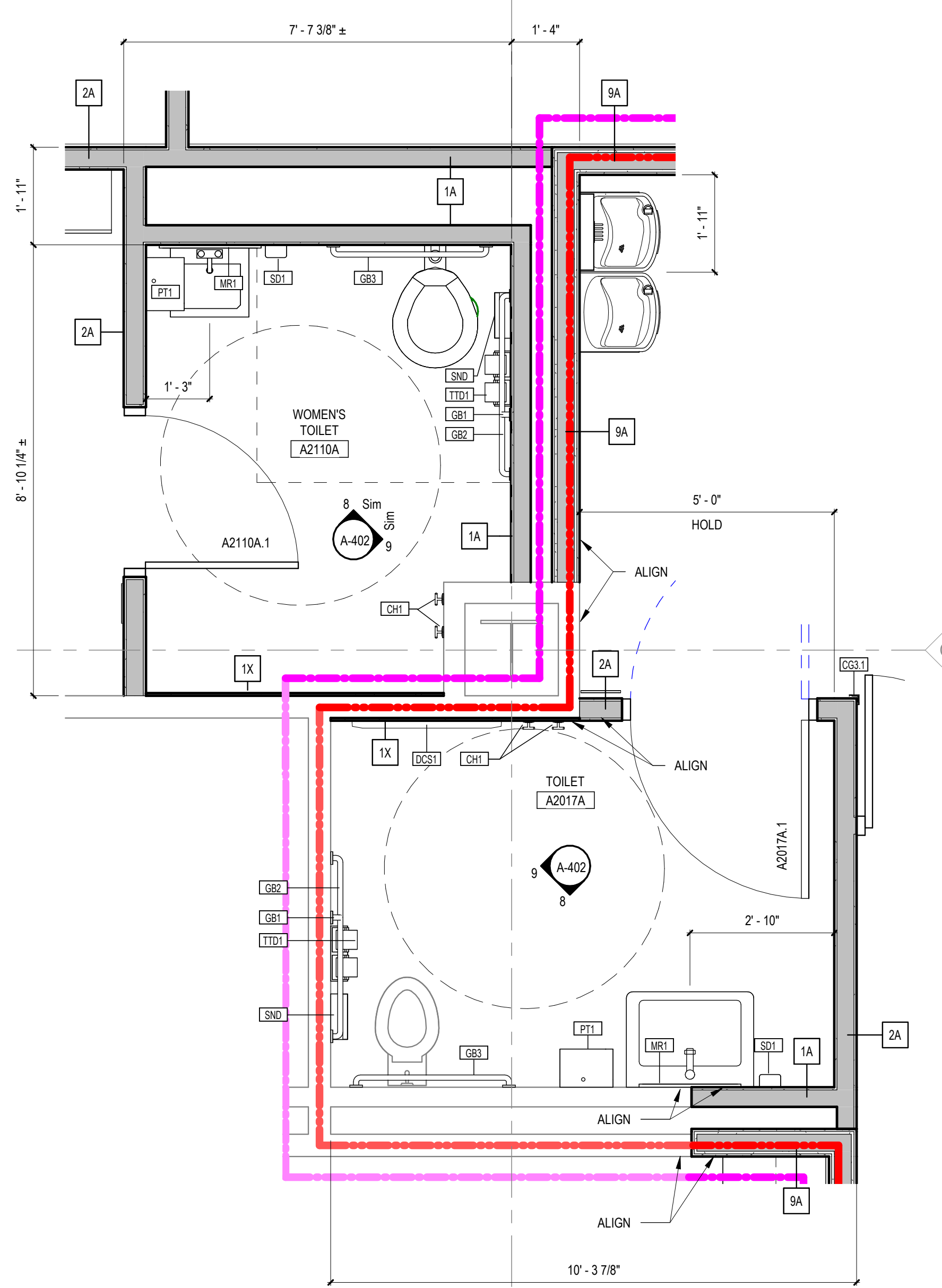
2 TOILET ROOMS - A2110A & A2017A
