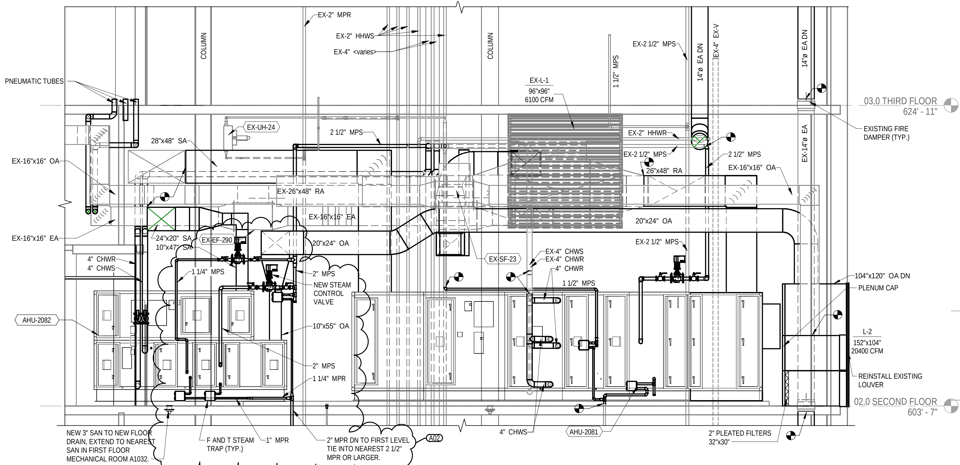
SECTION - MECHANICAL ROOM A2032 M-402/ 1/4" = 1'-0"
