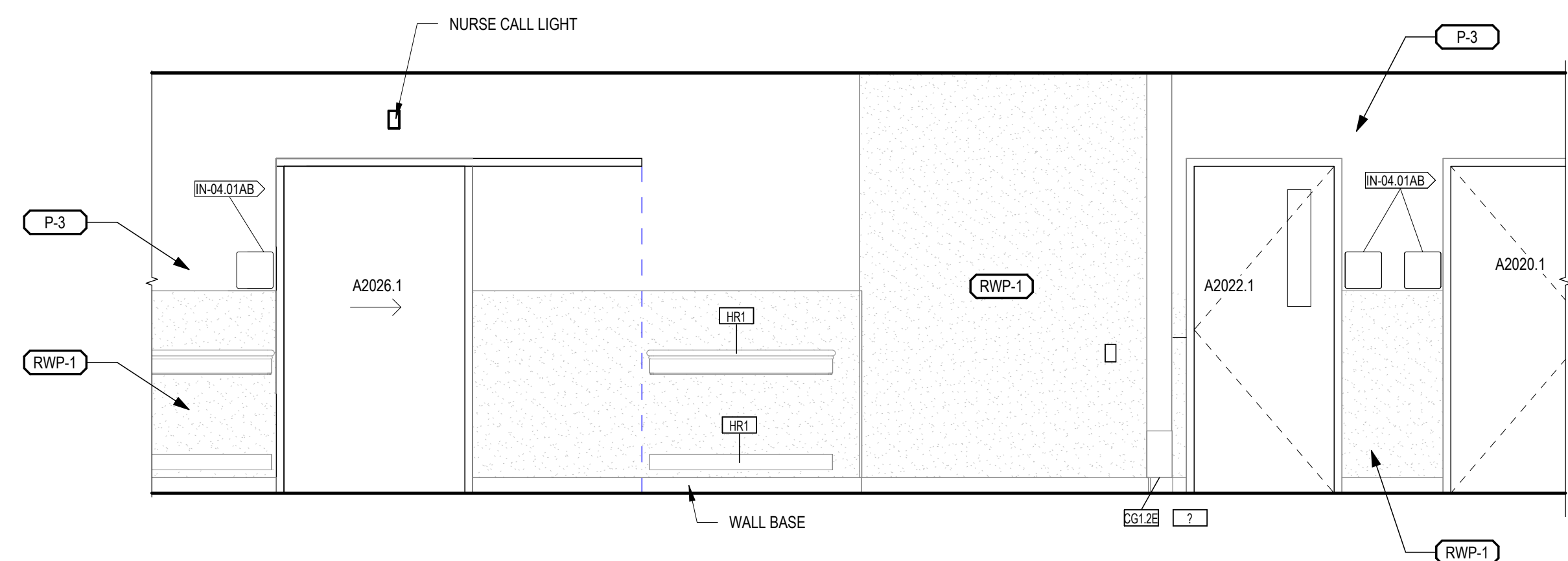
17 CORRIDOR CA213 - SOUTH A-102.1B 3/8" = 1'-0"
