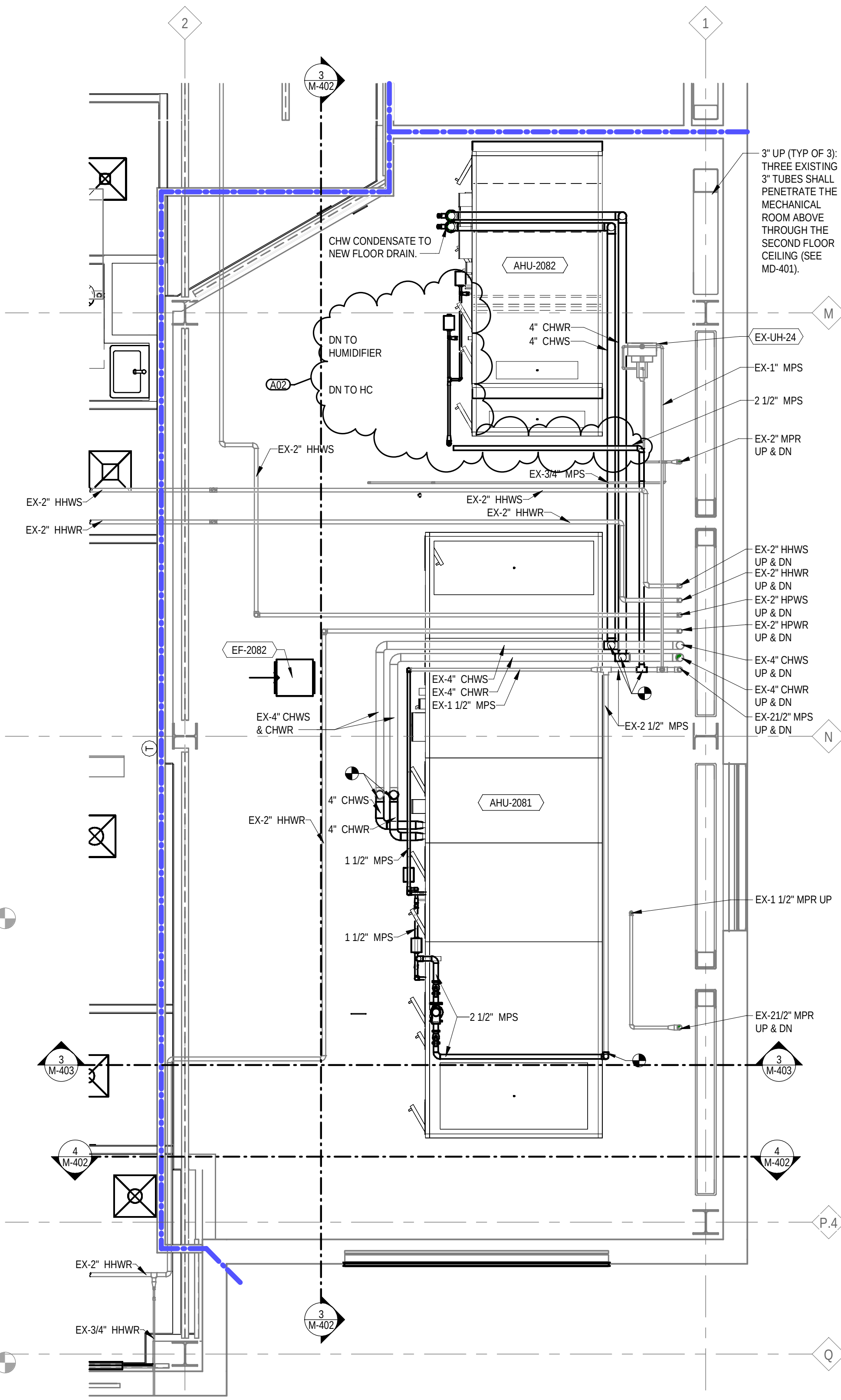
ENLARGED MECHANICAL ROOM A2032 PIPING PLAN MP102/ 1/4" = 1'-0"
