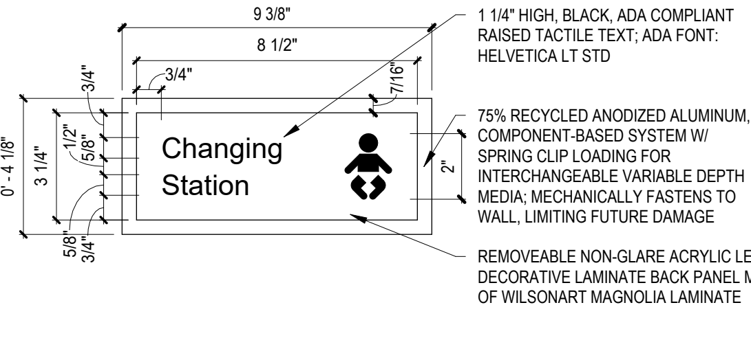
IN-09.07 CHANGING STATION ID NOT TO SCALE
