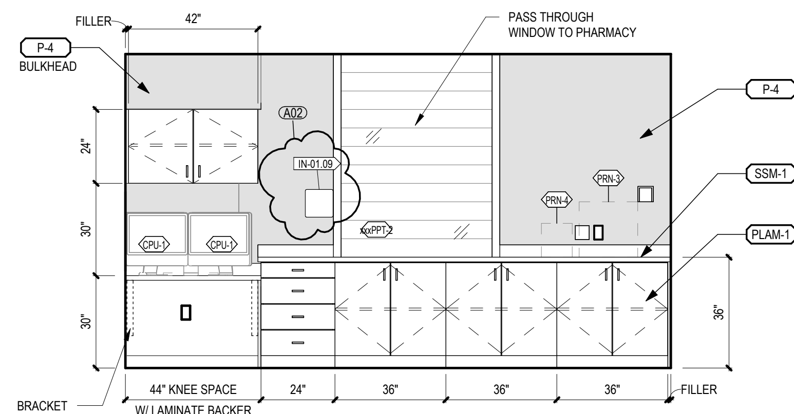
6 NURSE STATION INTERIOR A2075 - WEST 2 A-102.1C 3/8" = 1'-0"
