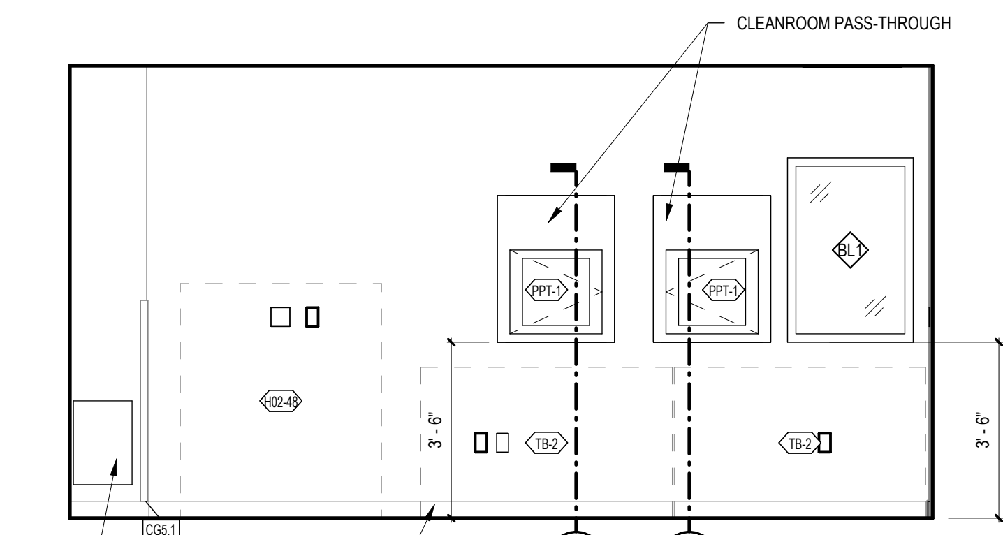
12 STERILE HAZARDOUS DRUG BUFFER ROOM A2057 - EAST A-132 3/8" = 1'-0"
