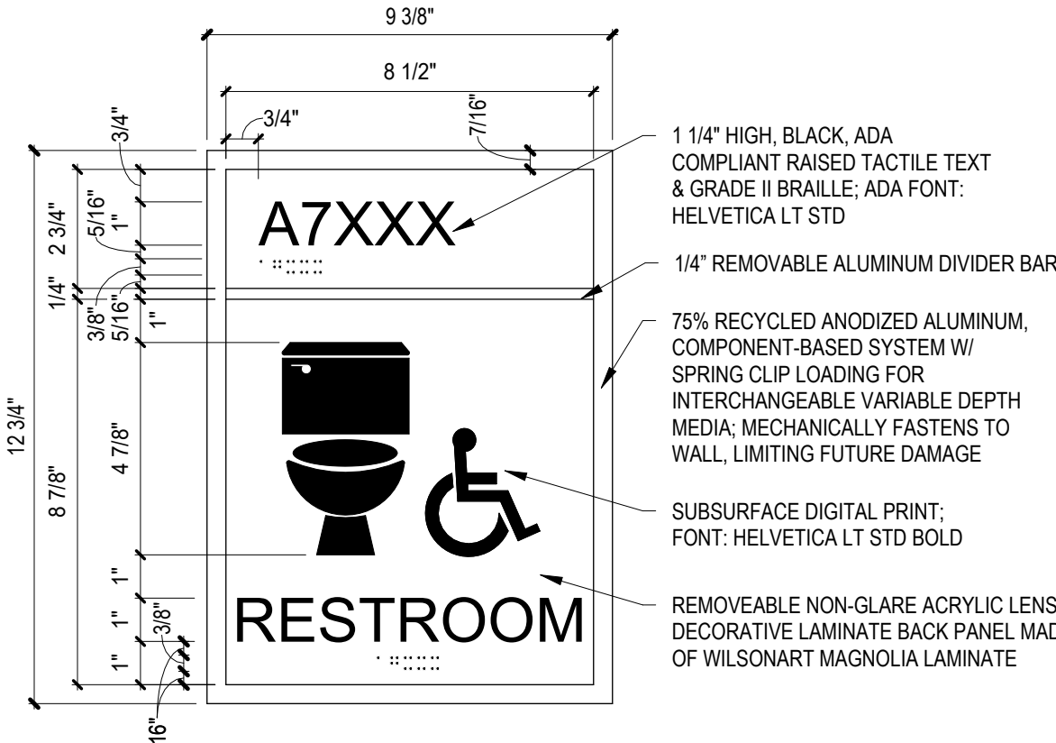
IN-09.03 ADA RESTROOM NOT TO SCALE
