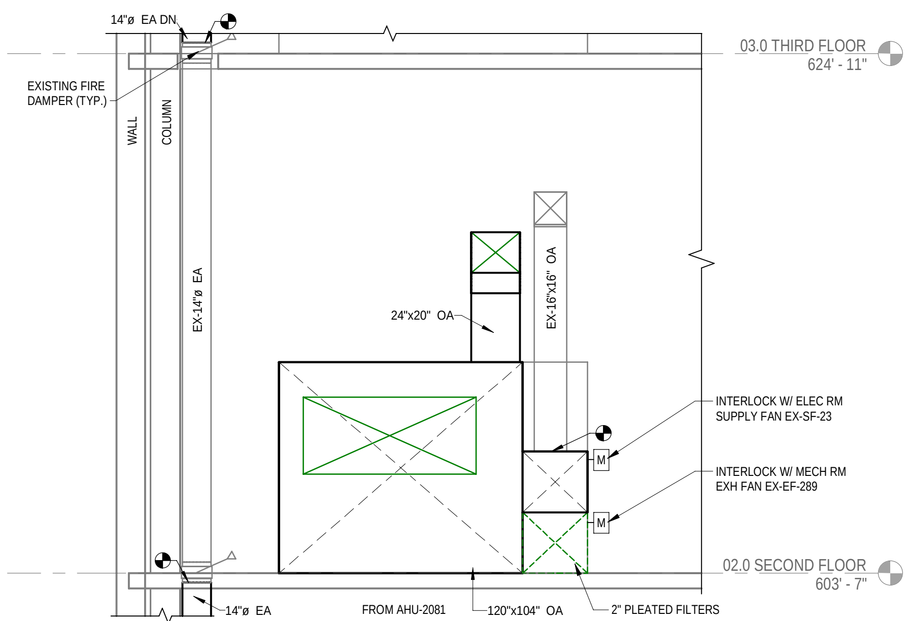
SECTION - AHU-2081 AIR INTAKE M-402/ 1/4" = 1'-0"
