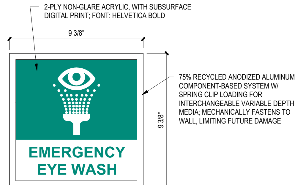
IN-01.38 EMERGENCY EYEWASH NOT TO SCALE
