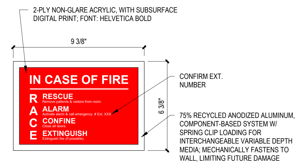
IN-01.03 IN CASE OF FIRE NOT TO SCALE
