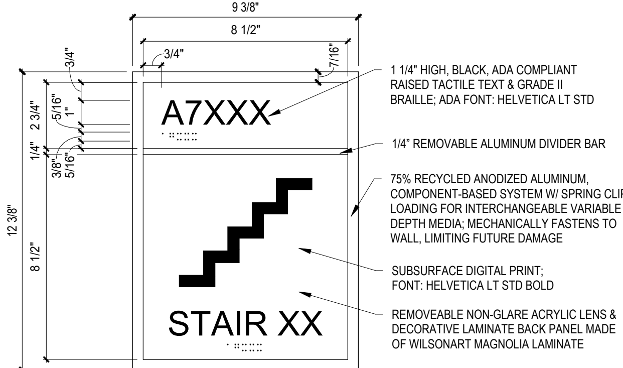
IN-01.10 ADA STAIRWELL NOT TO SCALE
