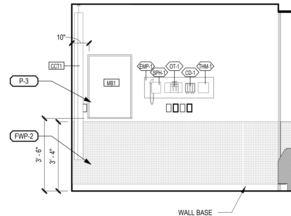
15 EXAM A2038 - EAST A-102.1A 3/8" = 1'-0"
