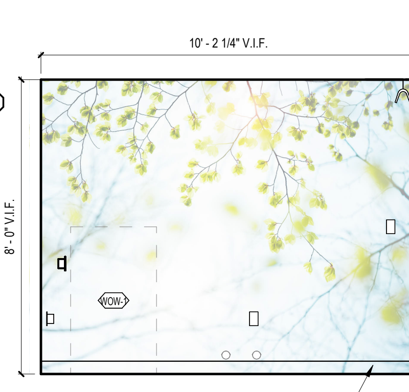
2 NURSE STATION INTERIOR A2075 - WEST 1 A-102.1C 3/8" = 1'-0"
