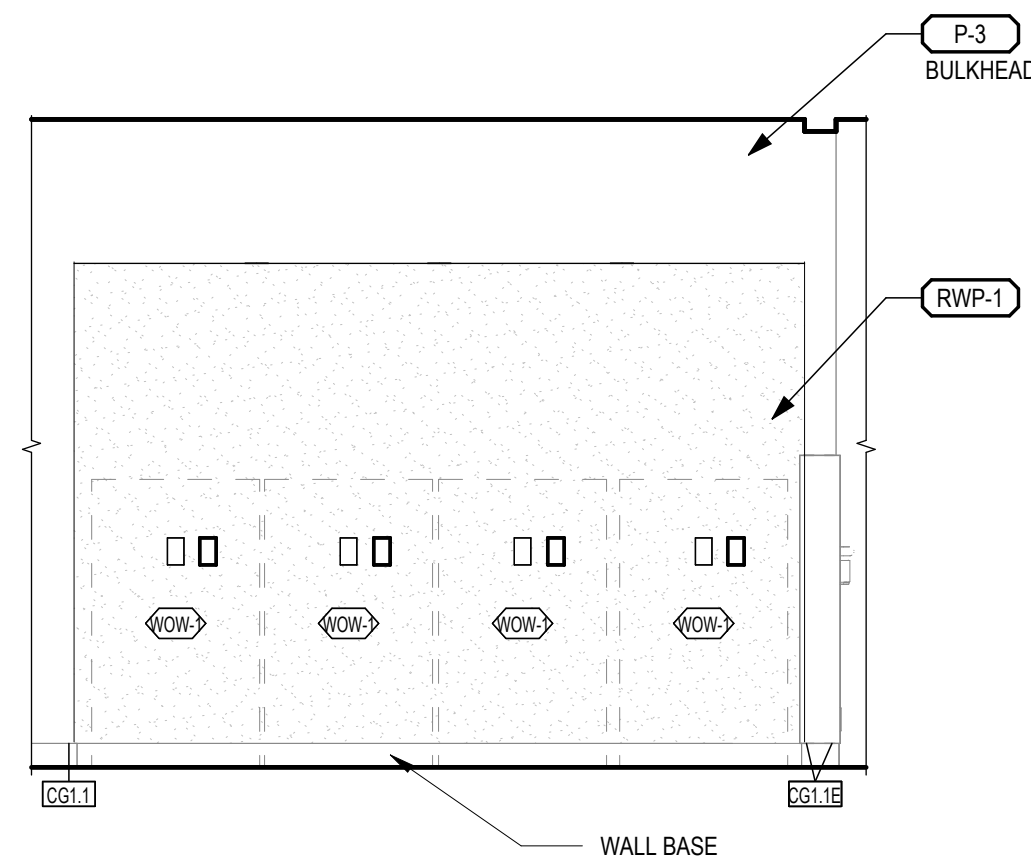
16 ALCOVE A2044 - WEST A-102.1C 3/8" = 1'-0"
