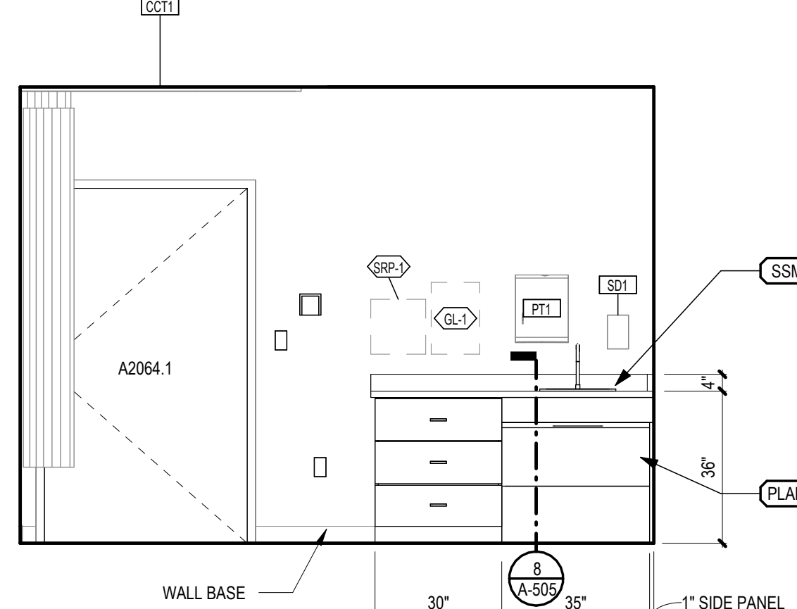
2 INFUSION ROOM A2064 - EAST A-102.1A 3/8" = 1'-0"
