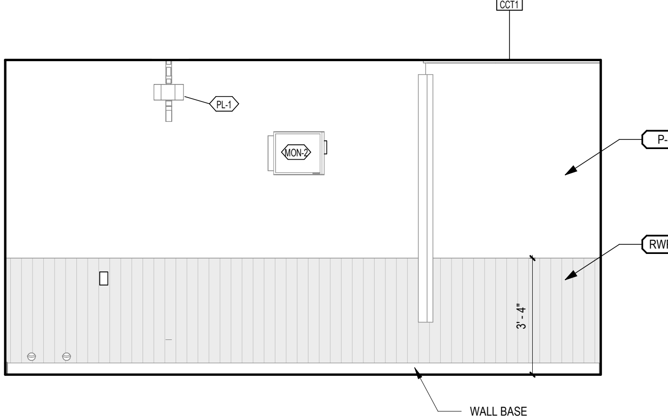
1 INFUSION ROOM A2064 - NORTH A-102.1A 3/8" = 1'-0"
