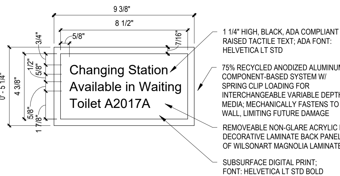
IN-09.08A CHANGING STATION ID NOT TO SCALE
