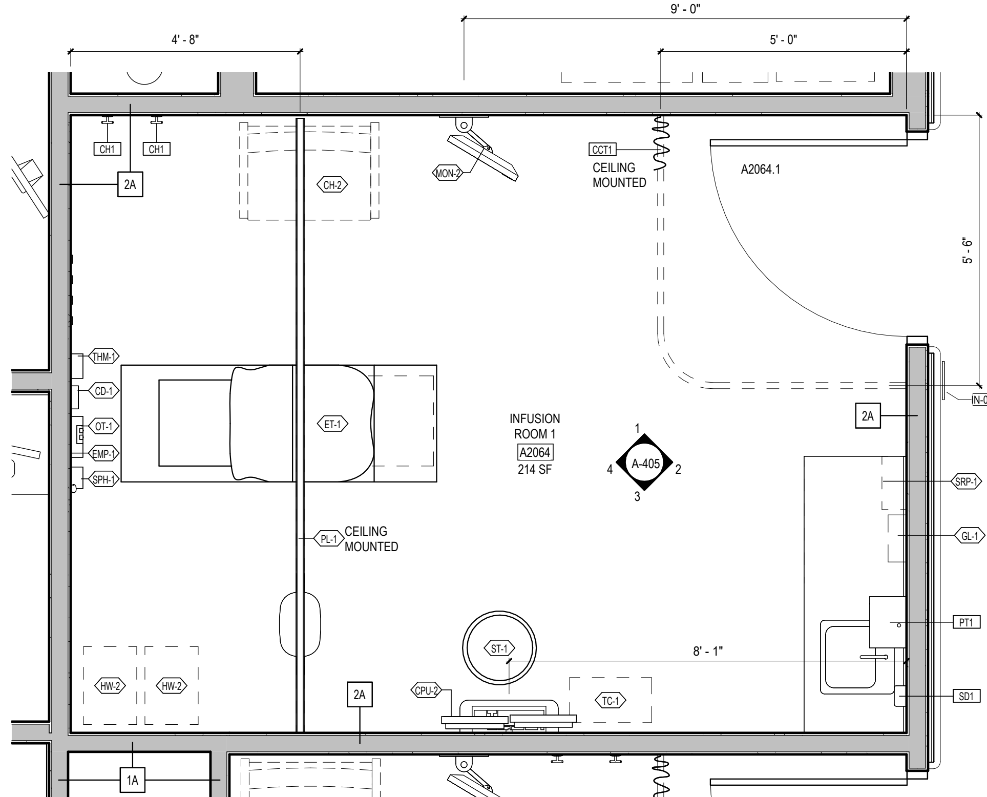
4 INFUSION ROOM 1 - A2064
