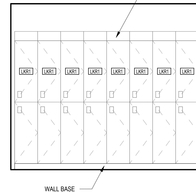
7 LOCKER ROOM A2047A - NORTH A-102.1C 3/8" = 1'-0"
