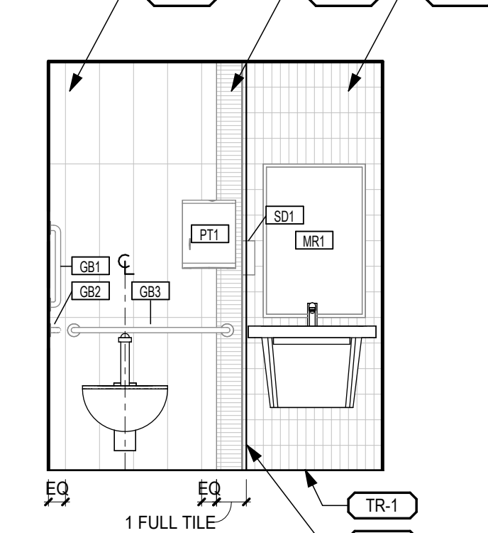
9 STAFF TOILET A2045 - EAST A-102.1C 3/8" = 1'-0"
