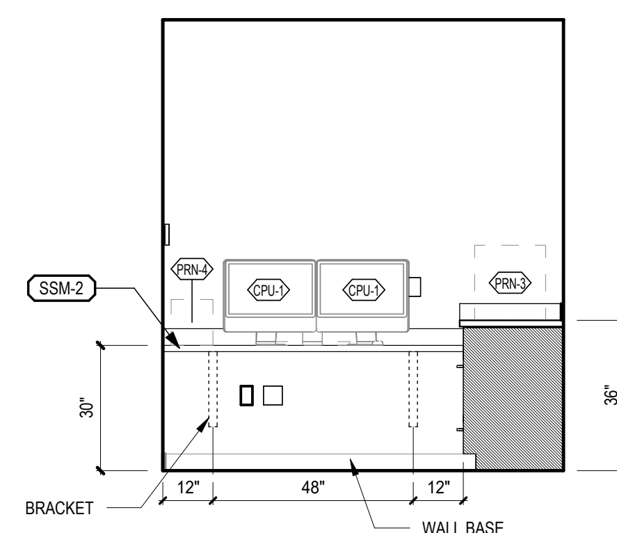
8 PHARMACIST WORK AREA A2053 - NORTH A-132 3/8" = 1'-0"
