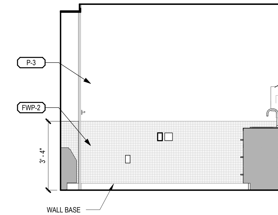
16 EXAM A2038 - WEST A-102.1A 3/8" = 1'-0"
