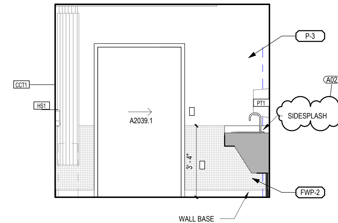
12 EXAM A2039 - SOUTH A-102.1A 3/8" = 1'-0"
