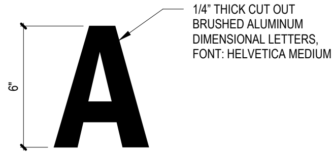
IN-19.03 GRAPHIC TEXT - METAL NOT TO SCALE
