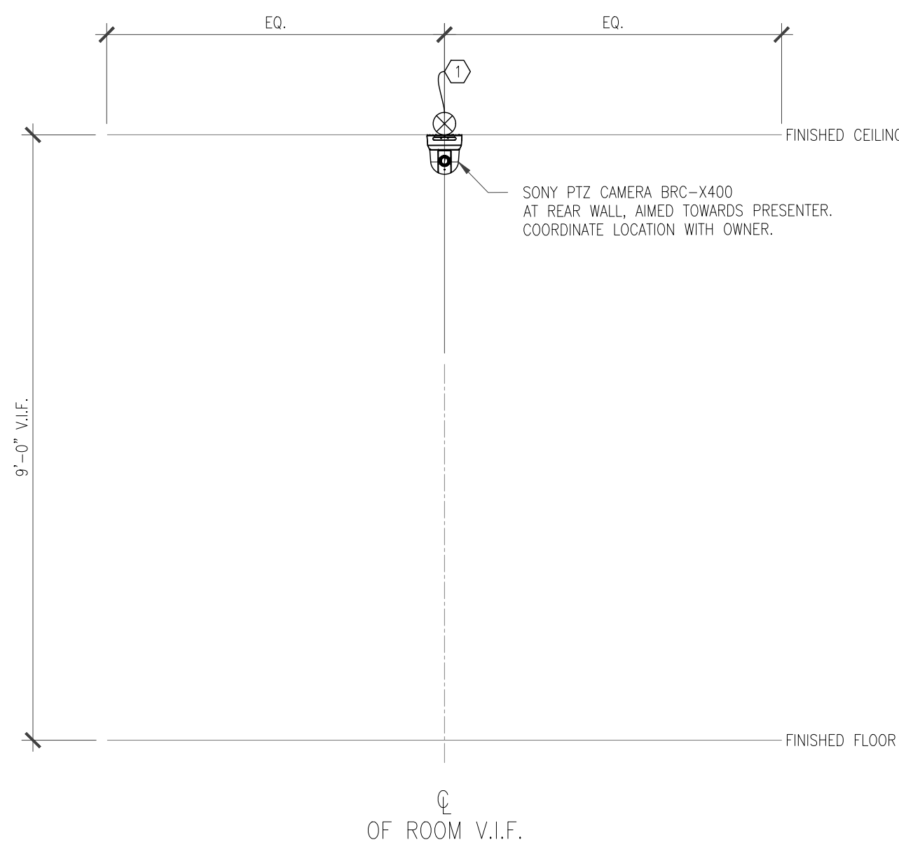
D EDUCATION BLDG RM 1-6 - AV EQUIPMENT ELEVATION SCALE: 1/2" = 1'-0" - TYP OF 6 PLACES
