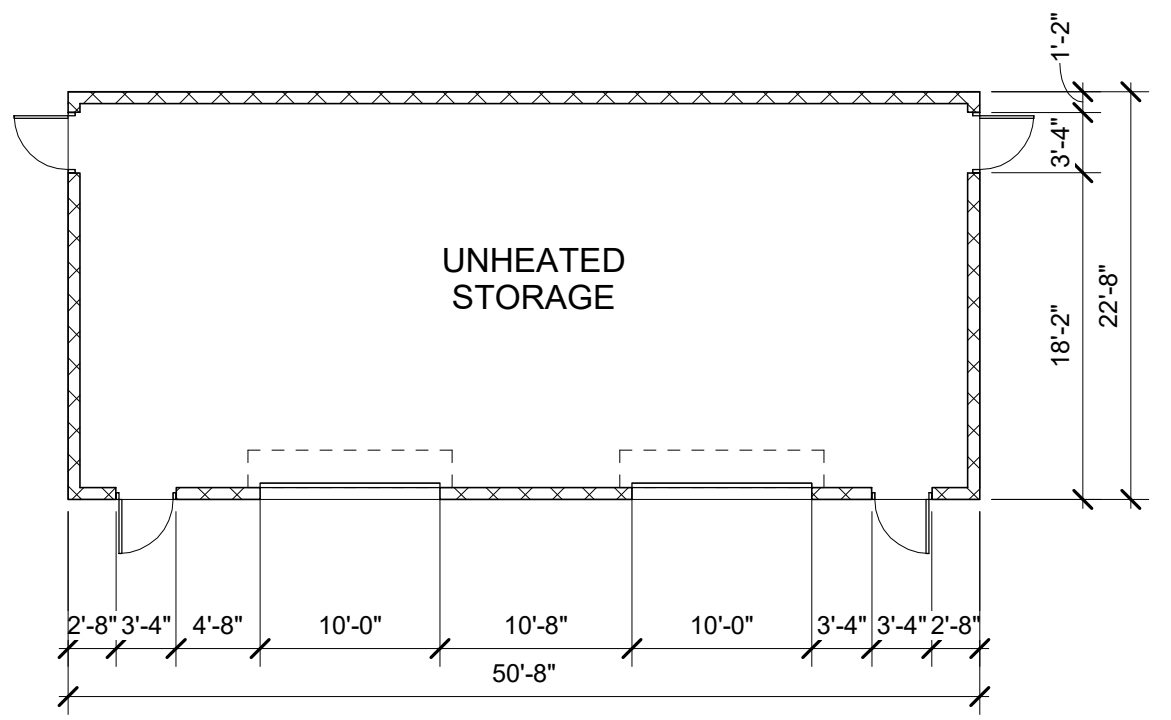
(A5) (BID OPTION) 1,000 SQ FT UNHEATED STORAGE BUILDING FLOOR PLAN SCALE 3/32" = 1'-0"
